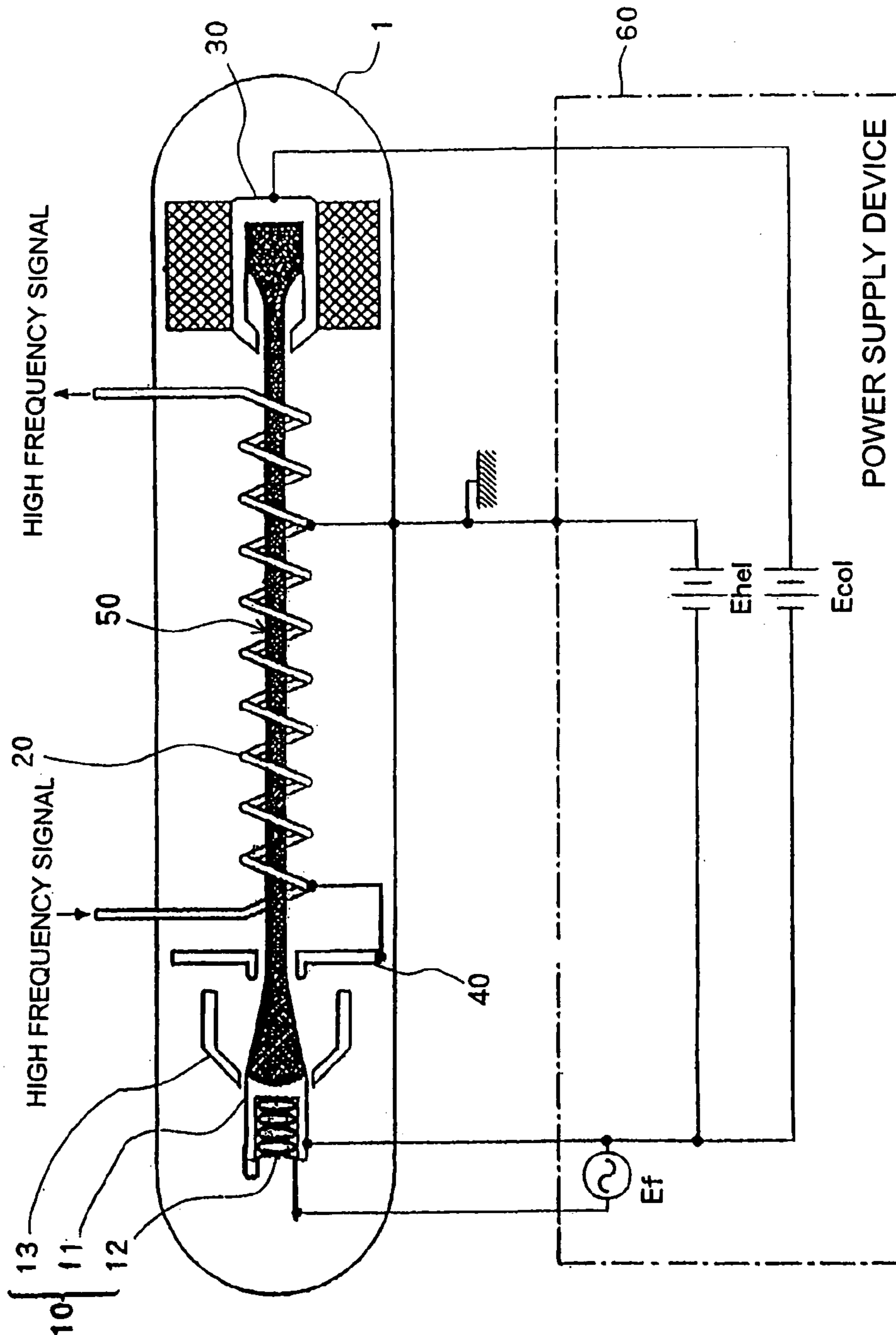
FIG. 1 (PRIOR ART)
