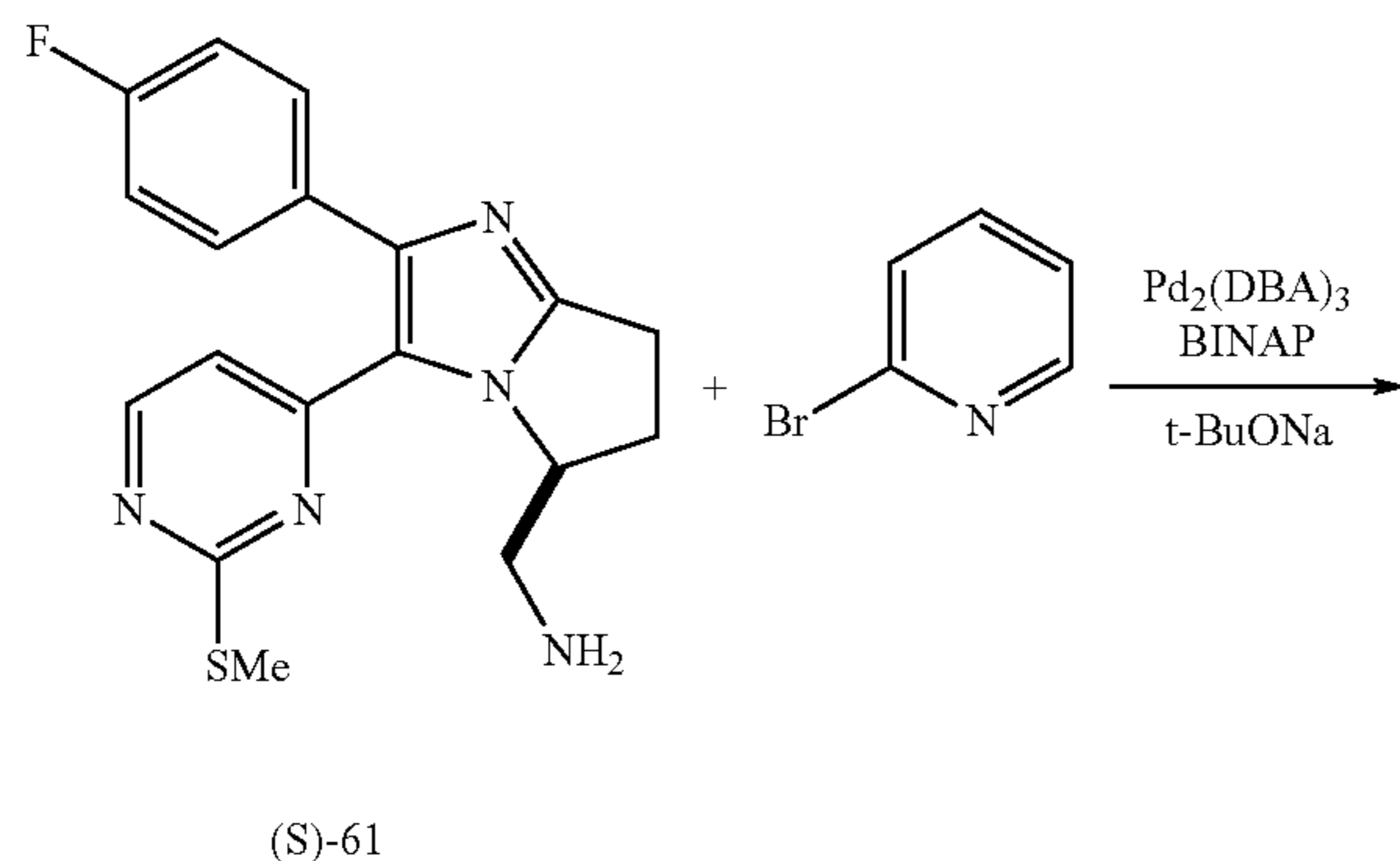
Scheme 18
