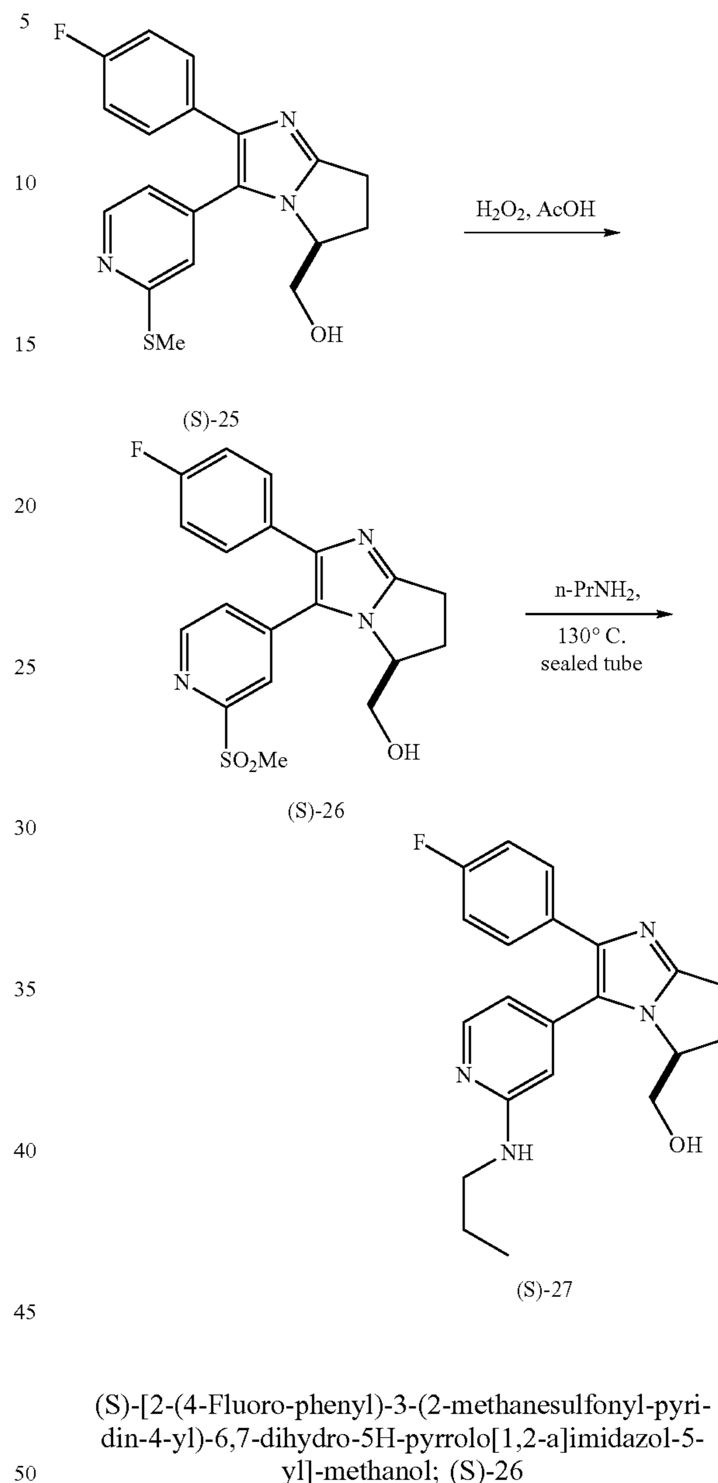
Scheme 6
