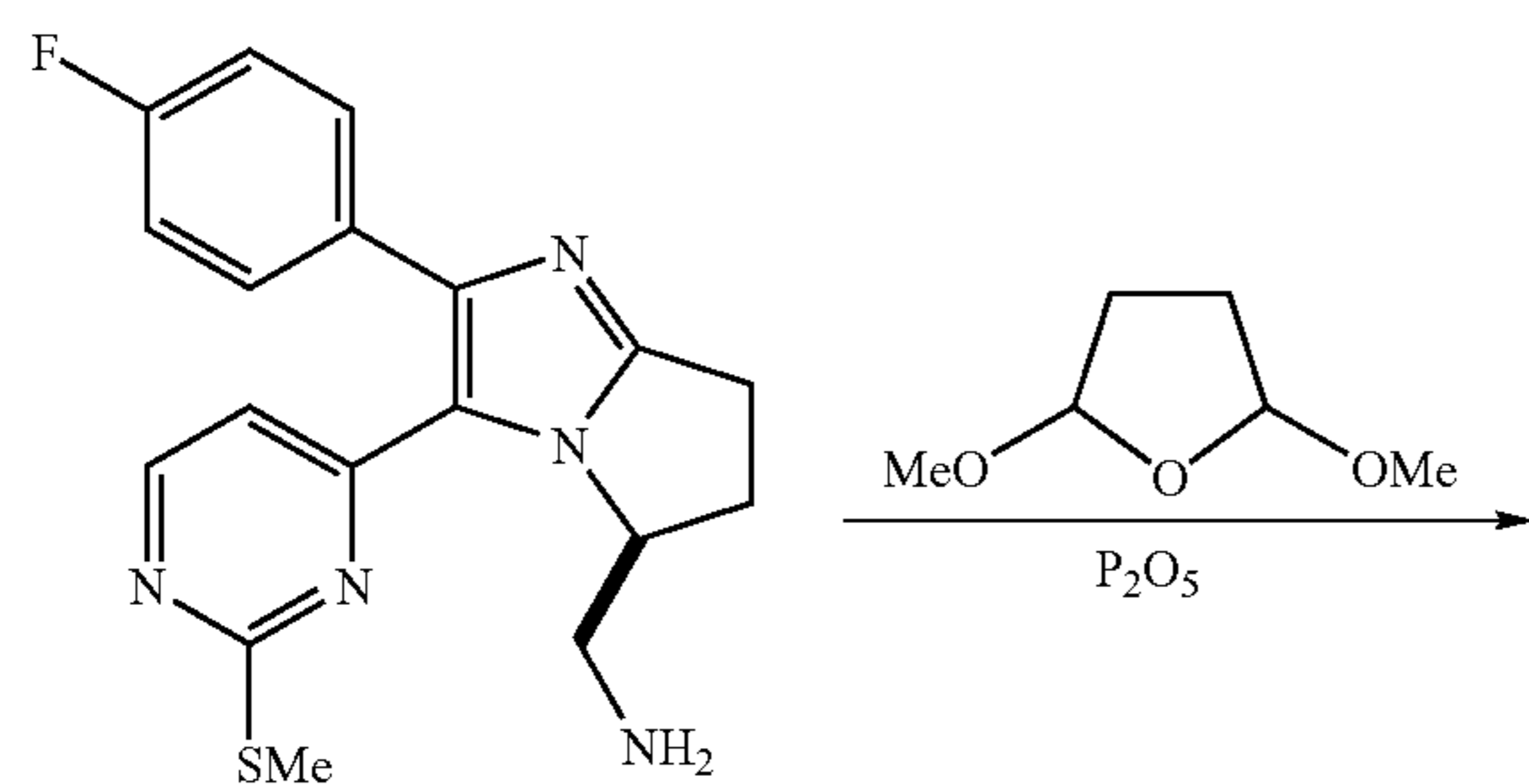
Scheme 19
