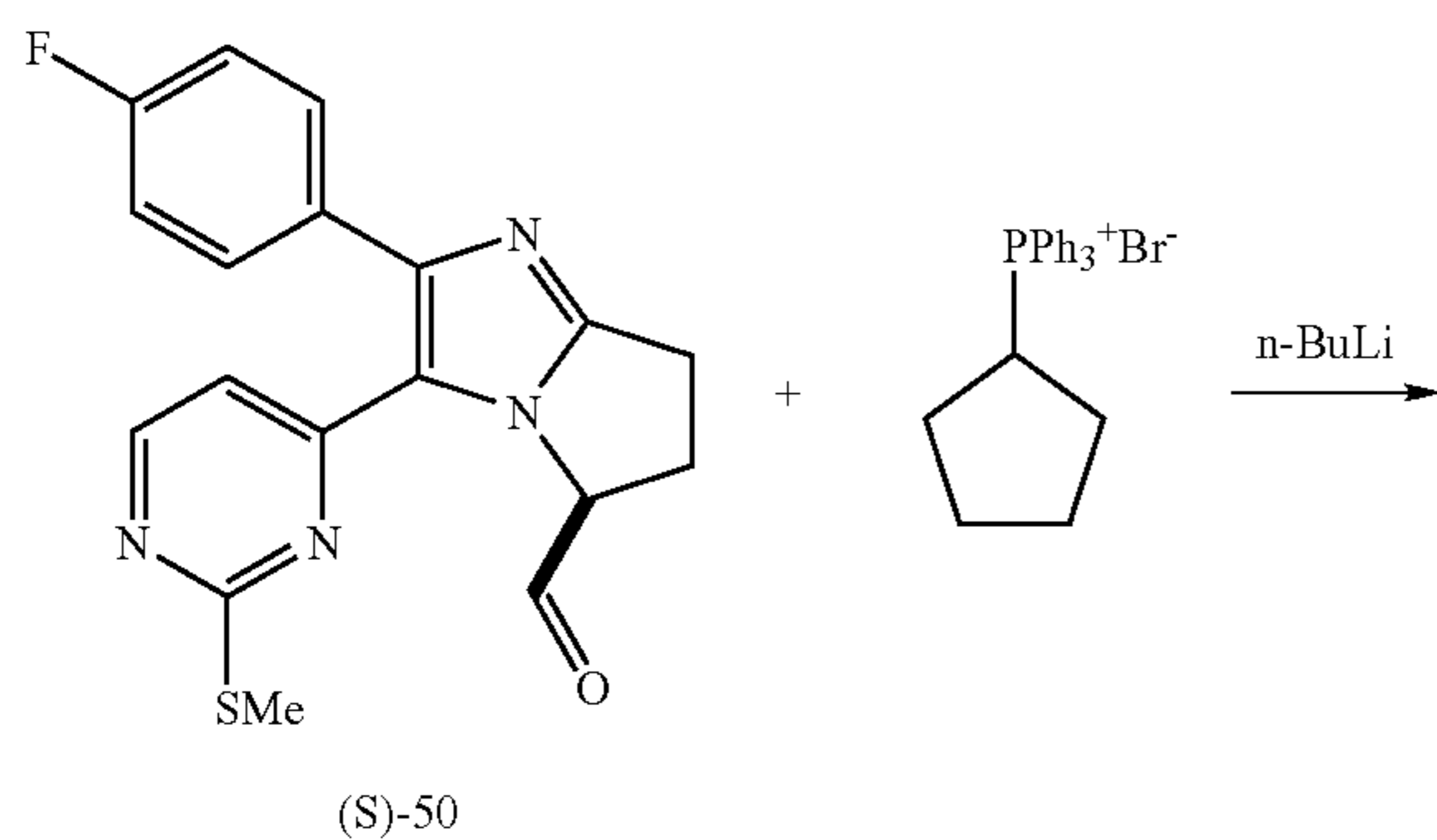
Scheme 20
