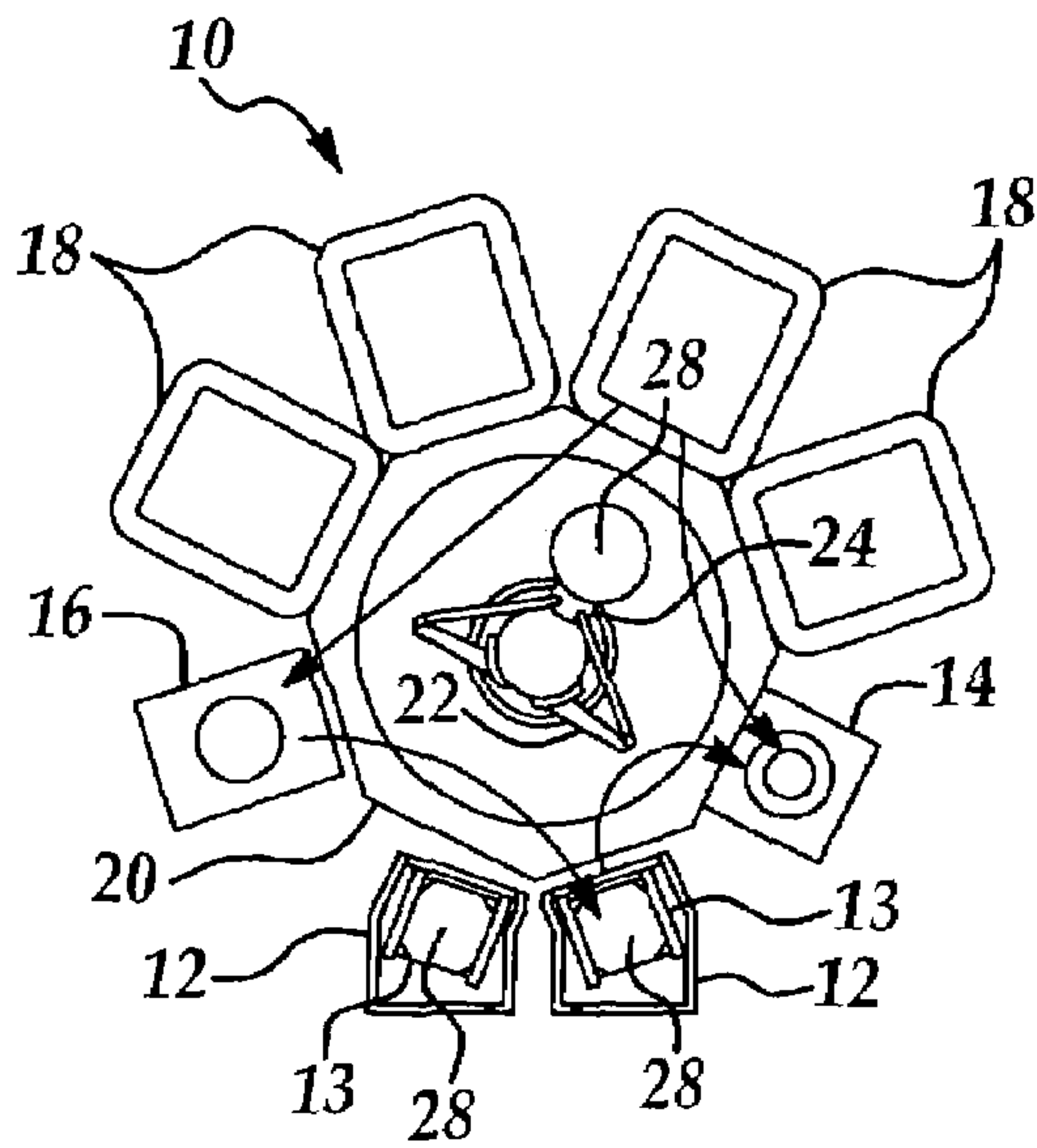
Figure 1 Prior Art
