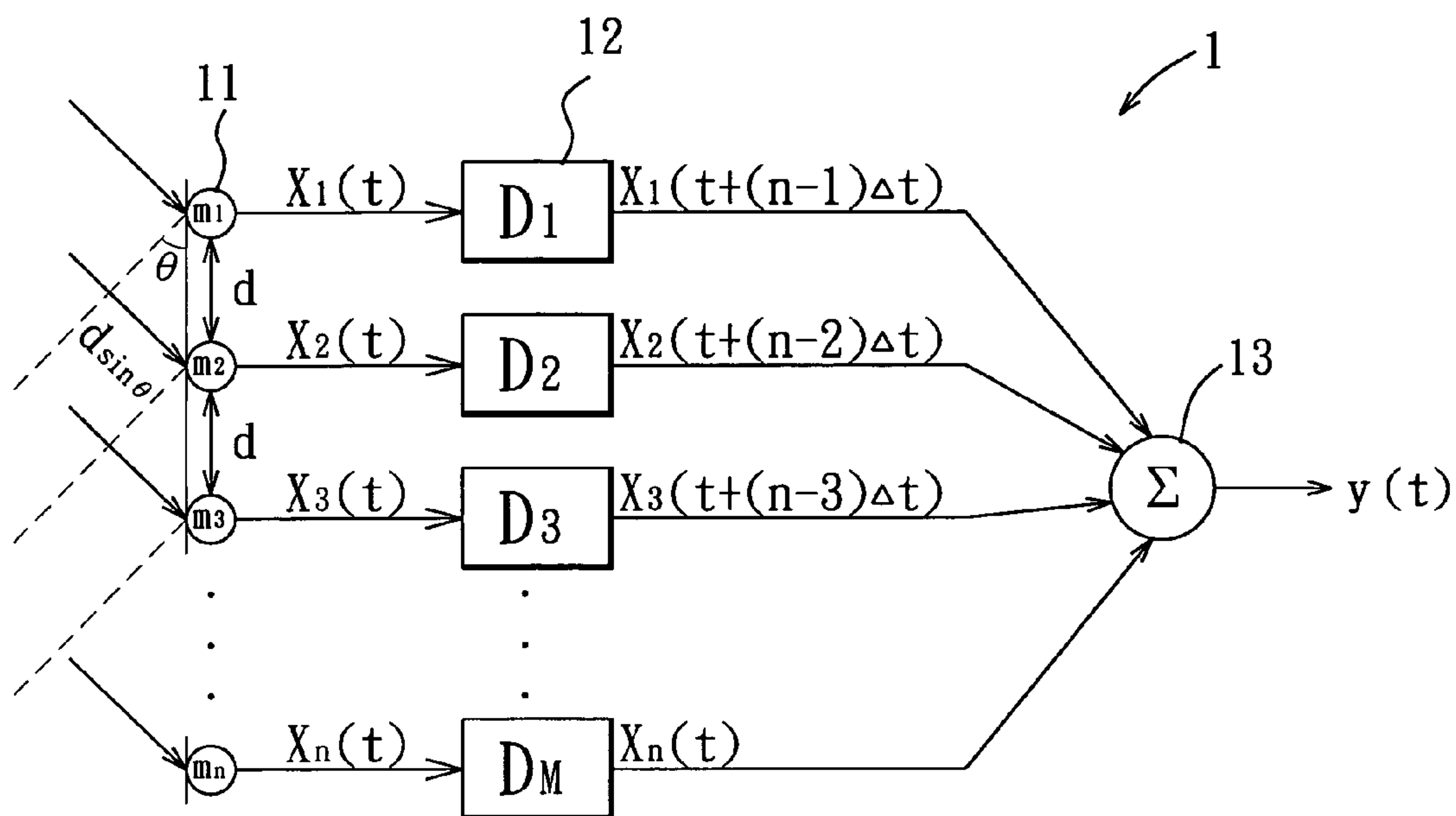
FIG. 1 PRIOR ART
