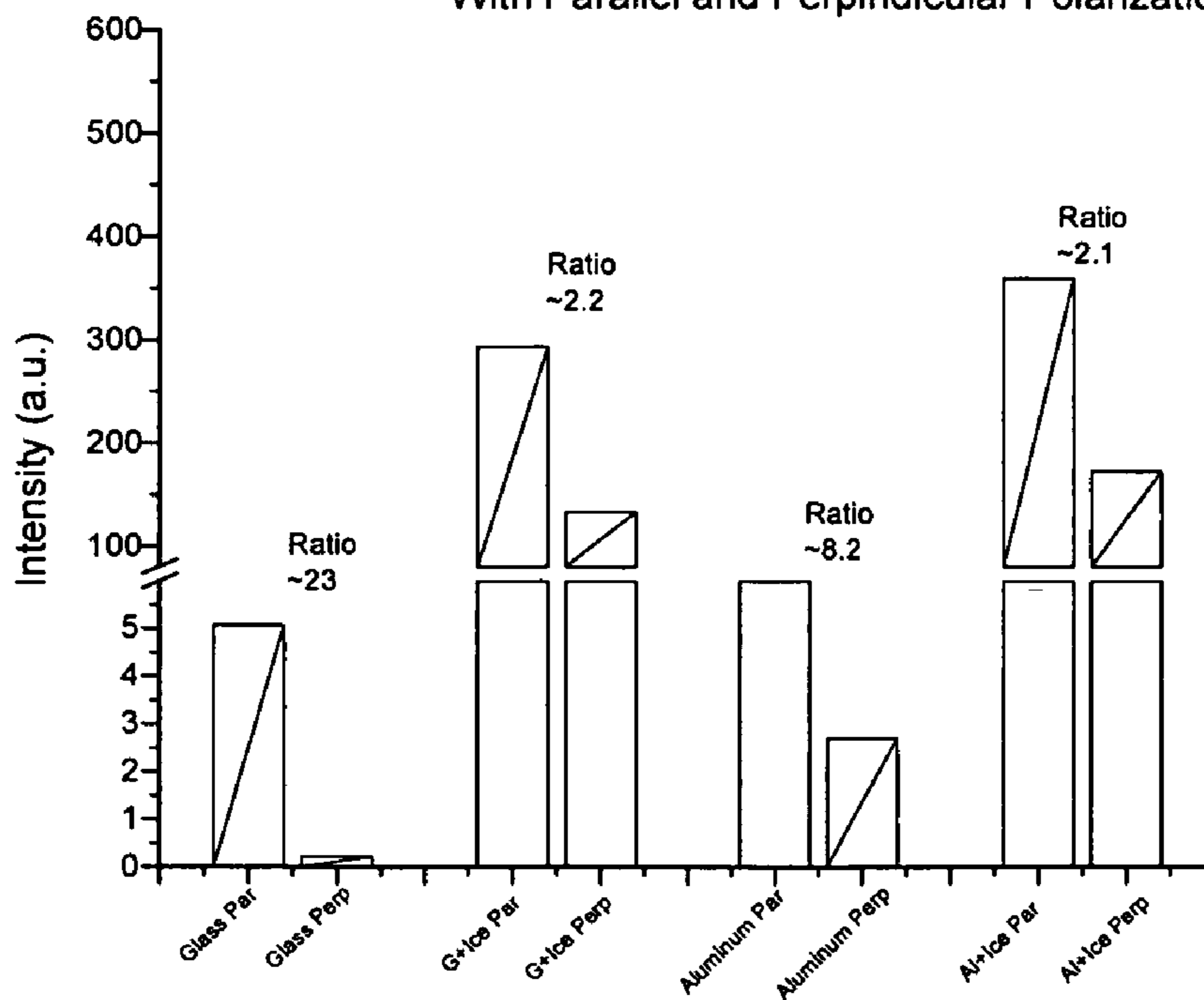
Scattering Intensity w/ and w/out Ice on Glass and Aluminum With Parallel and Perpendicular Polarization
