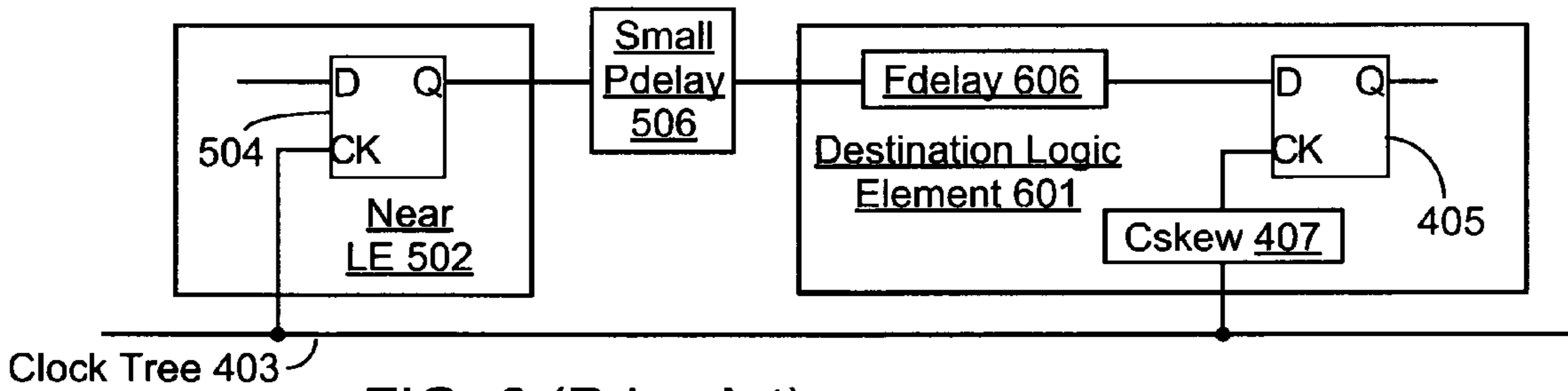
FIG. 6 (Prior Art): No Hold Time Violation
