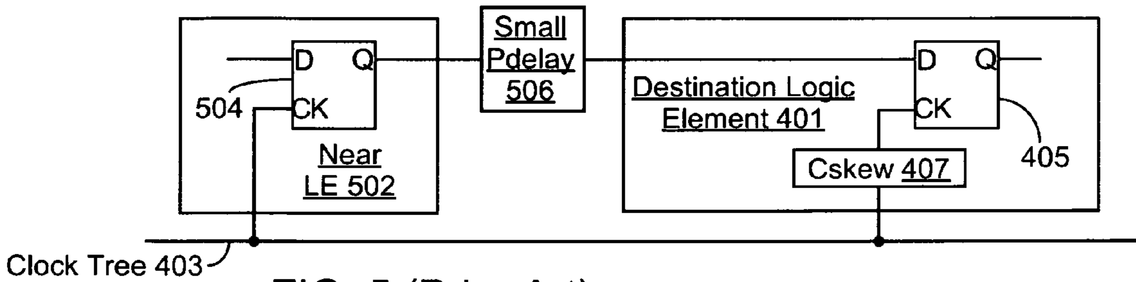
FIG. 5 (Prior Art): Hold Time Violation
