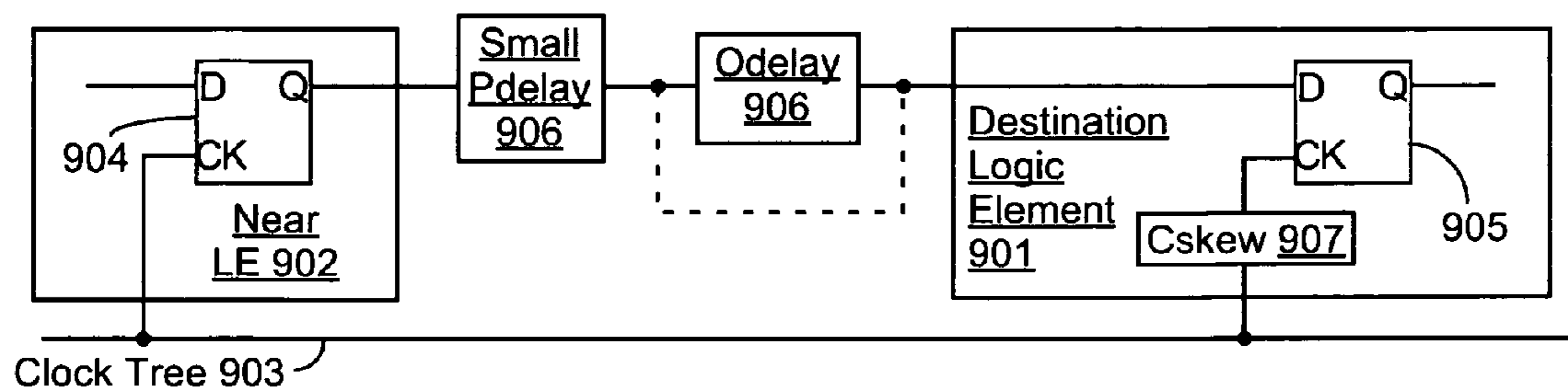
FIG. 9: Insert Delay, No Hold Time Violation
