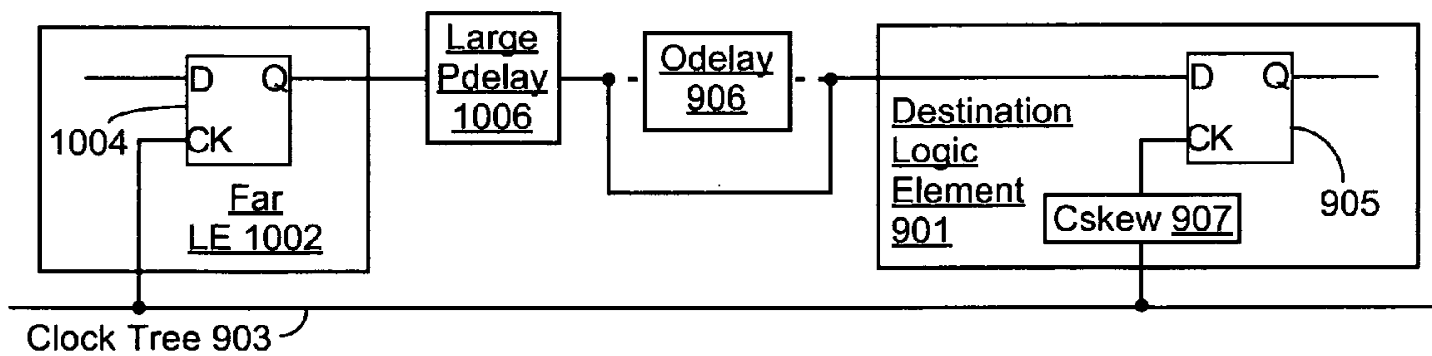
FIG. 10: Bypass Delay, No Large Setup Time
