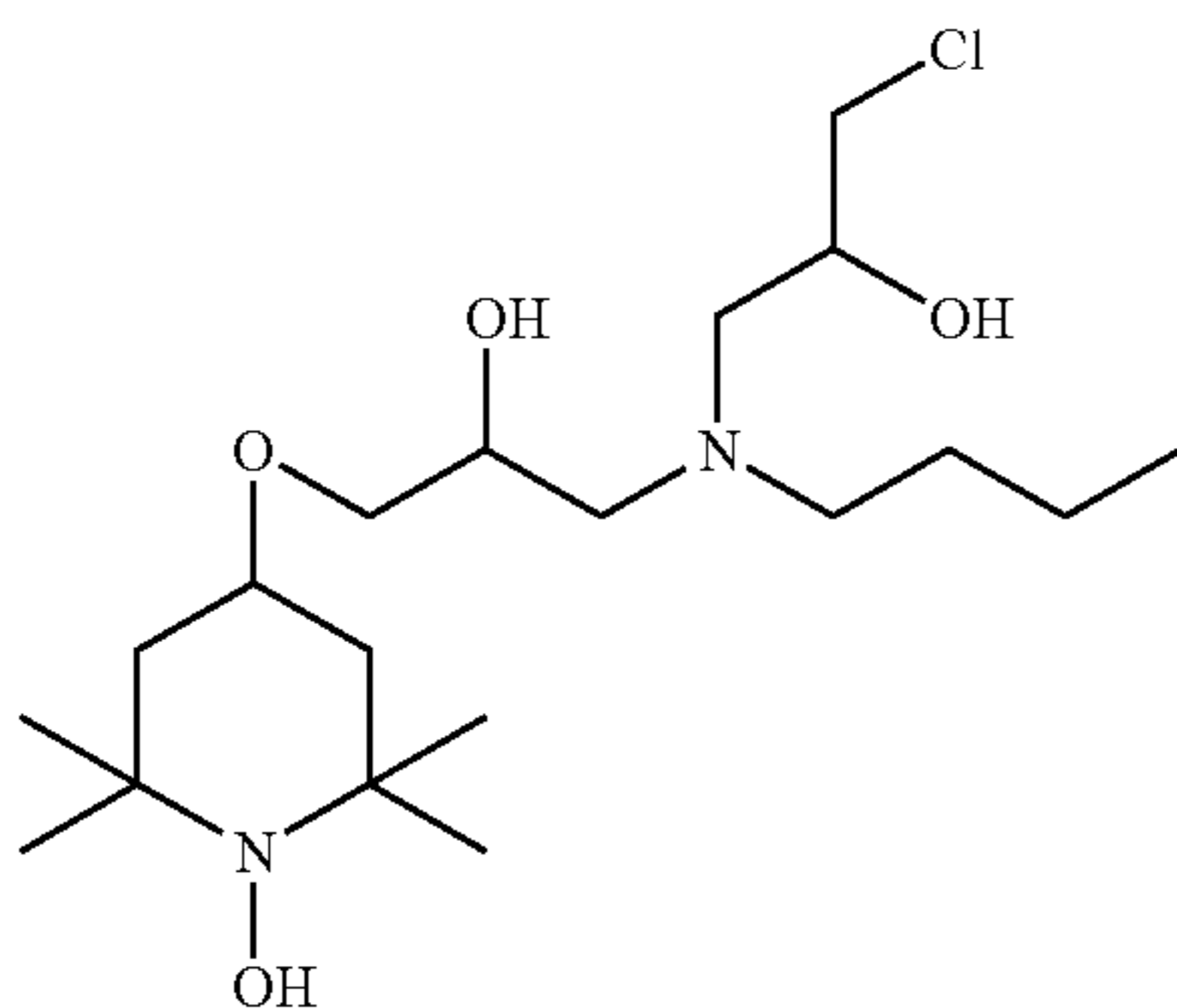
4-{3-[Butyl-(3-chloro-2-hydroxy-propyl)-amino]-2-hydroxy-propoxy}-2,2,6,6-tetramethyl-piperidin-1-ol
