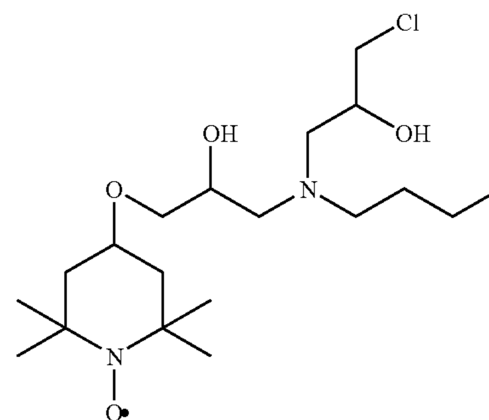
4-{3-[Butyl-(3-chloro-2-hydroxy-propyl)-amino]-2-hydroxy-propoxy}-2,2,6,6-tetramethyl-piperidin-1-oxyl
