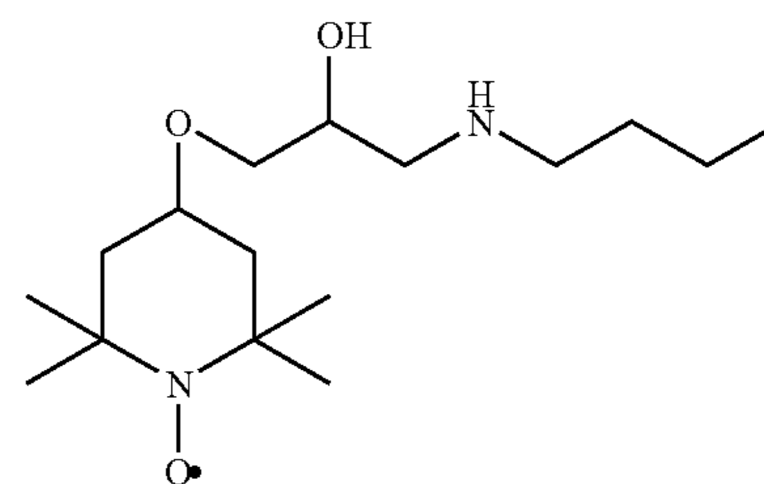
4-(3-Butylamino-2-hydroxy-propoxy)-2,2,6,6-tetramethyl-piperidin-1-oxyl
