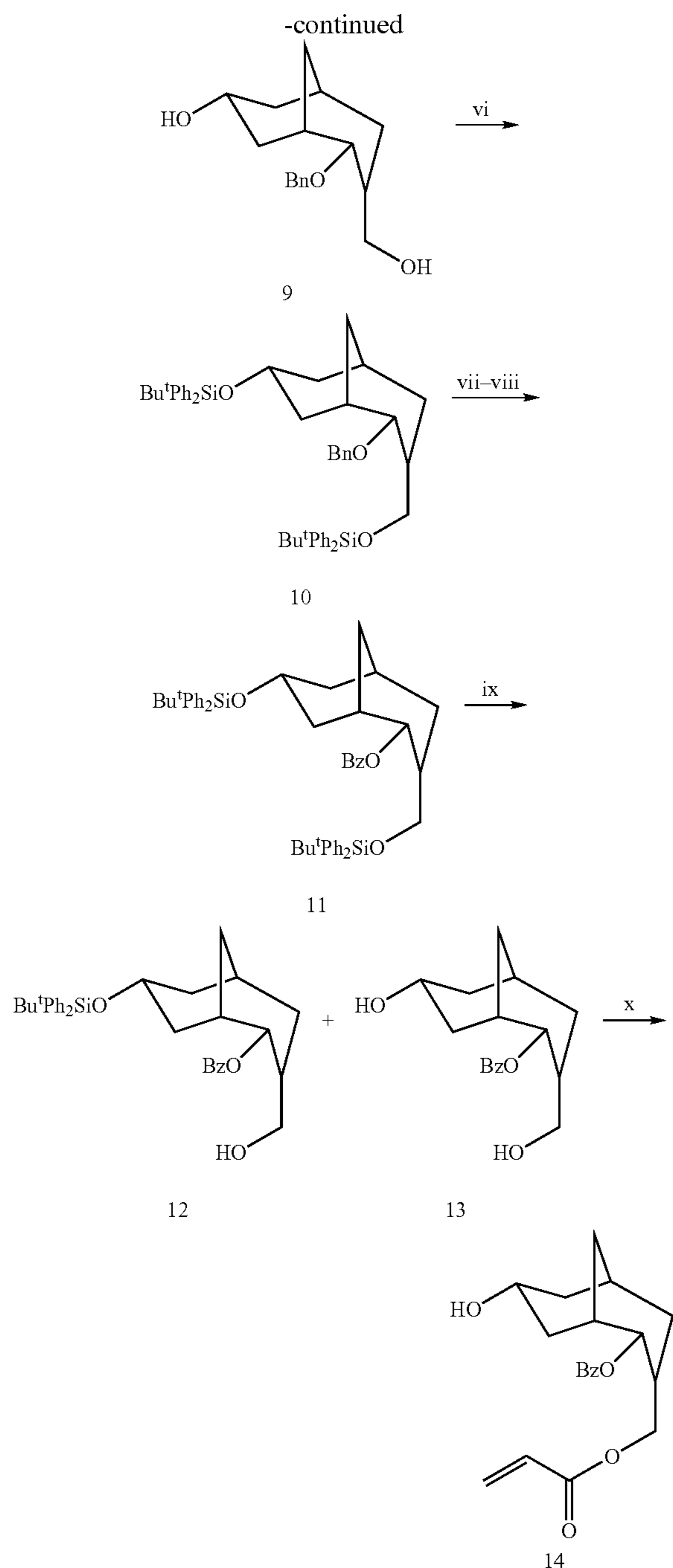
Scheme 1: Reagents and conditions: i. \text{NaN}_3 , \text{H}_2\text{SO}_4 , \text{Ac}_2\text{O} , (57%). ii. \text{KOH} , THF (85%). iii. \text{NaH} , \text{BnBr} , THF (95%). iv. \text{Ac}_2\text{O} , \text{AcOH} , \text{H}_2\text{O}_2 (77%). v. \text{LAH} , THF (76%). vi. \text{TBDPSCl} , Imidazole, DMF, (92%). vii. \text{Pd}(\text{OH})_2/\text{C} , 50Psi, 24 h, THF, (90%), viii. \text{BzCl} , \text{Et}_3\text{N} , DMAP, \text{CH}_2\text{Cl}_2 (95%) based on SM recovered. ix. \text{HF} -Pyridine, THF, 0^\circ\text{C} -RT, (70%). x. \text{LHMDS} , Acryloyl chloride, THF.
