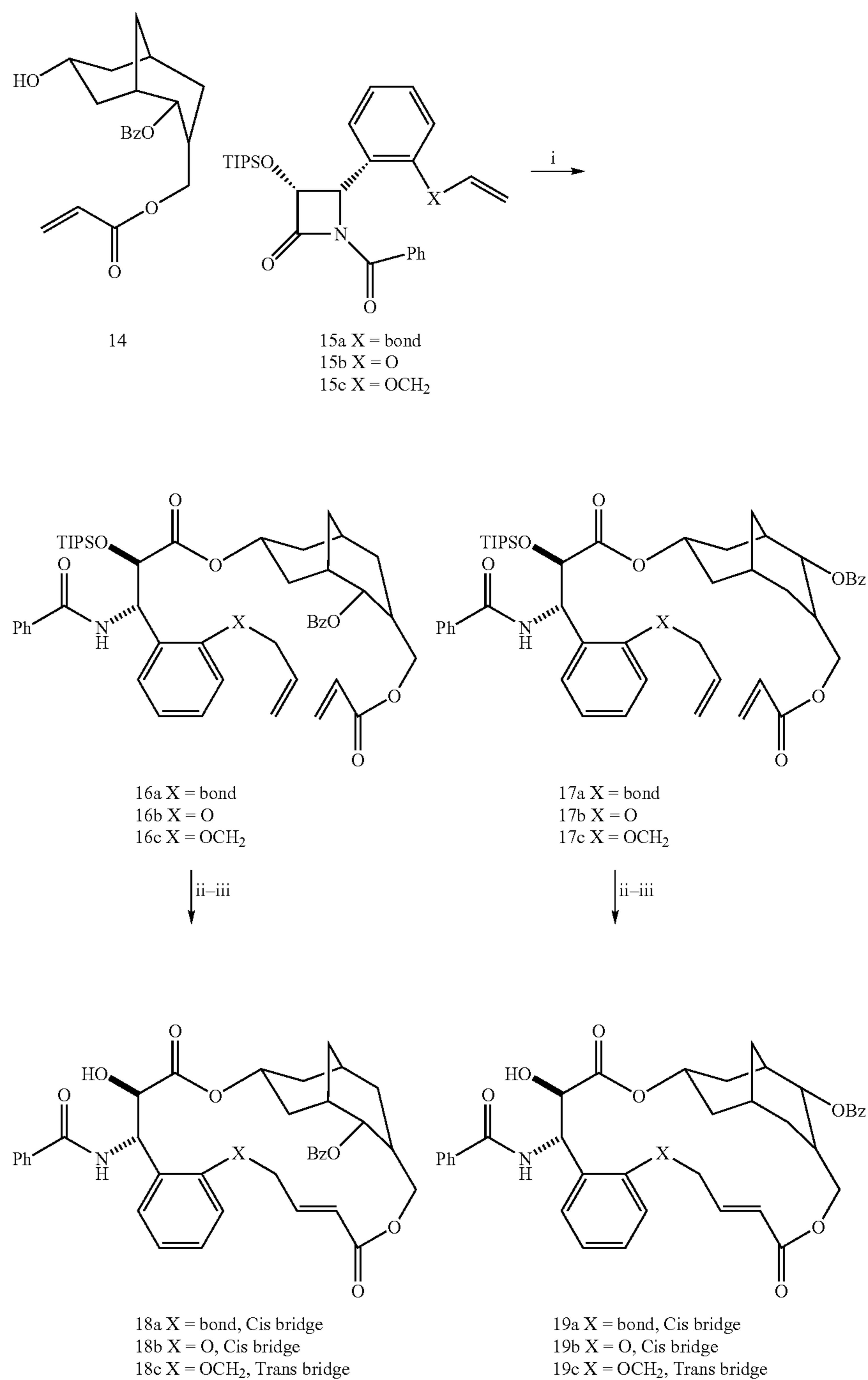
Scheme 2. Synthesis of Compounds 18 and 19
