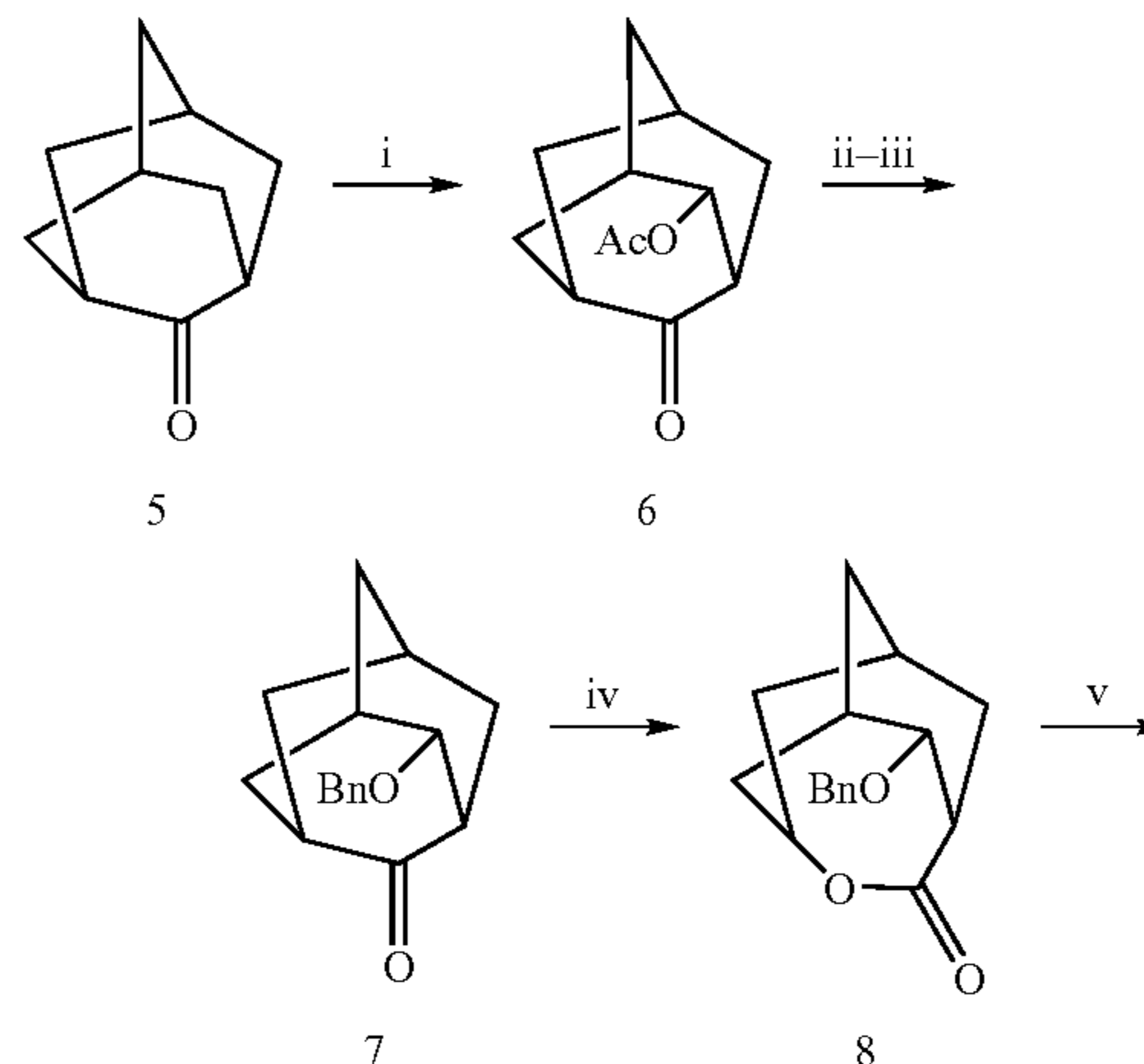
Scheme 1. Synthesis of Baccatin III Analog 14.
