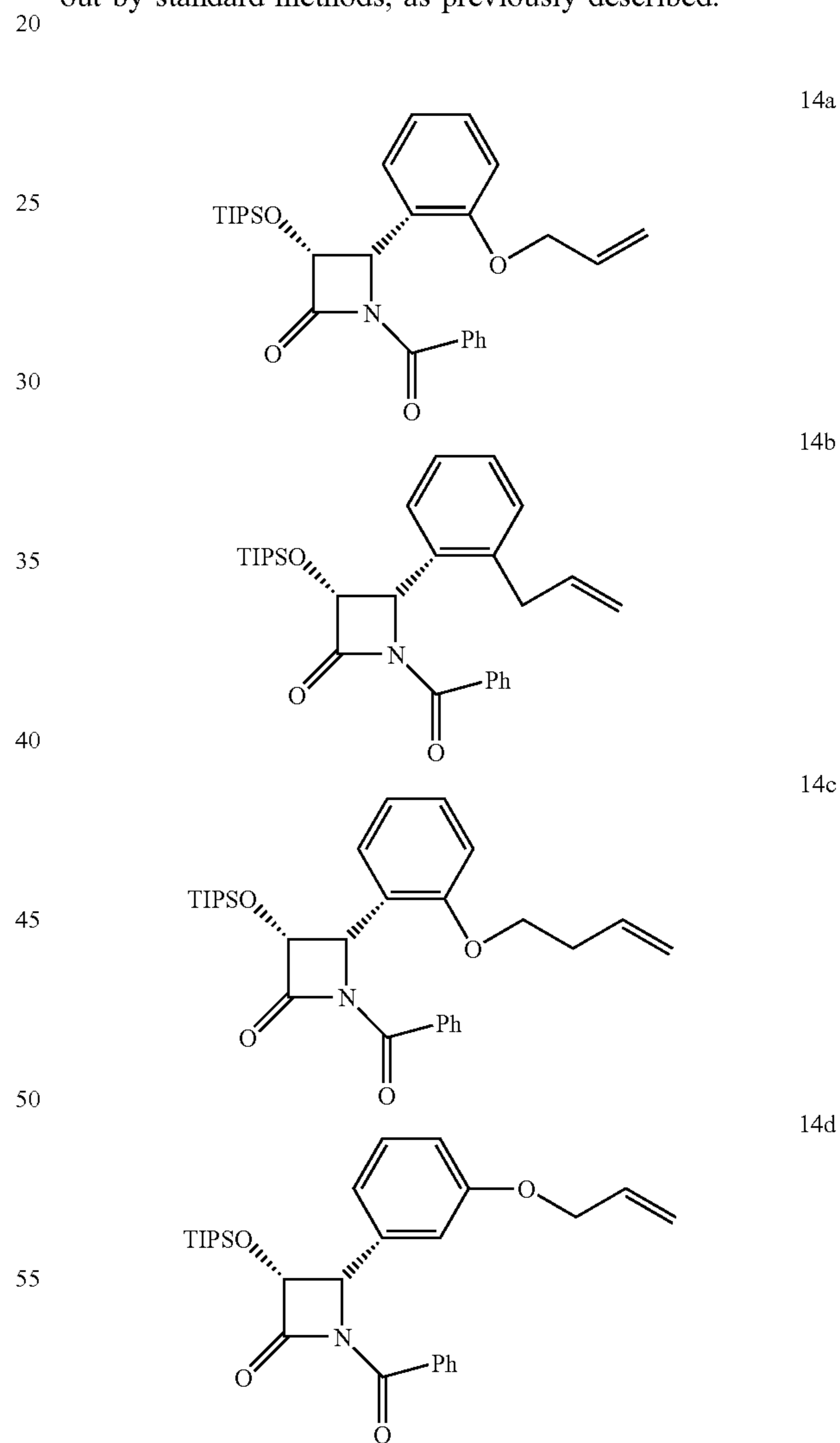
Scheme 1: Reagents and conditions: i. \text{NaN}_3 , \text{H}_2\text{SO}_4 , \text{Ac}_2\text{O} , (57%). ii. \text{KOH} , THF (85%). iii. \text{NaH} , \text{BnBr} , THF (95%). iv. \text{Ac}_2\text{O} , \text{AcOH} , \text{H}_2\text{O}_2 (77%). v. \text{LAH} , THF (76%). vi. \text{TBDPSCl} , Imidazole, DMF, (92%). vii. \text{Pd}(\text{OH})_2/\text{C} , 50Psi, 24 h, THF, (90%), viii. \text{BzCl} , \text{Et}_3\text{N} , DMAP, \text{CH}_2\text{Cl}_2 (95%) based on SM recovered. ix. \text{HF} -Pyridine, THF, 0^\circ\text{C} -RT, (70%). x. \text{LHMDS} , Acryloyl chloride, THF.
