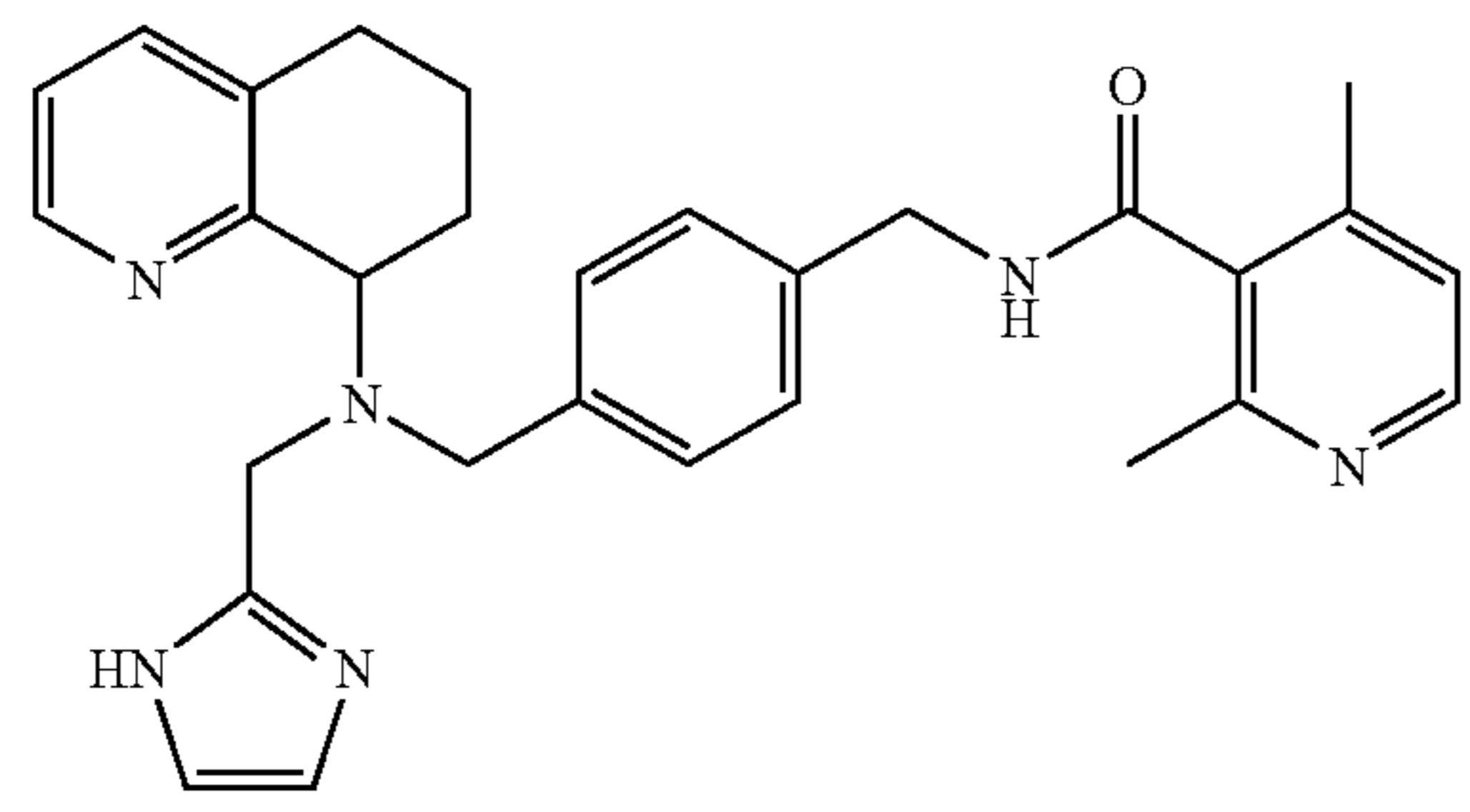
N-(4-[[1H-imidazol-2-ylmethyl]-(5,6,7,8-tetrahydro-quinolin-8-yl)-amino]-methyl)-benzyl)-2,4-dimethyl-nicotinamide
