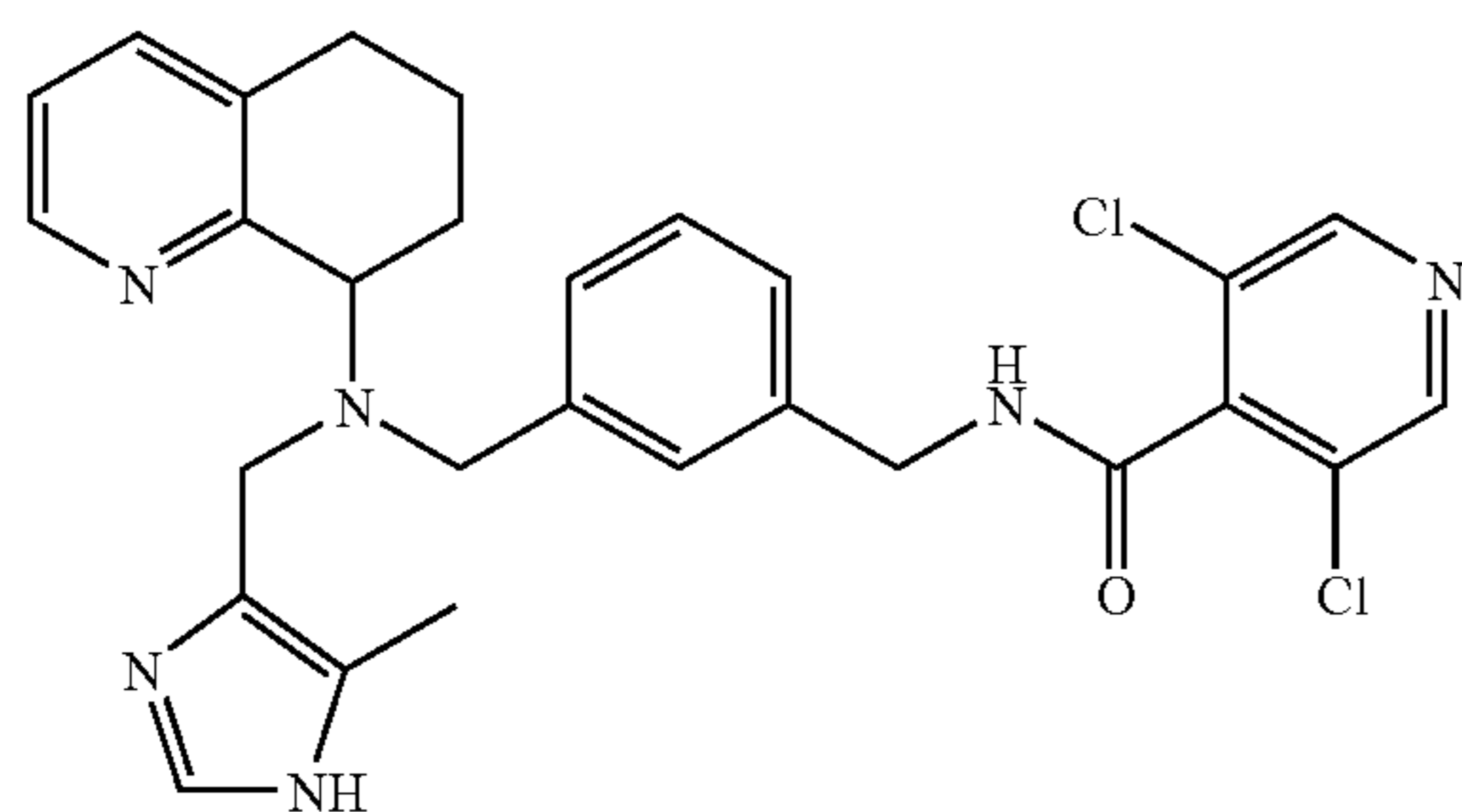
3,5-Dichloro-N-(3-((5-methyl-1H-imidazol-4-ylmethyl)-(5,6,7,8-tetrahydro-quinolin-8-yl)-amino)-methyl)-benzyl)-isonicotinamide
