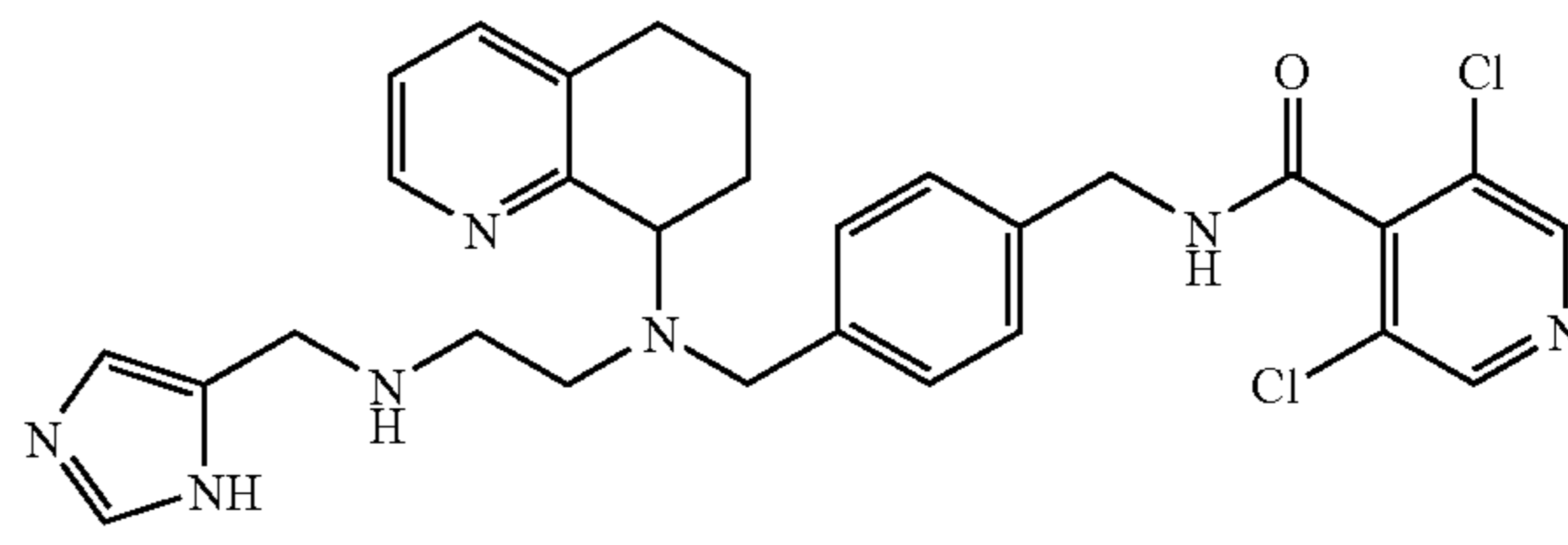
3,5-Dichloro-N-(4-[[2-[(3H-imidazol-4-ylmethyl)-amino]-ethyl]- (5,6,7,8-tetrahydro-quinolin-8-yl)-amino]-methyl)-benzyl)-isonicotinamide
