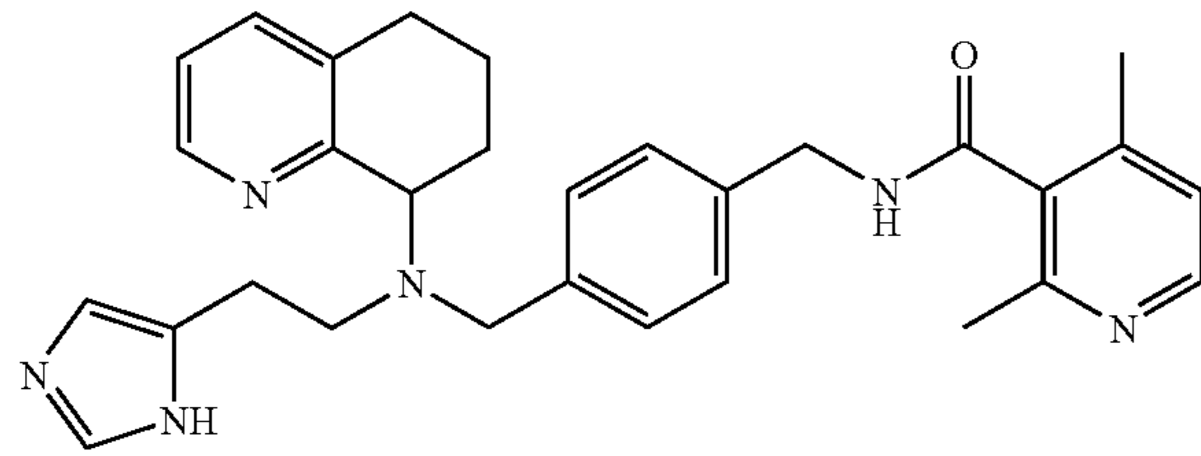
N-(3-[[[2-(1H-Imidazol-2-yl)-ethyl]-(5,6,7,8-tetrahydro-quinolin-8-yl)-amino]-methyl]-benzyl)-2,4-dimethyl-nicotinamide
