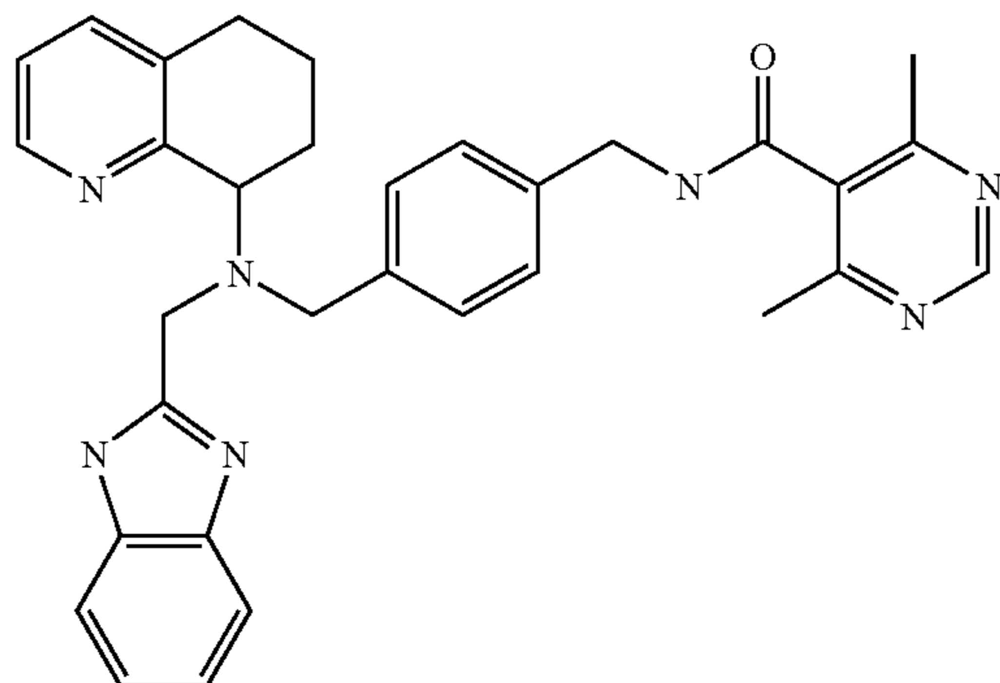
AMD11028: Preparation of 4,6-dimethyl-pyrimidine-5-carboxylic acid 4-[(1H-benzimidazol-2-ylmethyl)-(5,6,7,8-tetrahydro-quinolin-8-yl)-amino]-methyl-benzylamide
