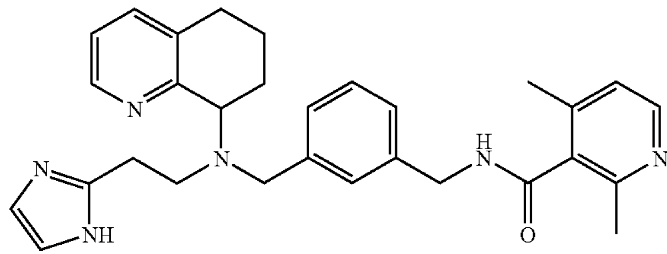
N-(3-[[[2-(1H-Imidazol-2-yl)-ethyl]-(5,6,7,8-tetrahydro-quinolin-8-yl)-amino]-methyl]-benzyl)-2,4-dimethyl-nicotinamide
