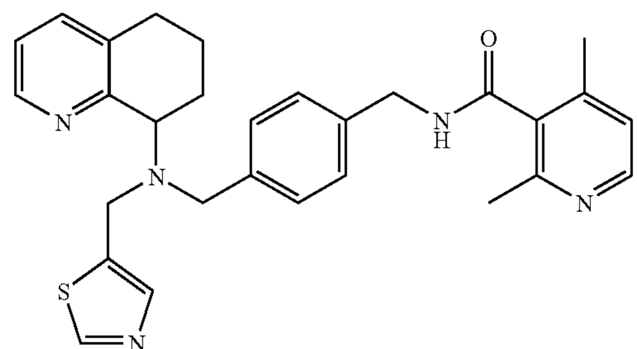
2,4-Dimethyl-N-(4-[[5,6,7,8-tetrahydro-quinolin-8-yl]-thiazol-5-ylmethyl-amino]-methyl)-benzyl)-nicotinamide
