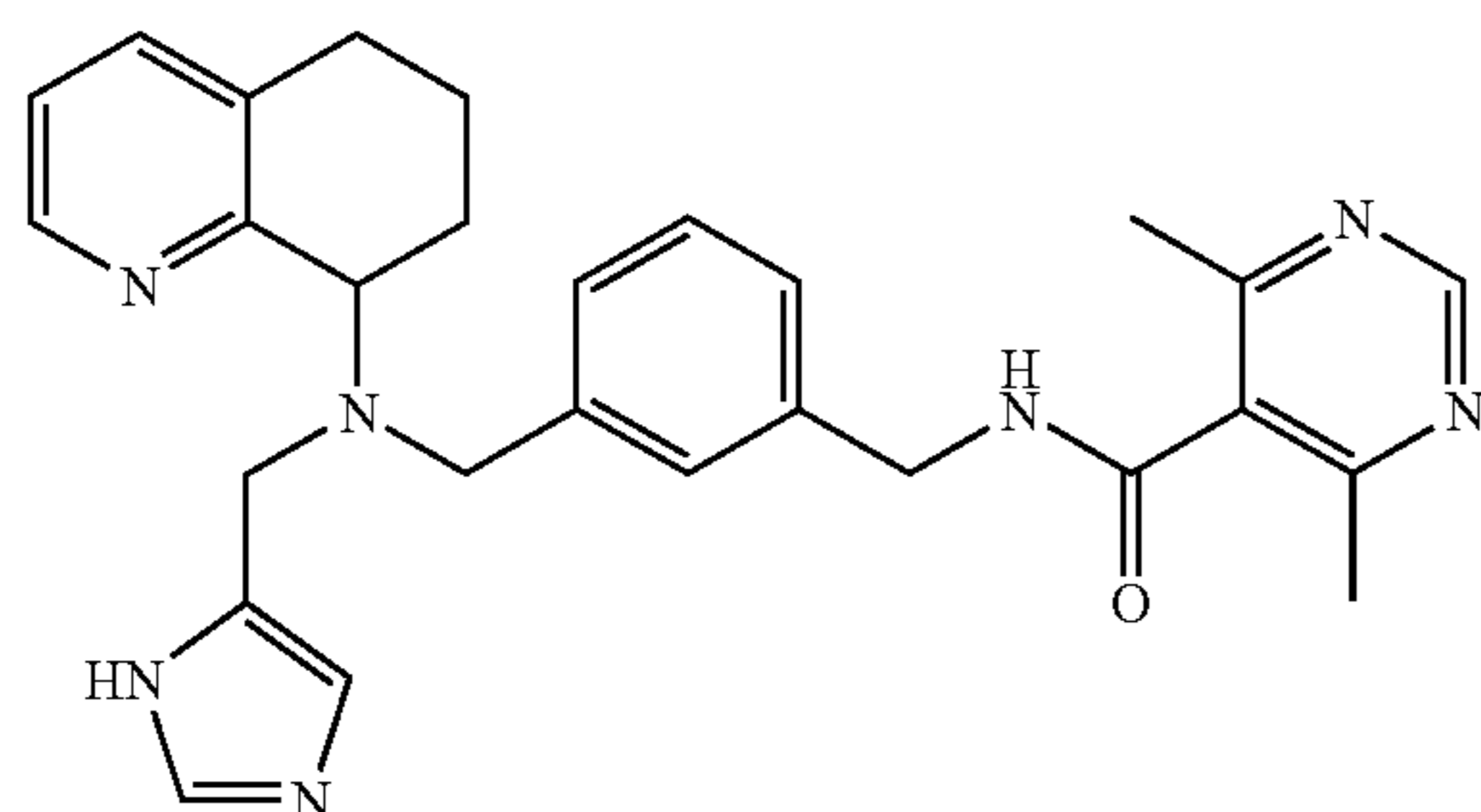
4,6-Dimethyl-pyrimidine-5-carboxylic acid 3-[(3H-imidazol-4-ylmethyl)-(5,6,7,8-tetrahydro-quinolin-8-yl)-amino]-methyl)-benzylamide
