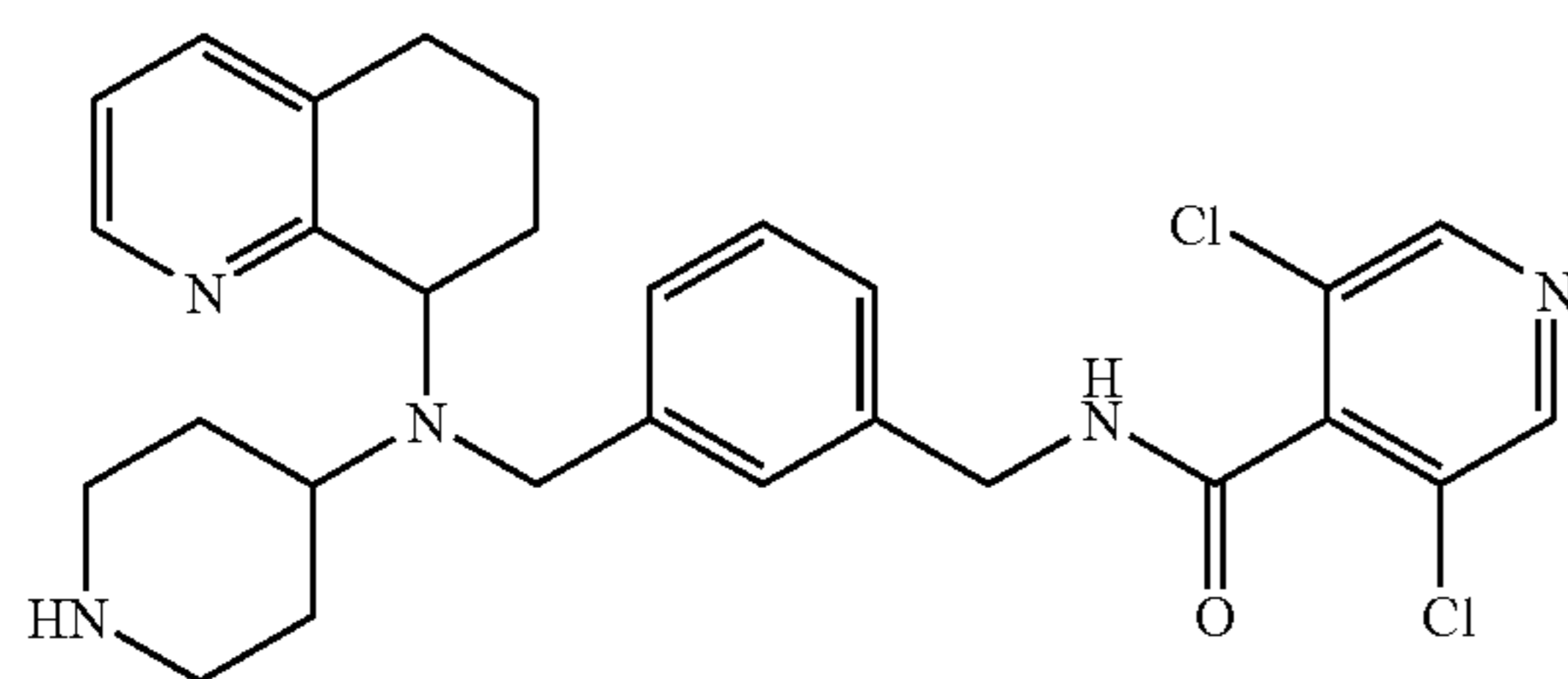
3,5-Dichloro-N-(3-[[piperidin-4-yl-(5,6,7,8-tetrahydro-quinolin-8-yl)-amino]-methyl]-benzyl)-isonicotinamide
