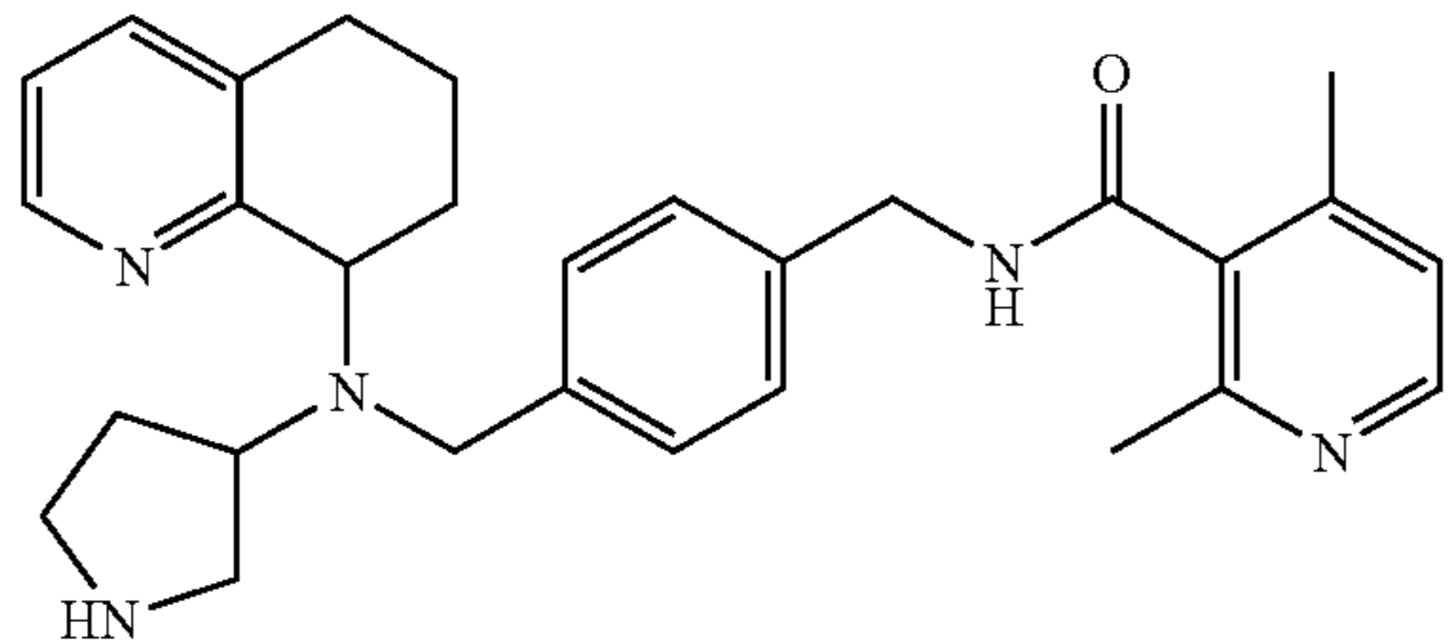
2,4-Dimethyl-N-(3-[[piperidin-3-yl-(5,6,7,8-tetrahydroquinolin-8-yl)-amino]-methyl]-benzyl)-nicotinamide
