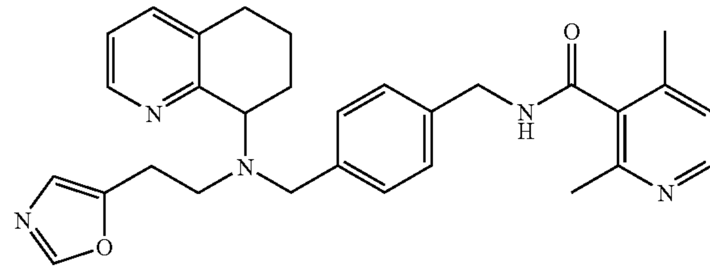
5 2,4-Dimethyl-N-(4-[[[2-oxazol-5-yl-ethyl]-(5,6,7,8-tetrahydro-quinolin-8-yl)-amino]-methyl]-benzyl)-nicotinamide
