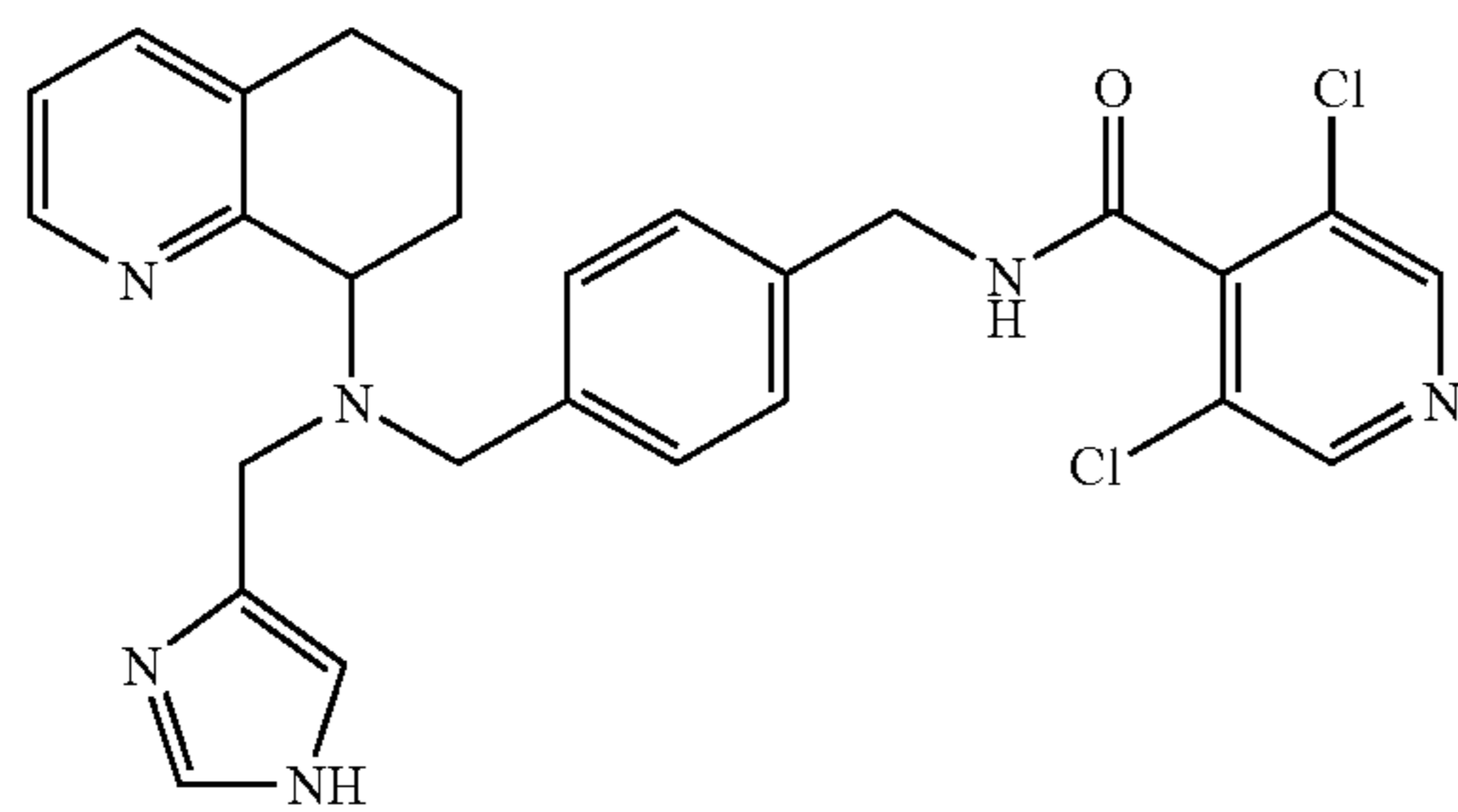
3,5-Dichloro-N-(4-[[1H-imidazol-4-ylmethyl]-(5,6,7,8-tetrahydro-quinolin-8-yl)-amino]-methyl)-benzyl)-isonicotinamide
