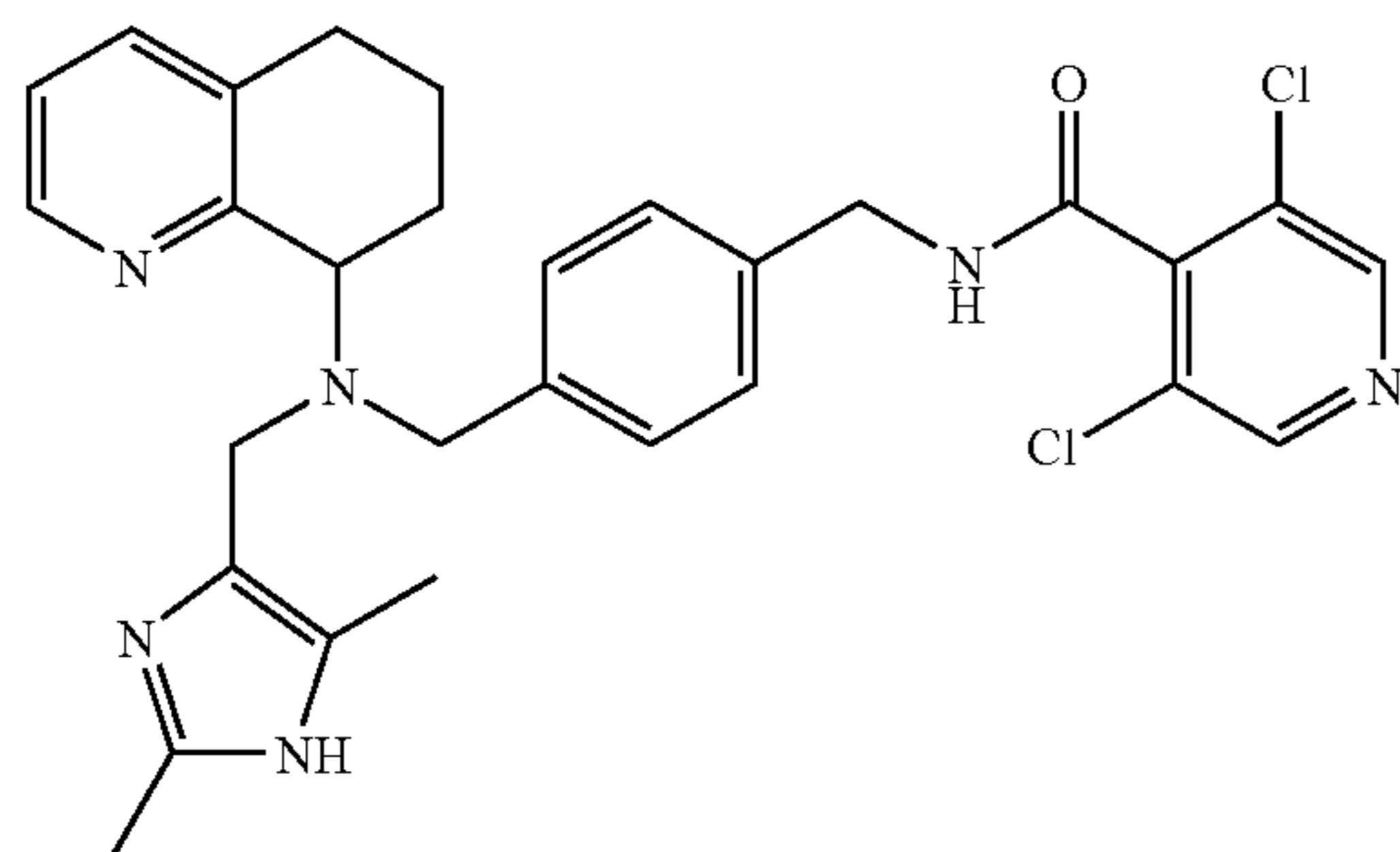
3,5-Dichloro-N-(3-((5-methyl-1H-imidazol-4-ylmethyl)-(5,6,7,8-tetrahydro-quinolin-8-yl)-amino)-methyl)-benzyl)-isonicotinamide
