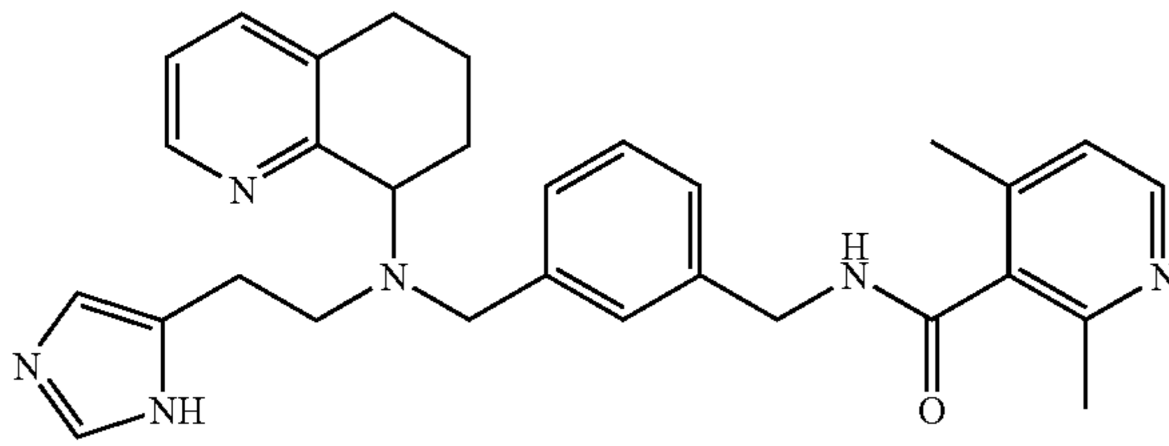
N-(4-[[[2-(3H-Imidazol-4-yl)-ethyl]-(5,6,7,8-tetrahydro-quinolin-8-yl)-amino]-methyl]-benzyl)-2,4-dimethyl-nicotinamide
