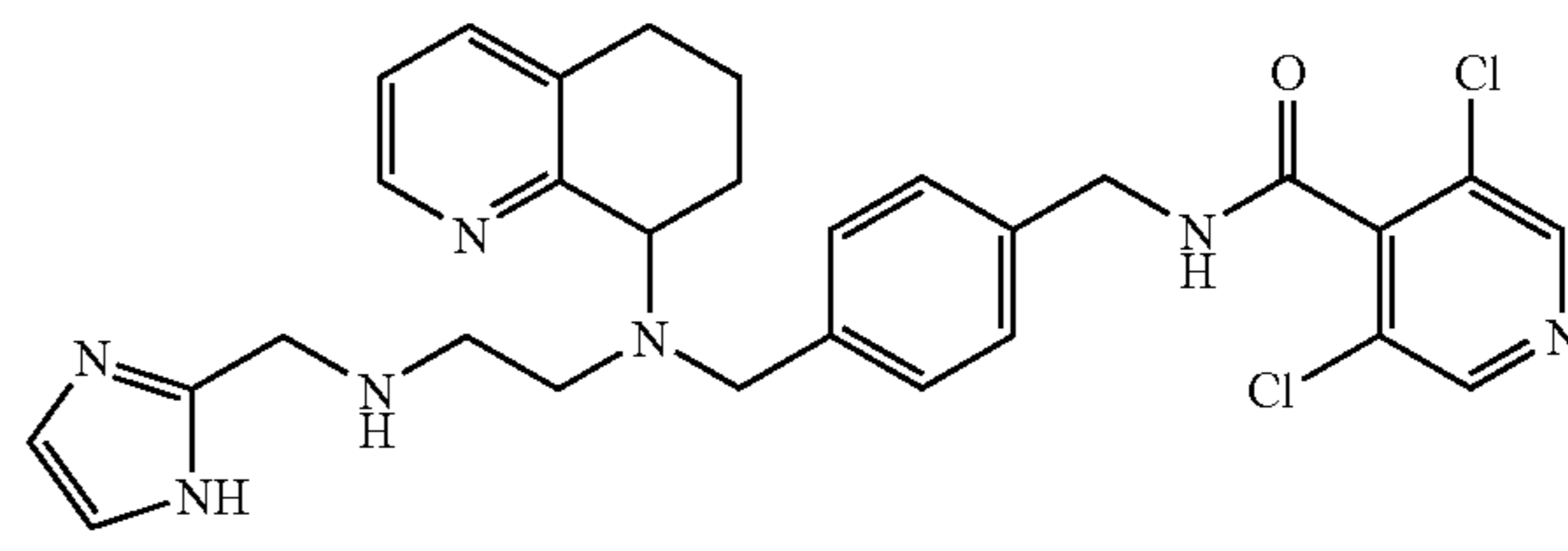
3,5-Dichloro-N-(4-[[2-[(1H-imidazol-2-ylmethyl)-amino]-ethyl]- (5,6,7,8-tetrahydro-quinolin-8-yl)-amino]-methyl)-benzyl)-isonicotinamide
