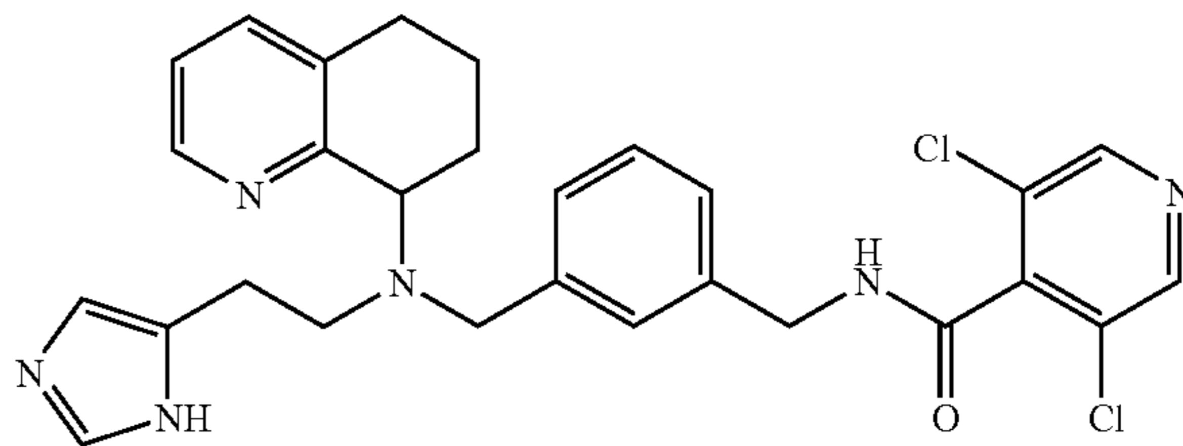
3,5-Dichloro-N-(4-[[[2-(3H-imidazol-4-yl)-ethyl]]-(5,6,7,8-tetrahydro-quinolin-8-yl)-amino]-methyl}-benzyl)-isonicotinamide
