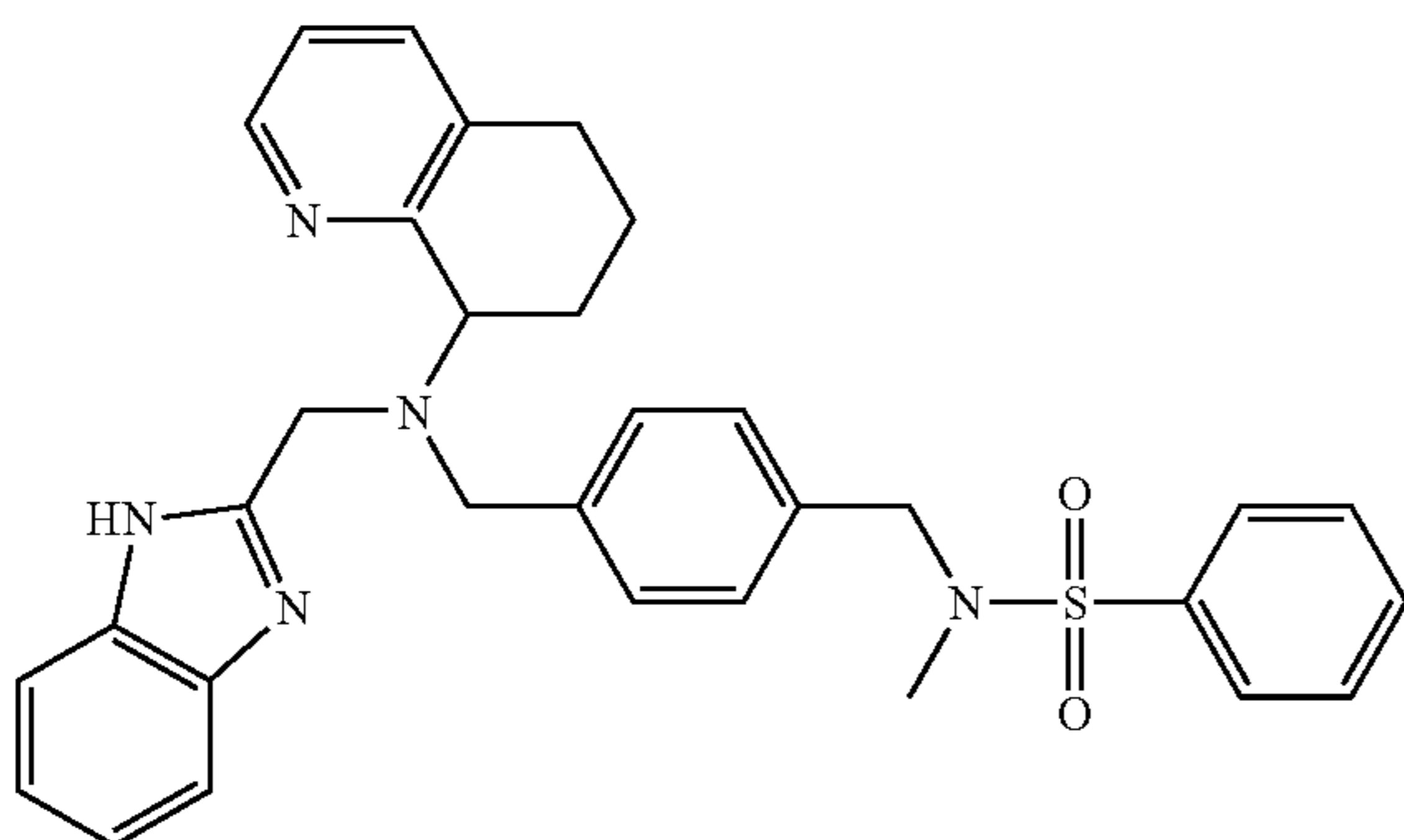
AMD9831: Preparation of N-(4-[(1H-benzimidazol-2-ylmethyl)-(5,6,7,8-tetrahydro-quinolin-8-yl)-amino]-methyl)-benzyl)-N-methyl-benzenesulfonamide
