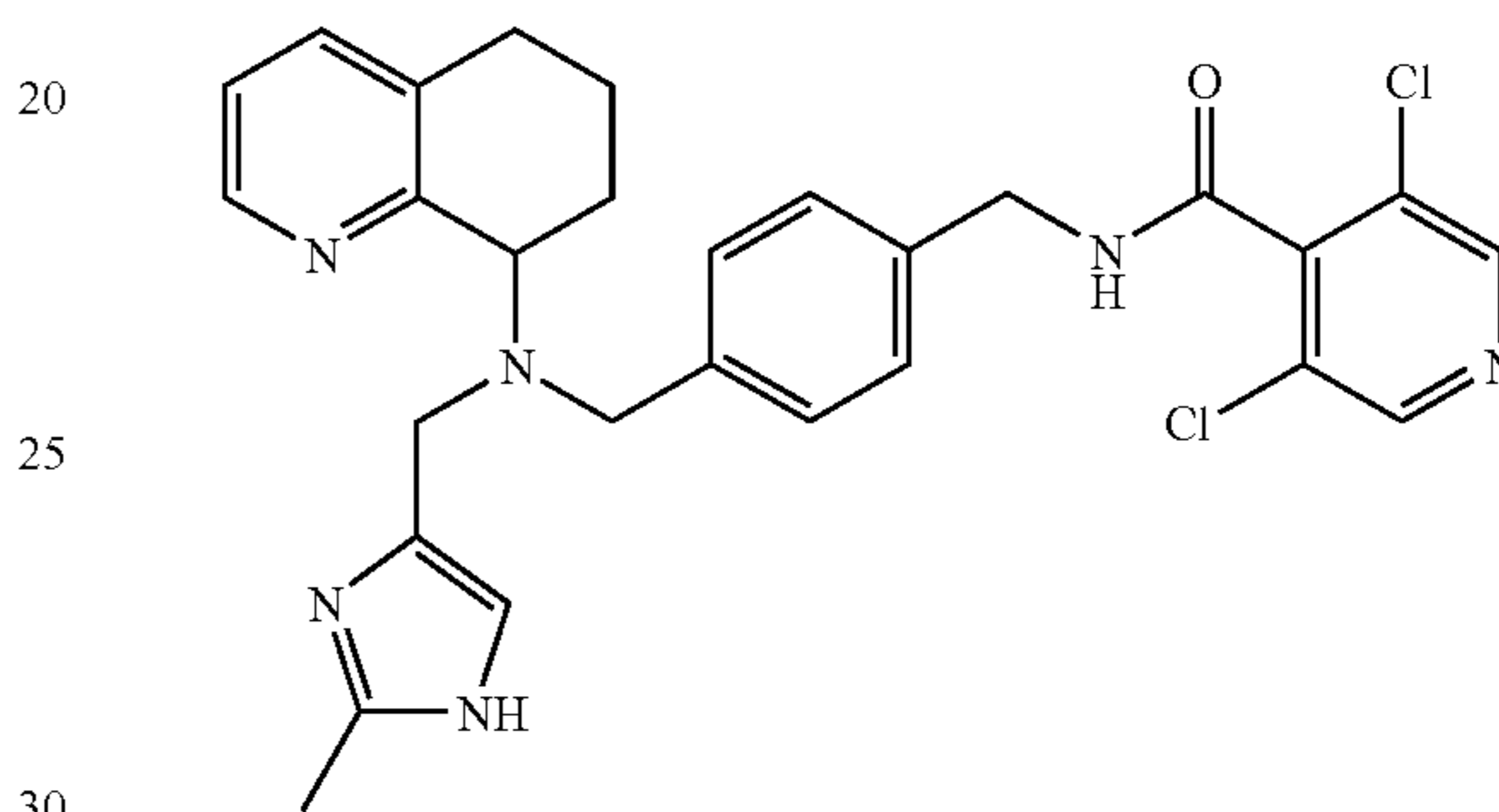
3,5-Dichloro-N-(4-[[2-methyl-1H-imidazol-4-ylmethyl]-(5,6,7,8-tetrahydro-quinolin-8-yl)-amino]-methyl)-benzyl)-isonicotinamide
