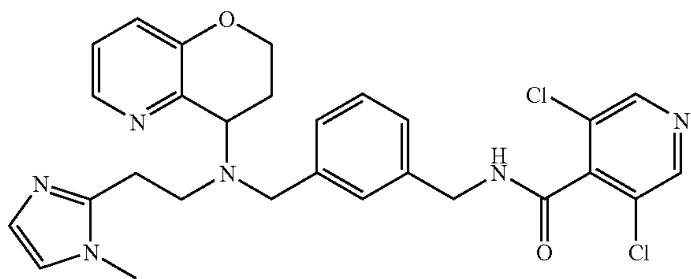
3,5-Dichloro-N-[3-((3,4-dihydro-2H-pyrano[3,2-b]pyridin-4-yl)-[2-(1-methyl-1H-imidazol-2-yl)-ethyl]-amino)-methyl]-benzyl]-isonicotinamide
