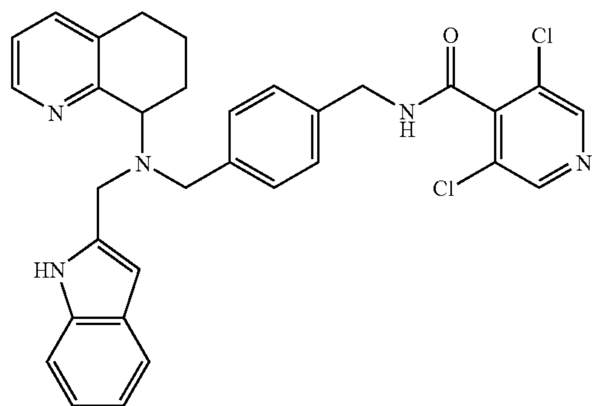
3,5-Dichloro-N-(4-[[1H-indol-2-ylmethyl)-(5,6,7,8-tetrahydro-quinolin-8-yl)-amino]-methyl}-benzyl)-isonicotinamide
