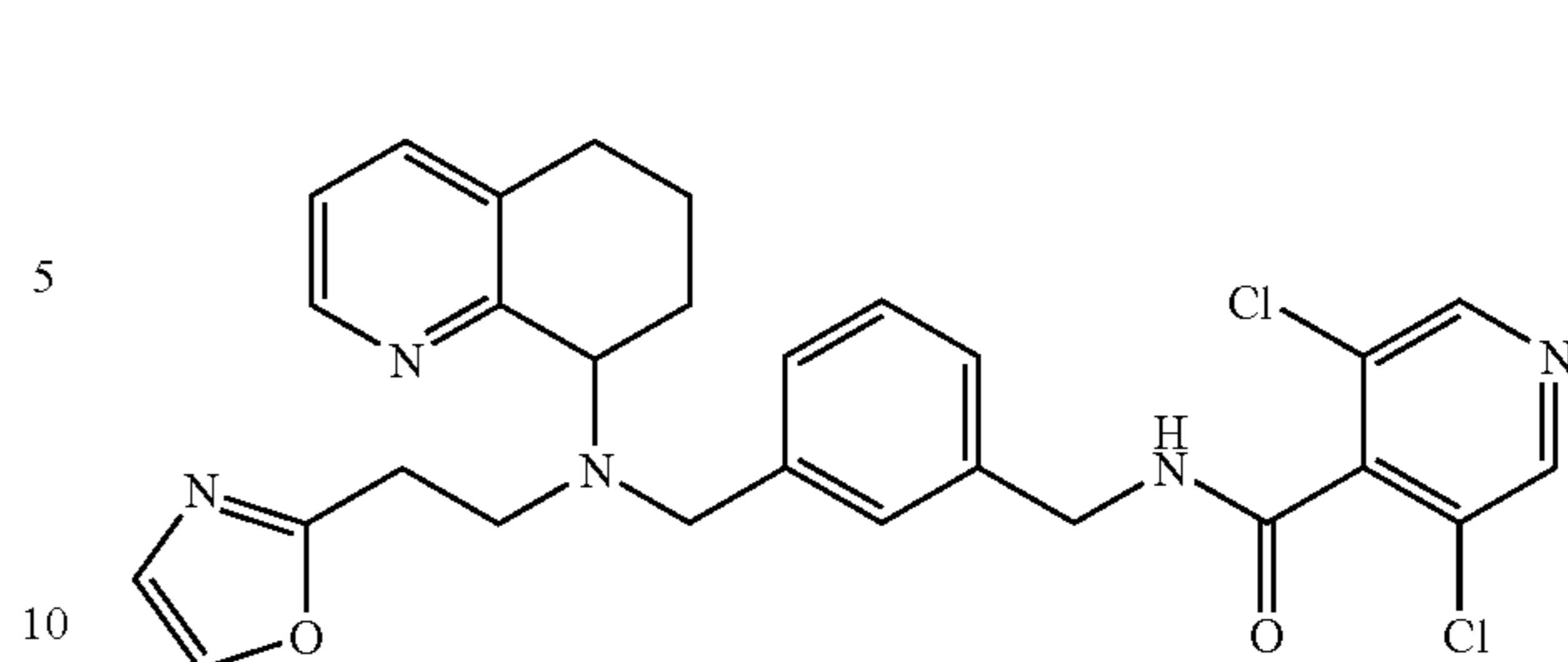
3,5-Dichloro-N-(3-[[2-(2-oxazol-2-yl-ethyl)-(5,6,7,8-tetrahydro-quinolin-8-yl)-amino]-methyl]-benzyl)-isonicotinamide
