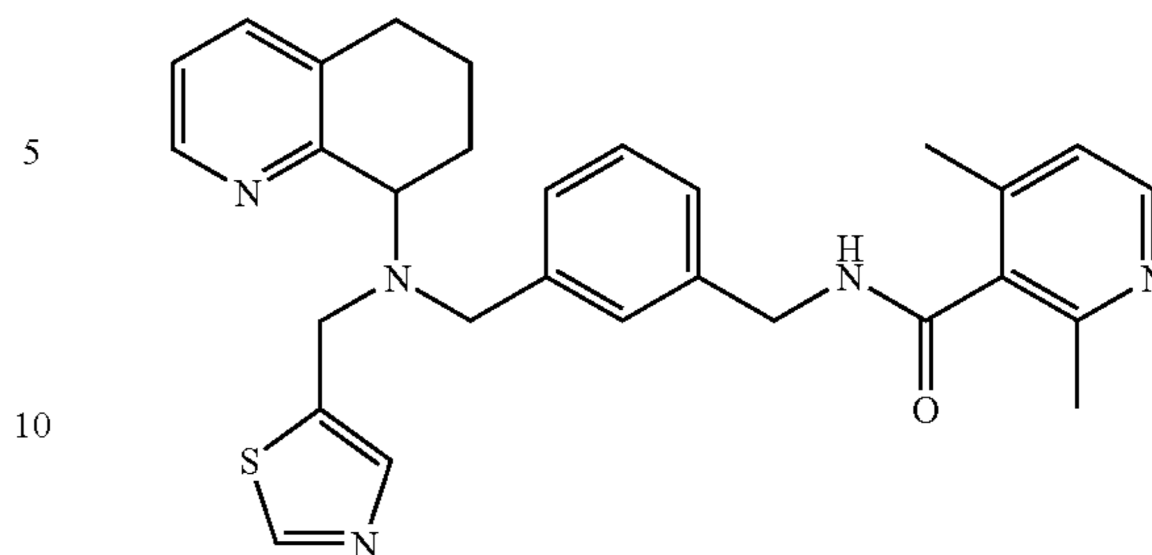
15 2,4-Dimethyl-N-(3-[[5,6,7,8-tetrahydro-quinolin-8-yl]-thiazol-5-ylmethyl-amino]-methyl)-benzyl)-nicotinamide
