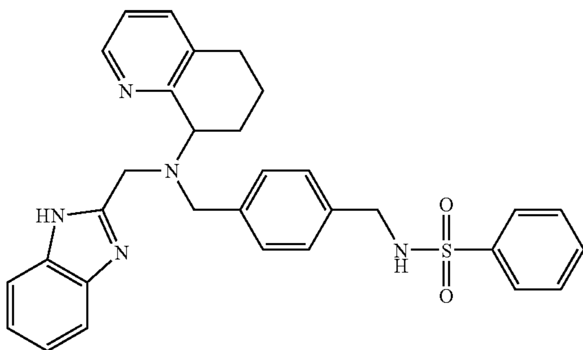
AMD9845: Preparation of N-(4-[(1H-benzimidazol-2-ylmethyl)-(5,6,7,8-tetrahydro-quinolin-8-yl)-amino]-methyl)-benzyl)-benzenesulfonamide
