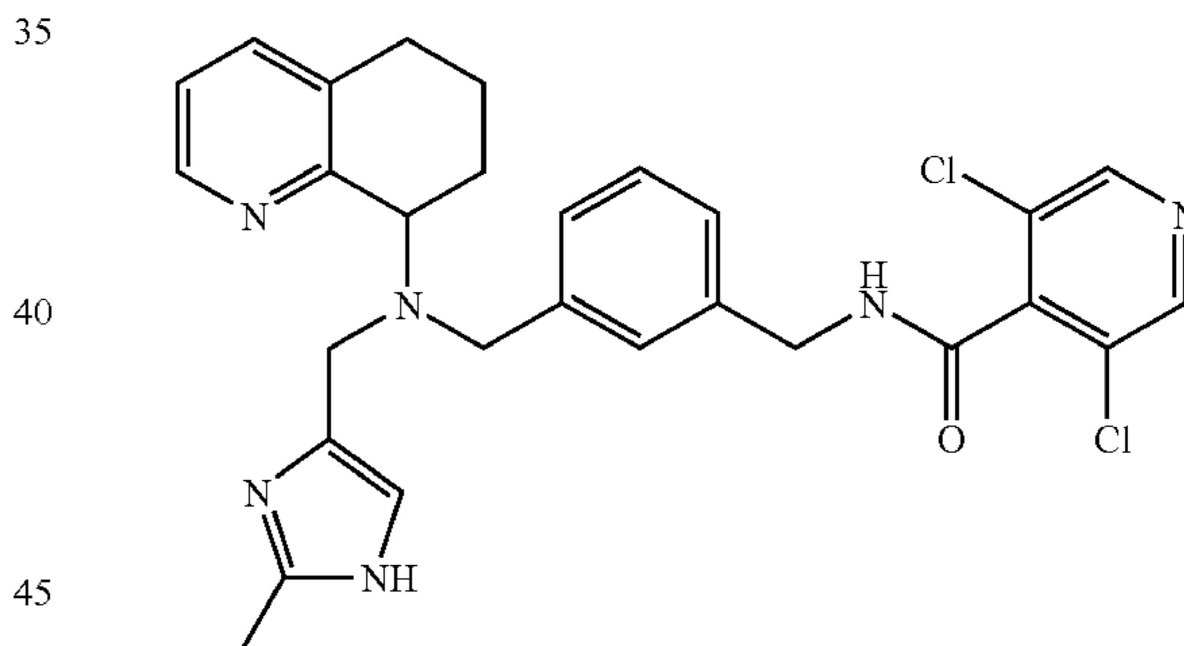
3,5-Dichloro-N-(4-[[2-methyl-1H-imidazol-4-ylmethyl]-(5,6,7,8-tetrahydro-quinolin-8-yl)-amino]-methyl)-benzyl)-isonicotinamide
