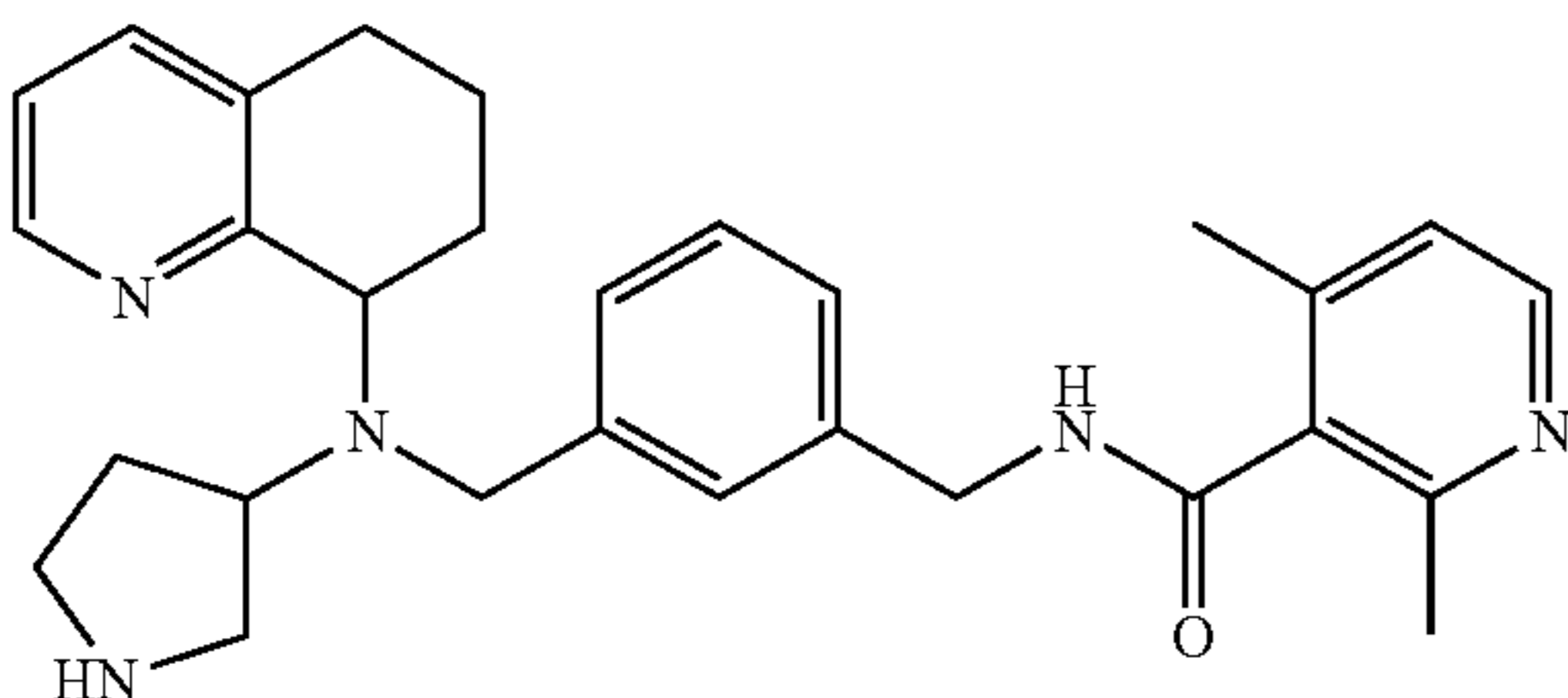
2,4-Dimethyl-N-(4-[[pyrrolidin-3-yl-(5,6,7,8-tetrahydroquinolin-8-yl)-amino]-methyl]-benzyl)-nicotinamide
