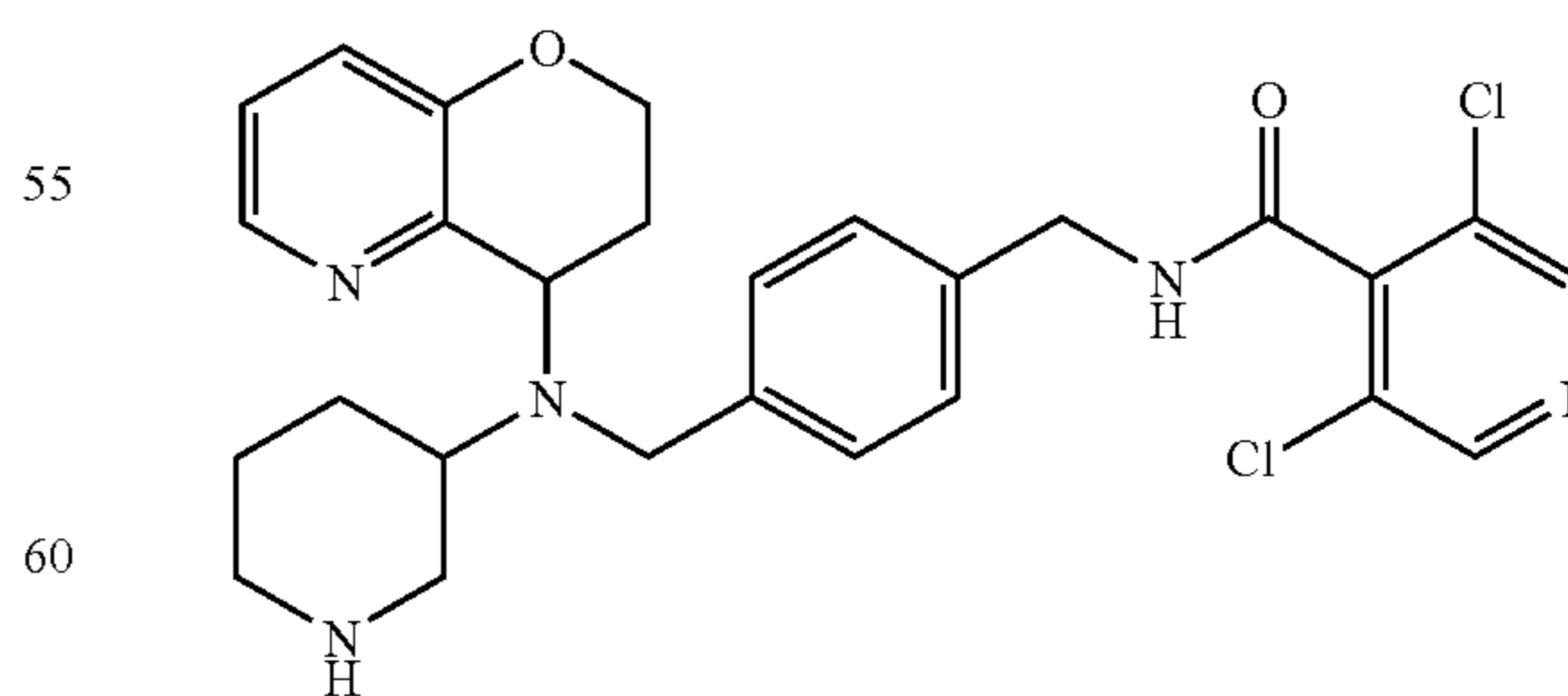
3,5-Dichloro-N-(4-[[3,4-dihydro-2H-pyrano[3,2-b]pyridin-4-yl)-piperidin-3-yl-amino]-methyl)-benzyl)-isonicotinamide
