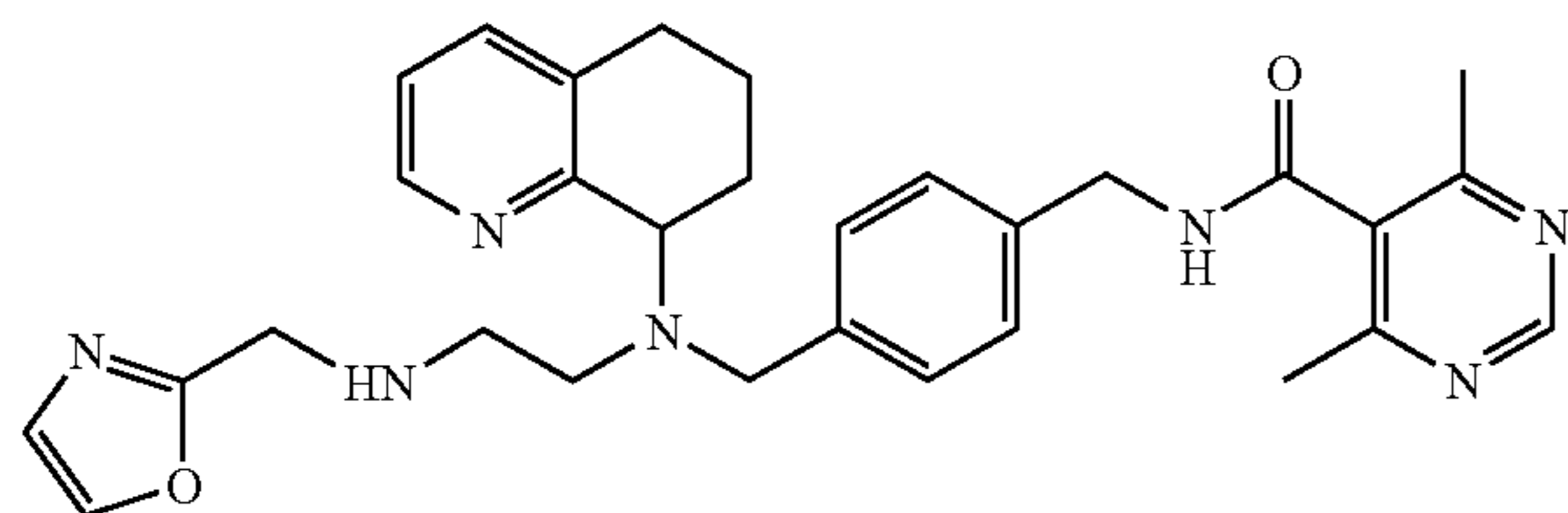
4,6-Dimethyl-pyrimidine-5-carboxylic acid 4-[[{2-[(oxazol-2-ylmethyl)-amino]-ethyl}-(5,6,7,8-tetrahydro-quinolin-8-yl)-amino]-methyl]-benzylamide
