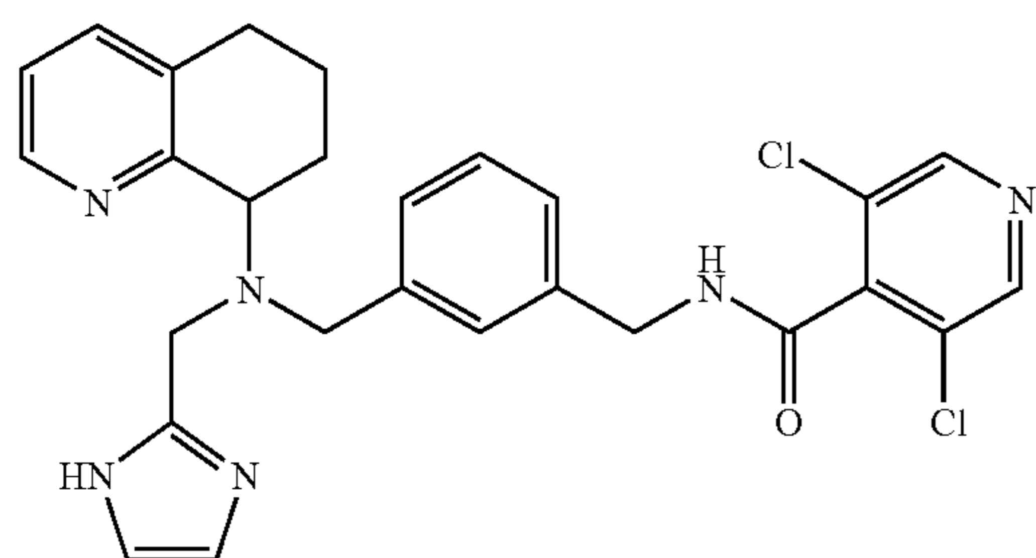
3,5-Dichloro-N-(3-[[[1H-imidazol-2-ylmethyl]-(5,6,7,8-tetrahydro-quinolin-8-yl)-amino]-methyl]-benzyl)-isonicotinamide
