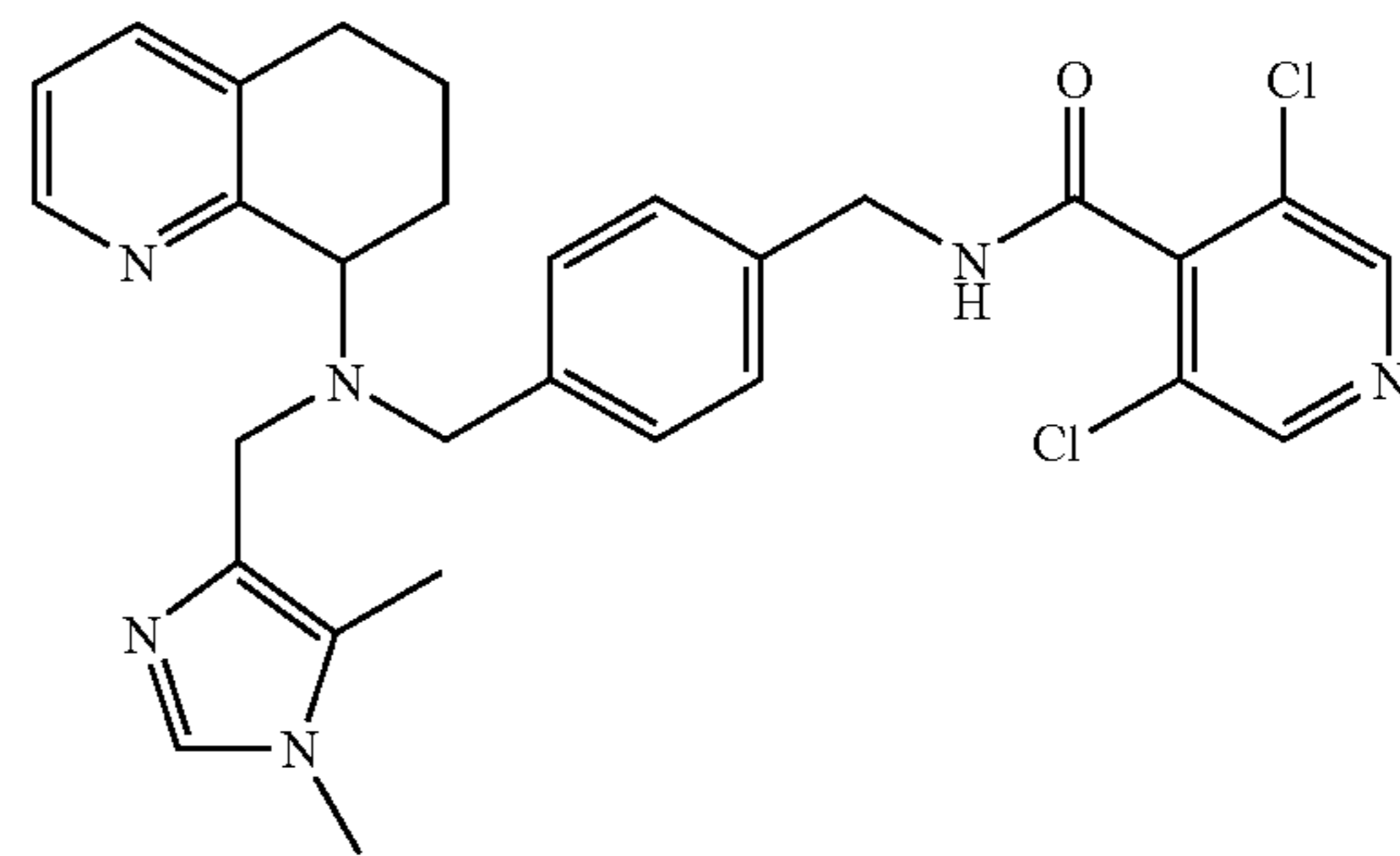
3,5-Dichloro-N-(3-((1,2-dimethyl-1H-imidazol-4-ylmethyl)-(5,6,7,8-tetrahydro-quinolin-8-yl)-amino)-methyl)-benzyl)-isonicotinamide
