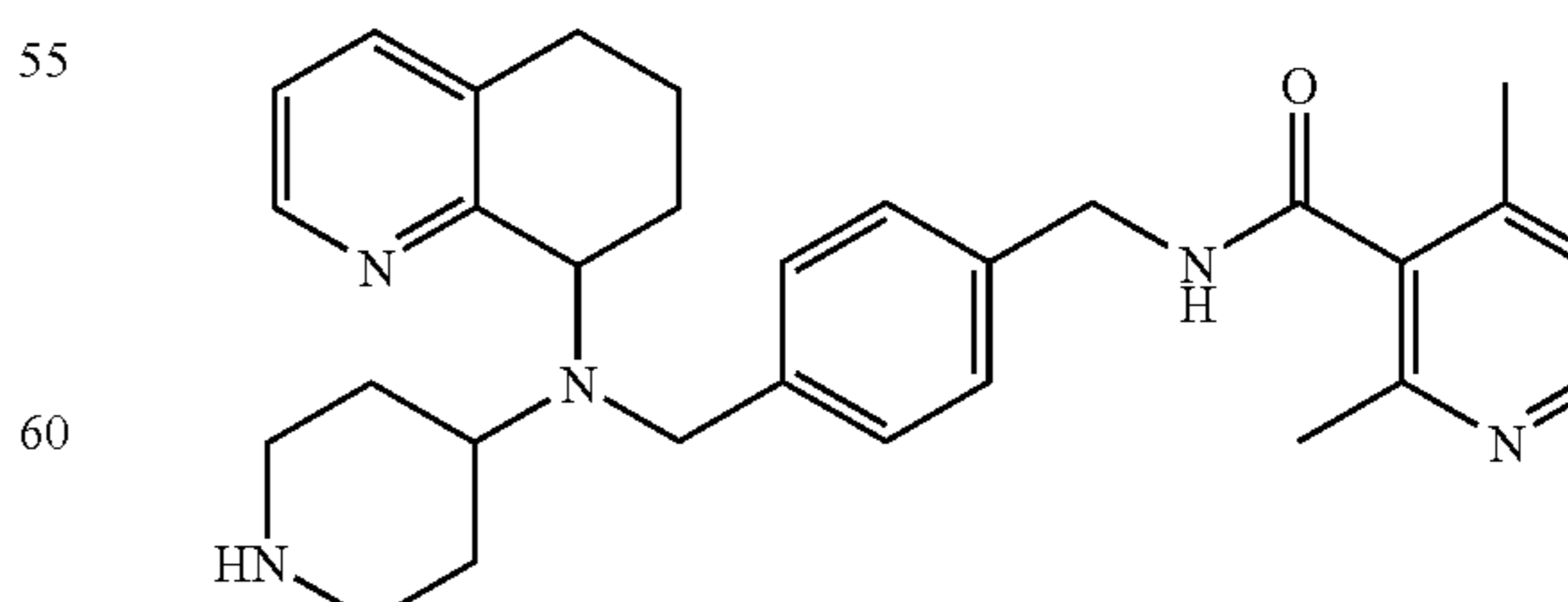
40 2,4-Dimethyl-N-(3-[[5,6,7,8-tetrahydro-quinolin-8-yl]-thiazol-2-ylmethyl-amino]-methyl)-benzyl)-nicotinamide
