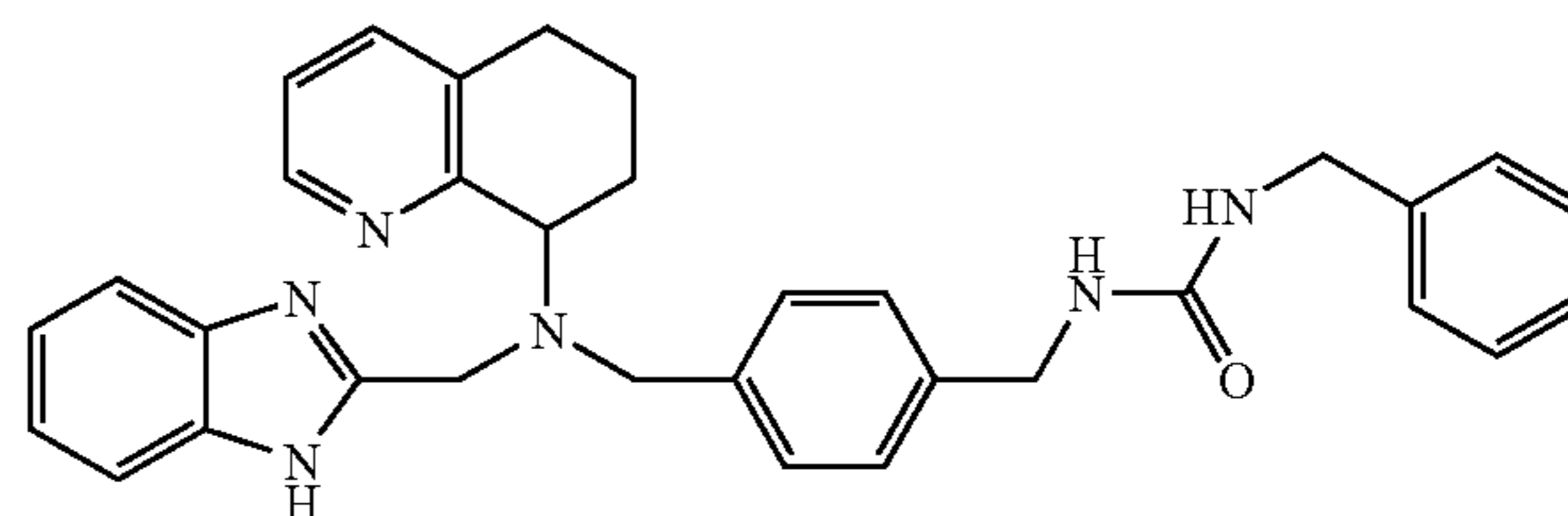
AMD9594: Preparation of 1-(4-[(1H-Benzimidazol-2-ylmethyl)-(5,6,7,8-tetrahydro-quinolin-8-yl)-amino]-methyl)-benzyl)-3-benzyl-urea (hydrobromide salt)
