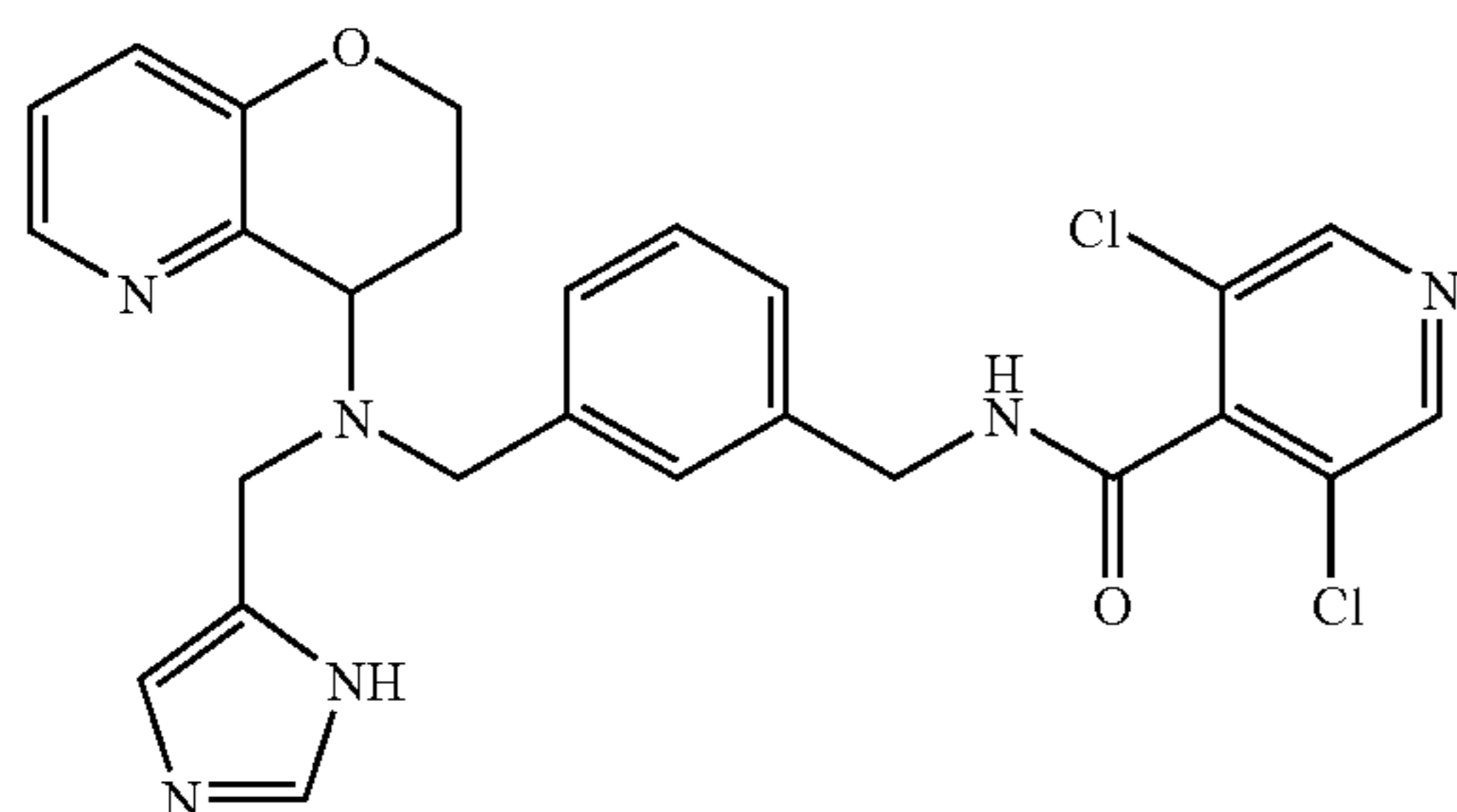
3,5-Dichloro-N-(3-[[3,4-dihydro-2H-pyrano[3,2-b]pyridin-4-yl)-(3H-imidazol-4-ylmethyl)-amino]-methyl)-benzyl)-isonicotinamide
