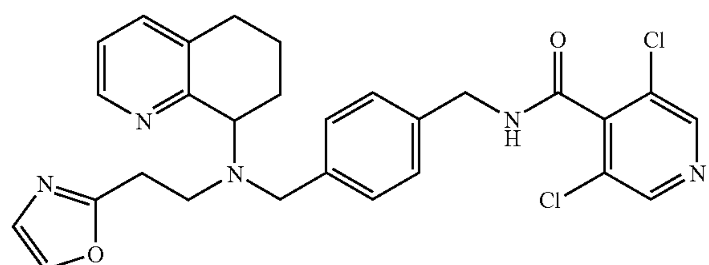
3,5-Dichloro-N-(3-[[[2-(2-methyl-oxazol-5-yl)-ethyl]-(5,6,7,8-tetrahydro-quinolin-8-yl)-amino]-methyl]-benzyl)-isonicotinamide
