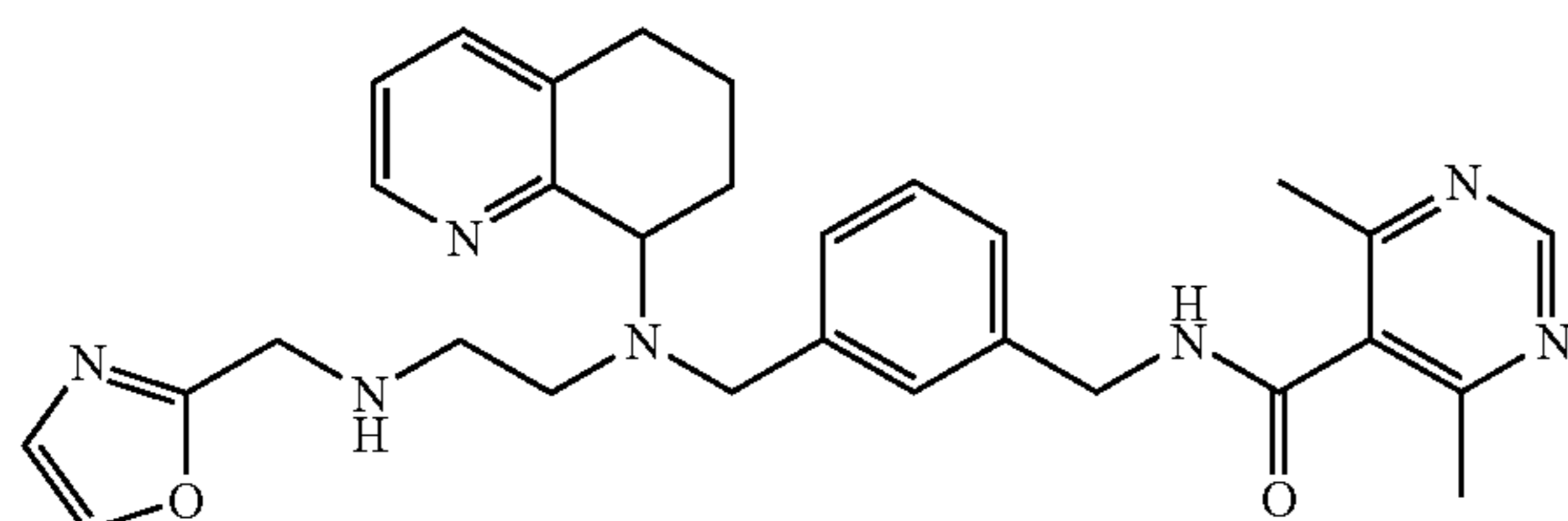
4,6-Dimethyl-pyrimidine-5-carboxylic acid 3-[[{2-[(oxazol-2-ylmethyl)-amino]-ethyl}-(5,6,7,8-tetrahydro-quinolin-8-yl)-amino]-methyl]-benzylamide
