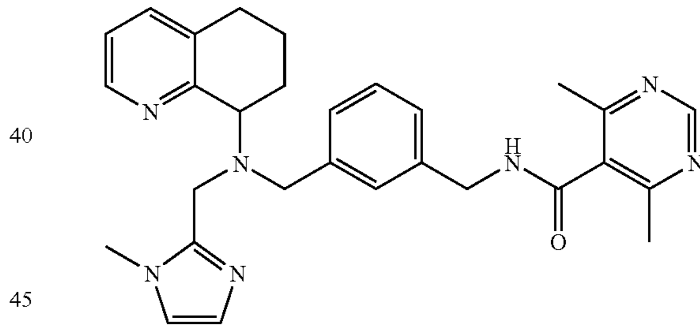
4,6-Dimethyl-pyrimidine-5-carboxylic acid 3-{[(1-methyl-1H-imidazol-2-ylmethyl)-(5,6,7,8-tetrahydro-quinolin-8-yl)-amino]-methyl}-benzamide
