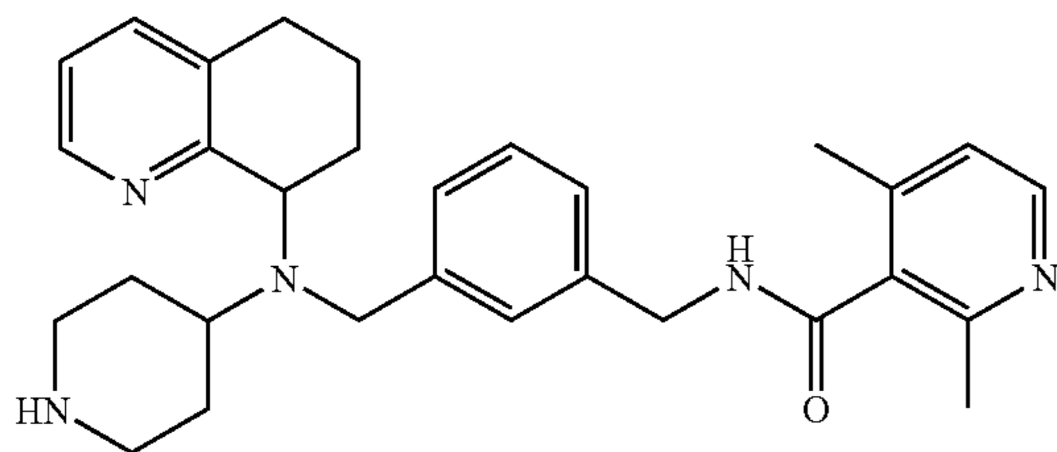
2,4-Dimethyl-N-(3-[[piperidin-4-yl-(5,6,7,8-tetrahydroquinolin-8-yl)-amino]-methyl]-benzyl)-nicotinamide
