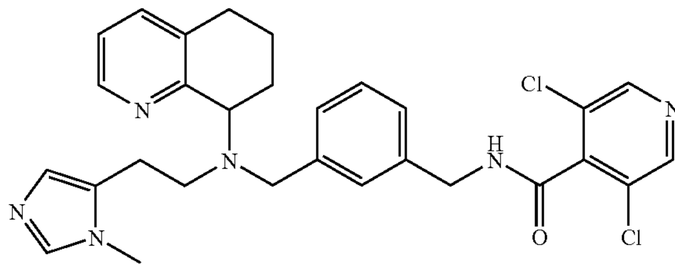
3,5-Dichloro-N-(4-[[[2-(3-methyl-3H-imidazol-4-yl)-ethyl]]-(5,6,7,8-tetrahydro-quinolin-8-yl)-amino]-methyl}-benzyl)-isonicotinamide
