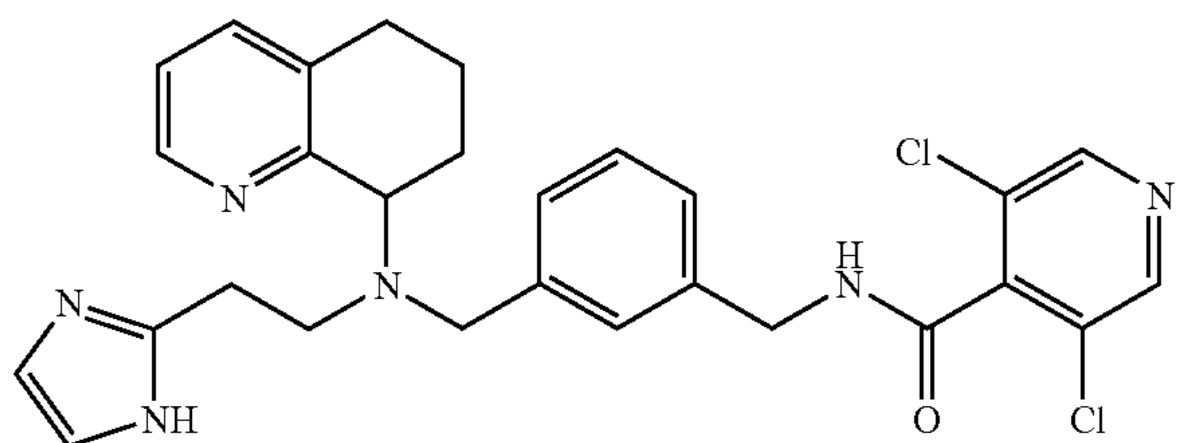
3,5-Dichloro-N-(4-[[[2-(1H-imidazol-2-yl)-ethyl]]-(5,6,7,8-tetrahydro-quinolin-8-yl)-amino]-methyl}-benzyl)-isonicotinamide
