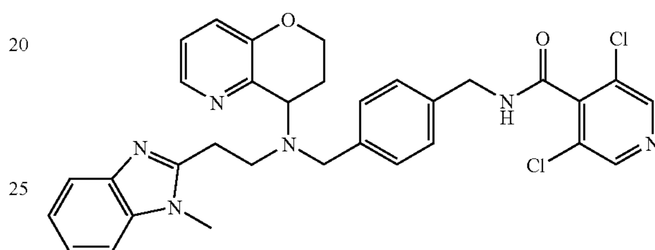
3,5-Dichloro-N-[4-((3,4-dihydro-2H-pyrano[3,2-b]pyridin-4-yl)-[2-(1-methyl-1H-benzoimidazol-2-yl)-ethyl]-amino)-methyl]-benzyl]-isonicotinamide
