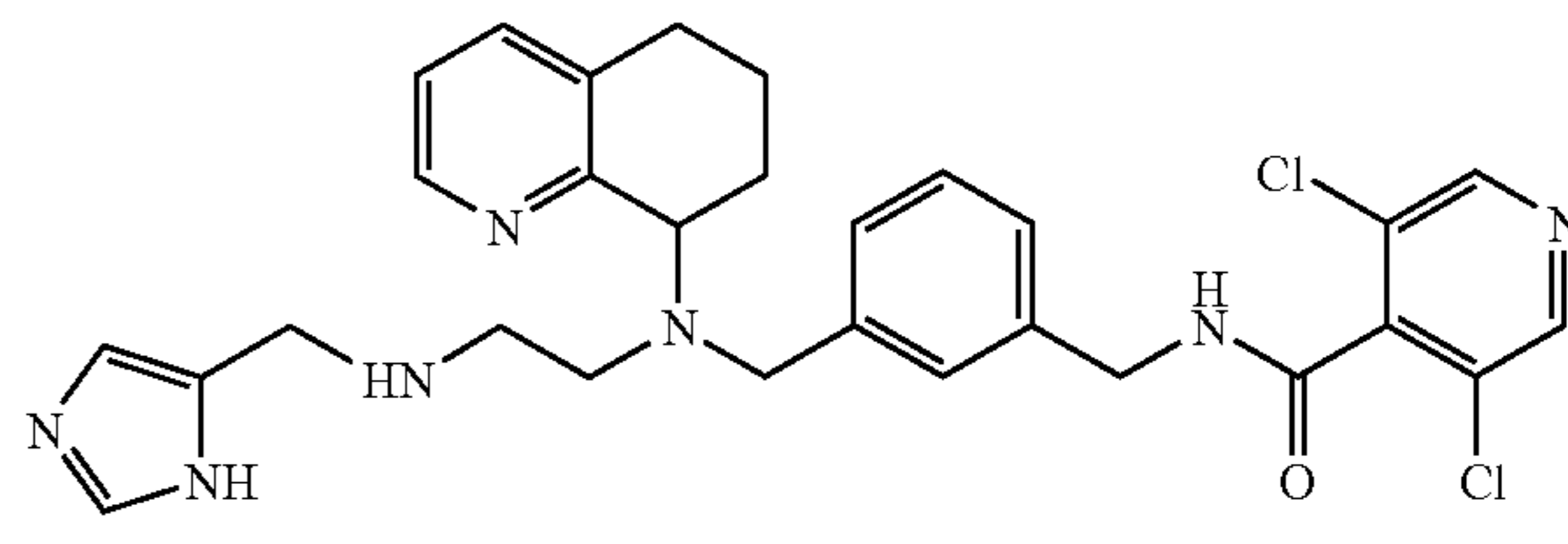
3,5-Dichloro-N-(3-[[2-[(3H-imidazol-4-ylmethyl)-amino]-ethyl]- (5,6,7,8-tetrahydro-quinolin-8-yl)-amino]-methyl)-benzyl)-isonicotinamide
