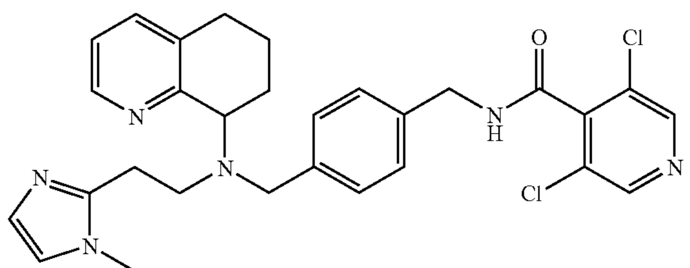
3,5-Dichloro-N-(3-[[[2-(1H-imidazol-2-yl)-ethyl]]-(5,6,7,8-tetrahydro-quinolin-8-yl)-amino]-methyl}-benzyl)-isonicotinamide
