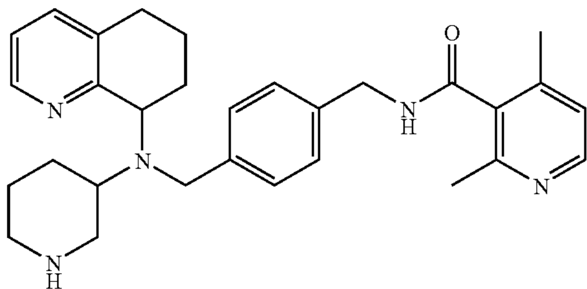
2,4-Dimethyl-N-(4-[[piperidin-3-yl-(5,6,7,8-tetrahydroquinolin-8-yl)-amino]-methyl]-benzyl)-nicotinamide
