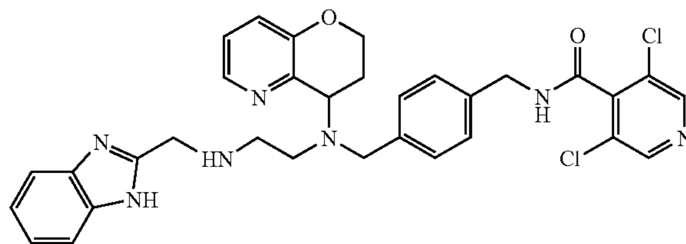
3,5-Dichloro-N-[3-((3,4-dihydro-2H-pyrano[3,2-b]pyridin-4-yl)-[2-(3H-imidazol-4-yl)-ethyl]-amino)-methyl]-benzyl]-isonicotinamide
