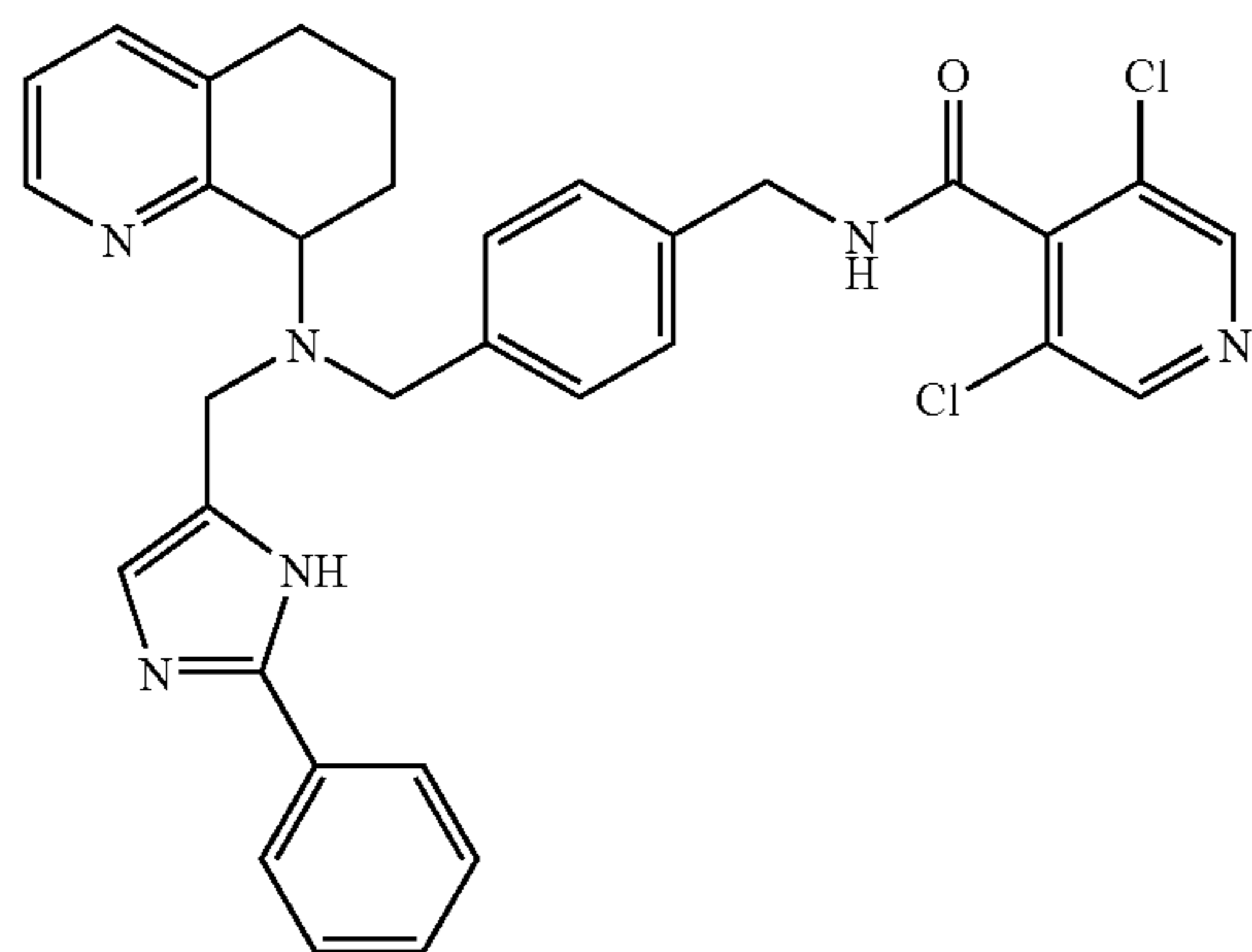
3,5-Dichloro-N-(4-(((2-phenyl-3H-imidazol-4-ylmethyl)-(5,6,7,8-tetrahydro-quinolin-8-yl)-amino)-methyl))-benzyl)-isonicotinamide
