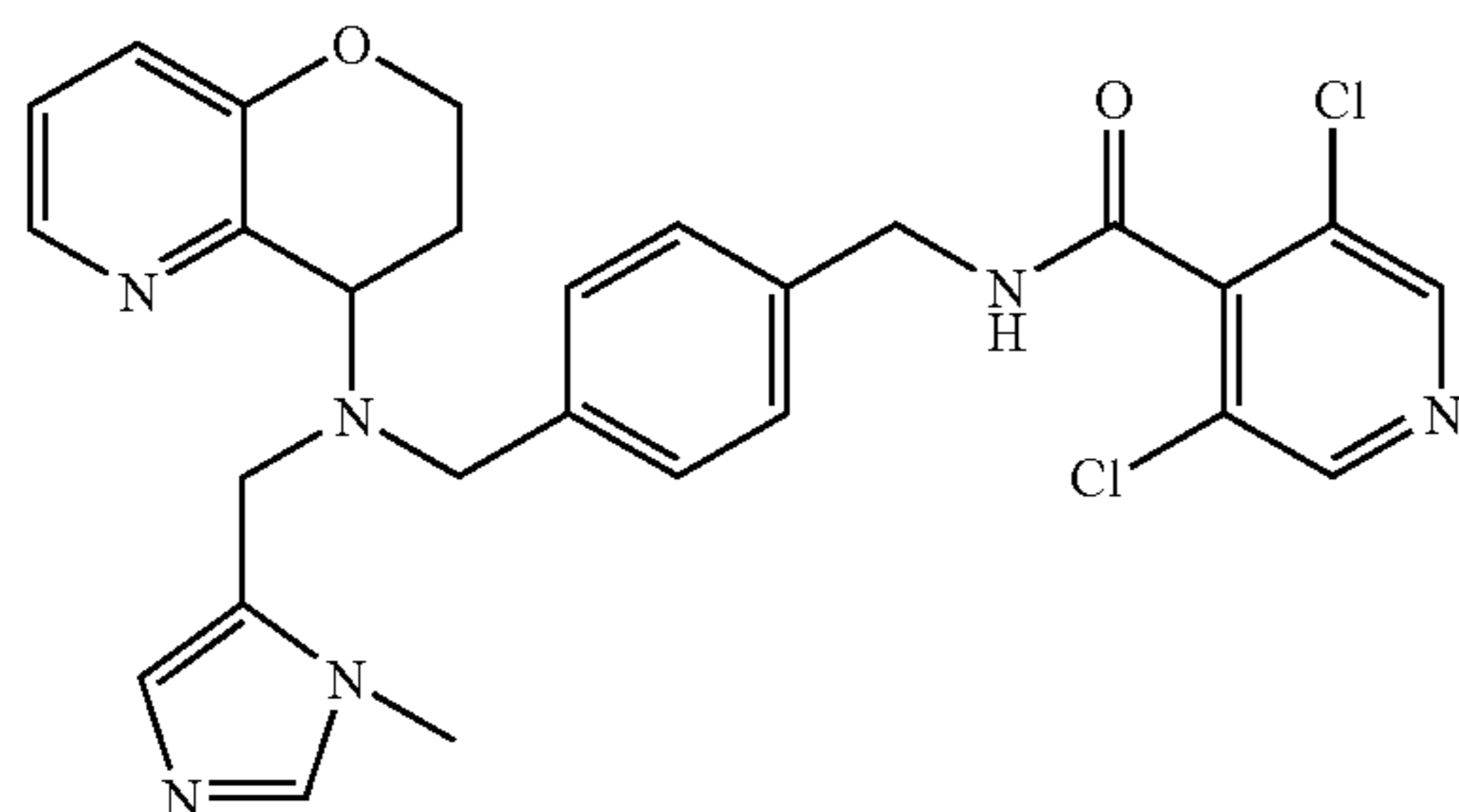
3,5-Dichloro-N-(4-[[3,4-dihydro-2H-pyrano[3,2-b]pyridin-4-yl)-(3-methyl-3H-imidazol-4-ylmethyl)-amino]-methyl)-benzyl)-isonicotinamide
