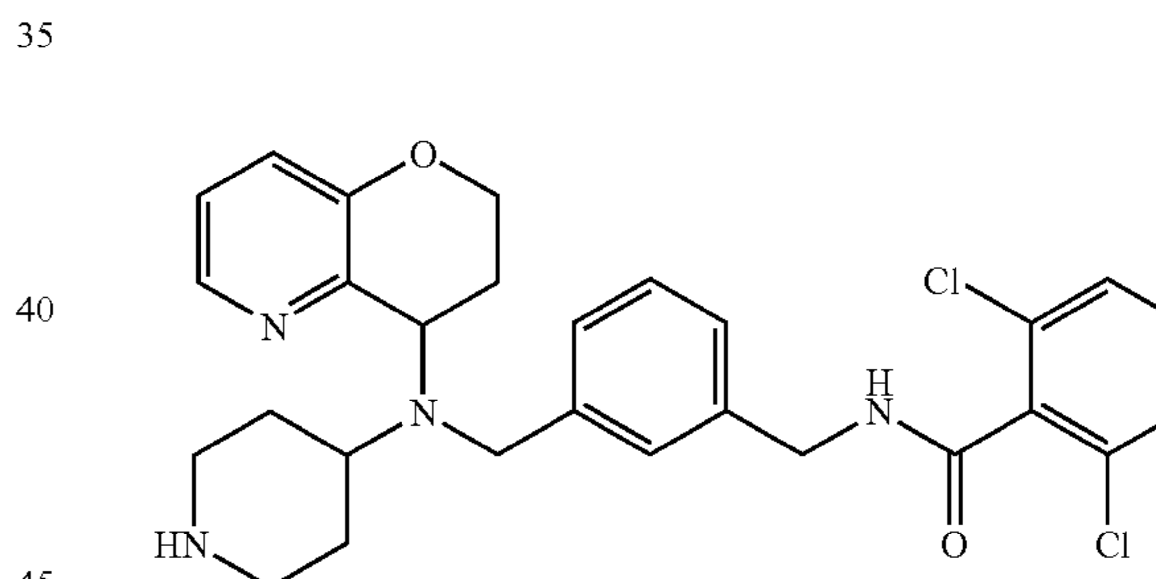
3,5-Dichloro-N-(4-[[3,4-dihydro-2H-pyrano[3,2-b]pyridin-4-yl)-piperidin-4-yl-amino]-methyl)-benzyl)-isonicotinamide
