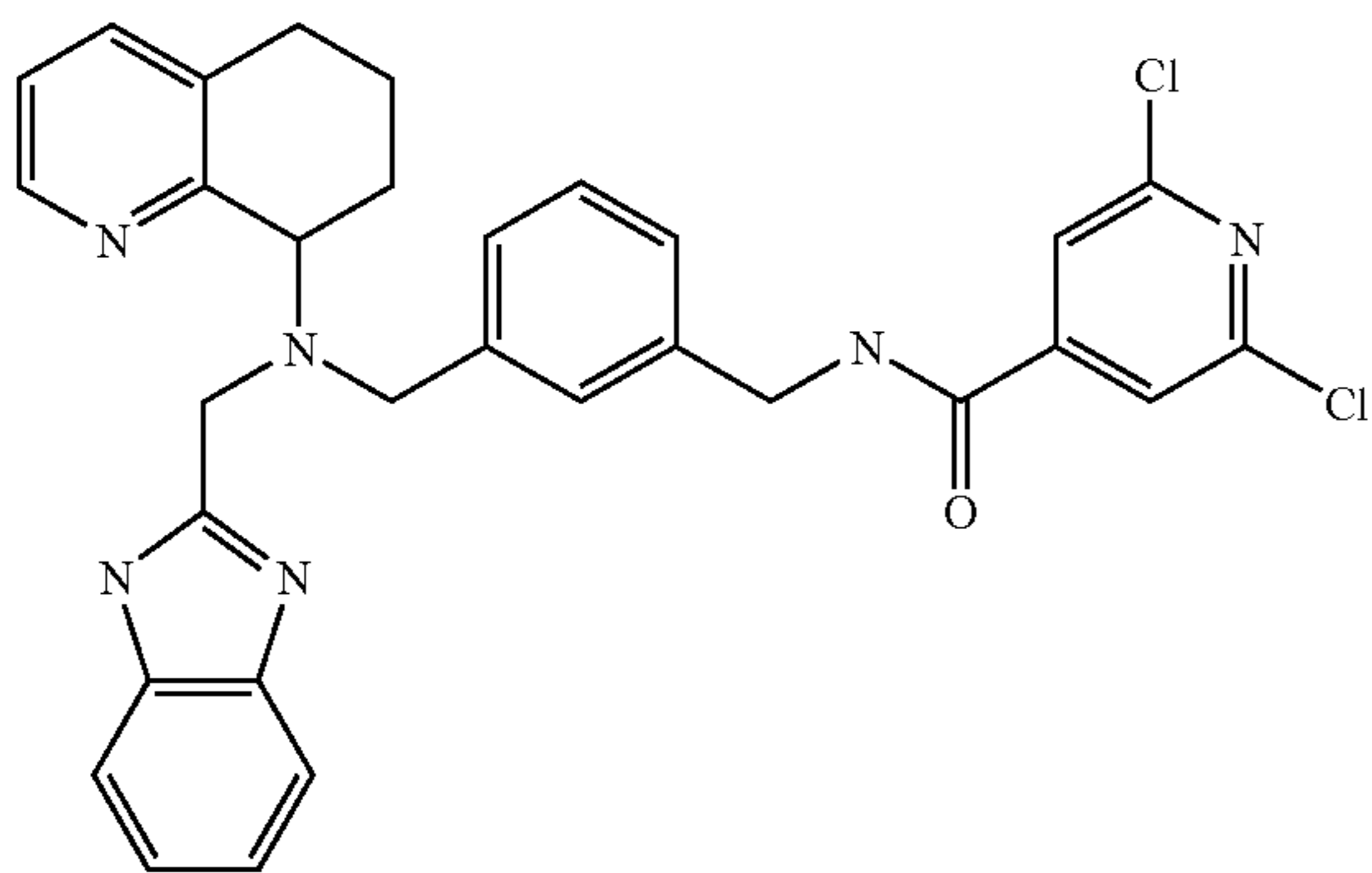
AMD9788: Preparation of: N-(3-(((1H-benzimidazol-2-ylmethyl)-(5,6,7,8-tetrahydro-quinolin-8-yl)-amino]-methyl)-benzyl)-2,6-dichloro-isonicotinamide
