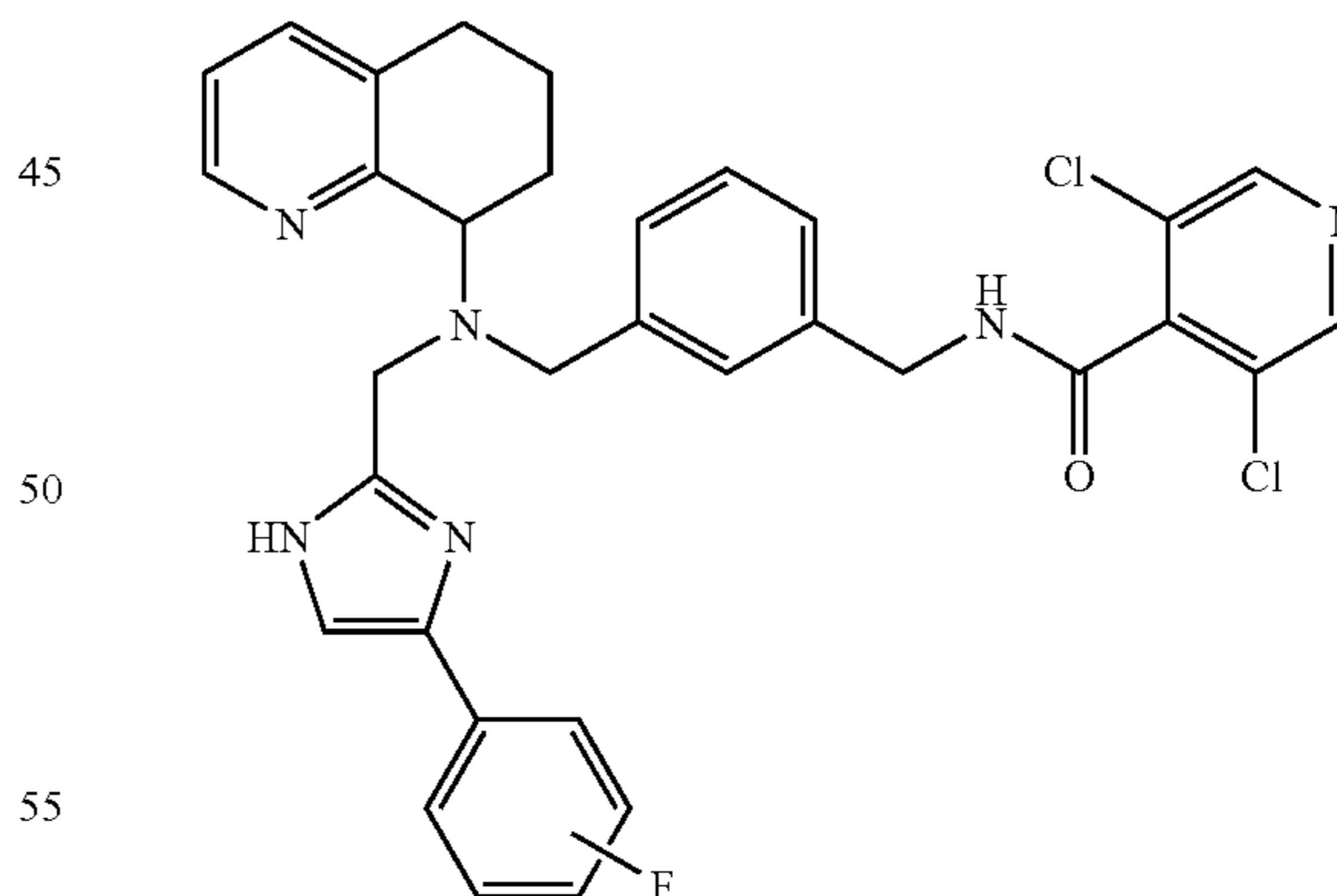
3,5-Dichloro-N-(4-[[[4-(4-fluoro-phenyl)-1H-imidazol-2-ylmethyl]-(5,6,7,8-tetrahydro-quinolin-8-yl)-amino]-methyl]-benzyl)-isonicotinamide
