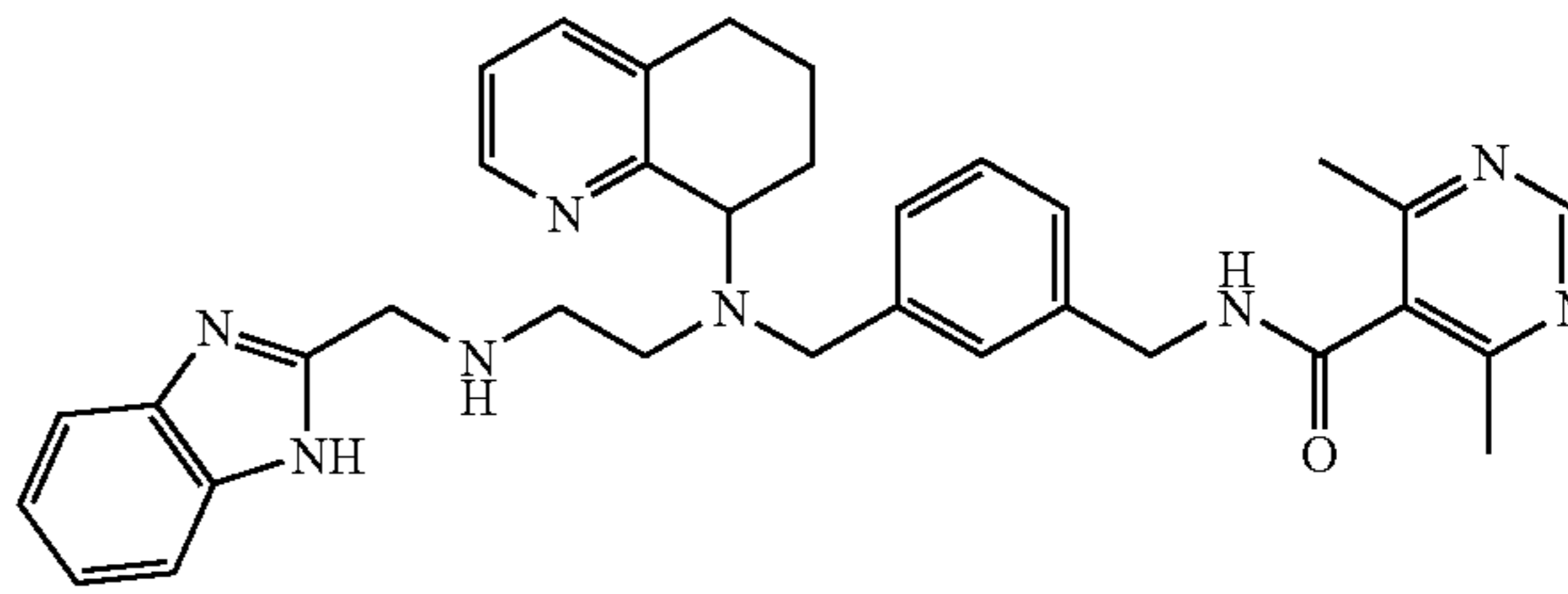
4,6-Dimethyl-pyrimidine-5-carboxylic acid 4-[[[2-[[[2-(1H-benzoimidazol-2-ylmethyl)-amino]-ethyl]-(5,6,7,8-tetrahydro-quinolin-8-yl)-amino]-methyl]-benzylamide
