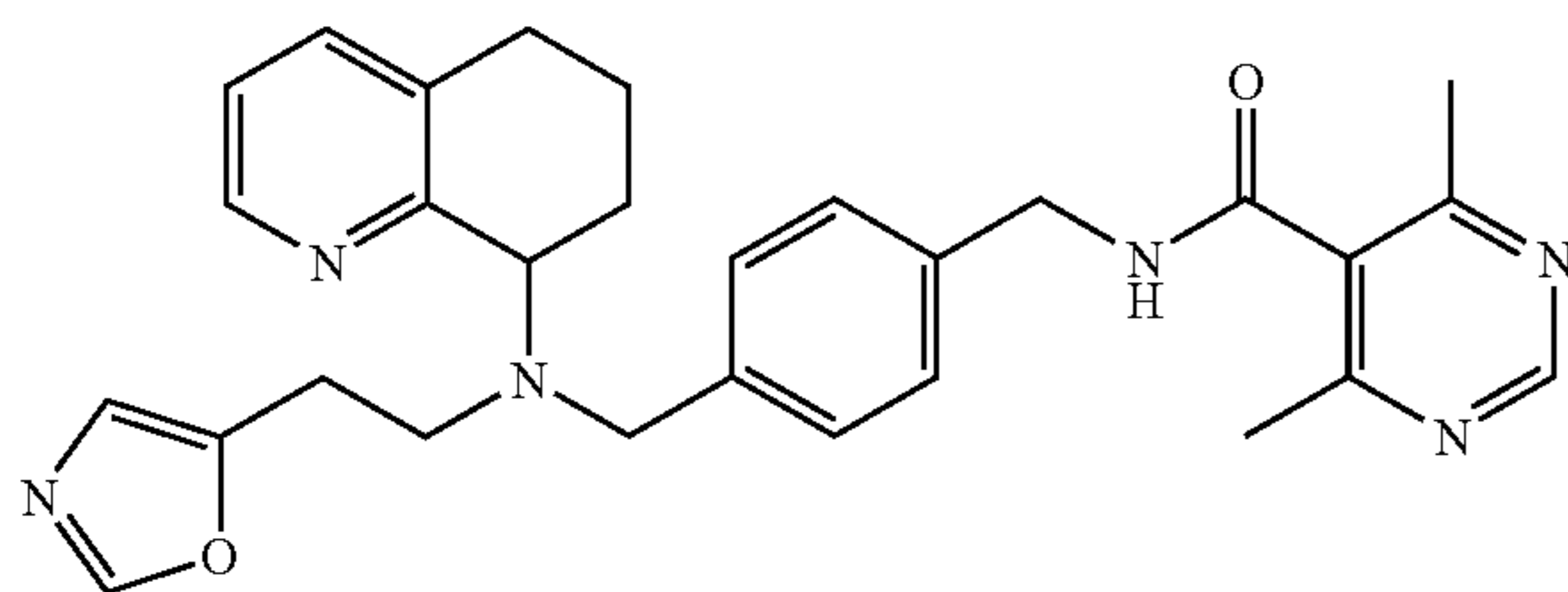
4,6-Dimethyl-pyrimidine-5-carboxylic acid 3-[[[2-(3-methyl-3H-imidazol-4-yl)-ethyl]-(5,6,7,8-tetrahydro-quinolin-8-yl)-amino]-methyl]-benzylamide
