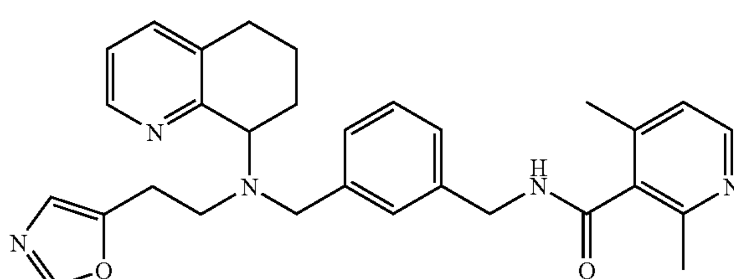
5 2,4-Dimethyl-N-(4-[[[2-oxazol-5-yl-ethyl]-(5,6,7,8-tetrahydro-quinolin-8-yl)-amino]-methyl]-benzyl)-nicotinamide
