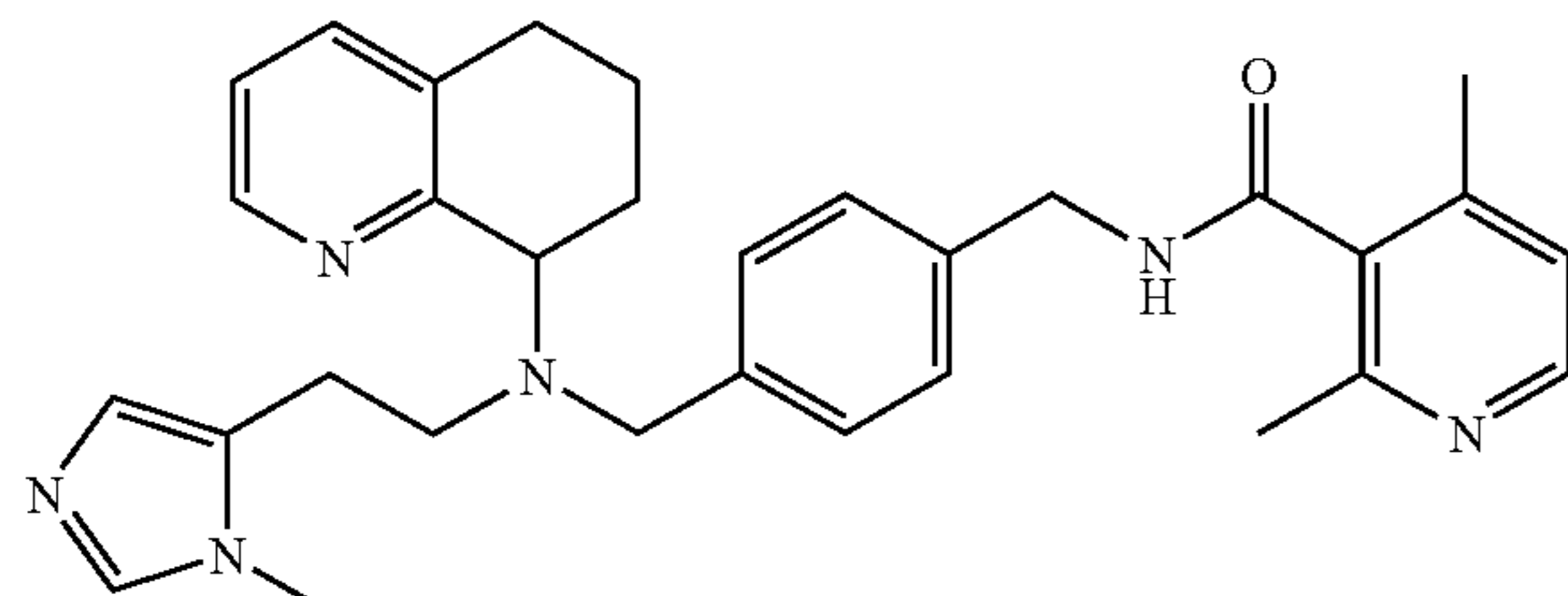
N-(3-[[[2-(3H-Imidazol-4-yl)-ethyl]-(5,6,7,8-tetrahydro-quinolin-8-yl)-amino]-methyl]-benzyl)-2,4-dimethyl-nicotinamide
