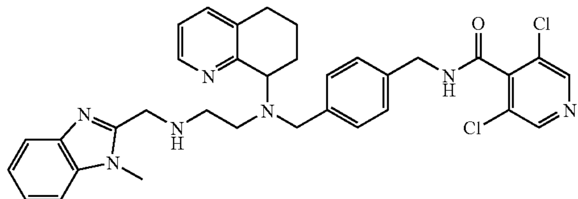
3,5-Dichloro-N-(4-[[2-[(1-methyl-1H-benzoimidazol-2-ylmethyl)-amino]-ethyl]- (5,6,7,8-tetrahydro-quinolin-8-yl)-amino]-methyl)-benzyl)-isonicotinamide
