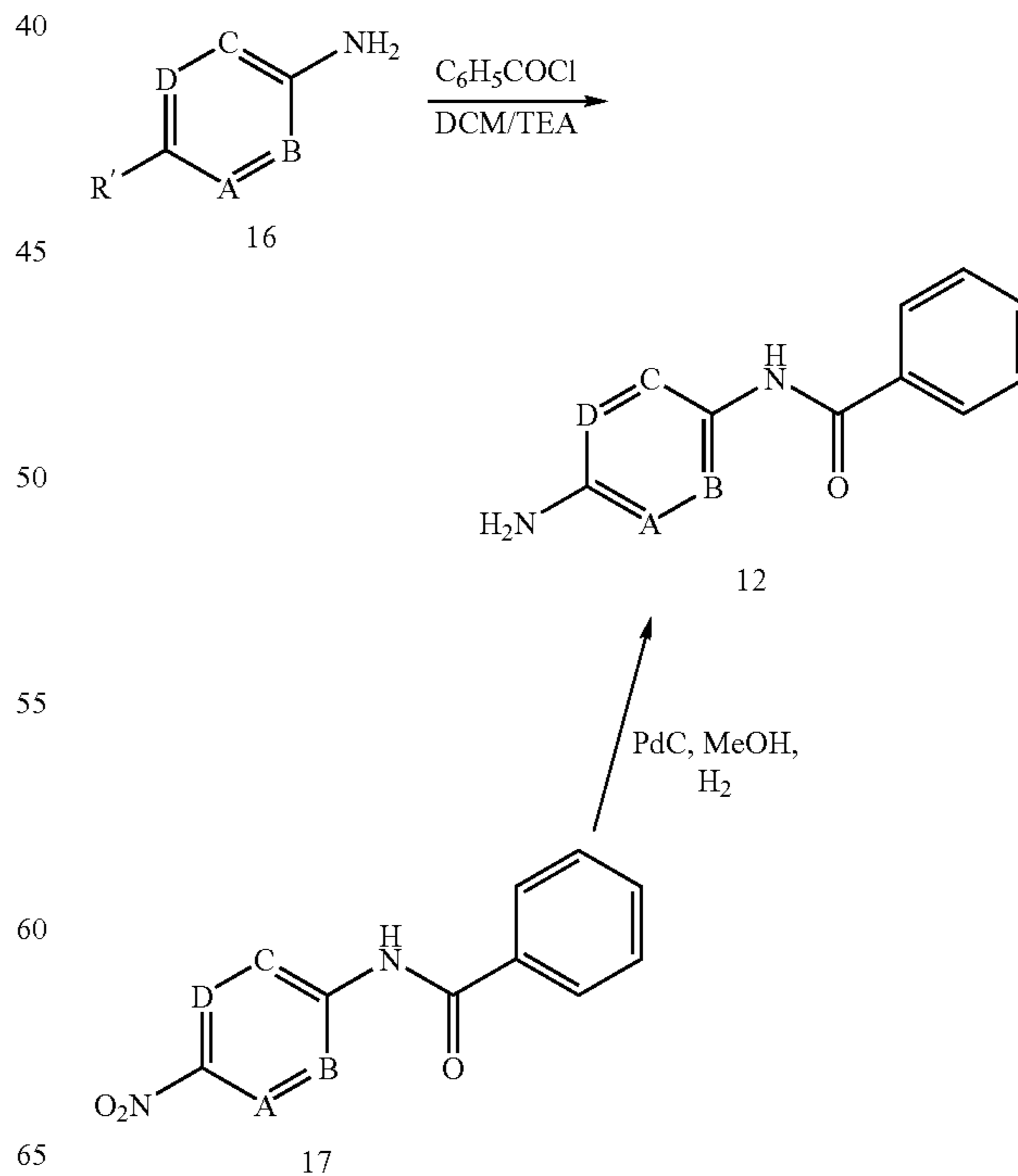
Scheme 13
