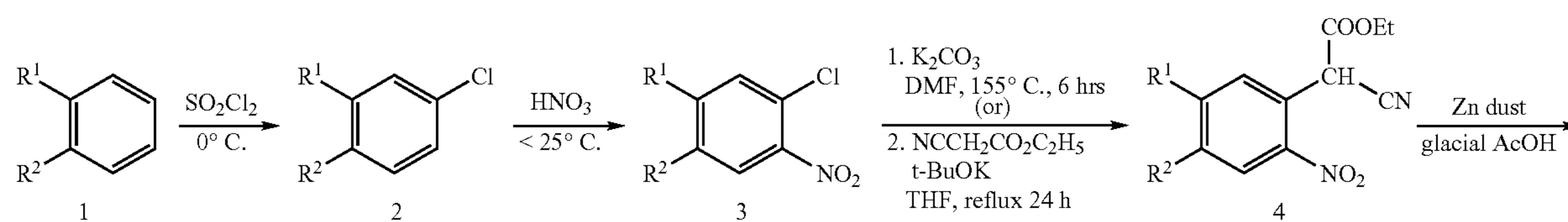
Scheme 11
