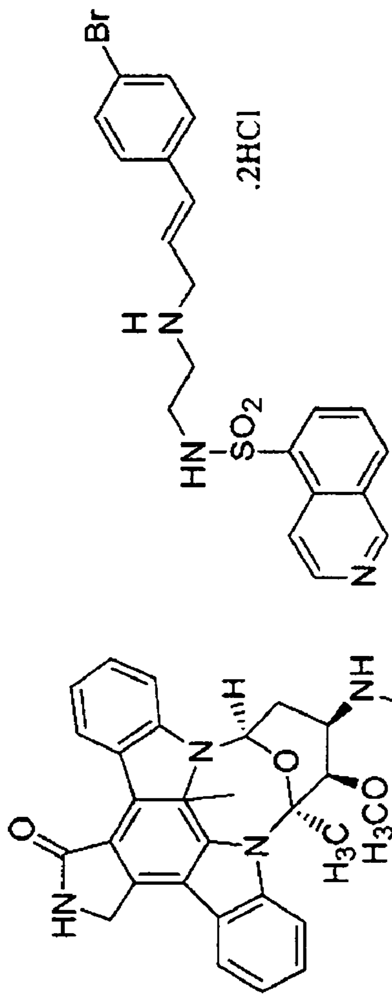
Staurosporine H-89
