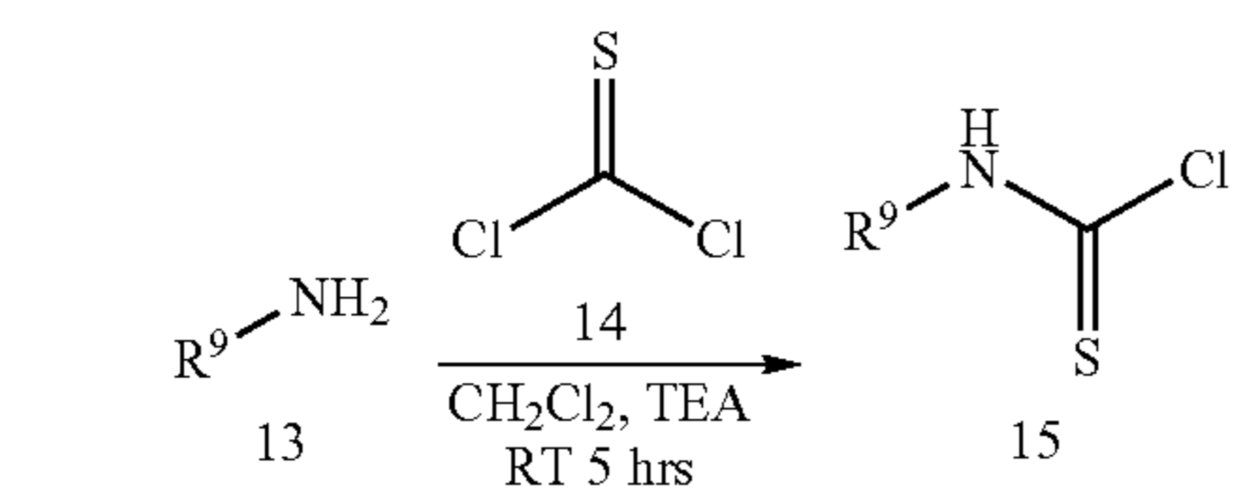
Scheme 12
