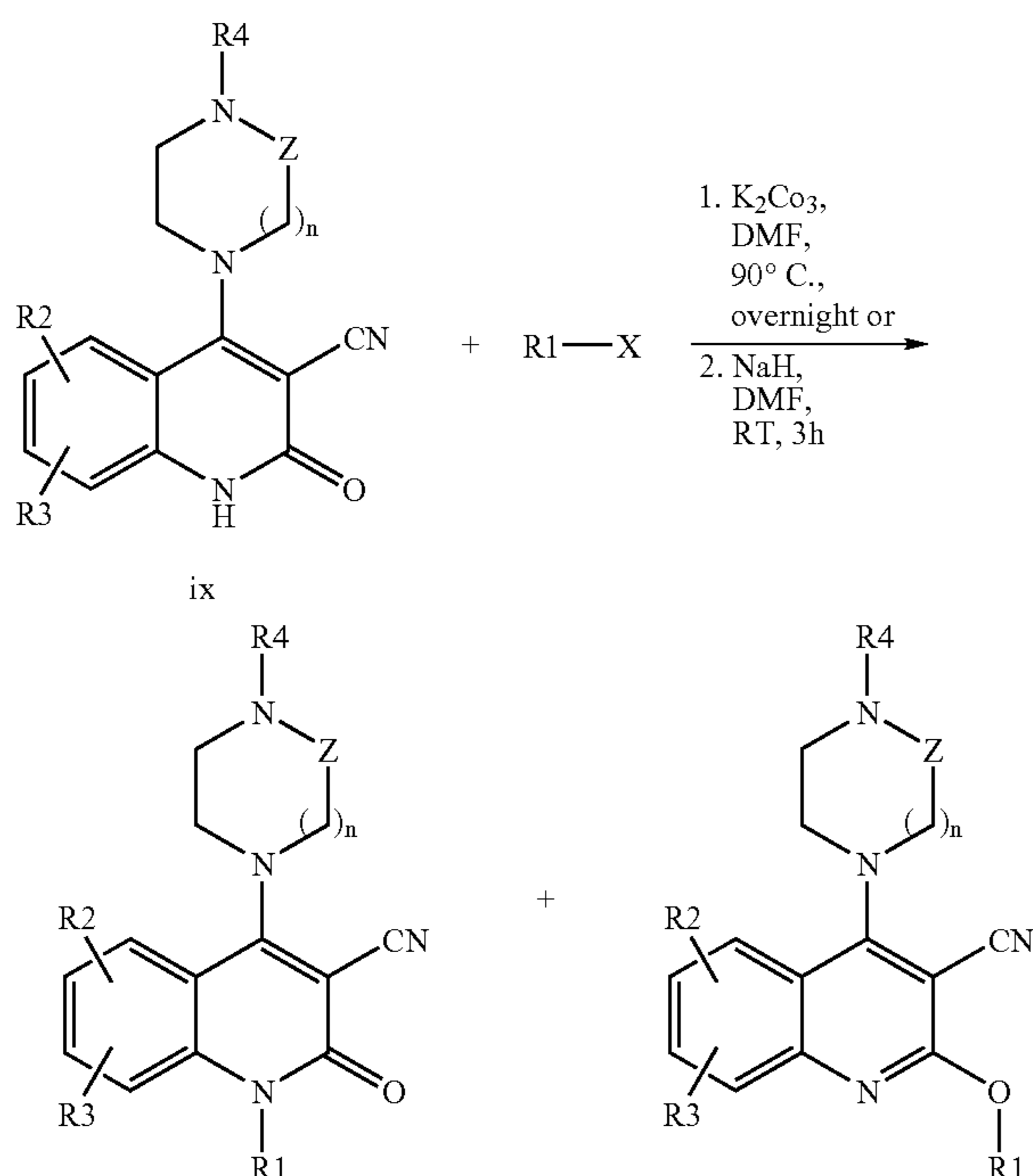
Reaction Scheme 6
