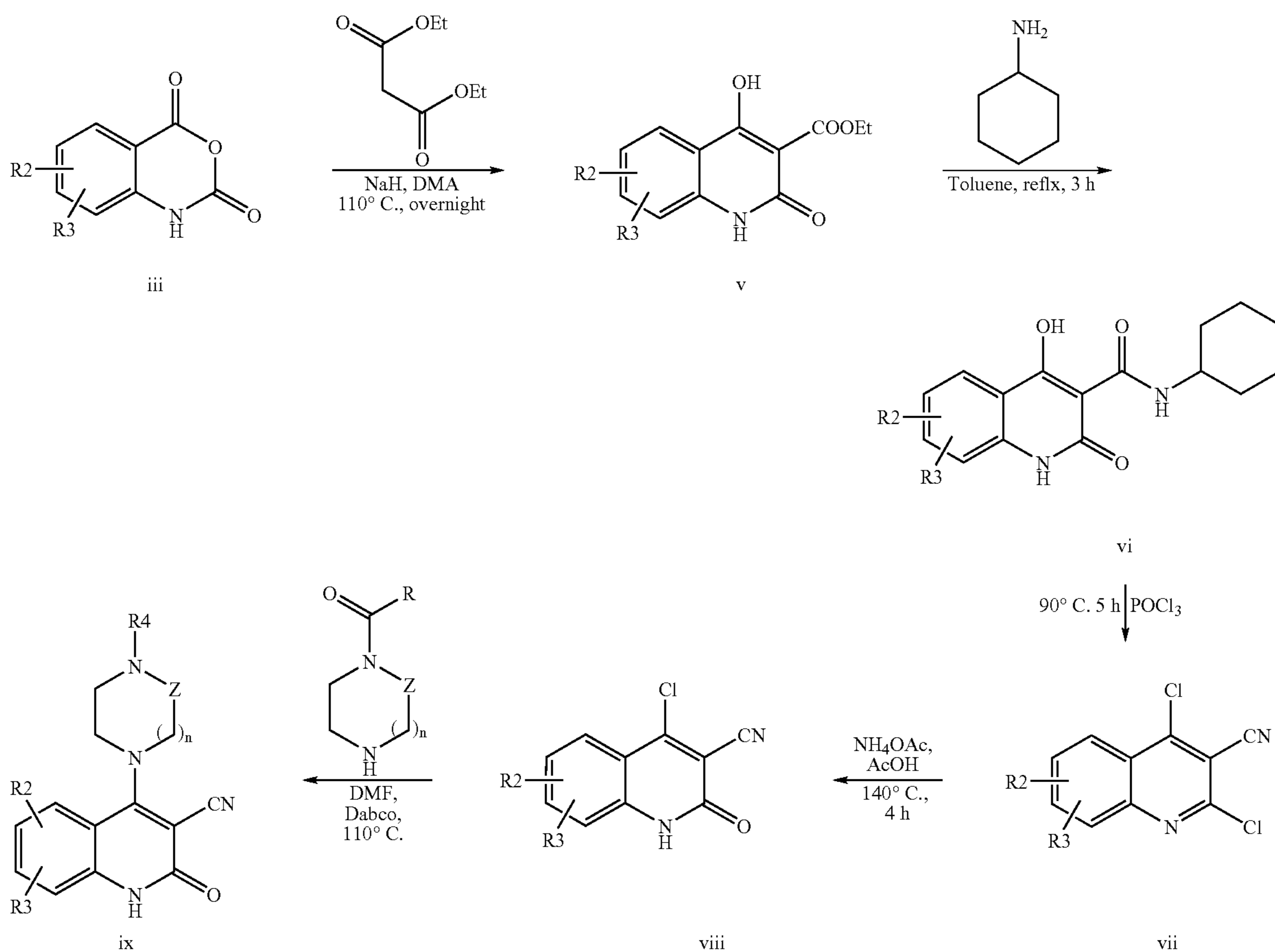
Reaction Scheme 4
