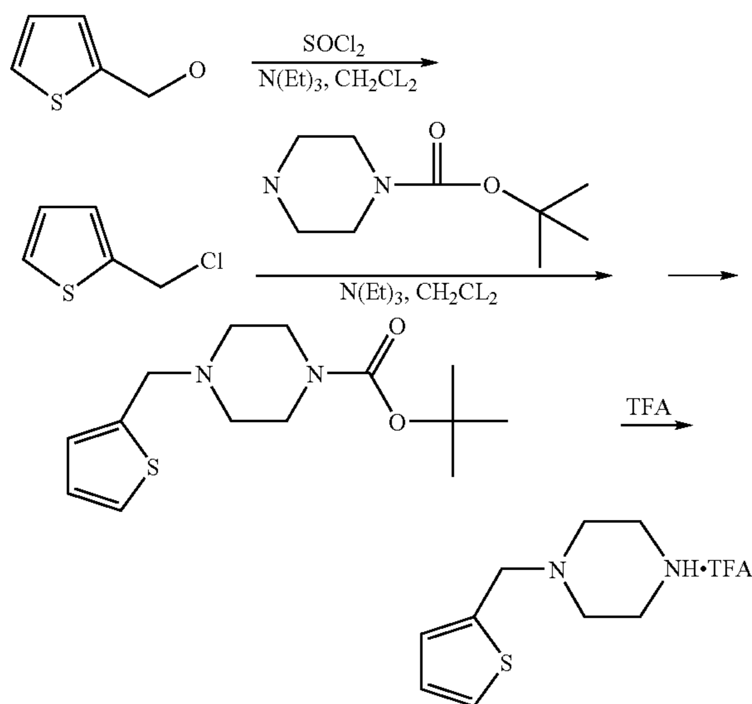
Reaction Scheme 6
