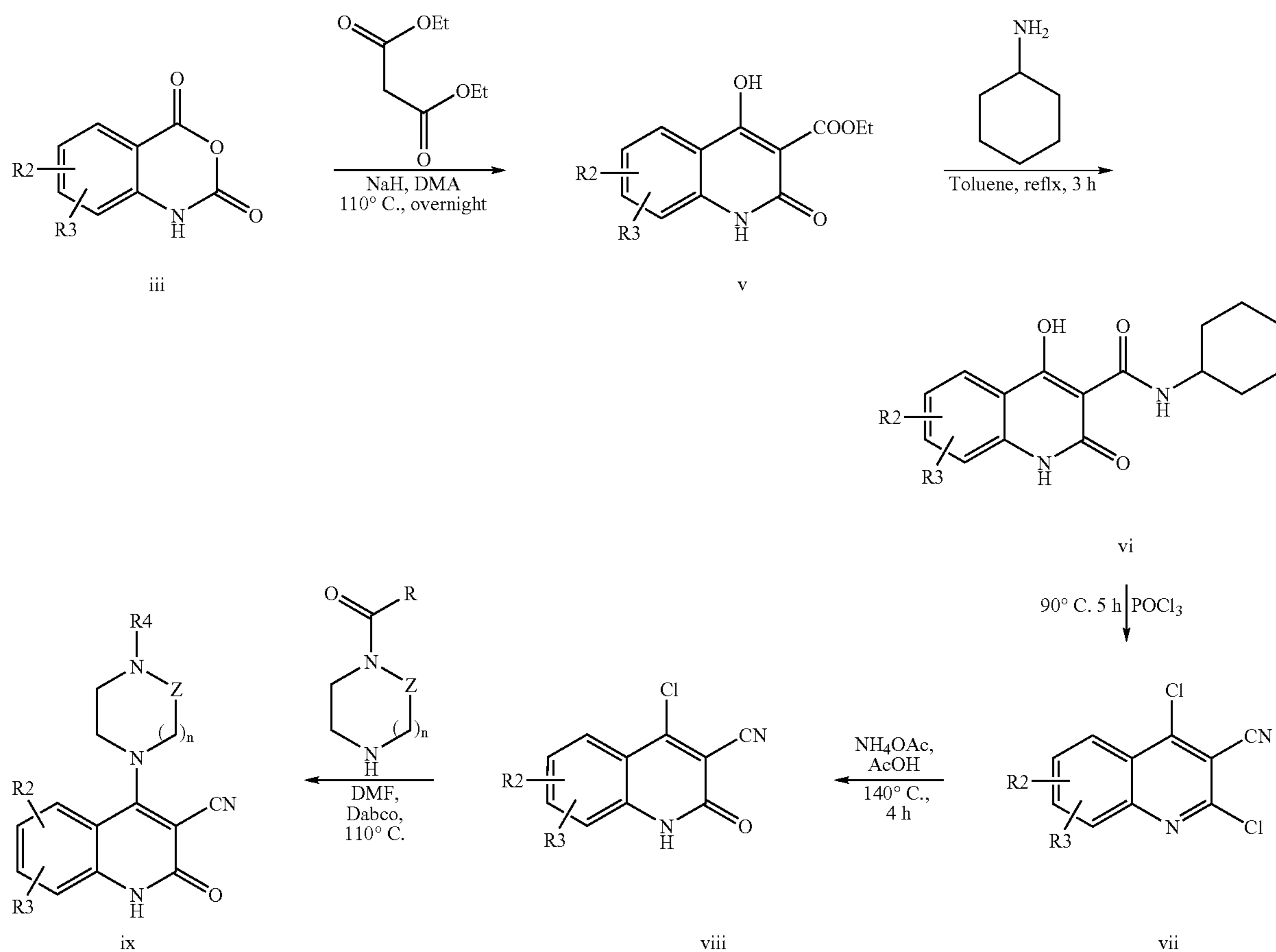
Reaction Scheme 4
