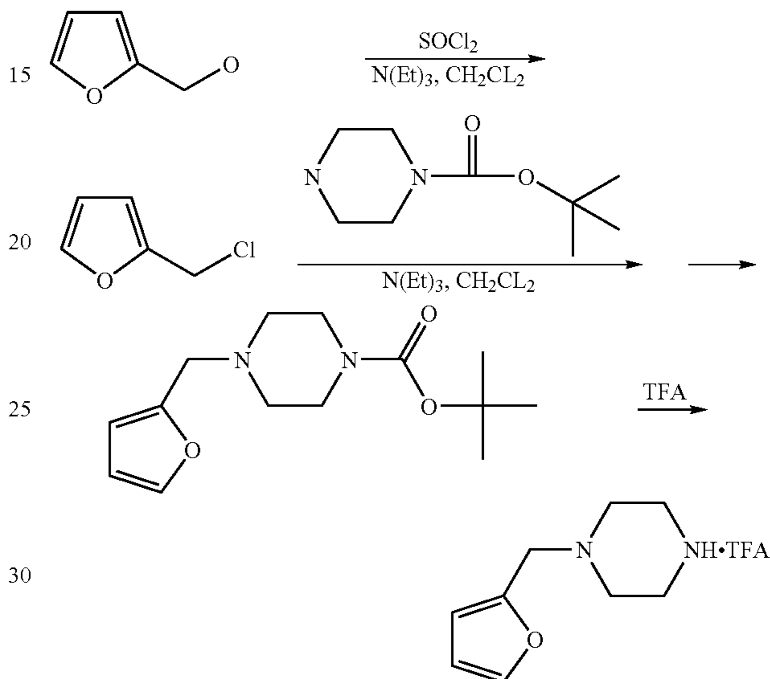
Reaction Scheme 7
