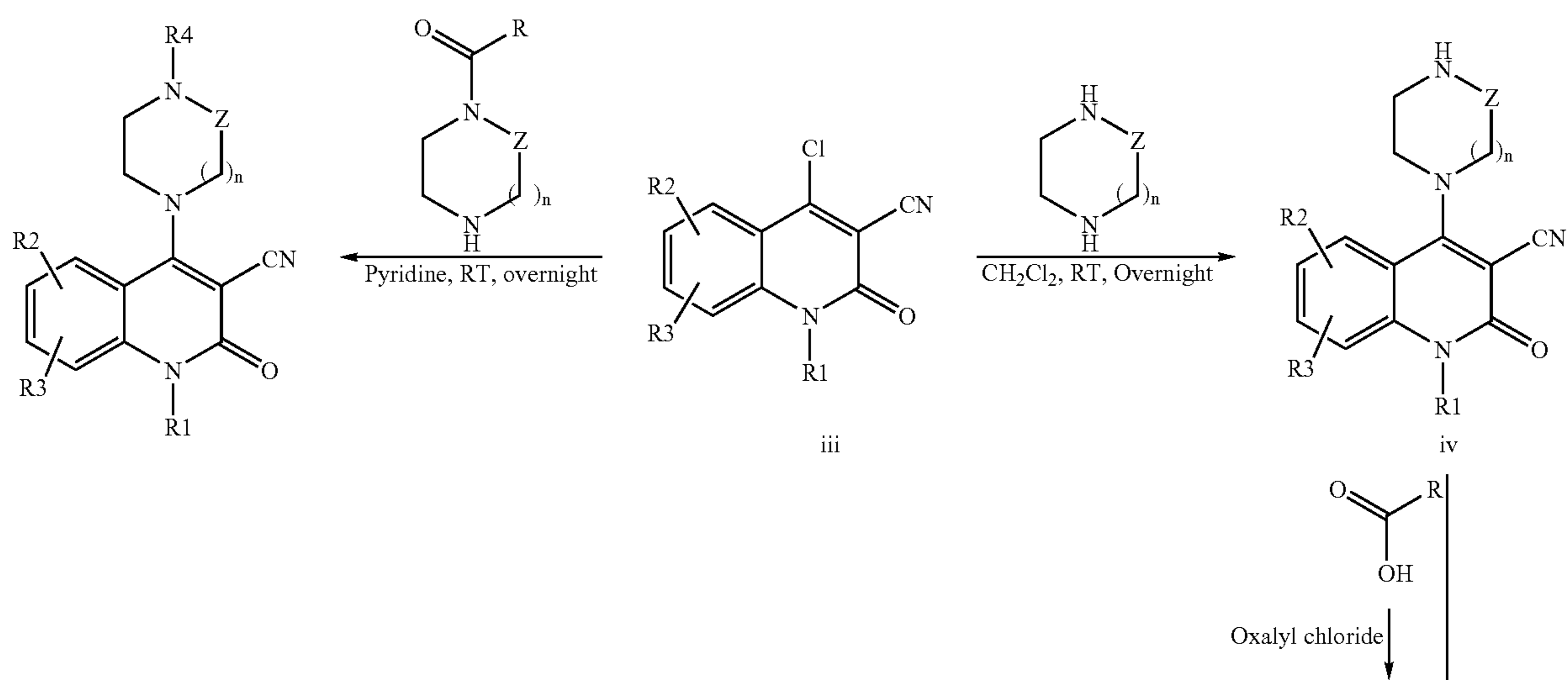
Reaction Scheme 3
