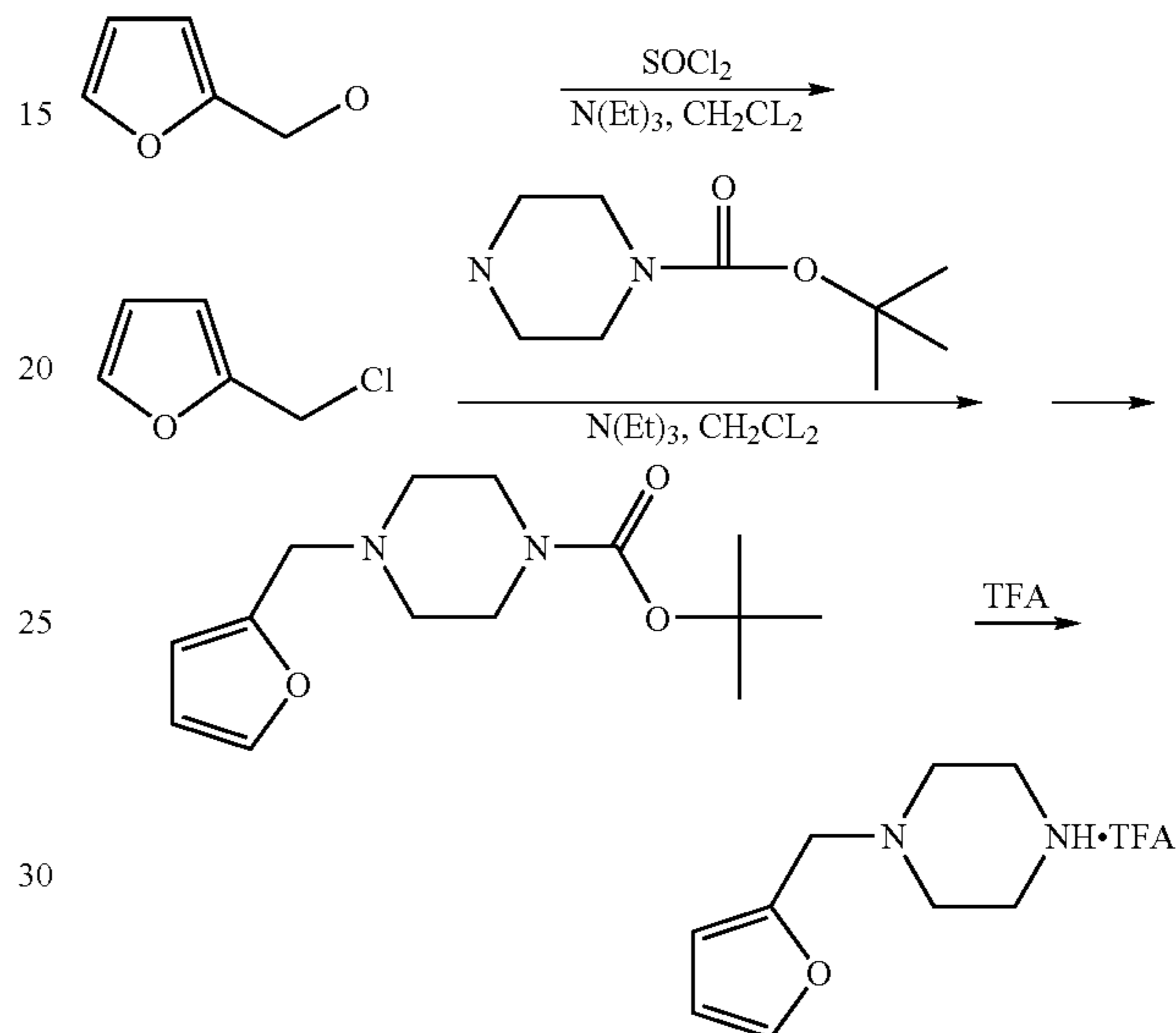
Reaction Scheme 7
