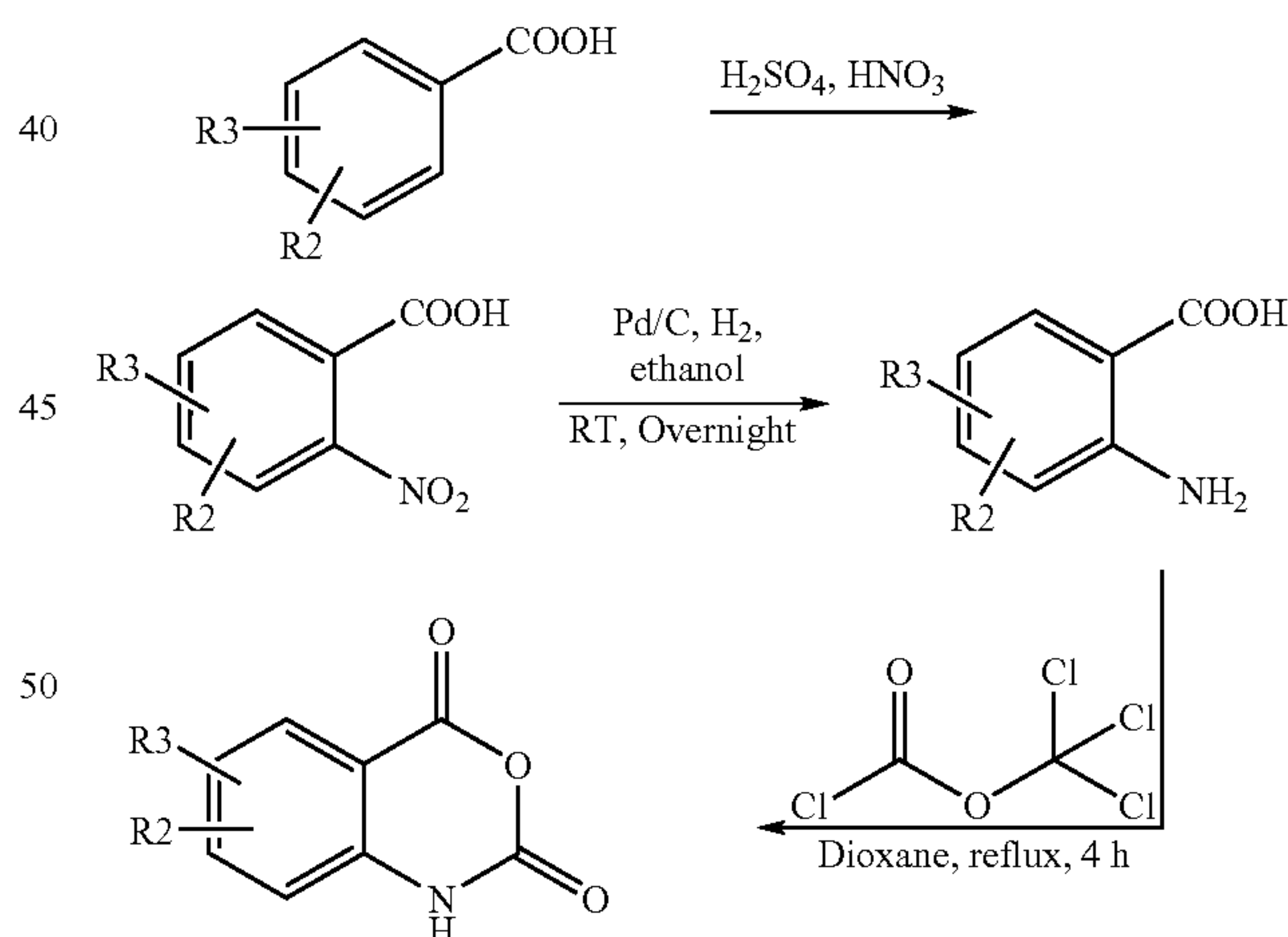
Reaction Scheme 1
