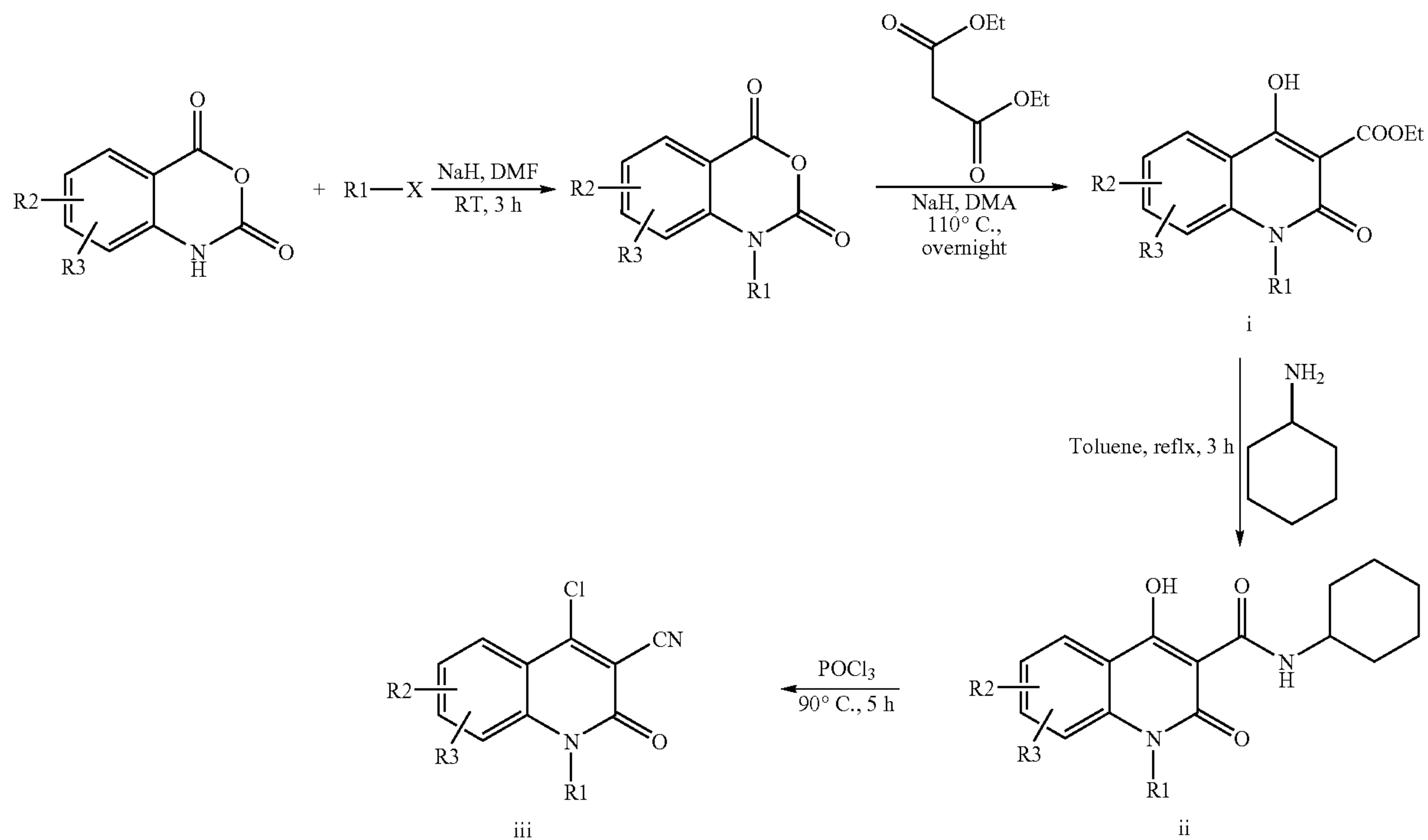
Reaction Scheme 2
