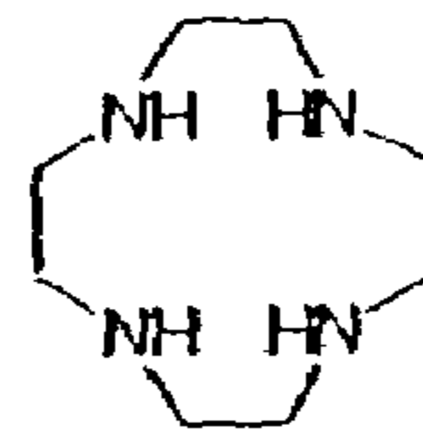
1,4,7,10-Tetraaza cyclododecane
