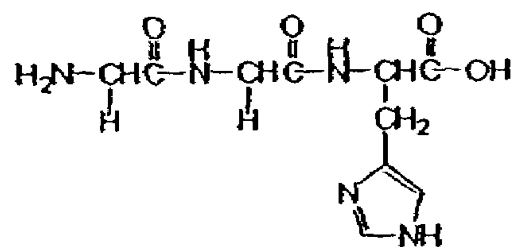
Glycyl-glycyl-histidine (GGH)
