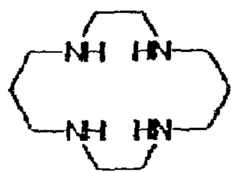
1,4,8,11-Tetraaza cyclotetradecane
