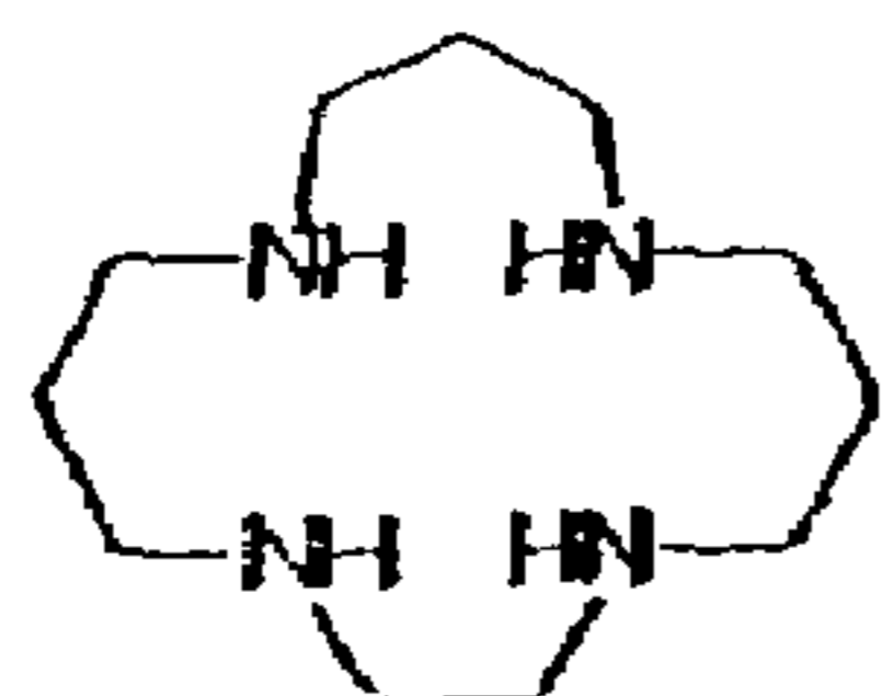
1,4,8,12-tetraaza cyclopentadecane
