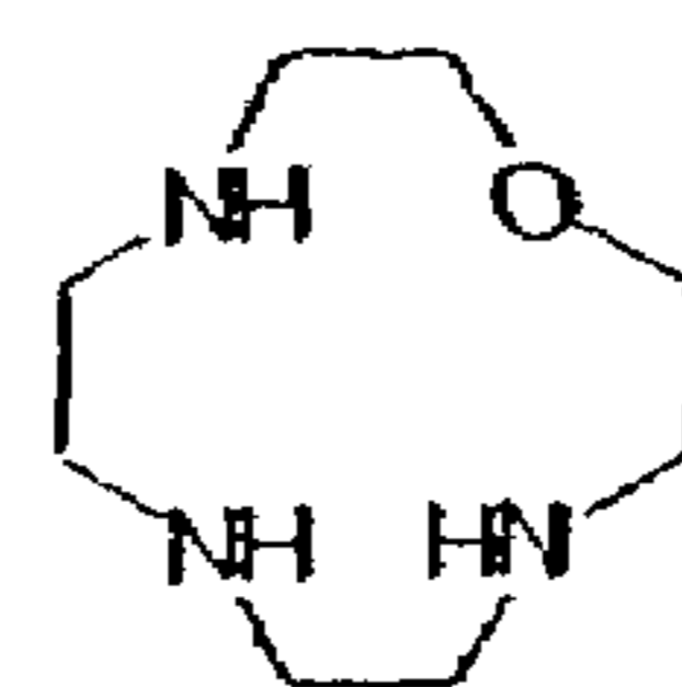
1-Oxa-4,7,10-triazacyclododecane
