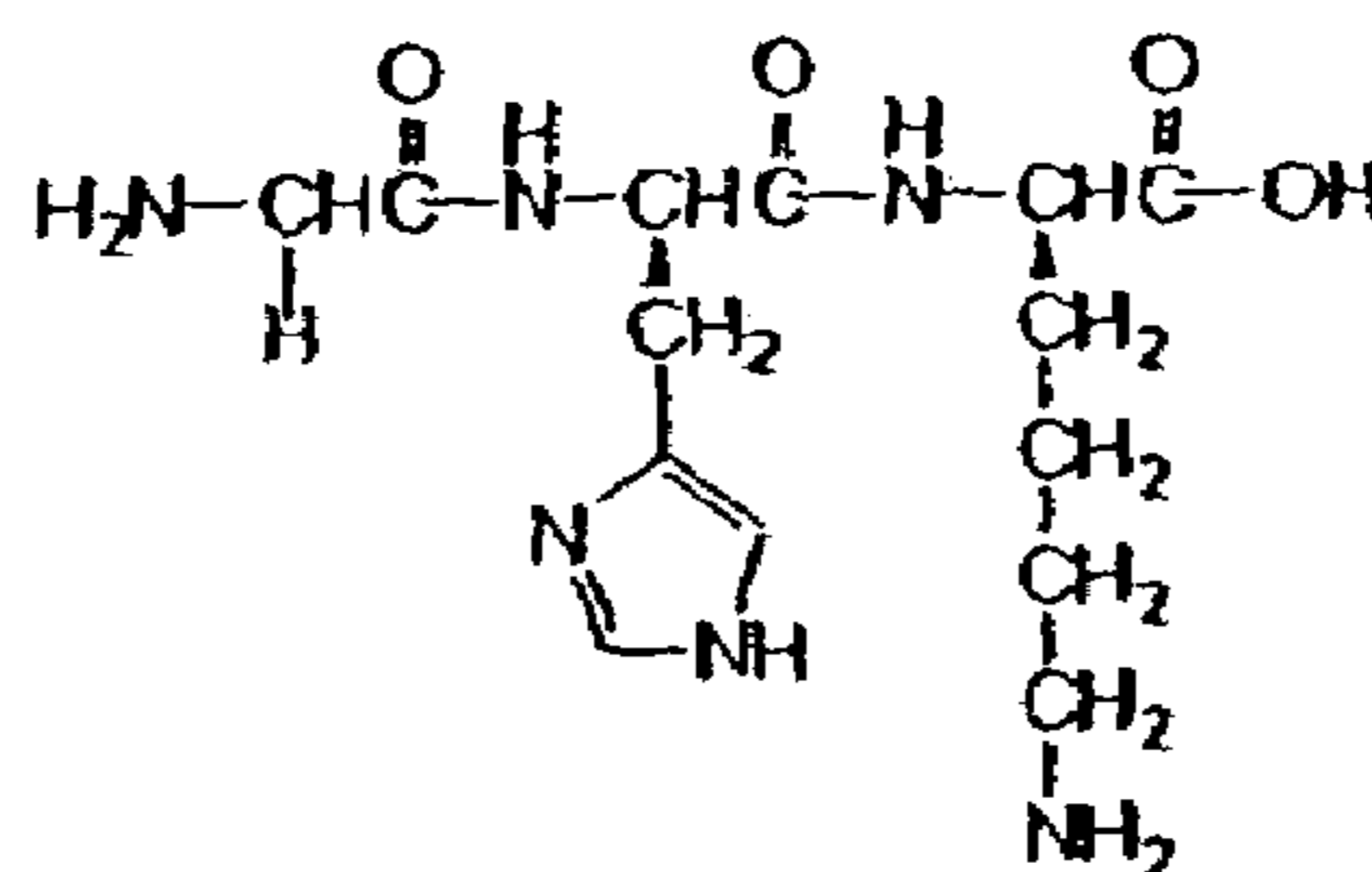
Glycyl-histidyl-lysine (GHK)
