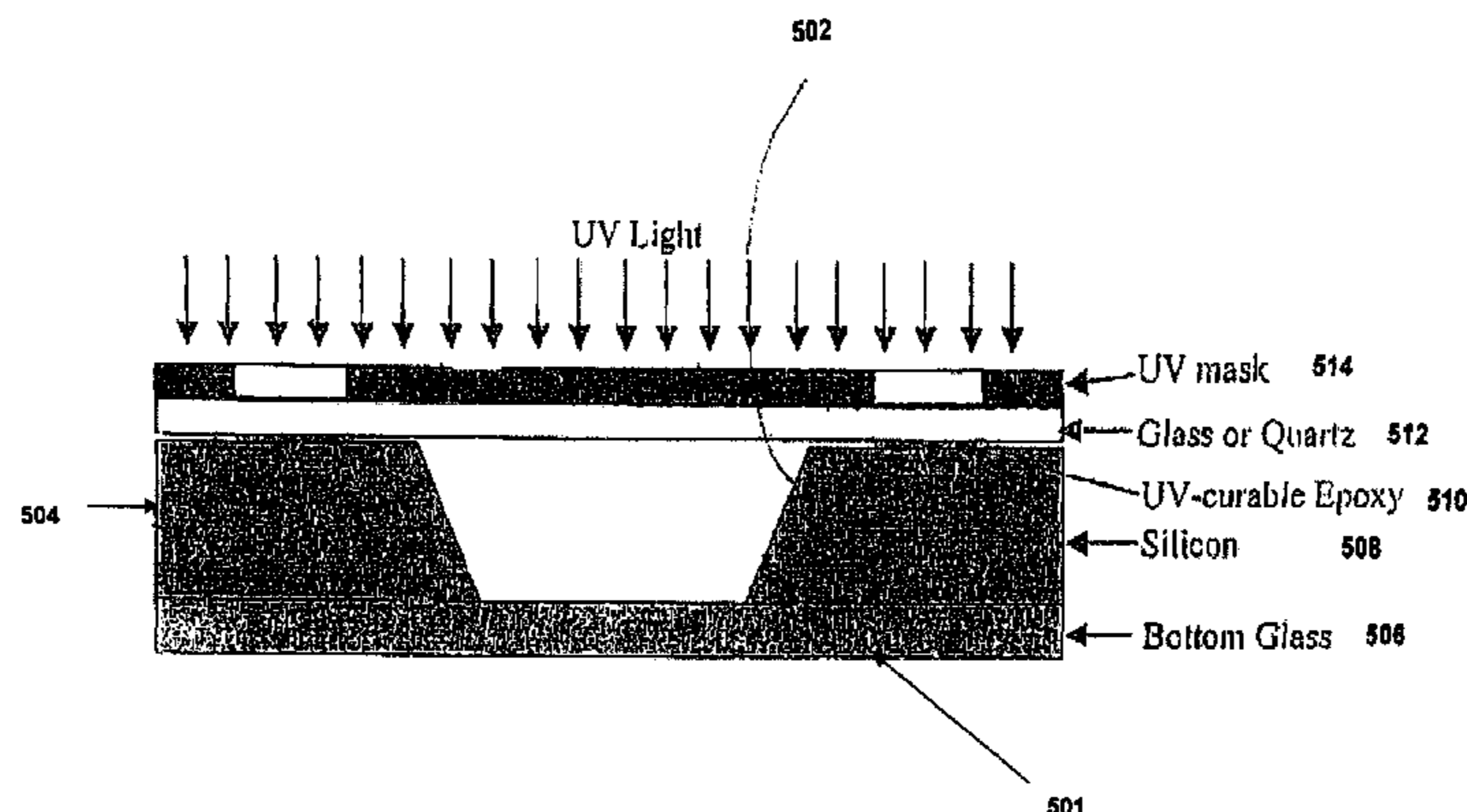
UV-curing sealing process
