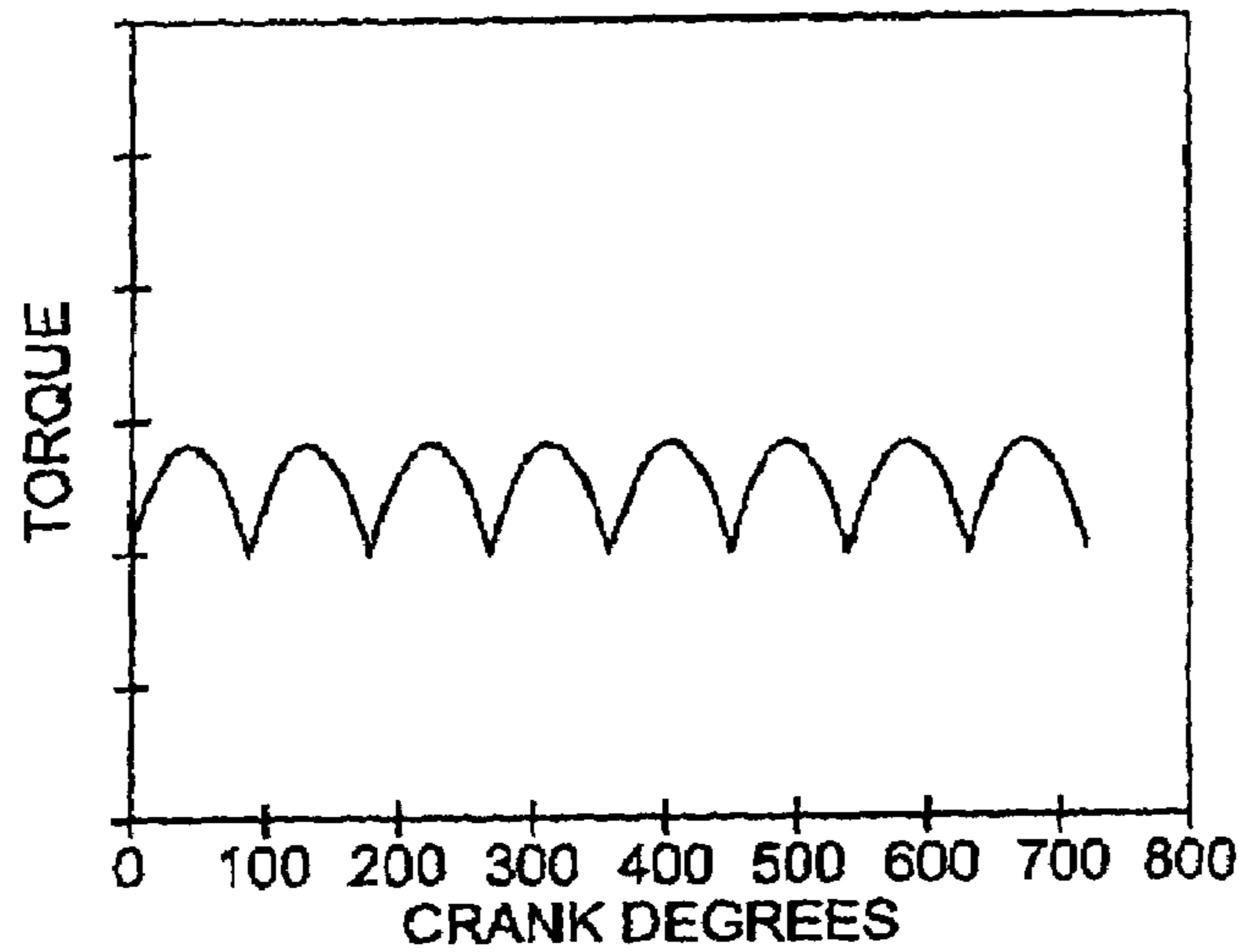
TORQUE PULSATIONS FOR ALL 8 CYLINDERS FIRING
