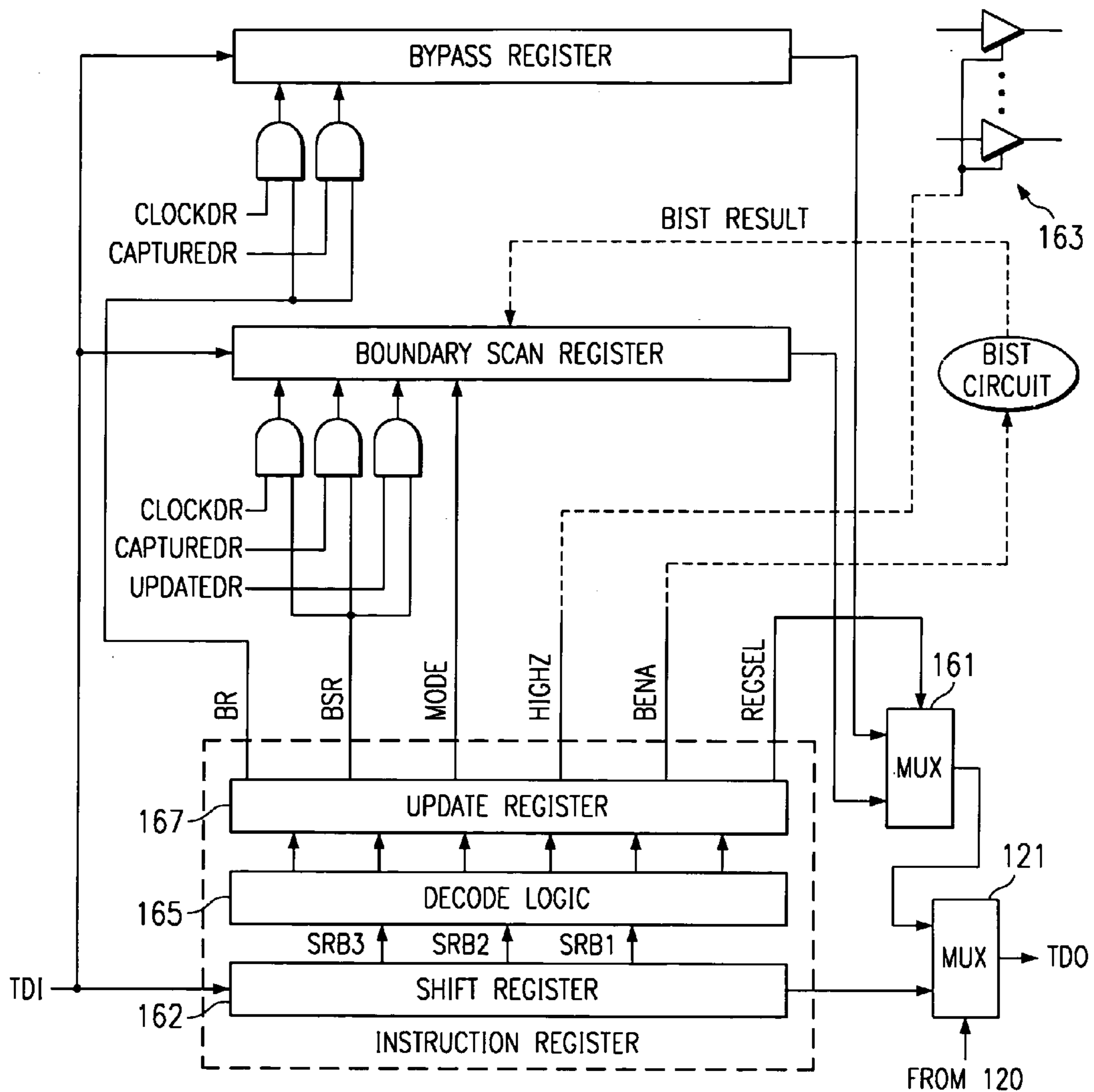
FIG. 16 (PRIOR ART)
