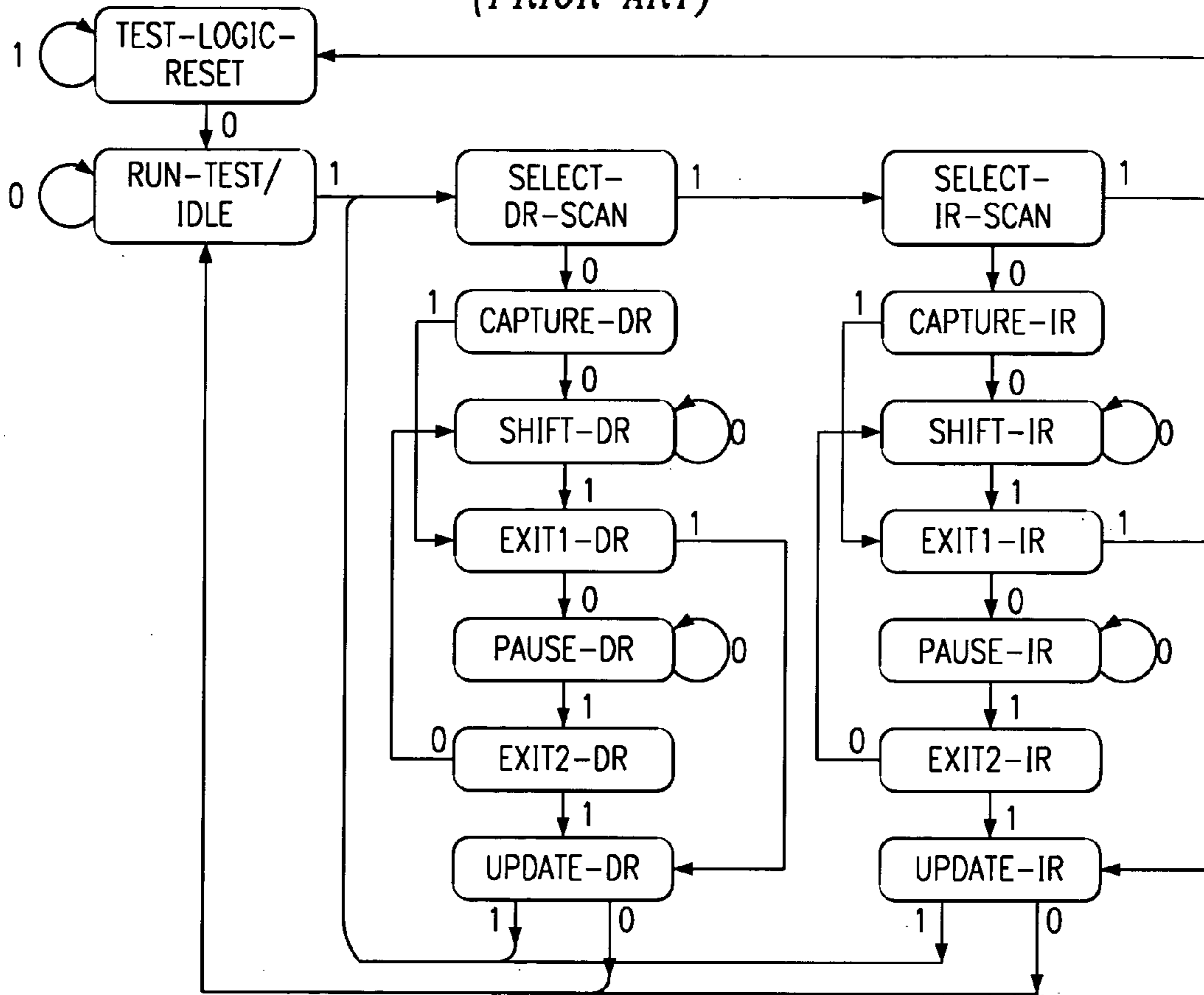
FIG. 14 (PRIOR ART)
