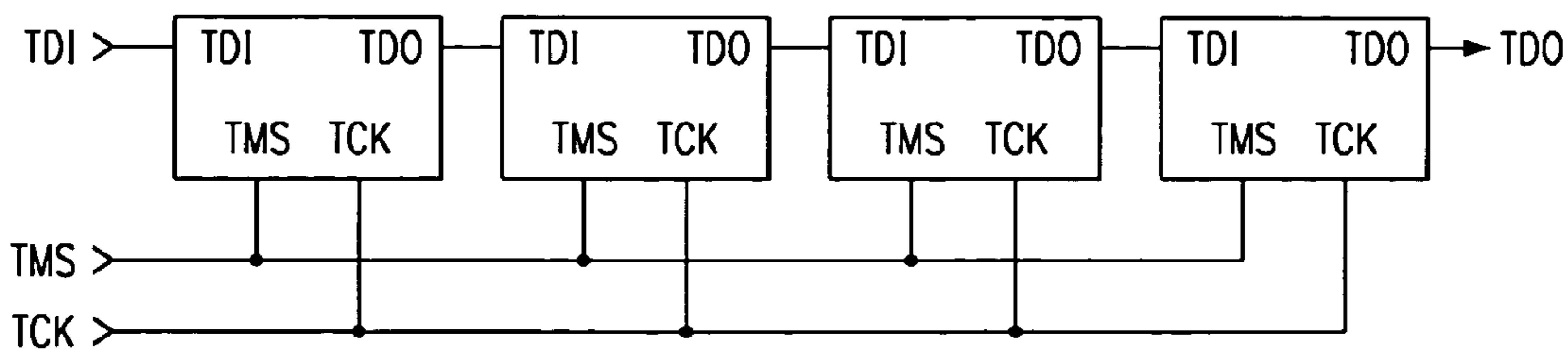
FIG. 13 (PRIOR ART)
