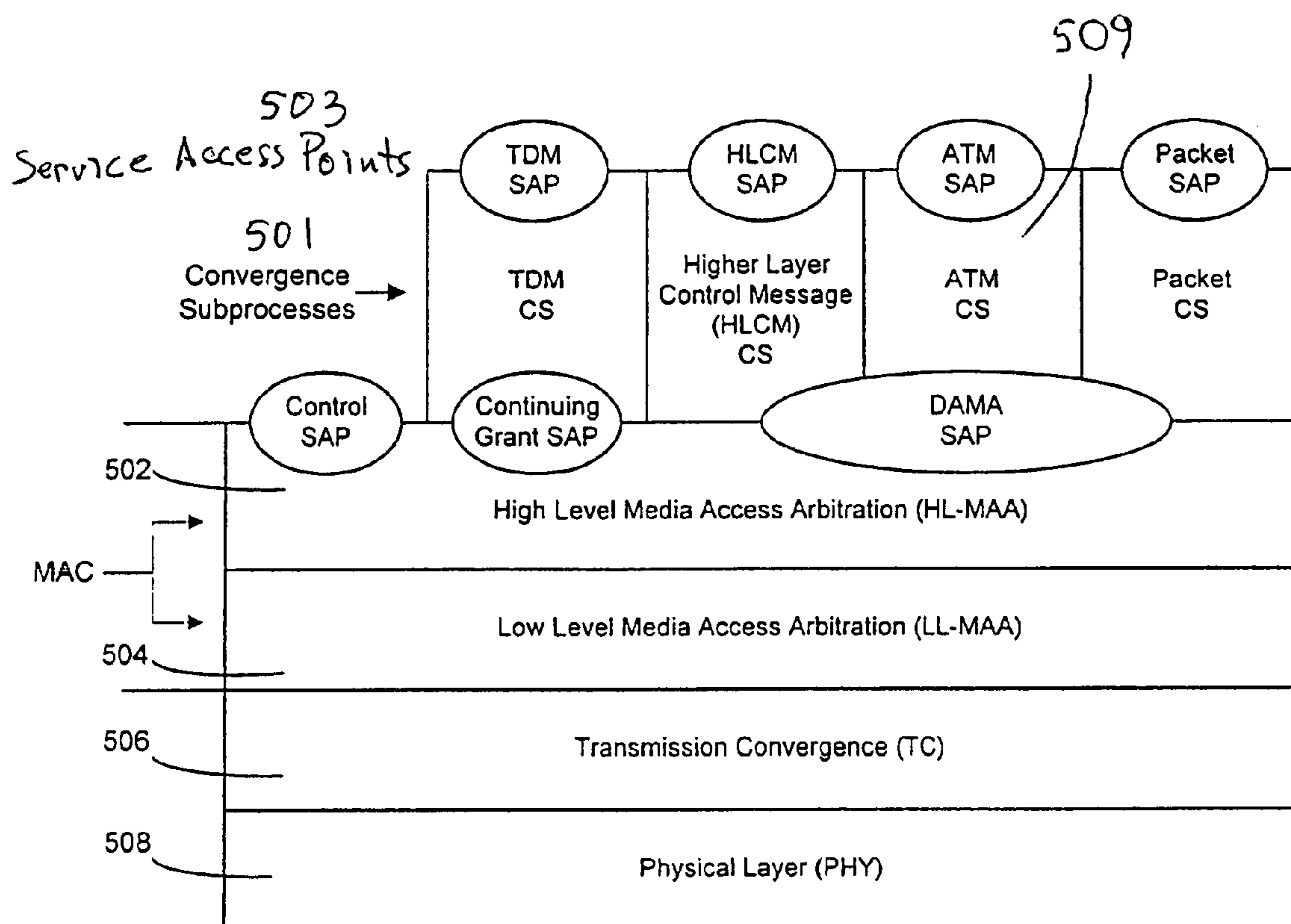
Layered Data Transport Architecture
