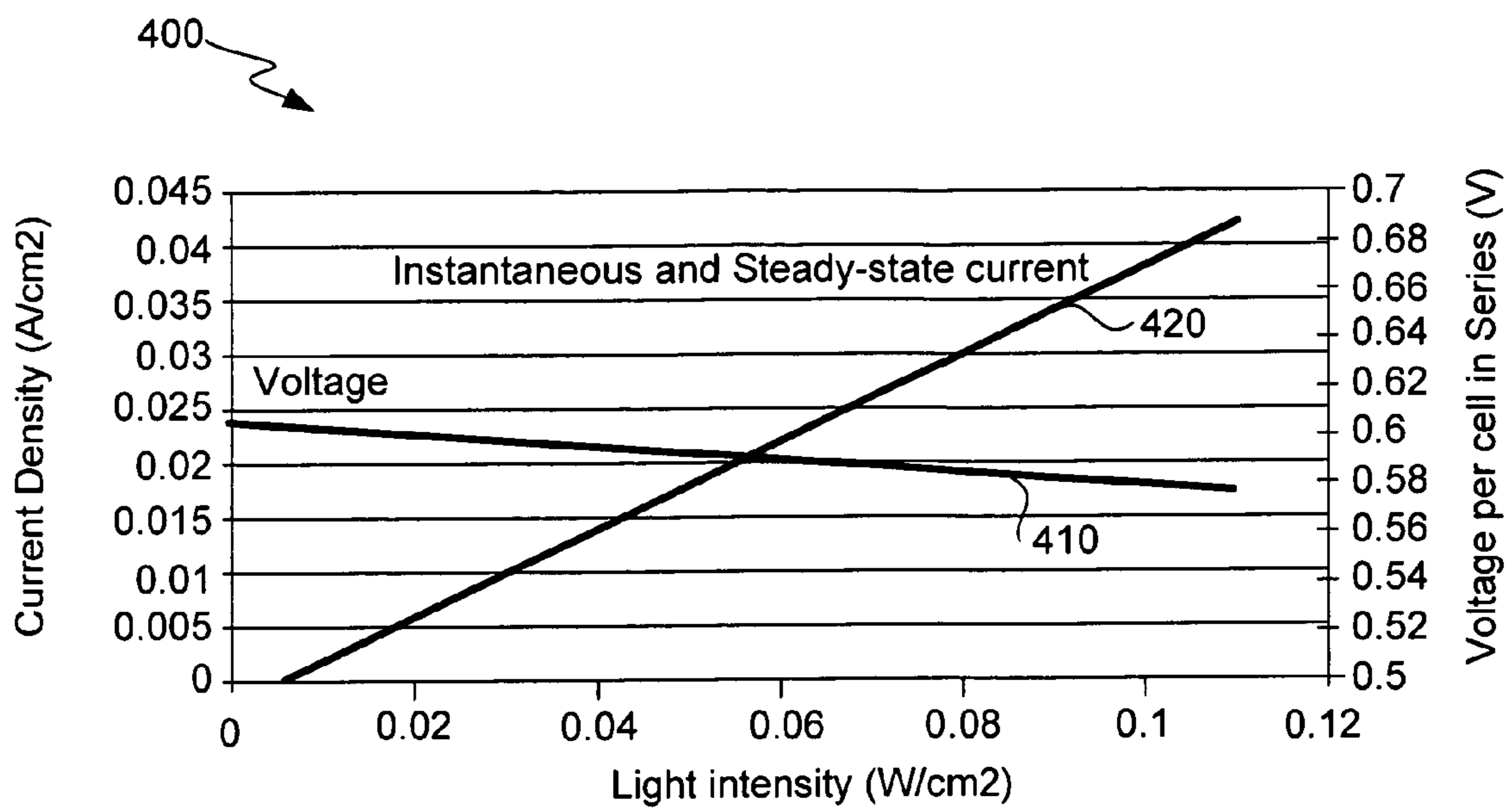
FIG. 5 Current Density vs. Light Intensity
