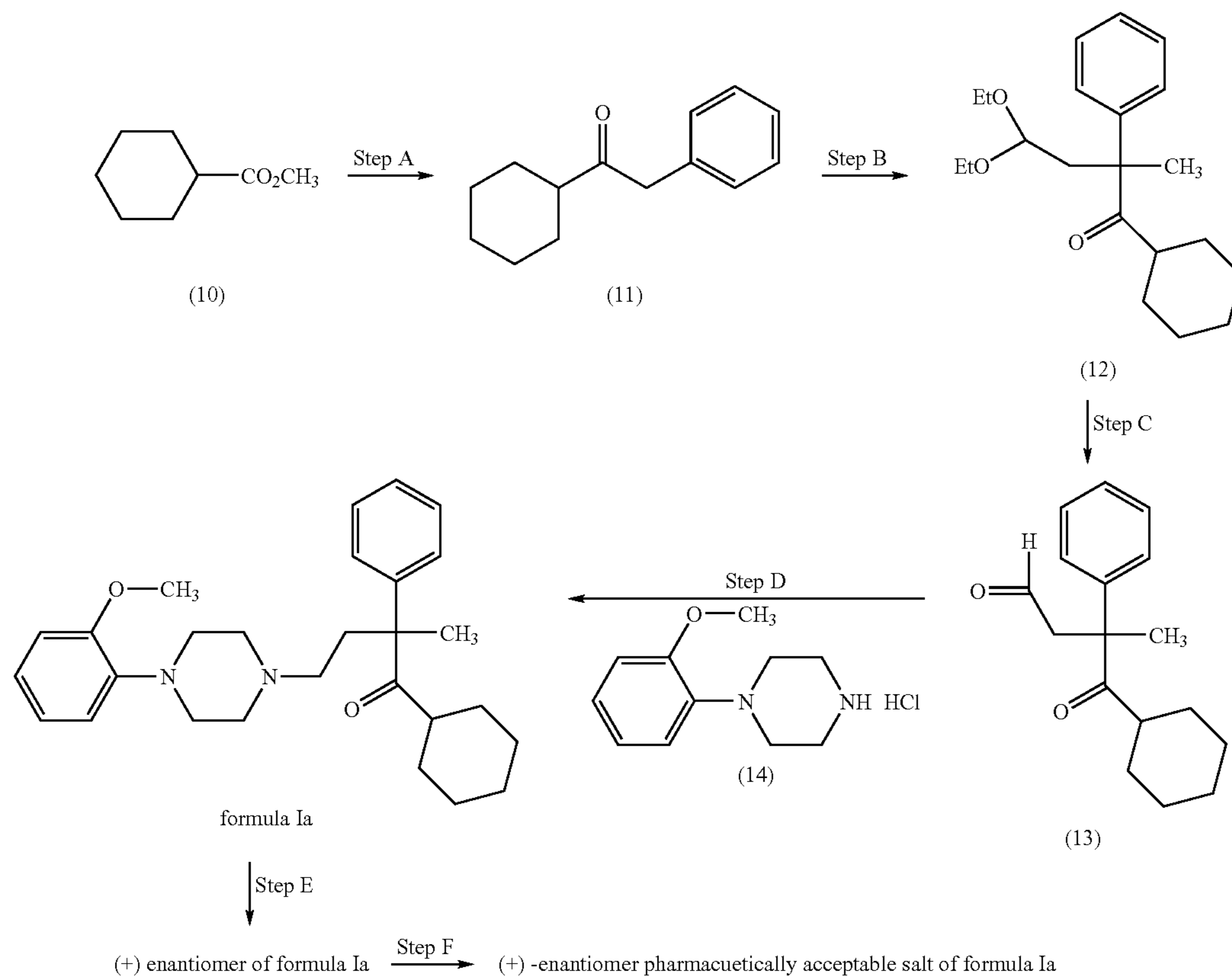
Scheme III
