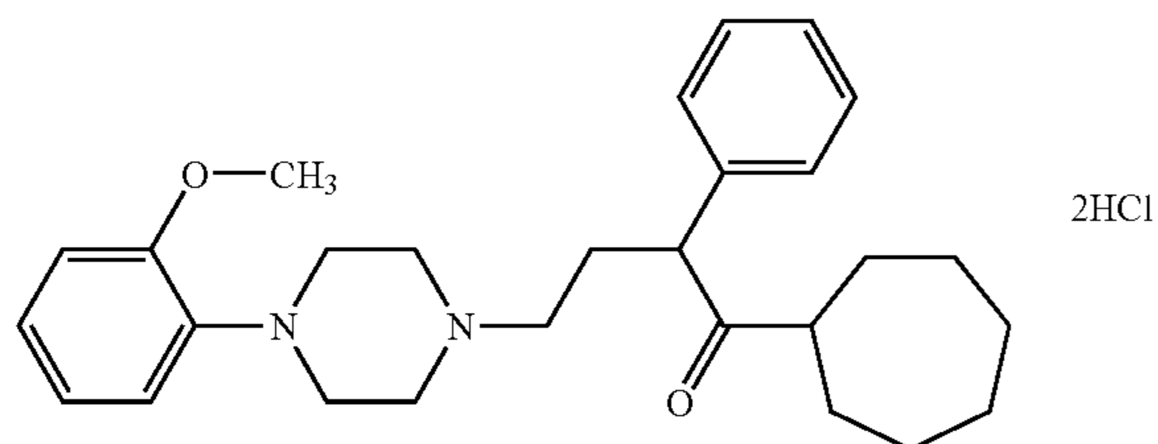
1-(2-methoxyphenyl)-4-[3-(cycloheptanecarbonyl)-3-(phenyl)propyl]piperazine dihydrochloride
