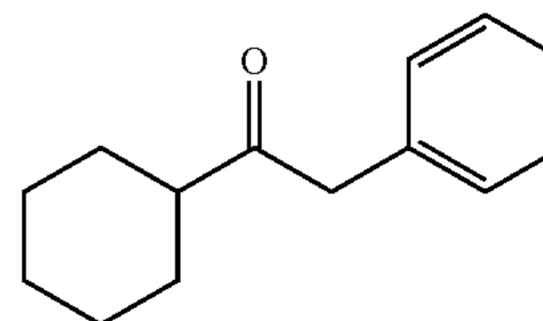
Preparation of 2-phenyl-1-cyclohexane-ethan-1-one
