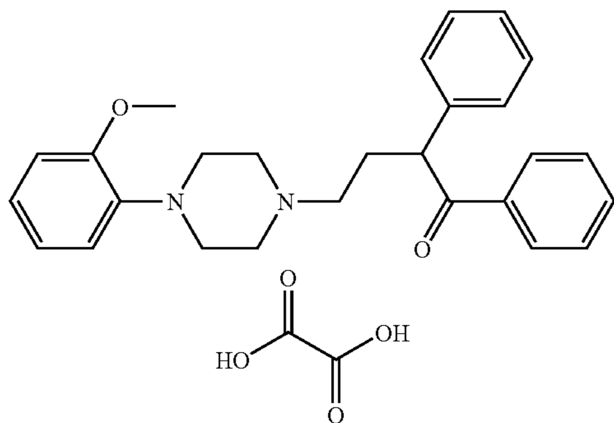
1-(2-methoxyphenyl)-4-[3-(benzoyl)-3-(phenyl)propyl]piperazine Oxalate
