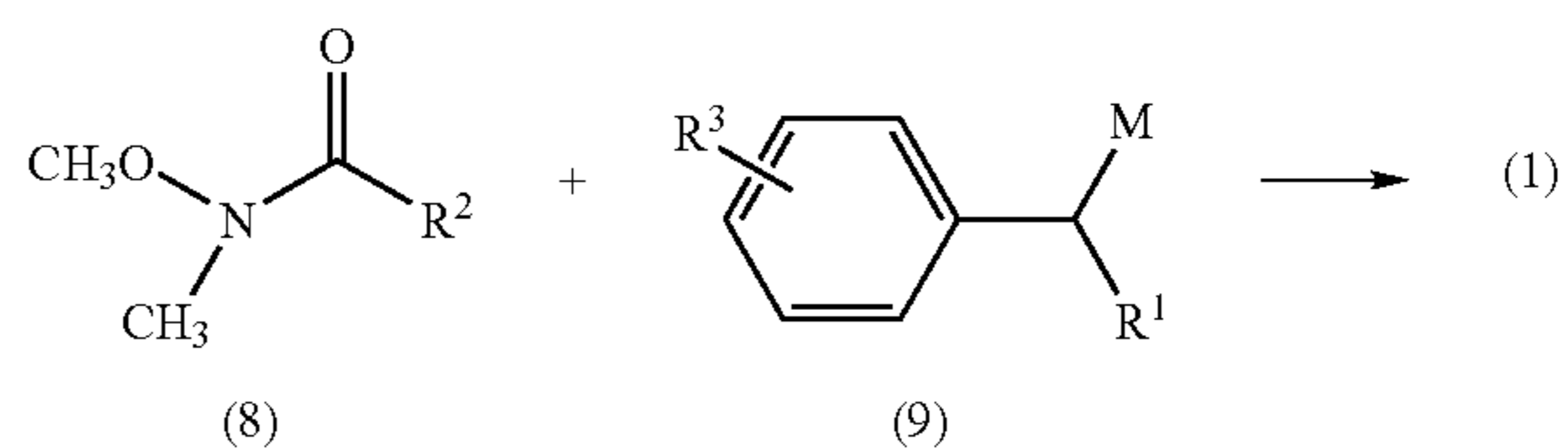
Scheme II
