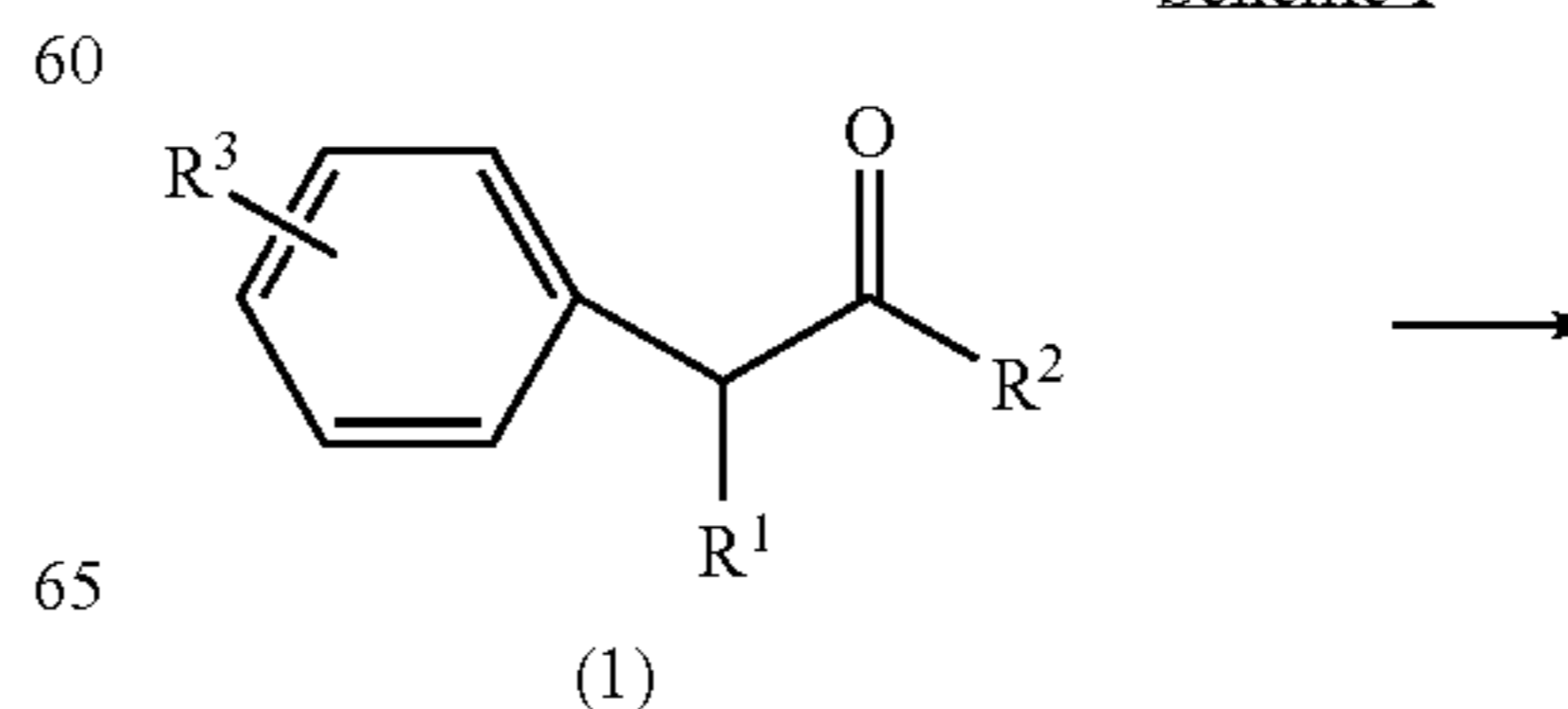
Scheme I
