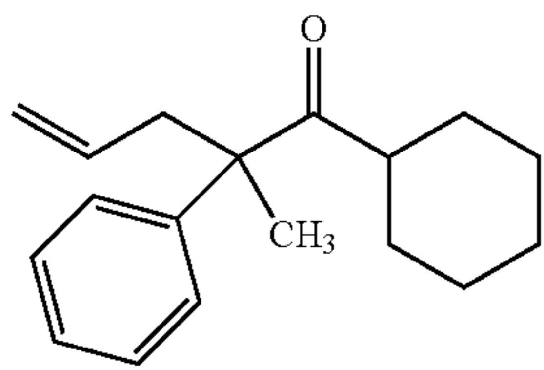
Preparation of 2-phenyl-2-methyl-4-pentenyl cyclohexane
