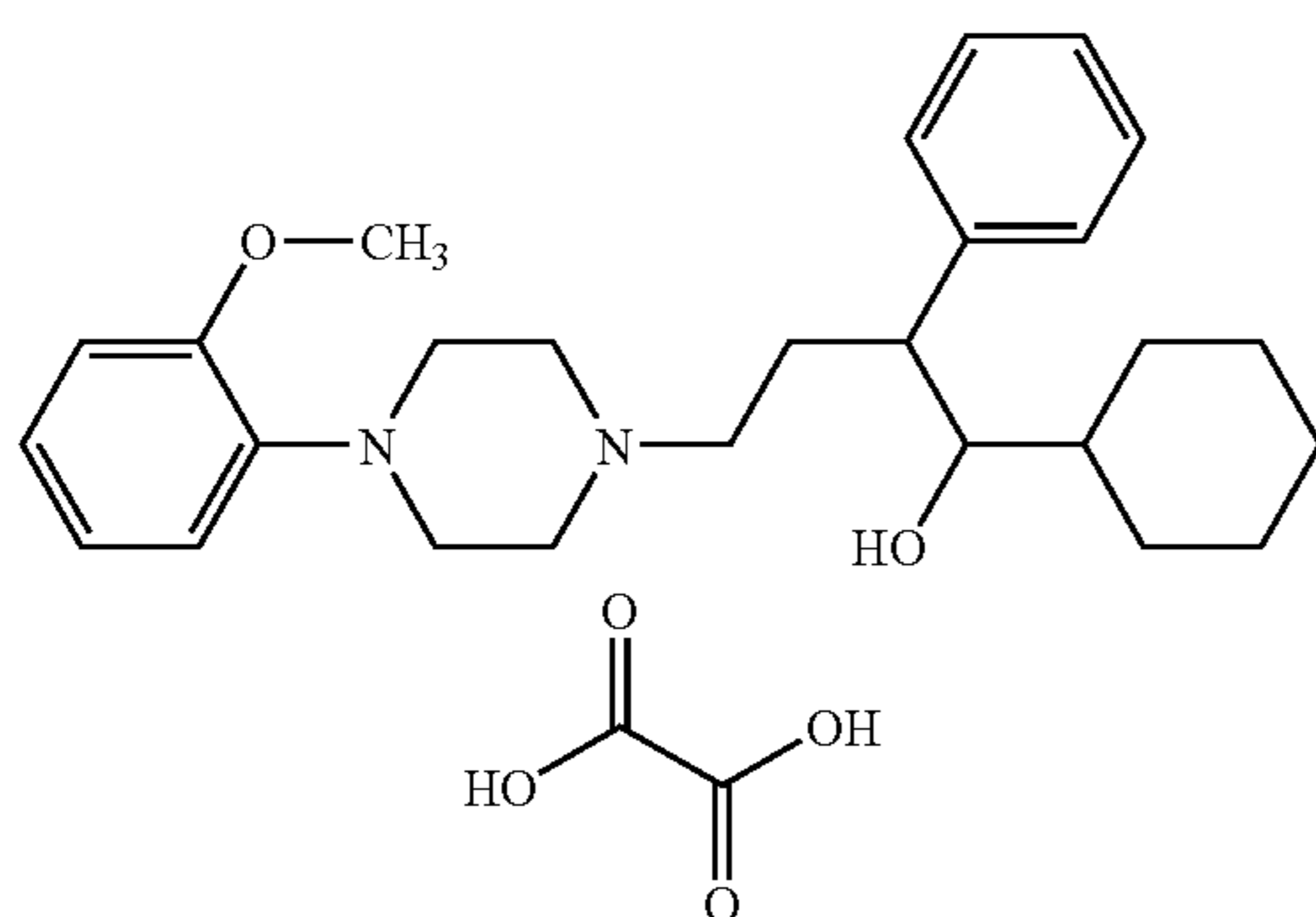
1-(2-methoxyphenyl)-4-[4-(cyclohexyl)-4-(hydroxy)-3-(phenyl)butyl]piperazine oxalate
