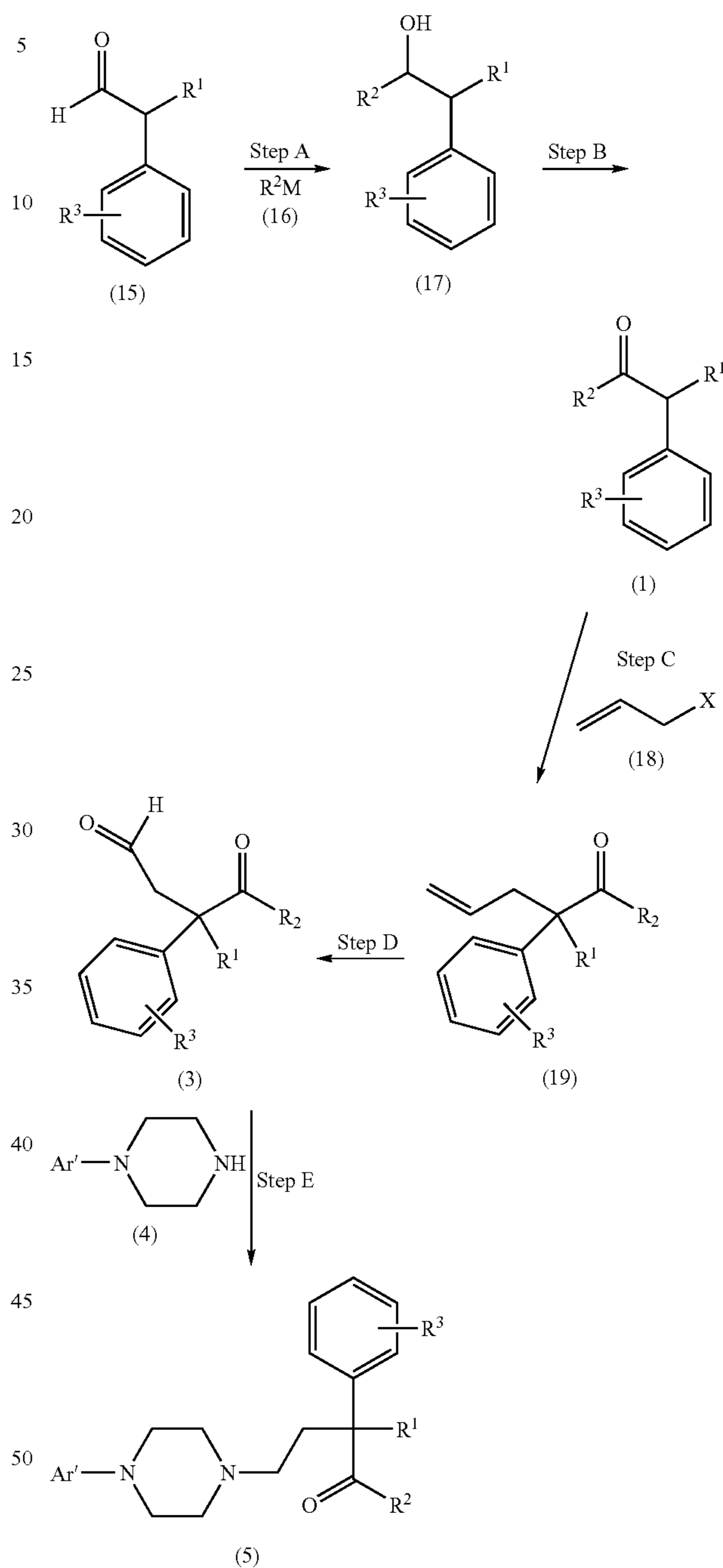
Scheme IV
