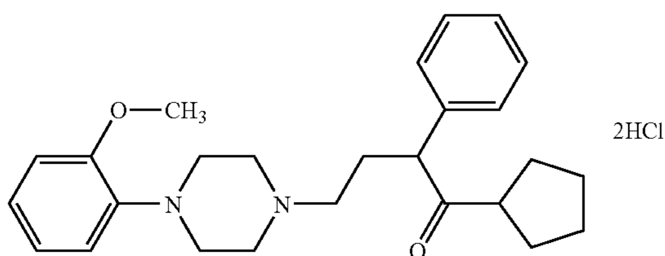
1-(2-methoxyphenyl)-4-[3-(cyclopentanecarbonyl)-3-(phenyl)propyl]piperazine dihydrochloride
