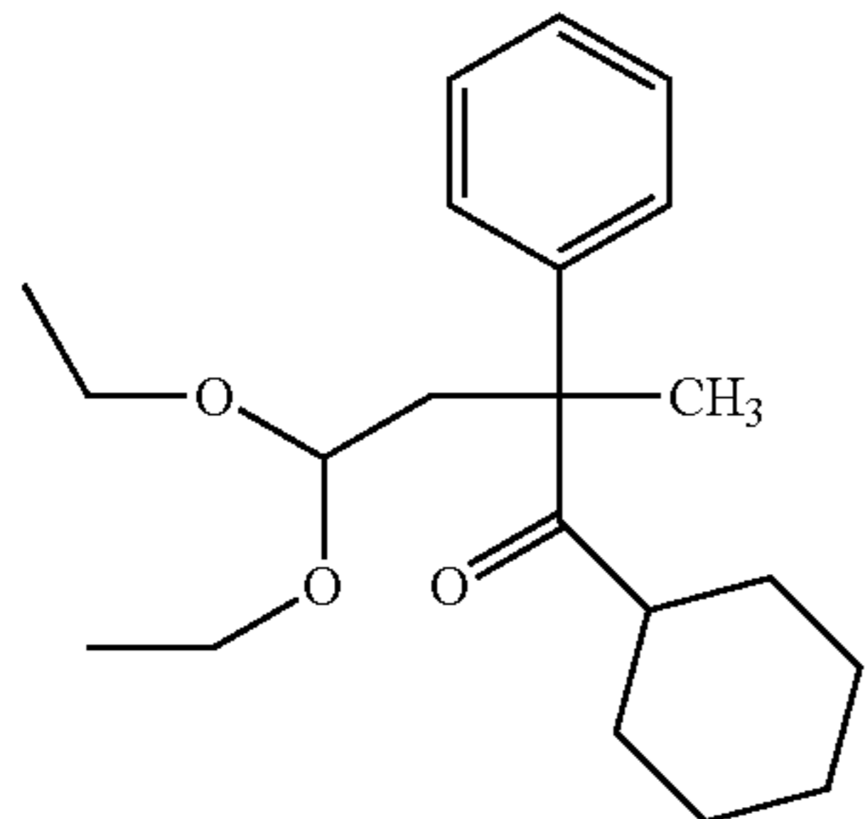
Preparation of 1,1-diethoxy-3-phenyl-3-cyclohexanecarbonyl-butane
