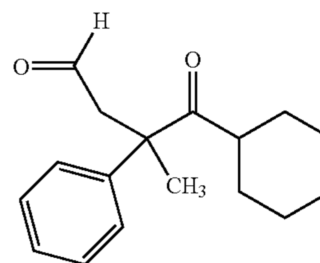
Preparation of 4-Cyclohexyl-3-methyl-4-oxo-3-phenylbutyraldehyde
