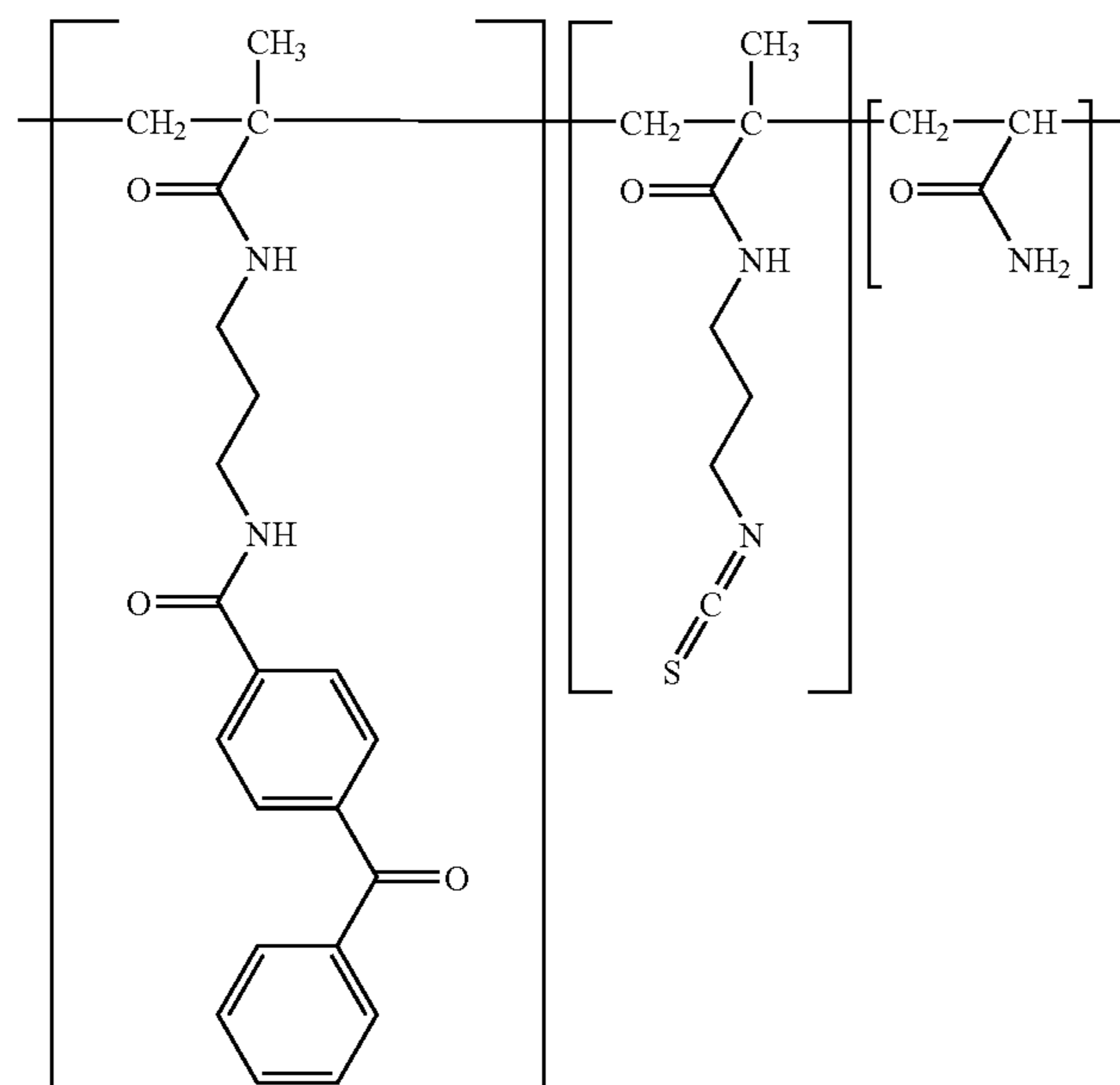
Comparative Compound VIII
