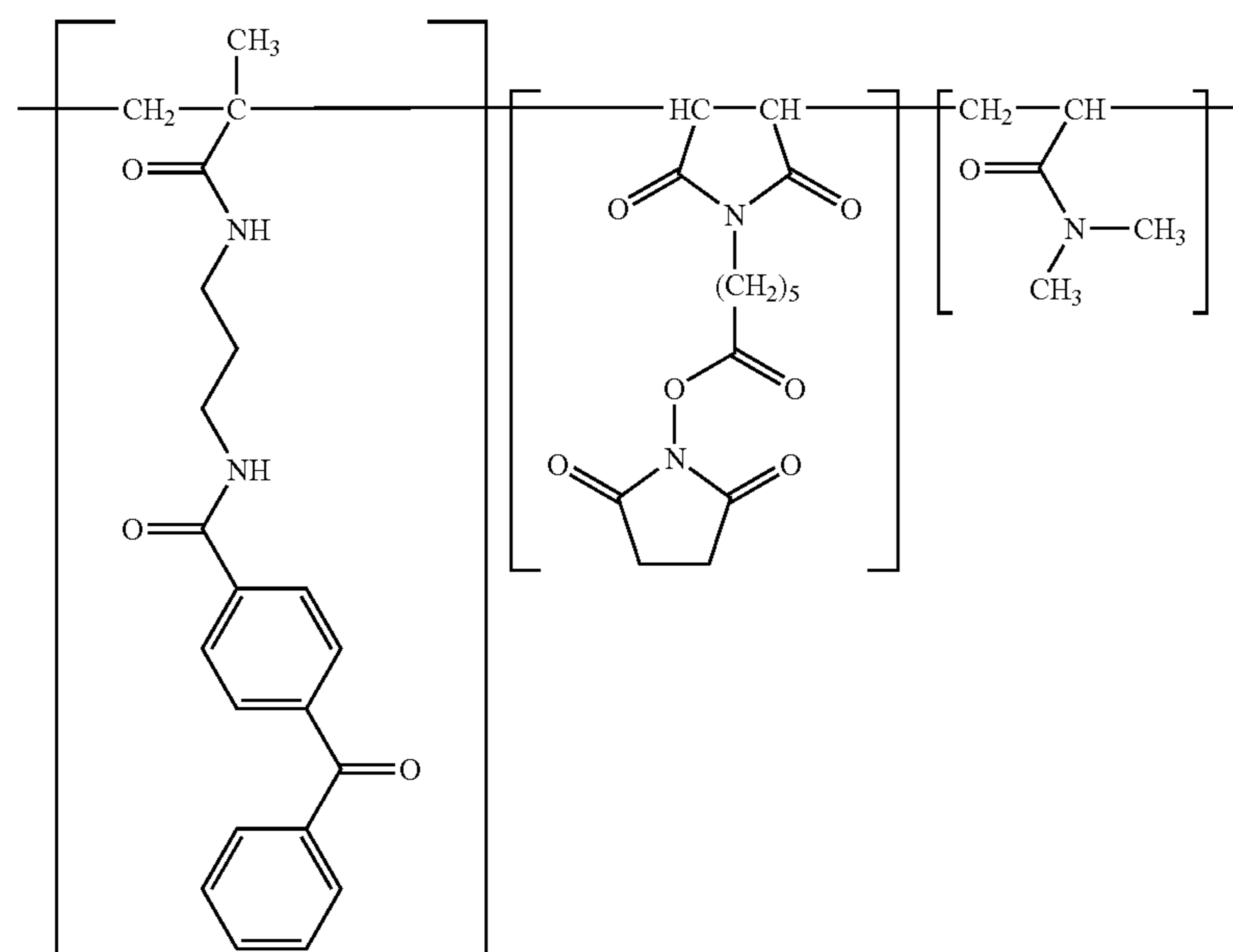
Compound V (Photo-DMA-NOS)
