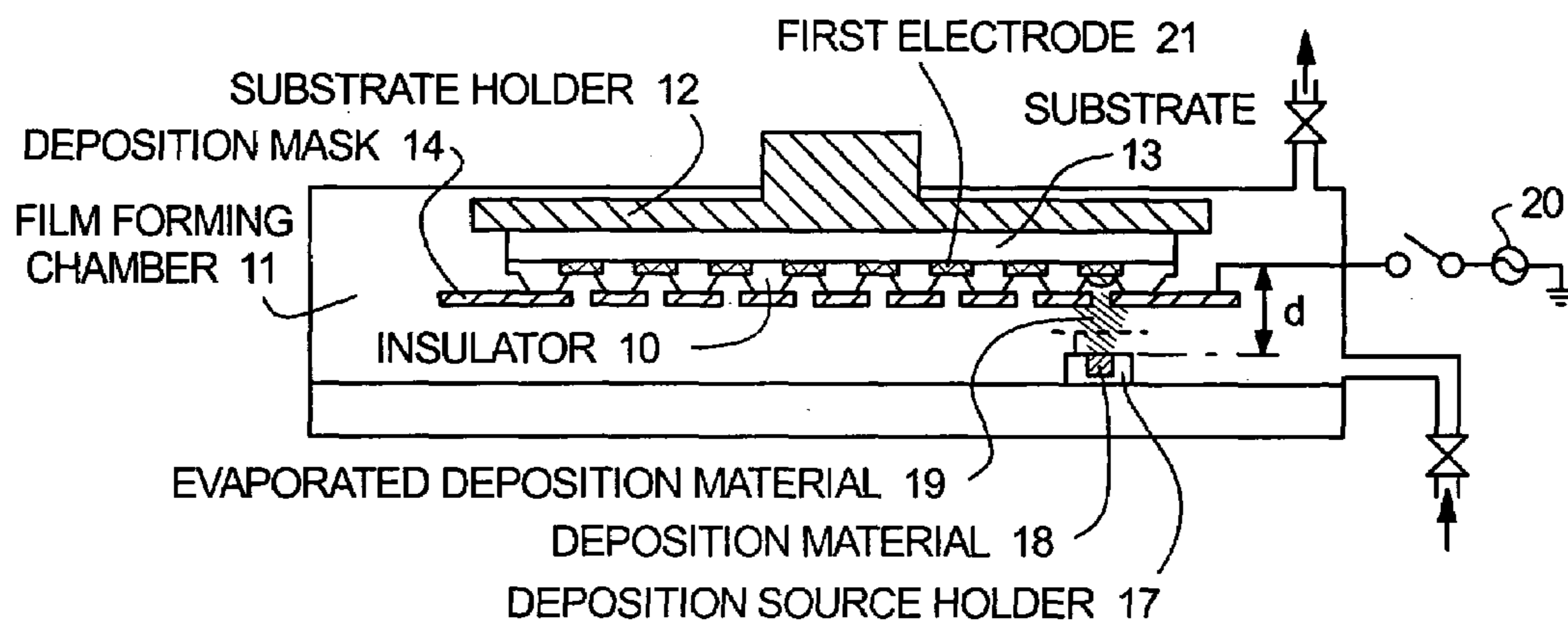
FIG. 1A SECTIONAL VIEW IN X DIRECTION
