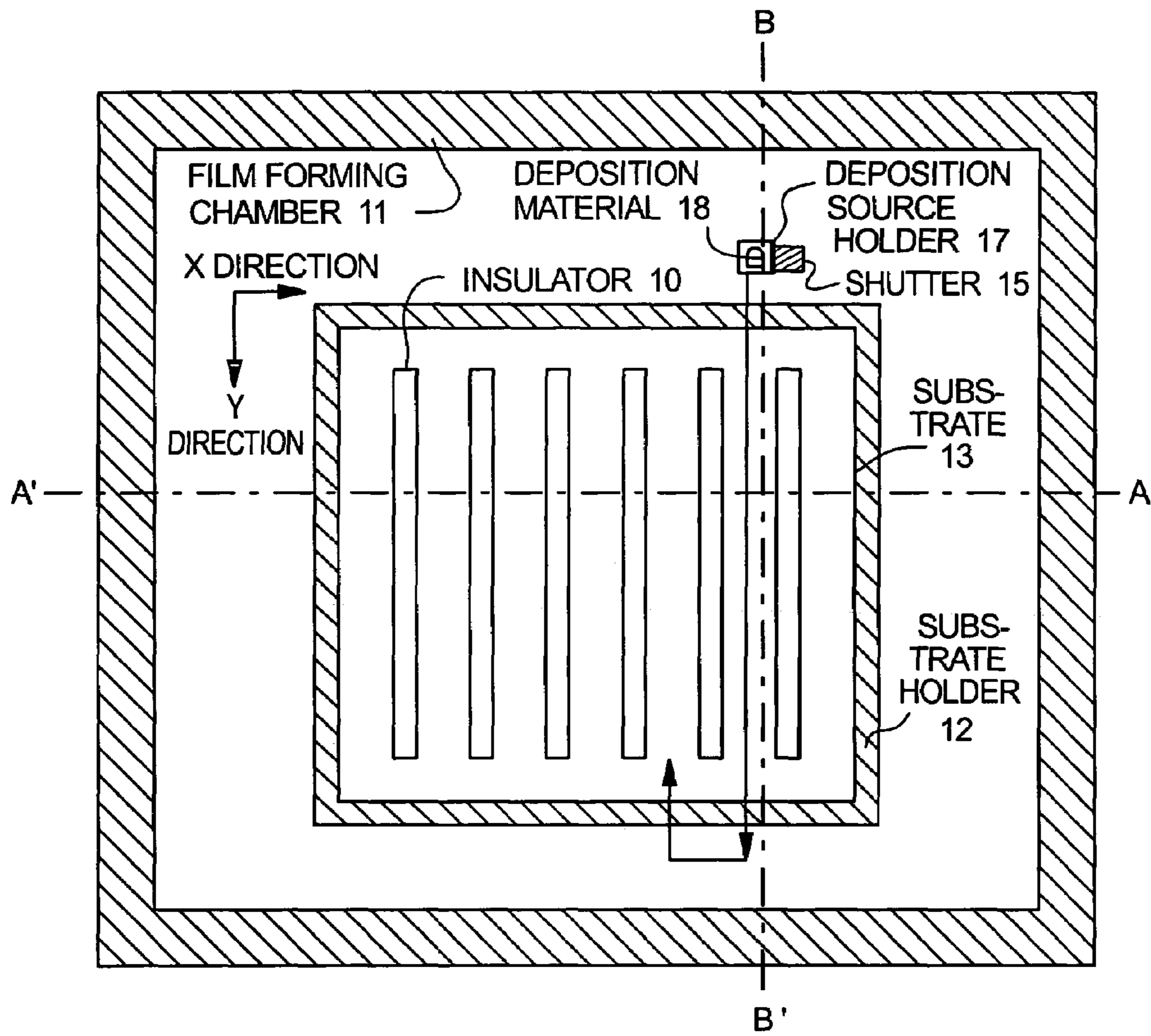
FIG. 1C PLAN VIEW
