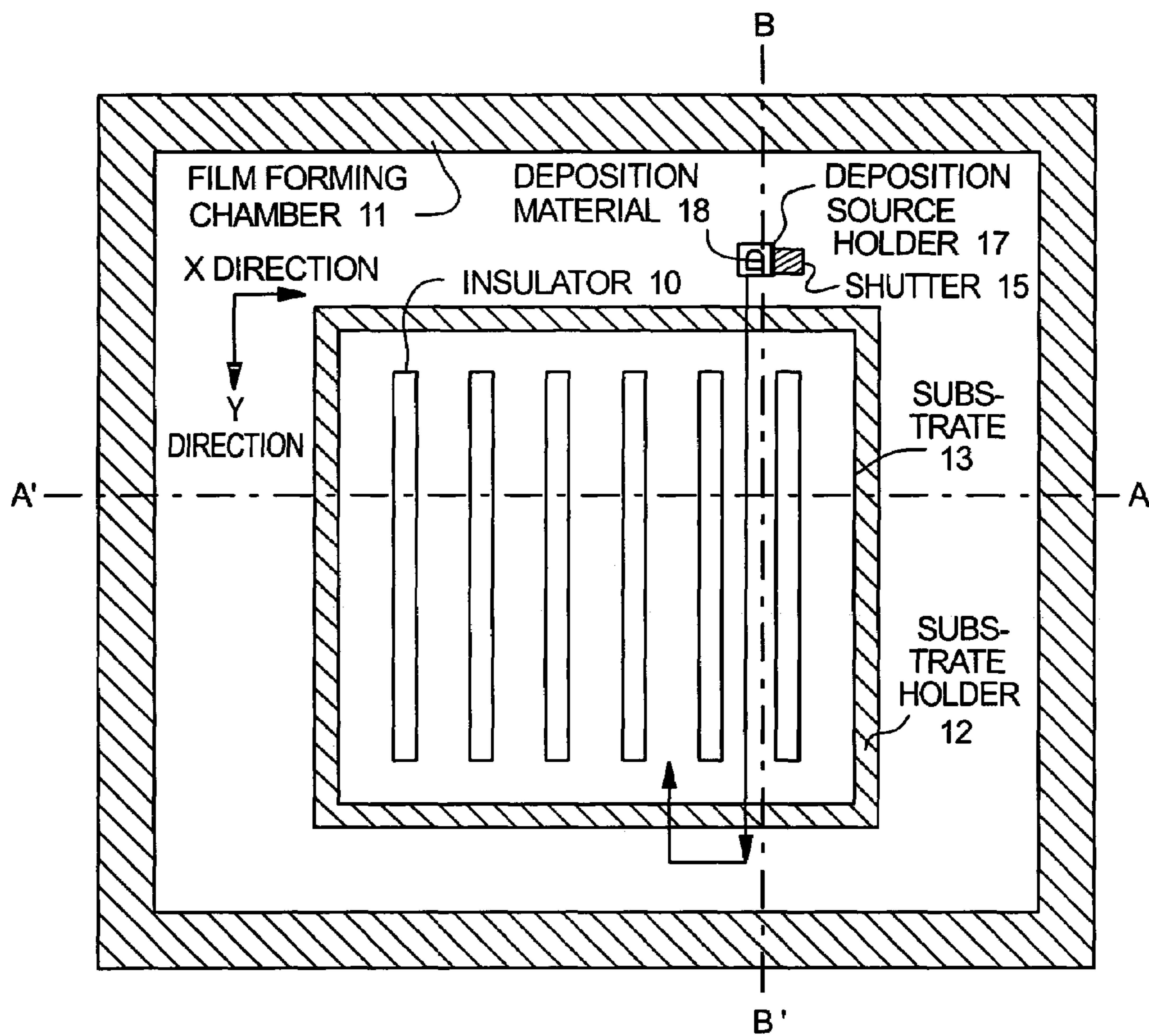
FIG. 1C PLAN VIEW
