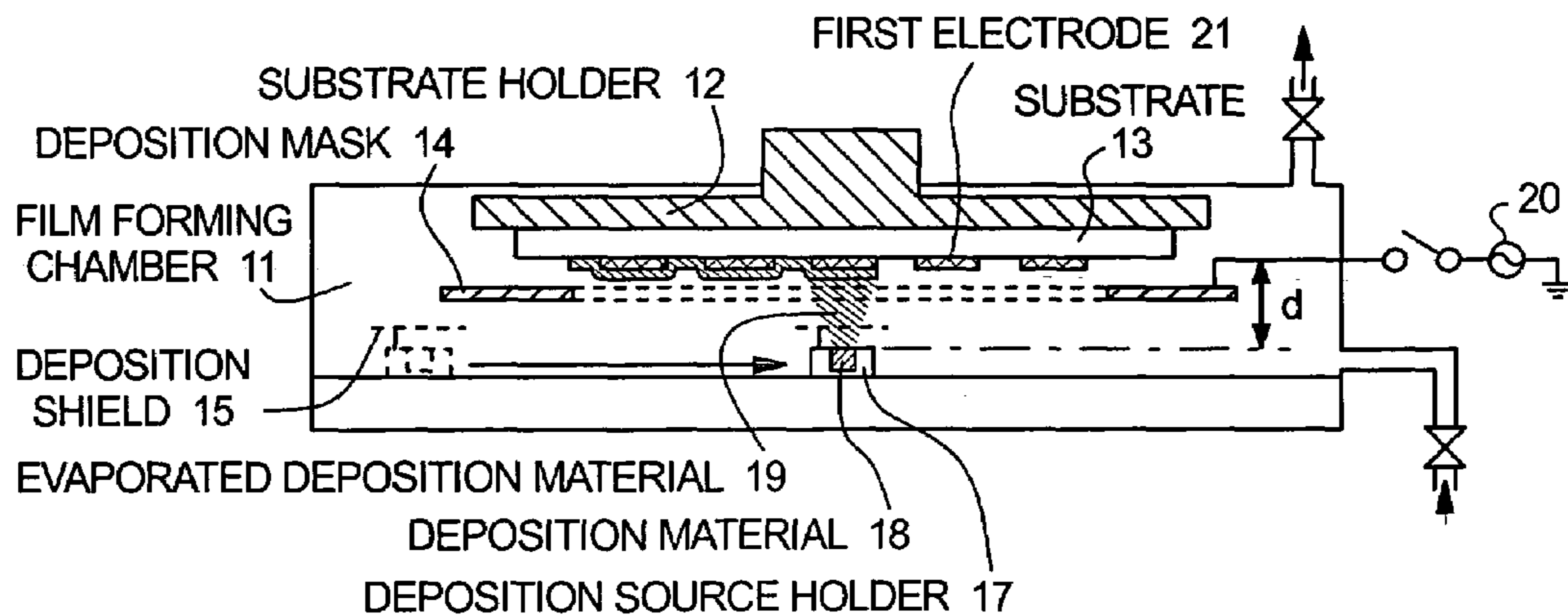
FIG. 1B SECTIONAL VIEW IN Y DIRECTION (IN THE MIDDLE OF FILM FORMATION)
