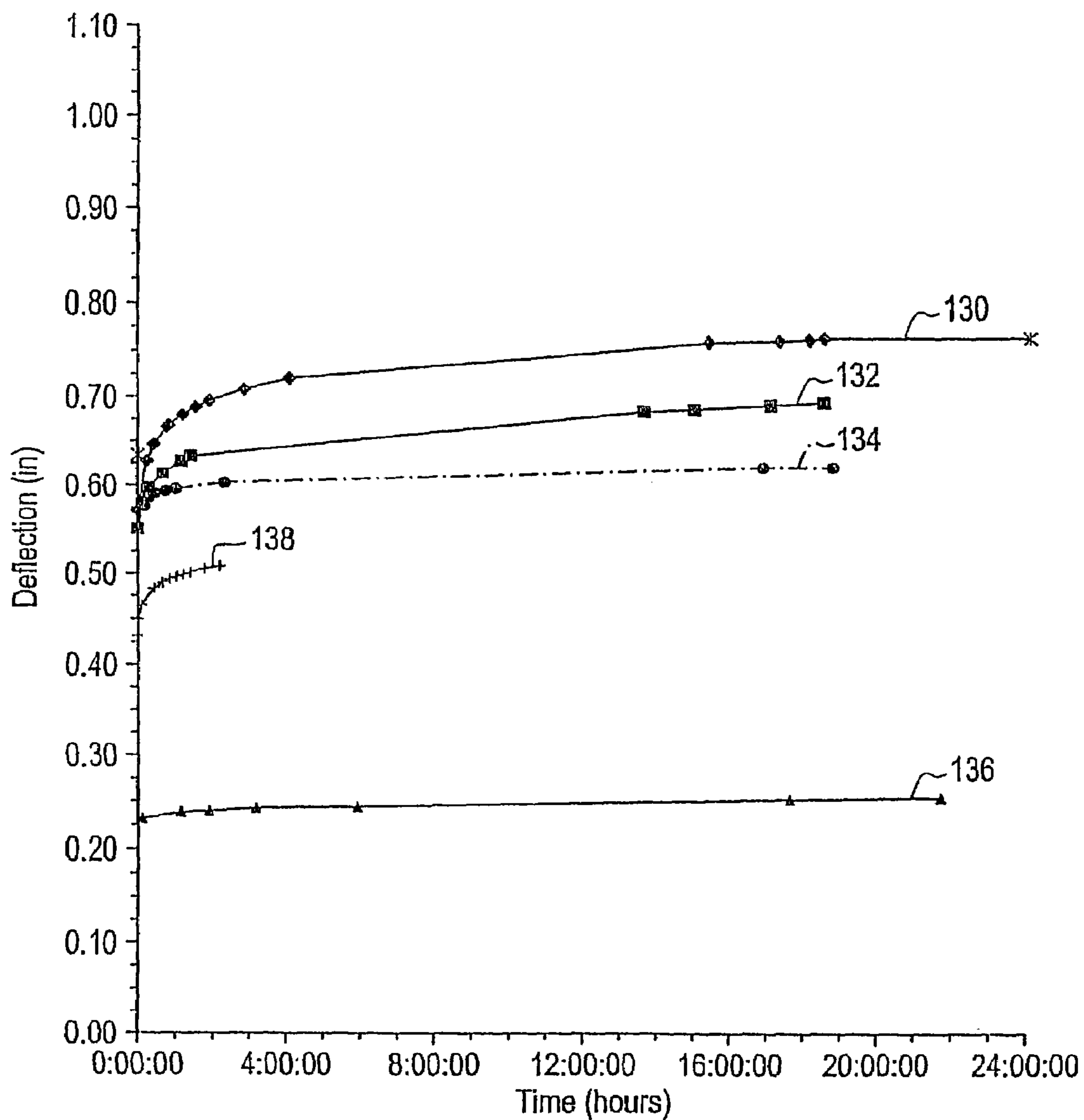
FIG. 27 Virginia Tech Load Test Summary
