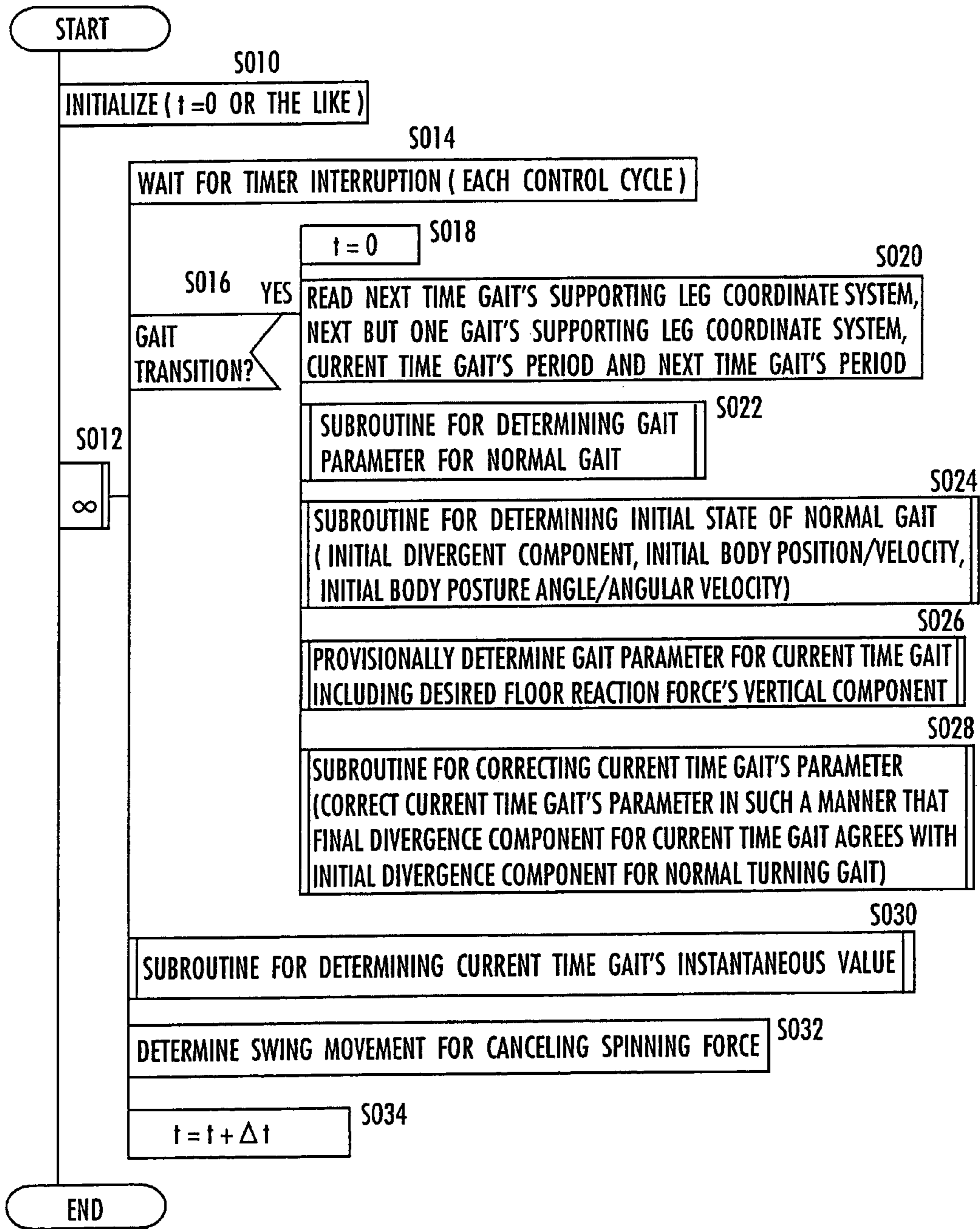
FIG.12 (FLOWCHART OF GAIT GENERATION PROCESS)
