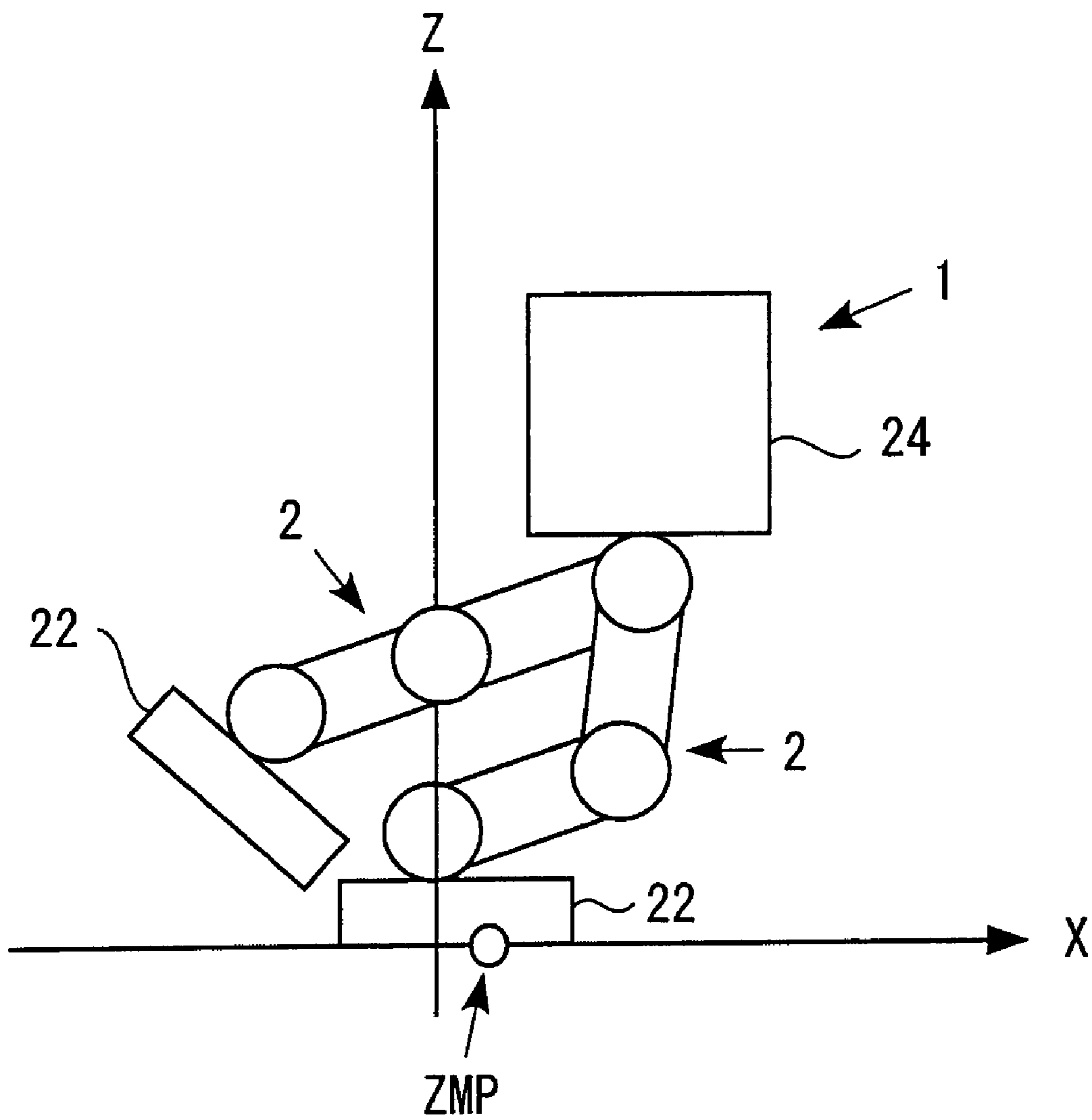
FIG.13 ( DIVERGENCE STATE OF BODY POSITION )
