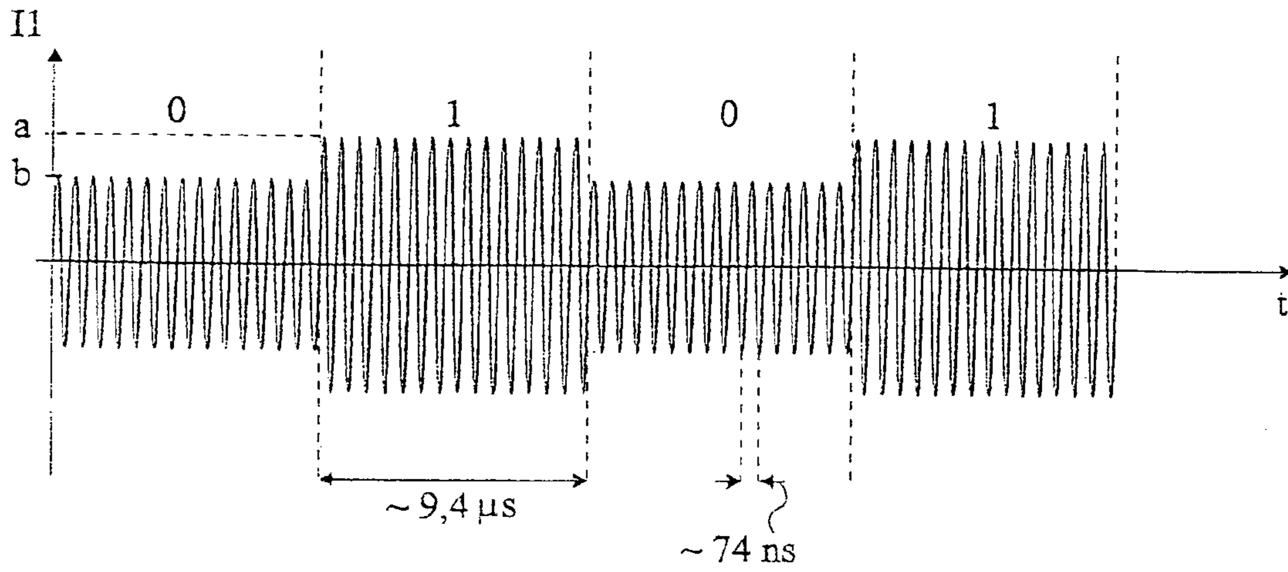
Fig 2 (PRIOR ART)
