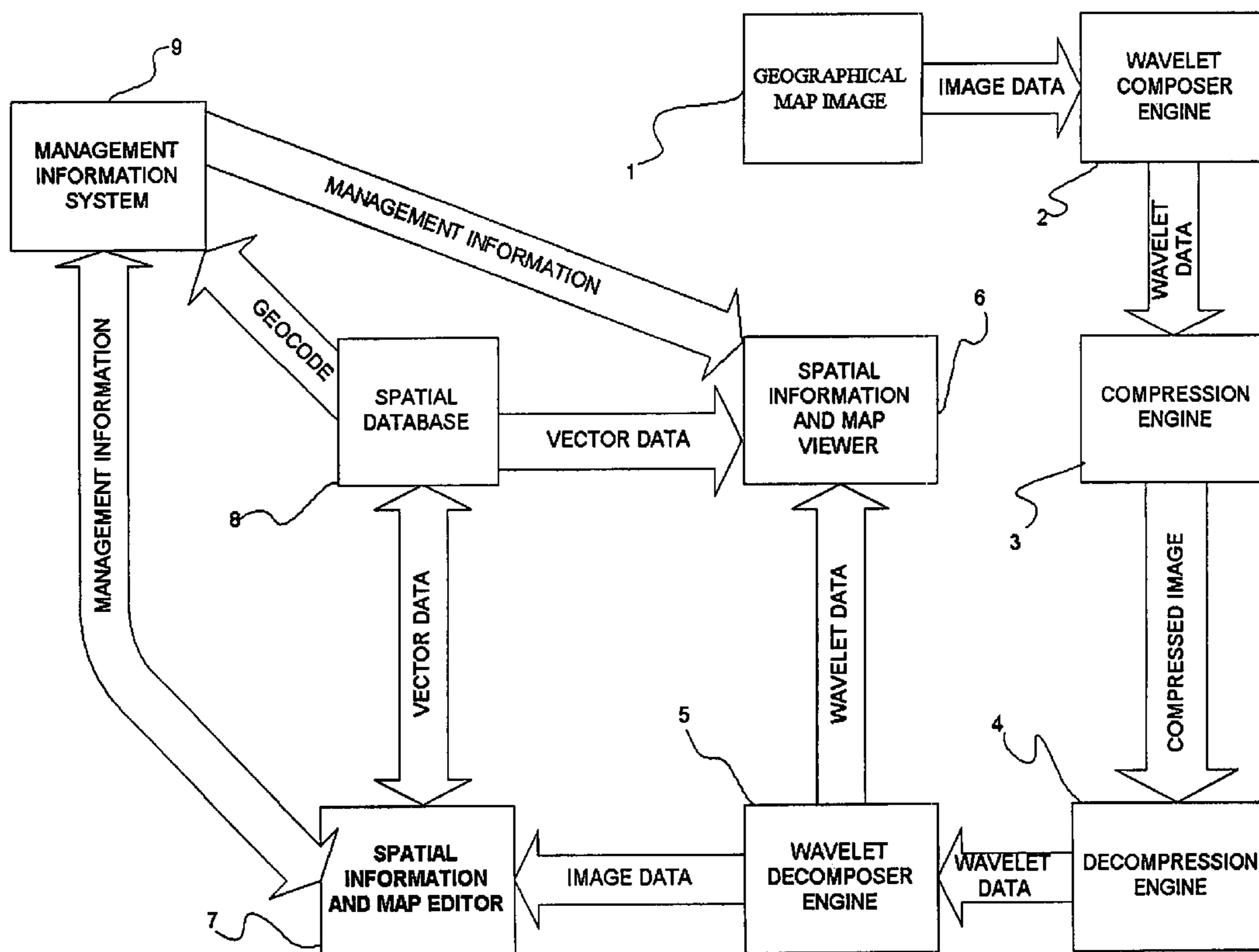
A PROCESS OF GIS VIEWER FLOW ON WORLD WIDE WEB DIAGRAM
