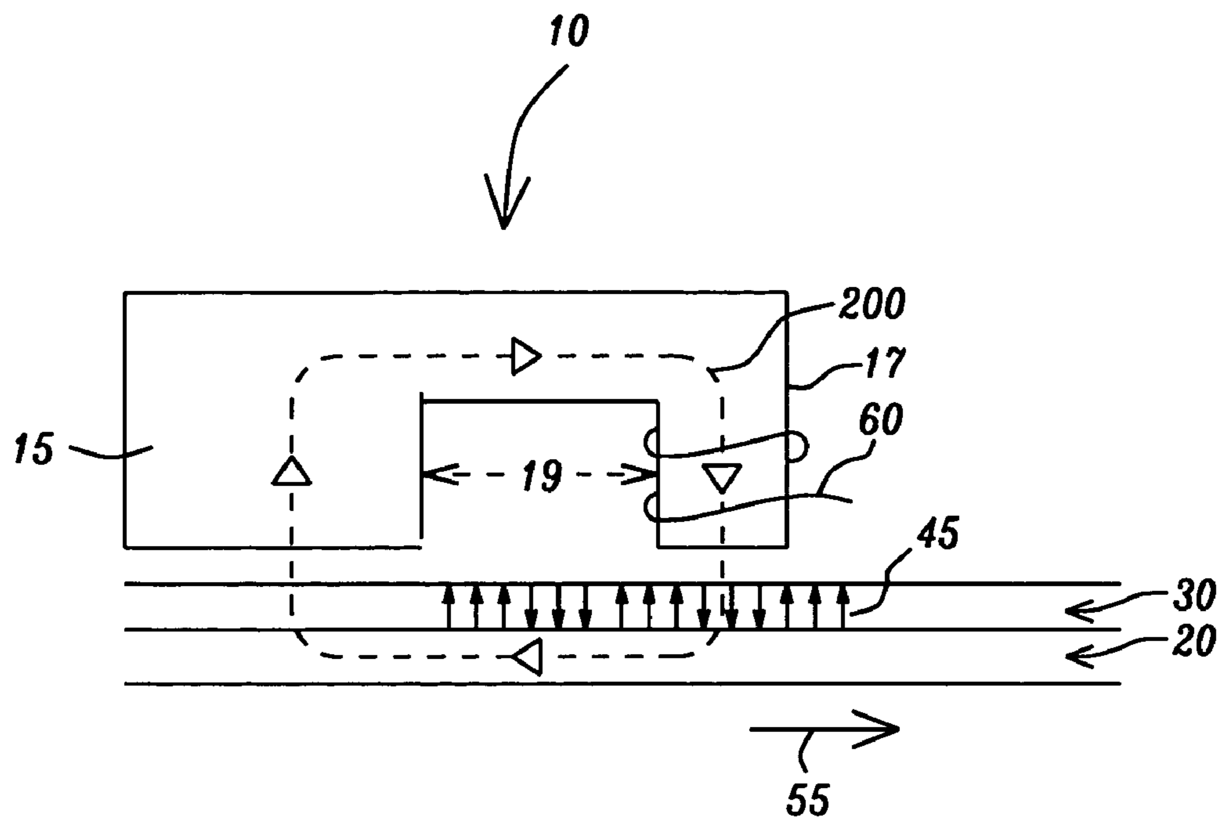
FIG. 1 - Prior Art
