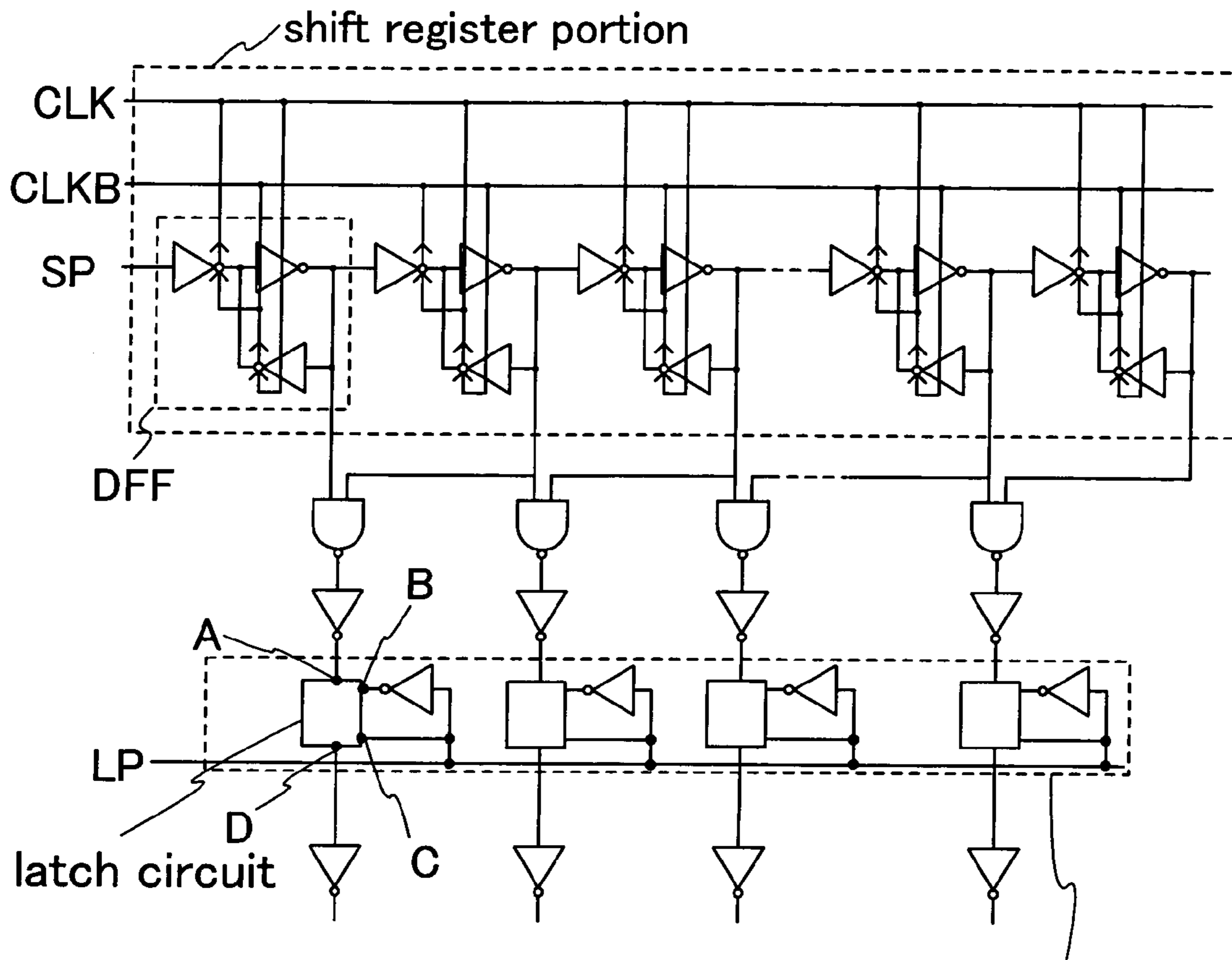
latch circuit array
