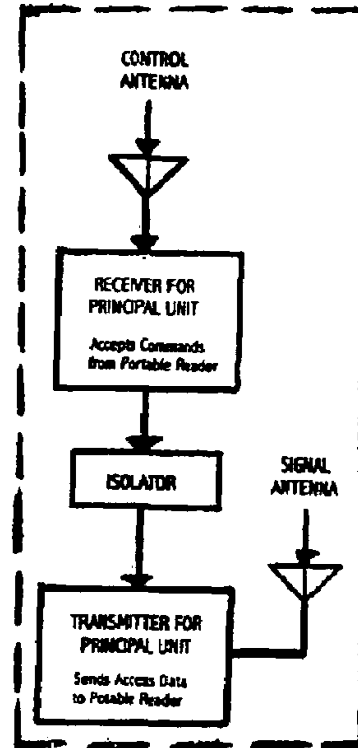
BLK. DIAG. - WIRELESS CNTRLER. OF PRINCIPAL UNIT
