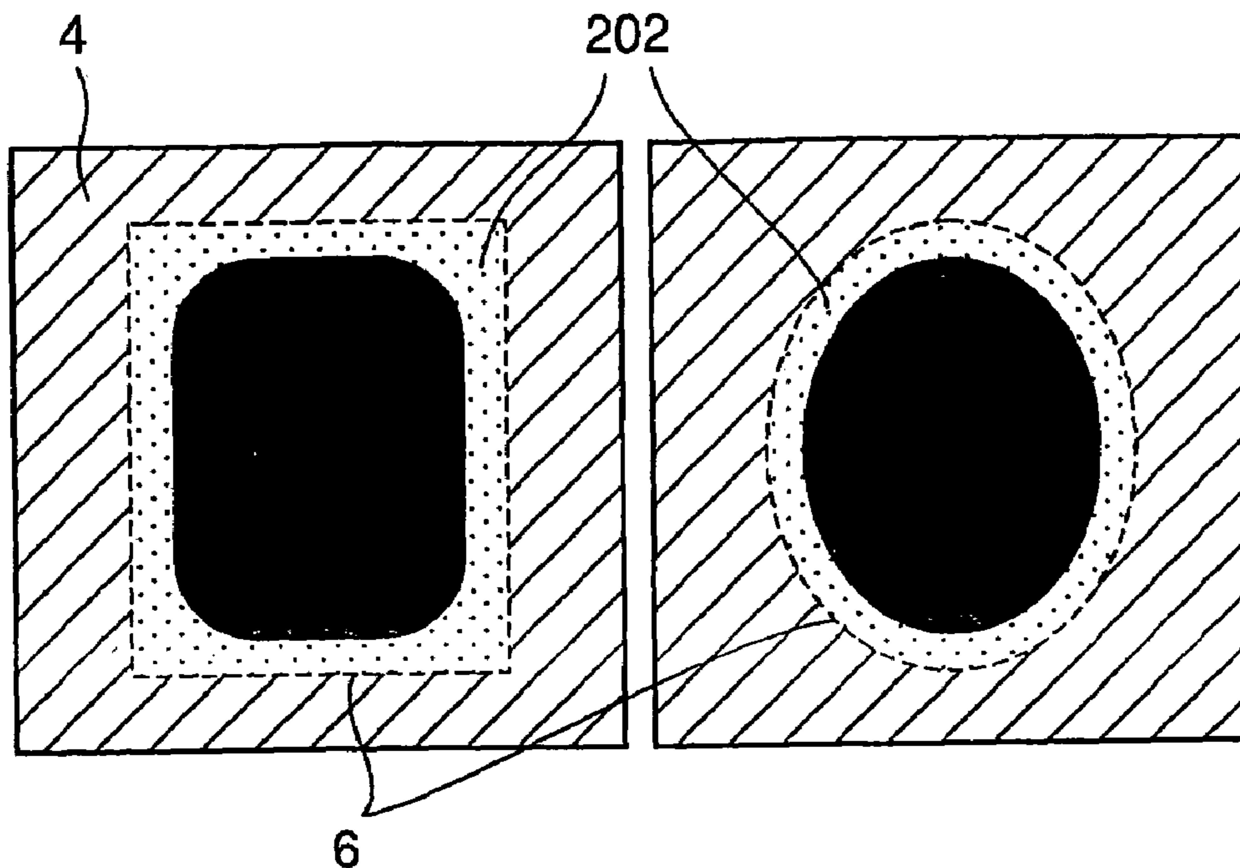
FIG. 9 - PRIOR ART
