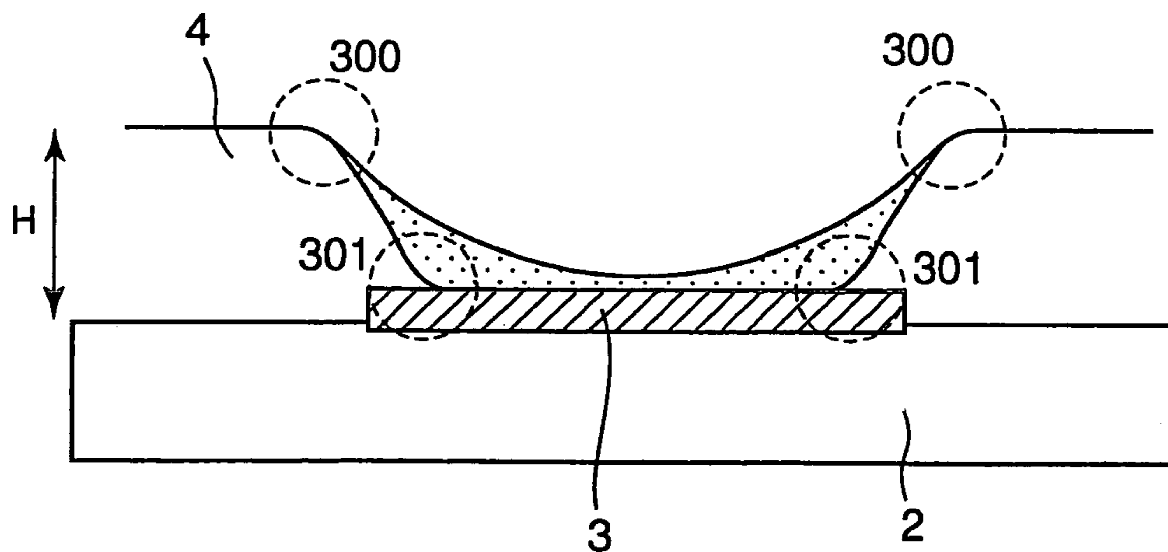
FIG. 12 - PRIOR ART
