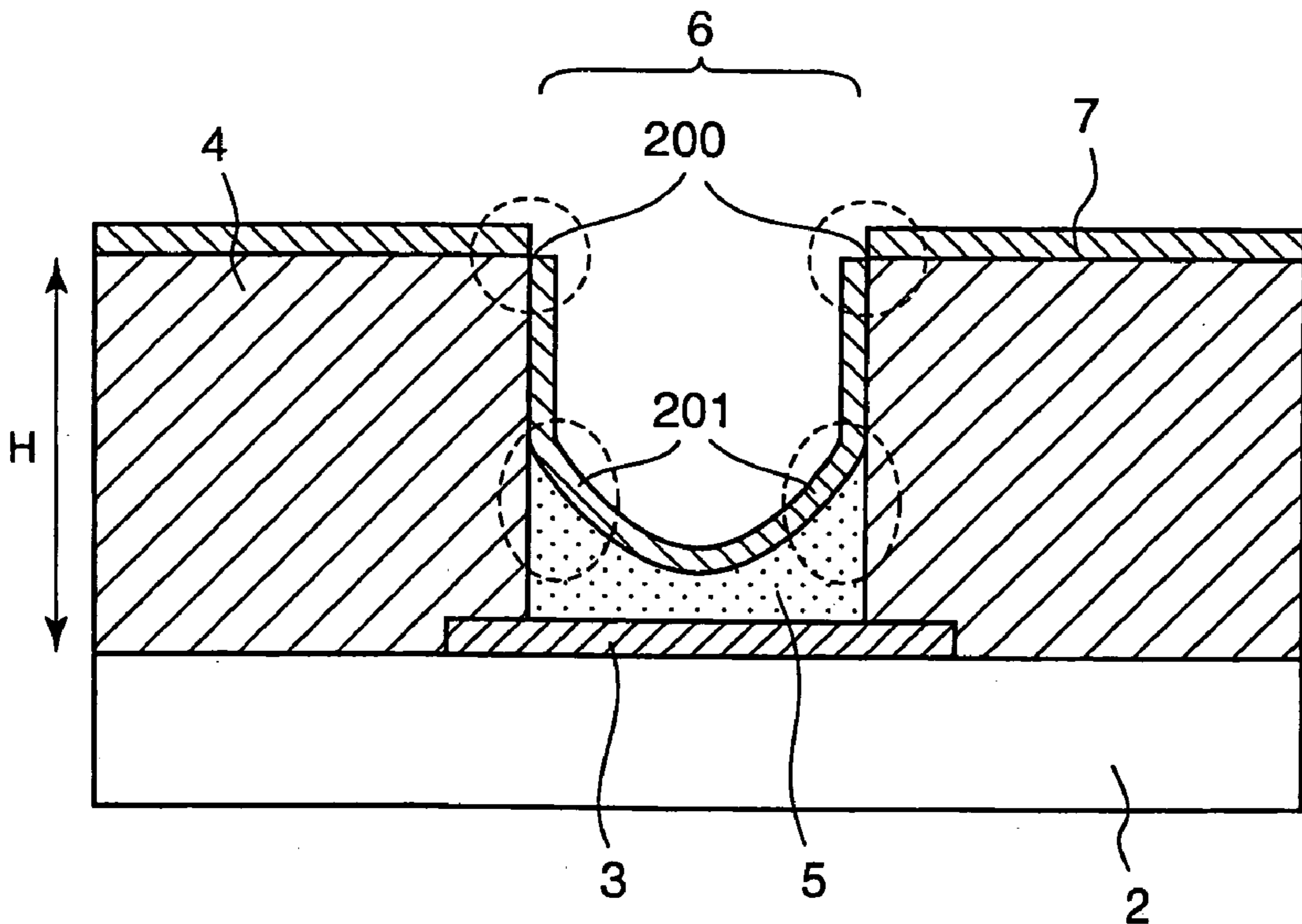
FIG. 6 - PRIOR ART
