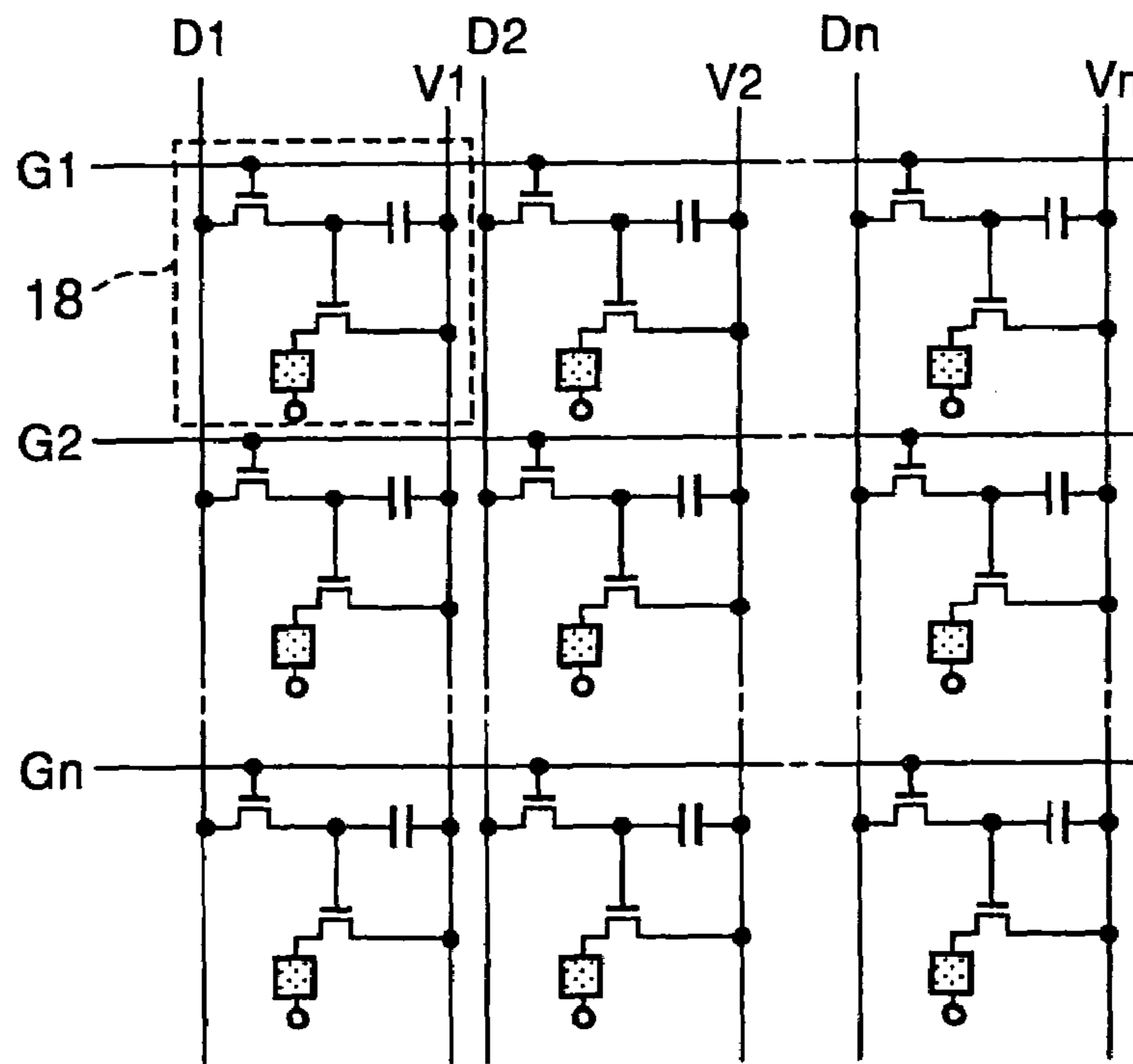
FIG. 16 - PRIOR ART
