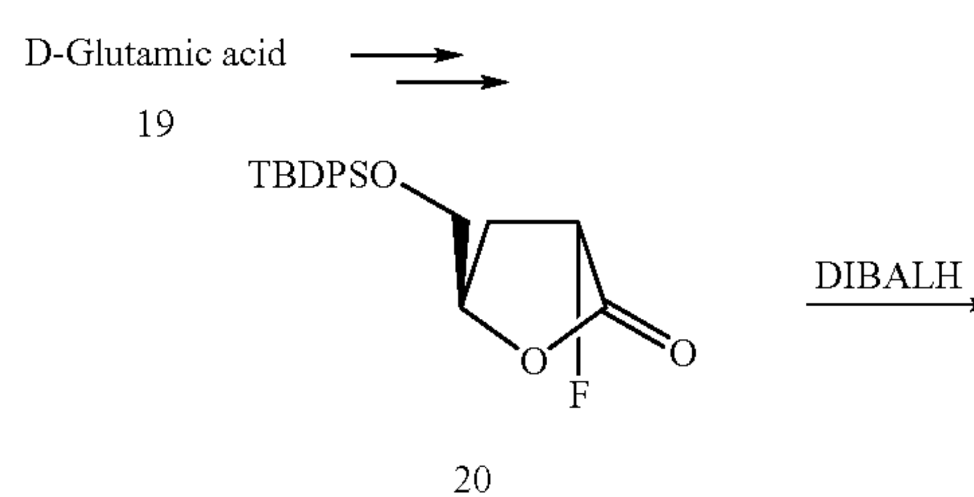
Scheme 3
