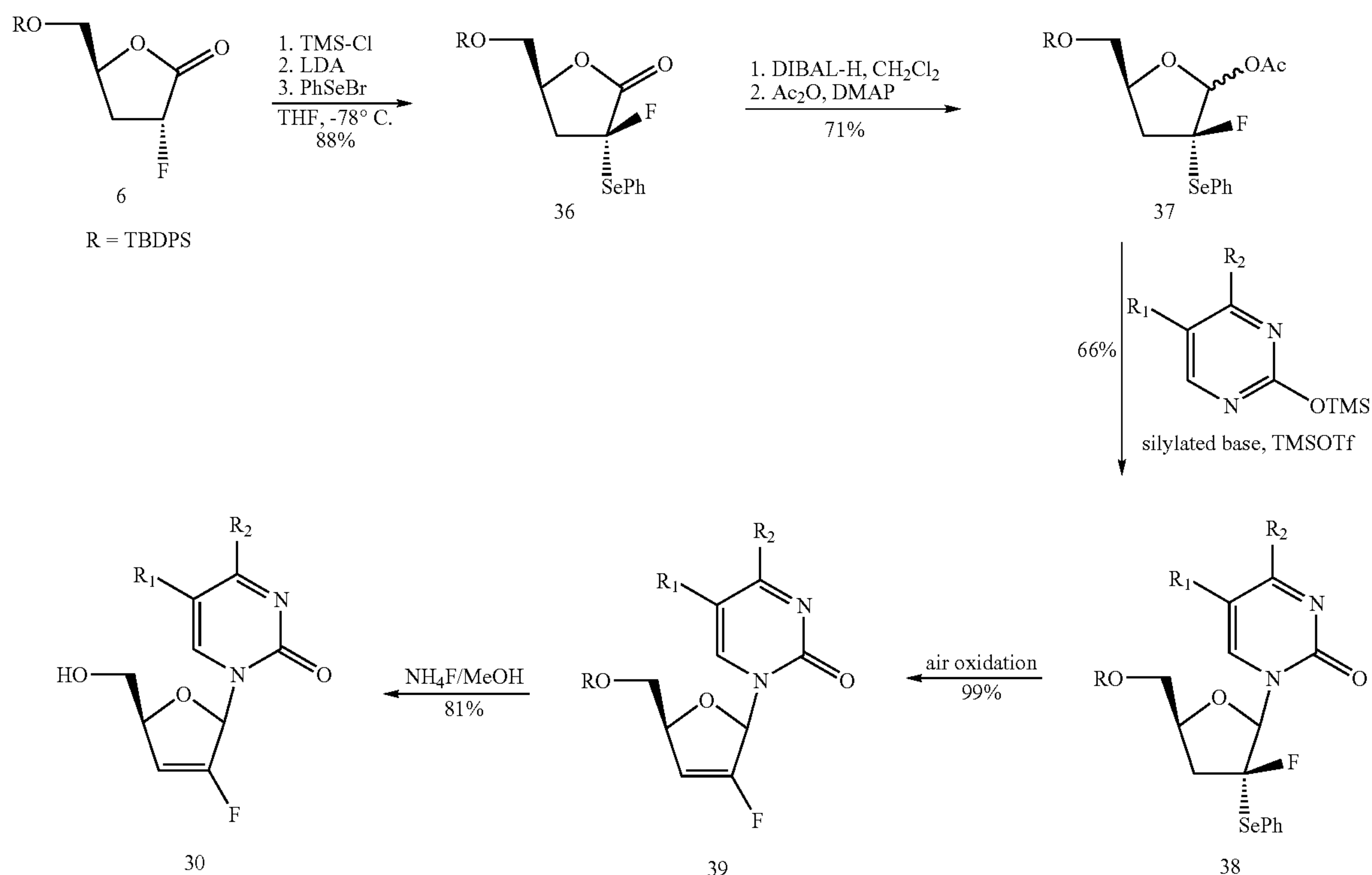
Scheme 7
