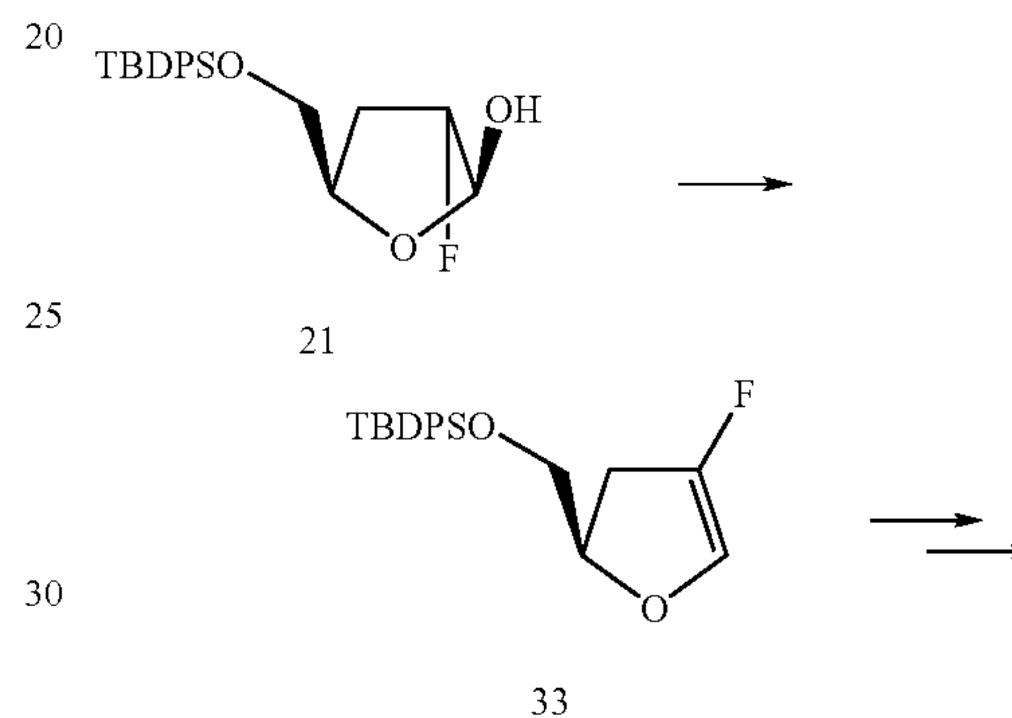
Scheme 8
