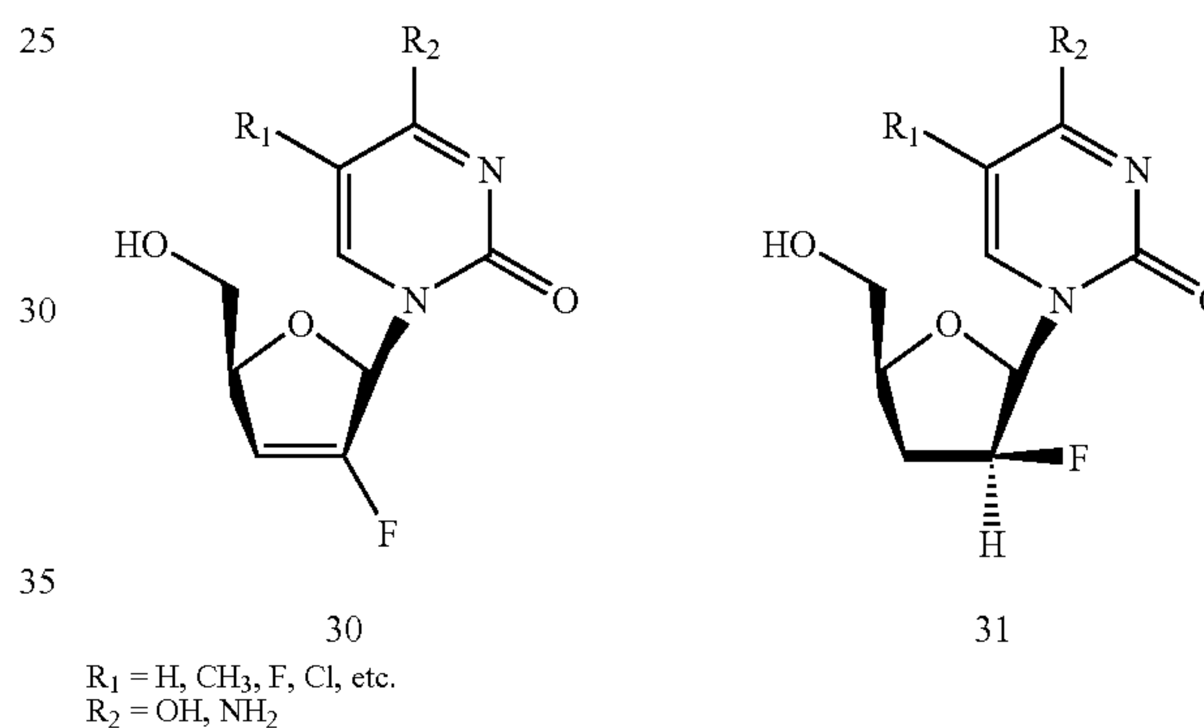
Scheme 5
