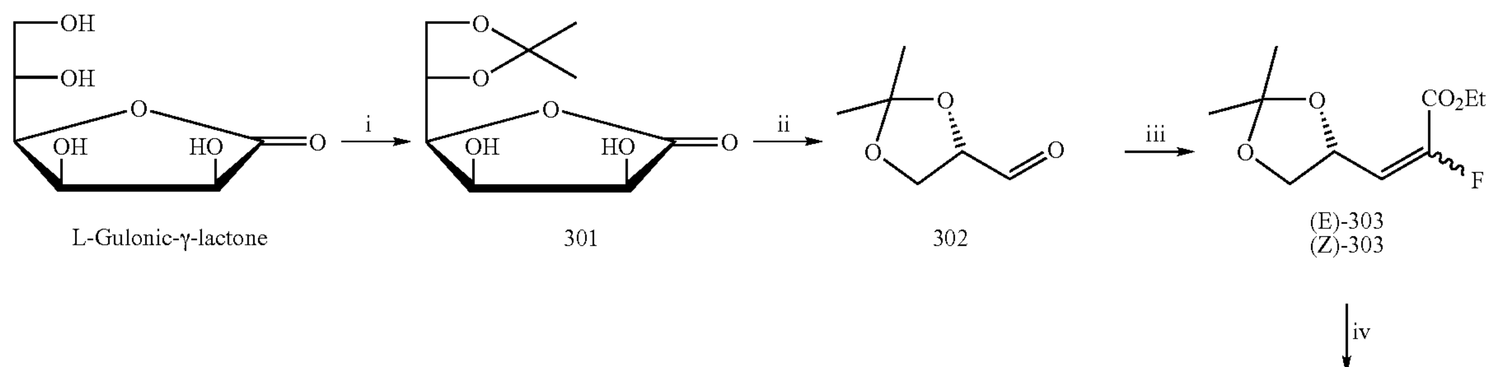
Scheme 9
