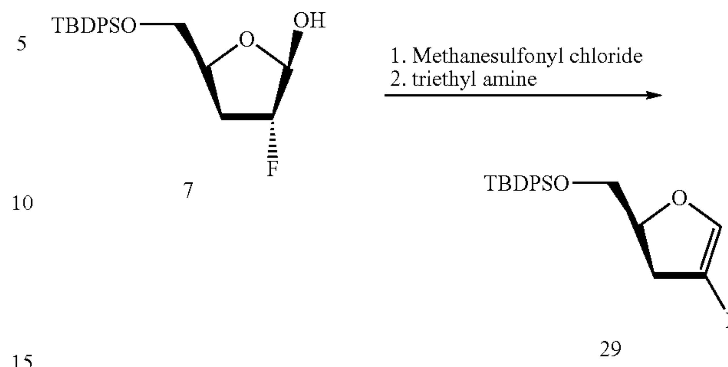
Scheme 4
