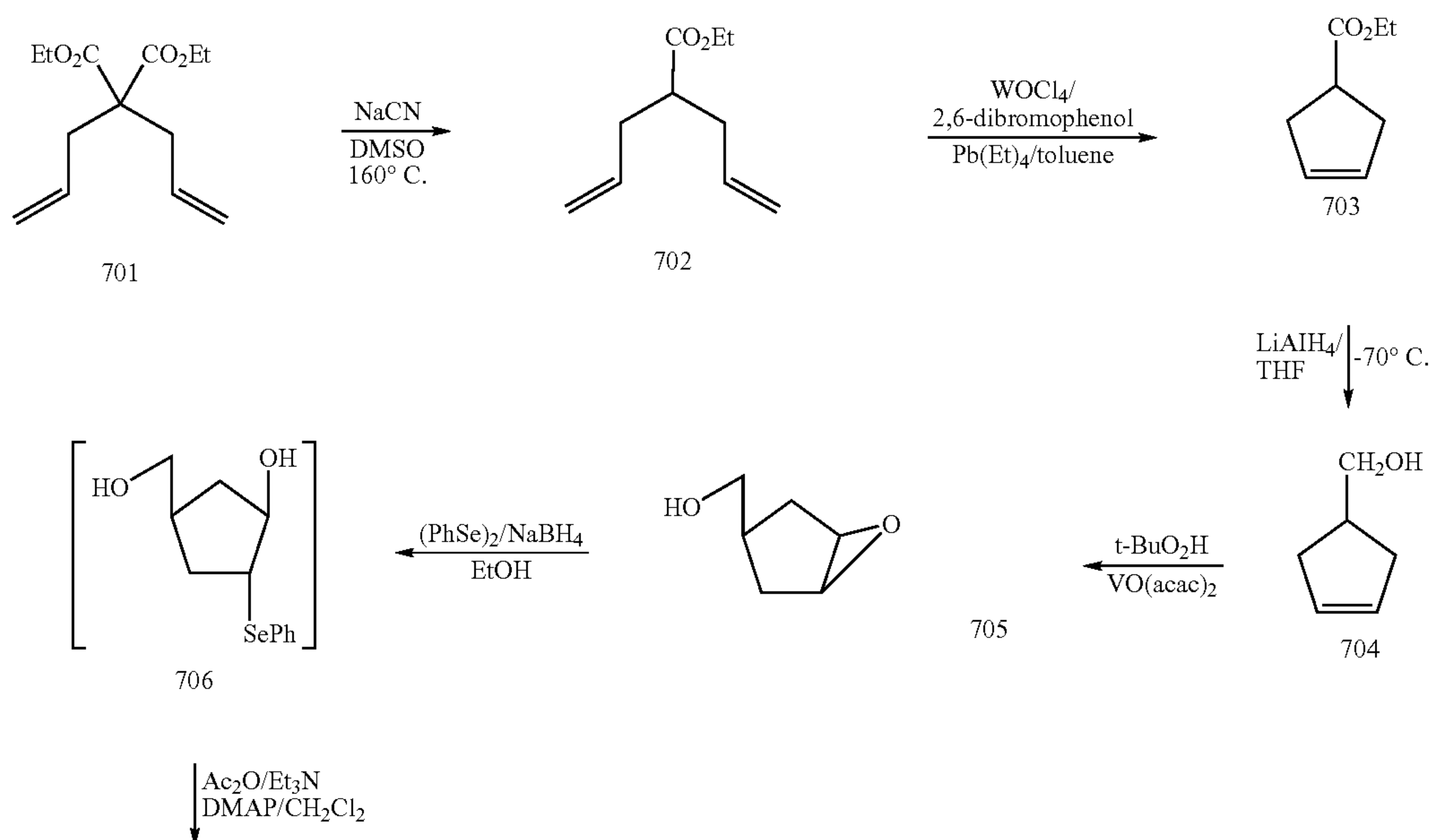
Scheme 11
