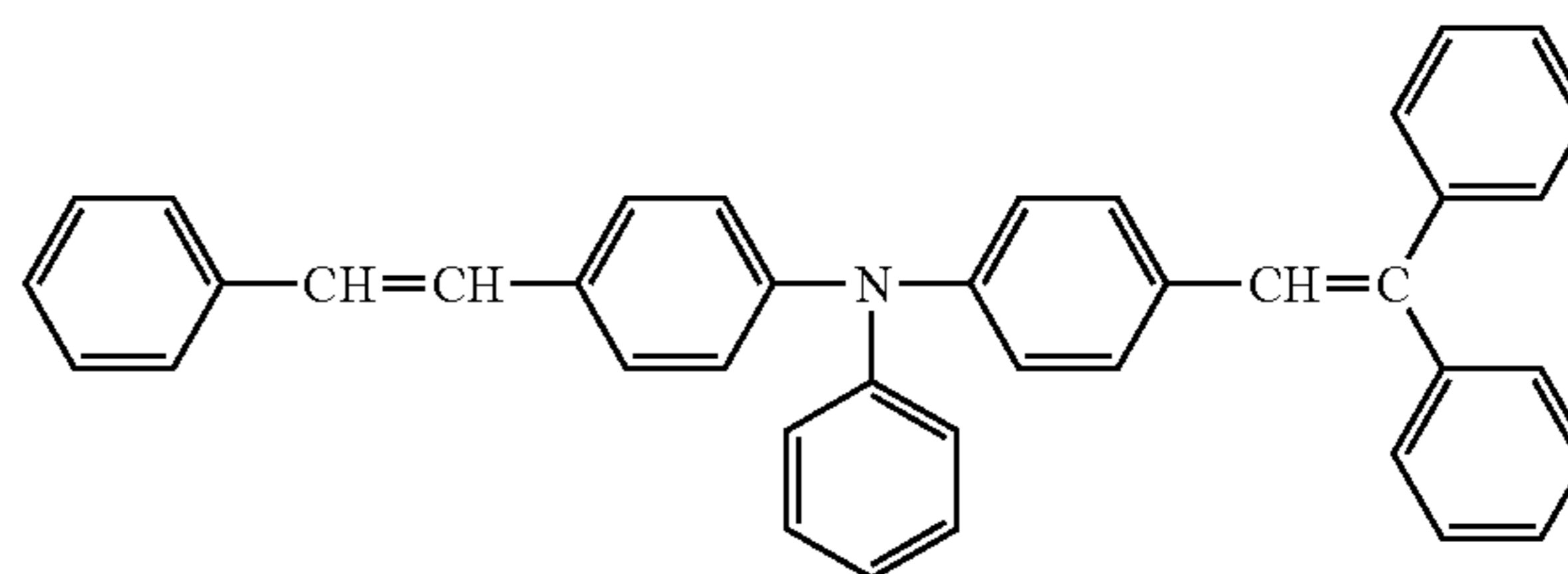
Structural Formula (2)
