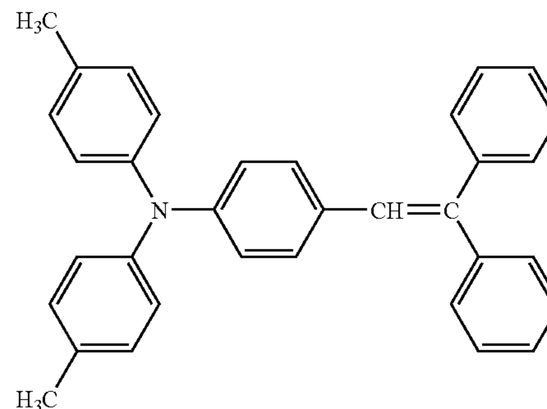
Structural Formula (1)
