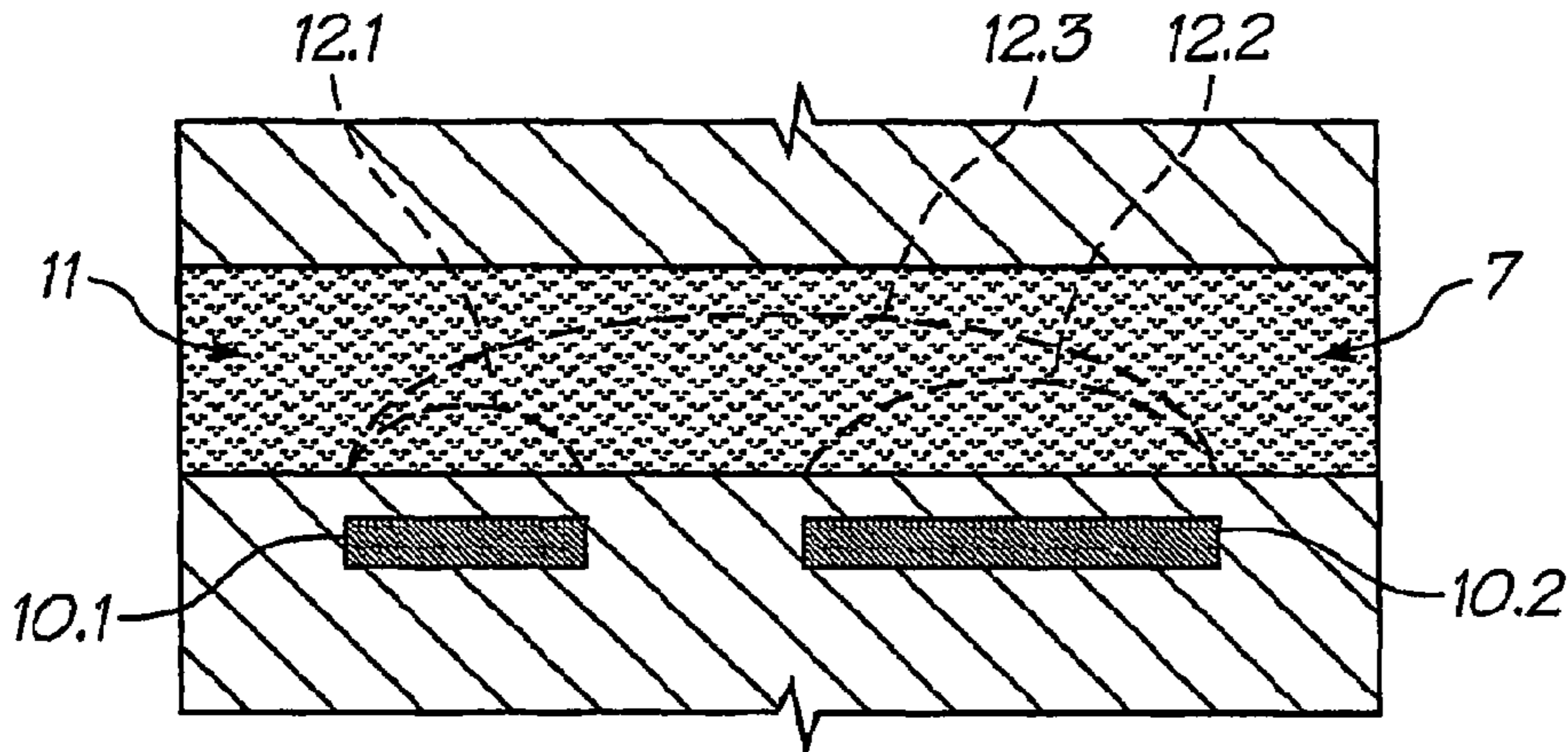
FIG. 52 (PRIOR ART)
