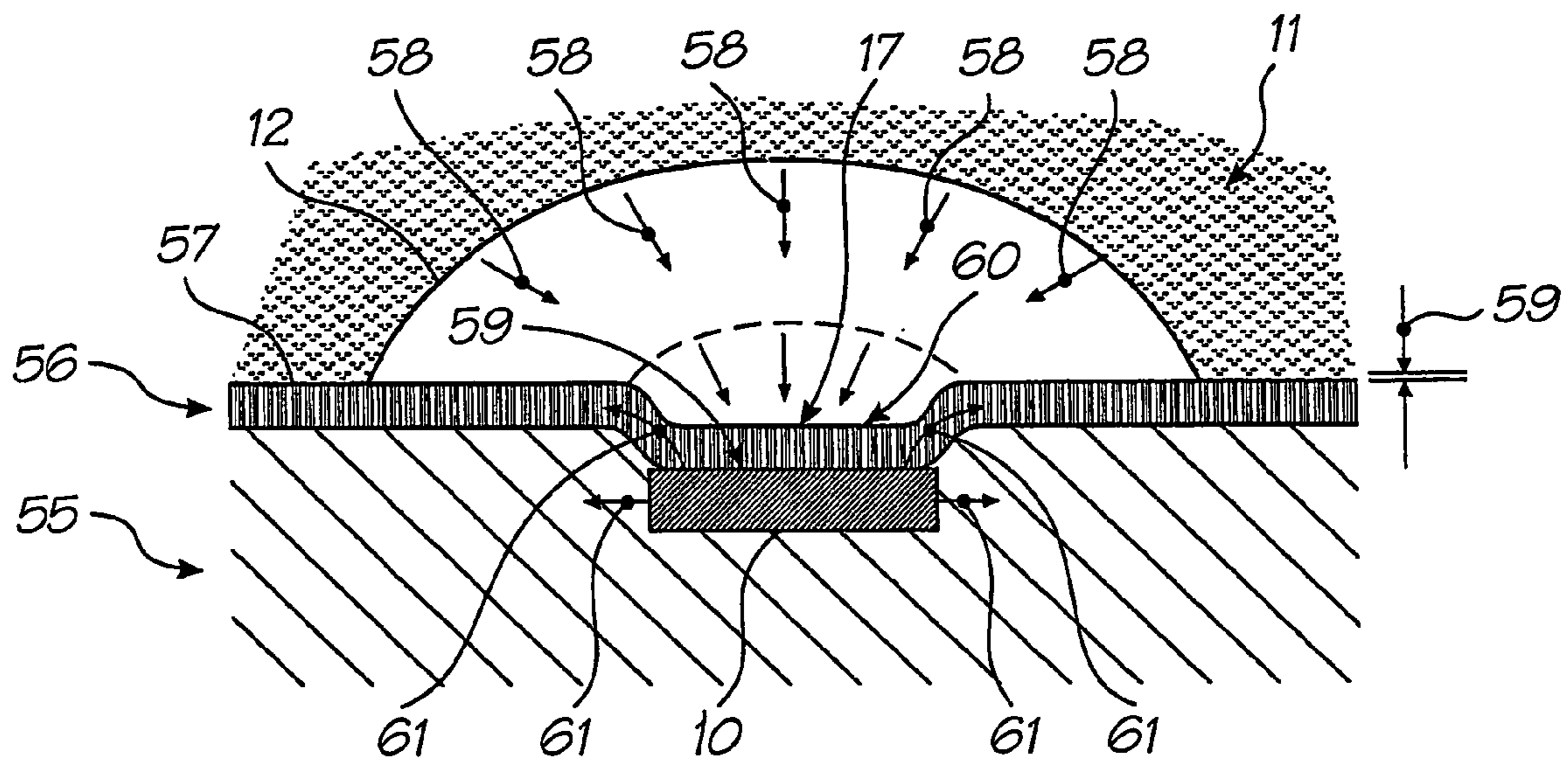
FIG. 47 (PRIOR ART)
