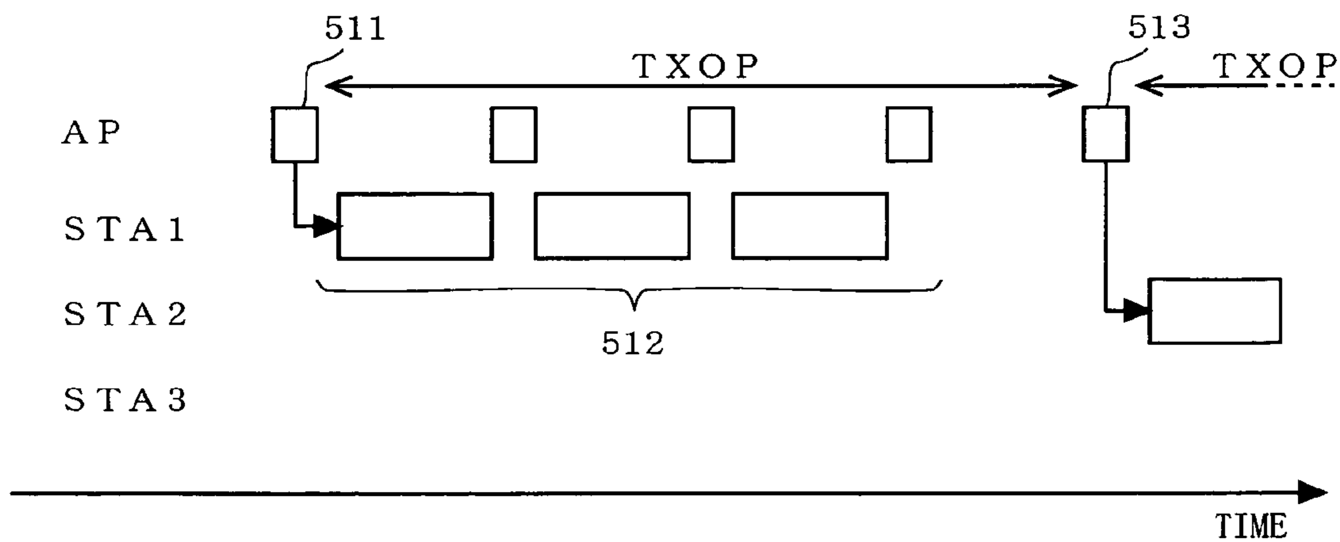
FIG. 25 PRIOR ART
