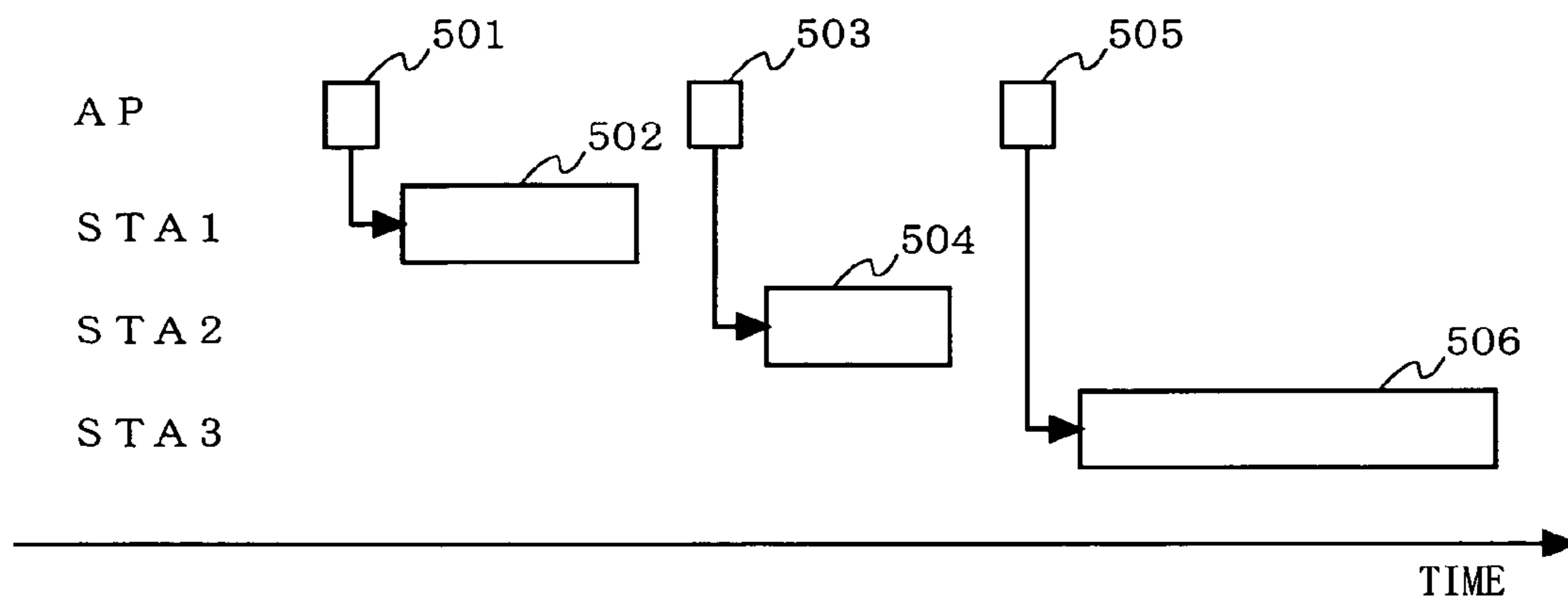
FIG. 24 PRIOR ART
