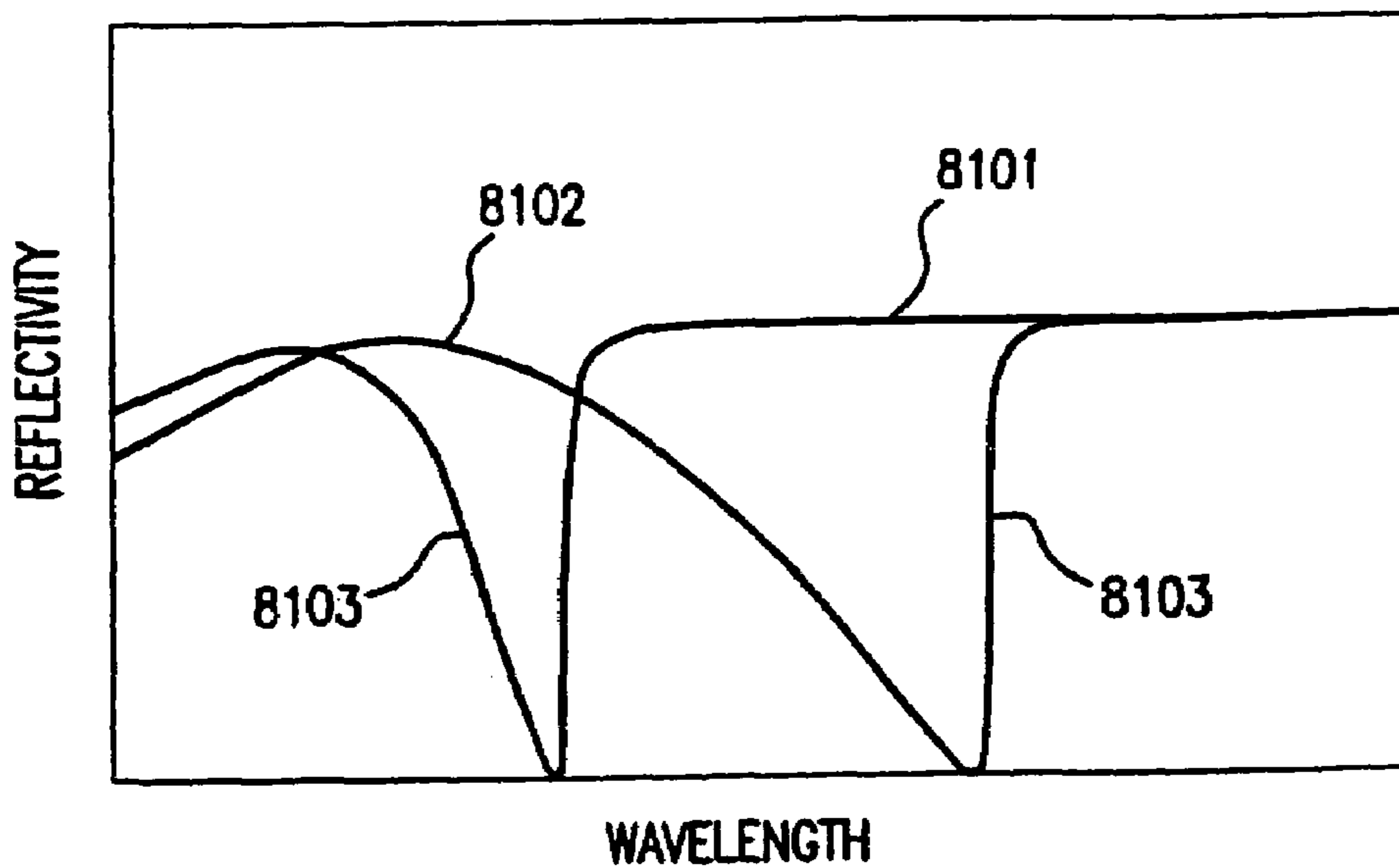
FIG. 81 PRIOR ART
