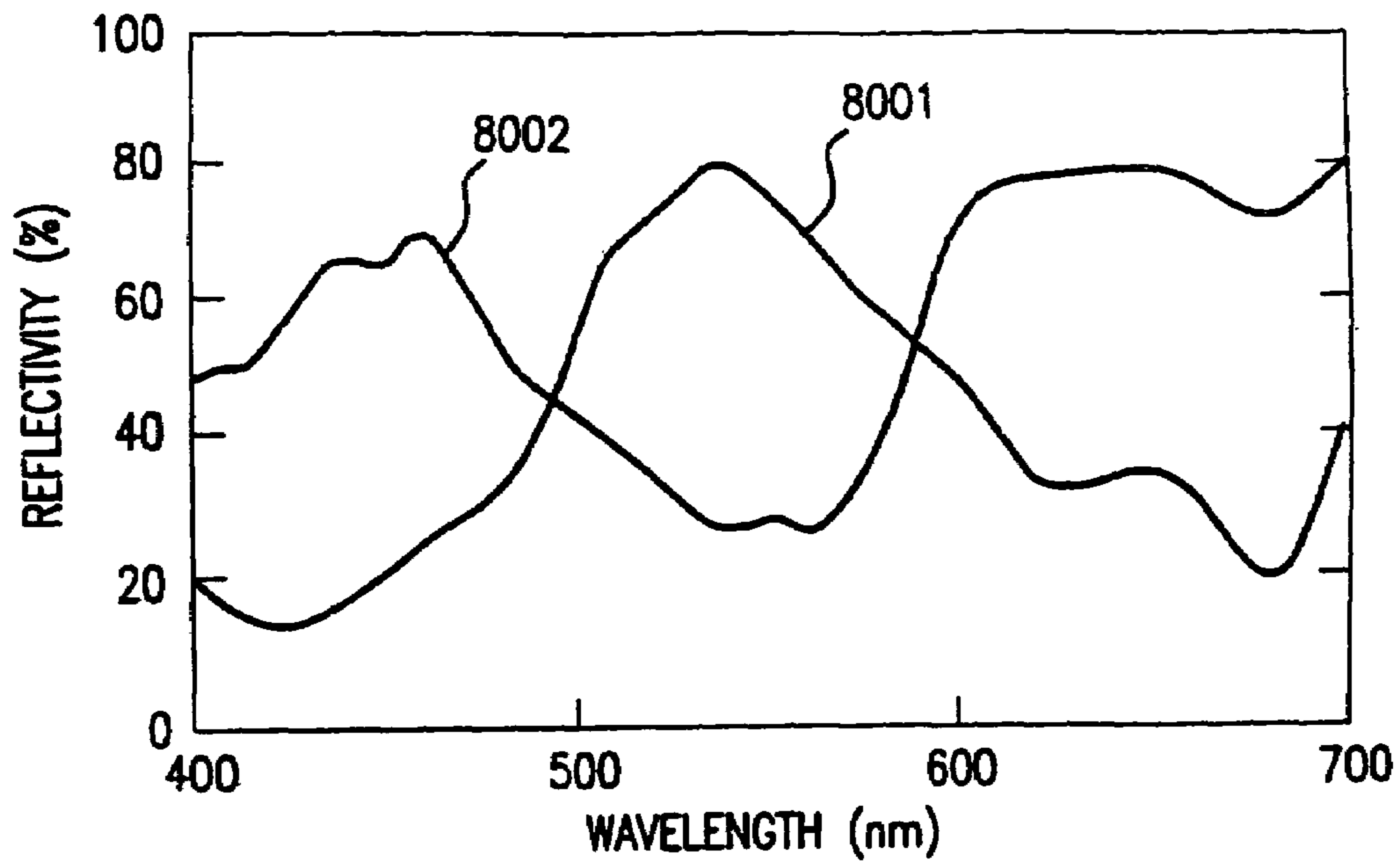
FIG. 80 PRIOR ART
