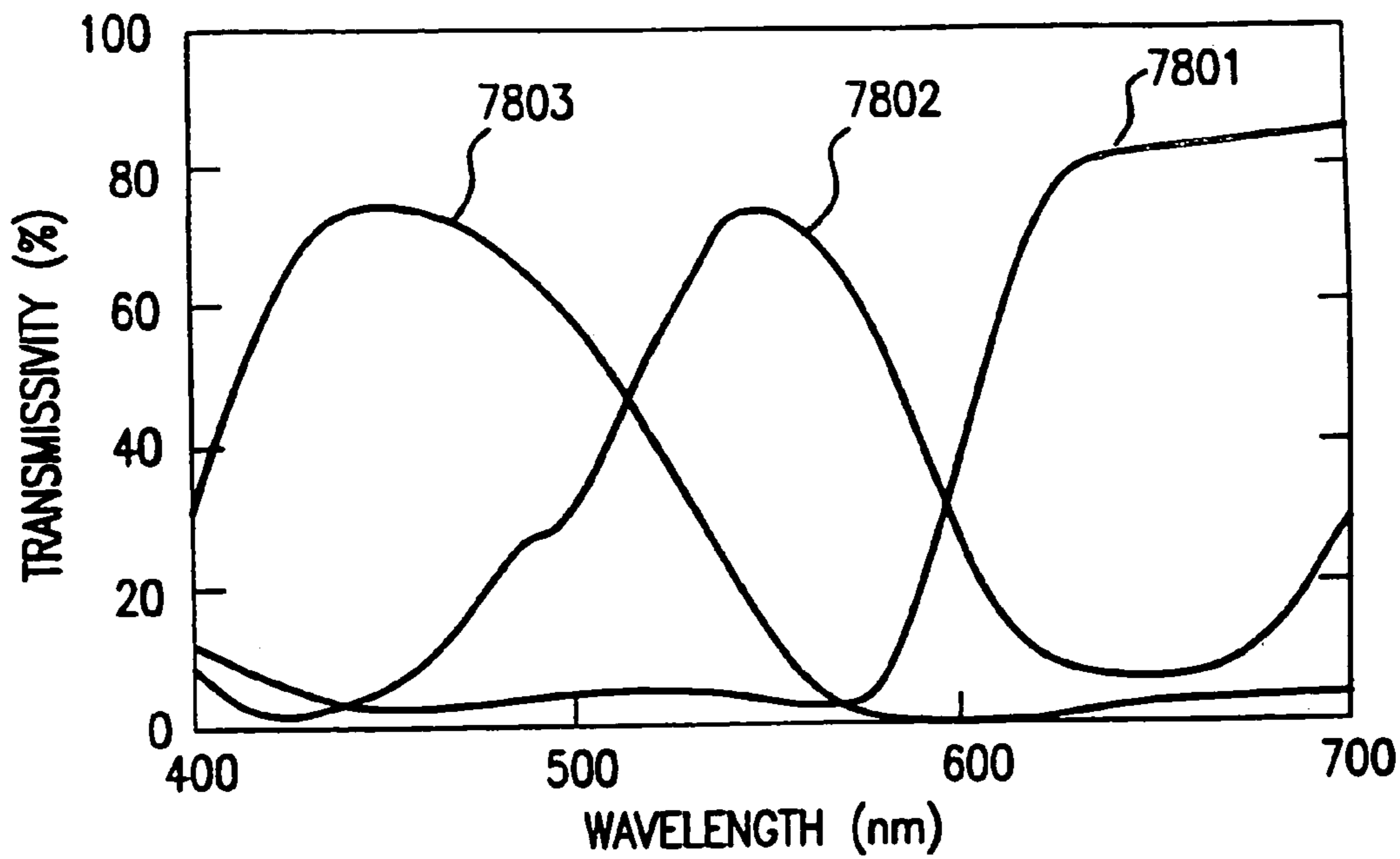
FIG. 78 PRIOR ART
