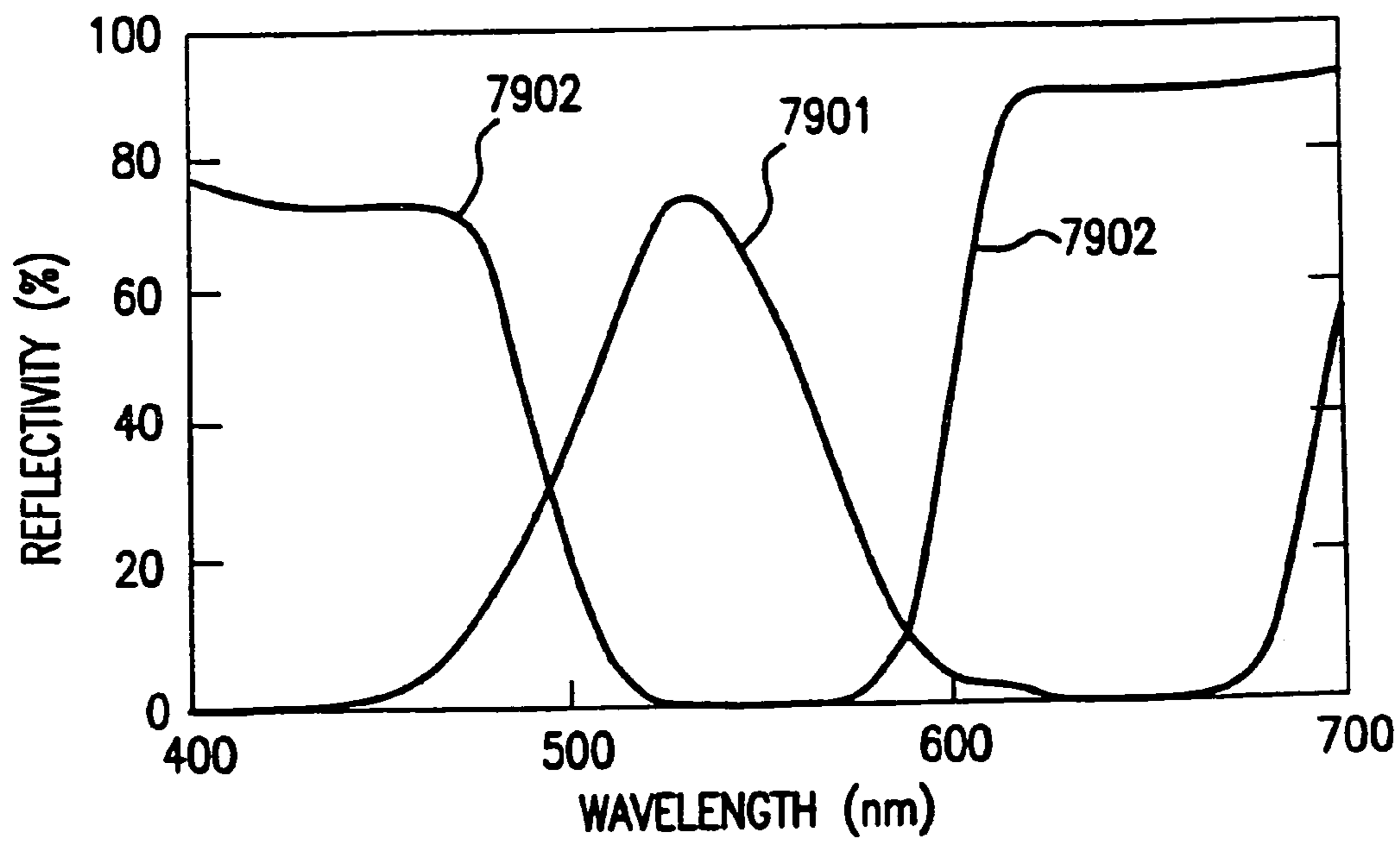
FIG. 79 PRIOR ART
