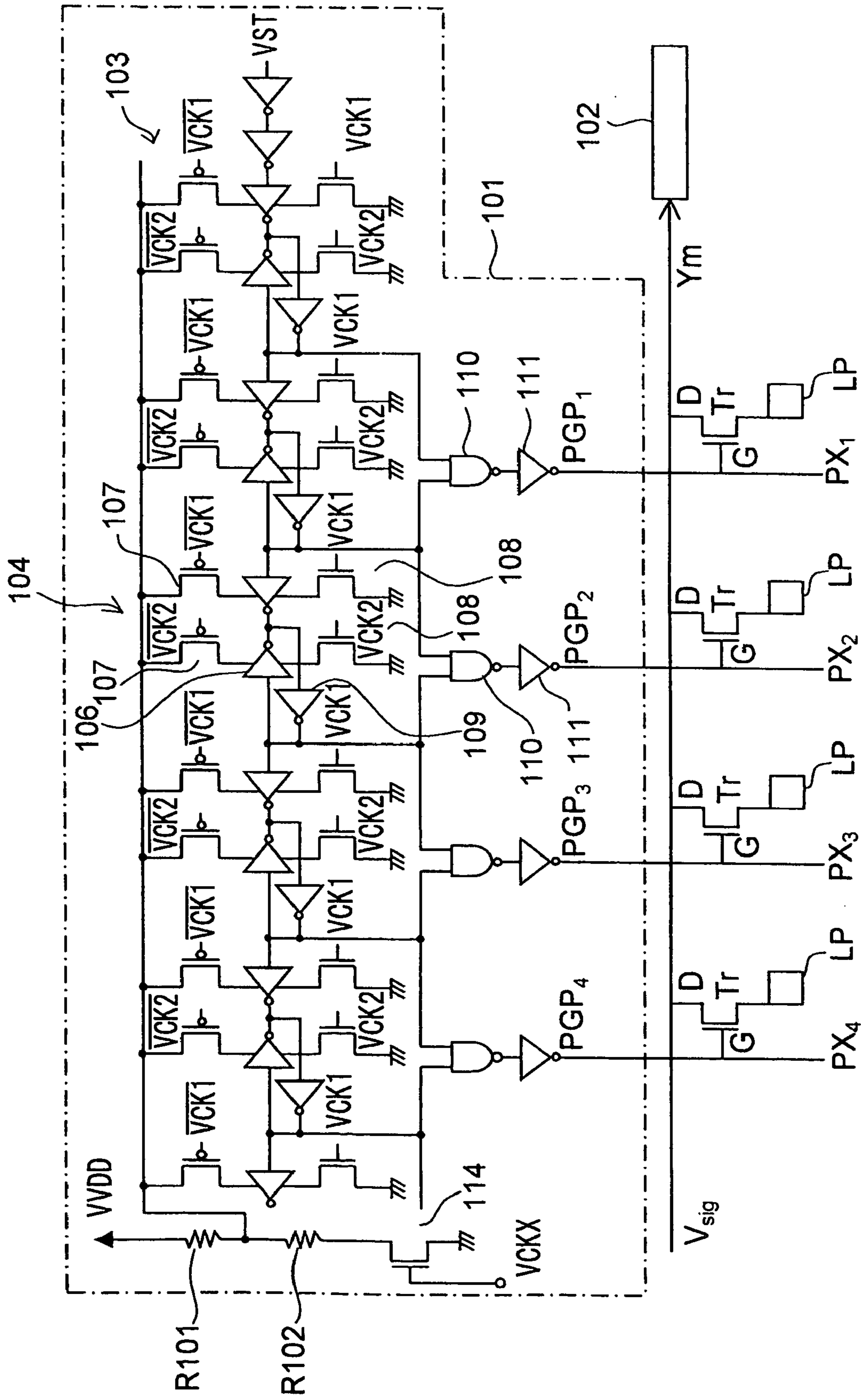
FIG. 8 PRIOR ART
