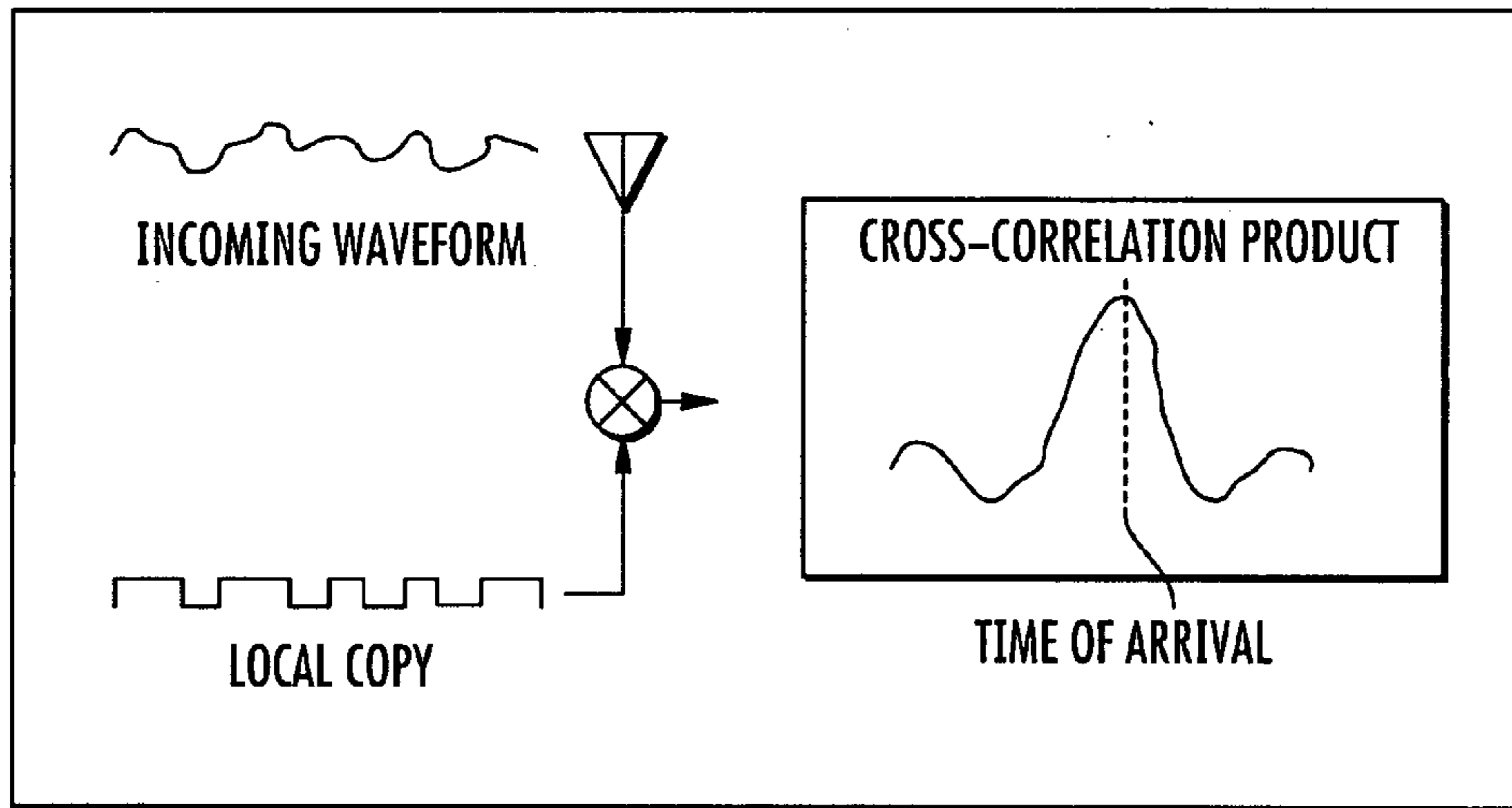
FIG. 3 PRIOR ART
