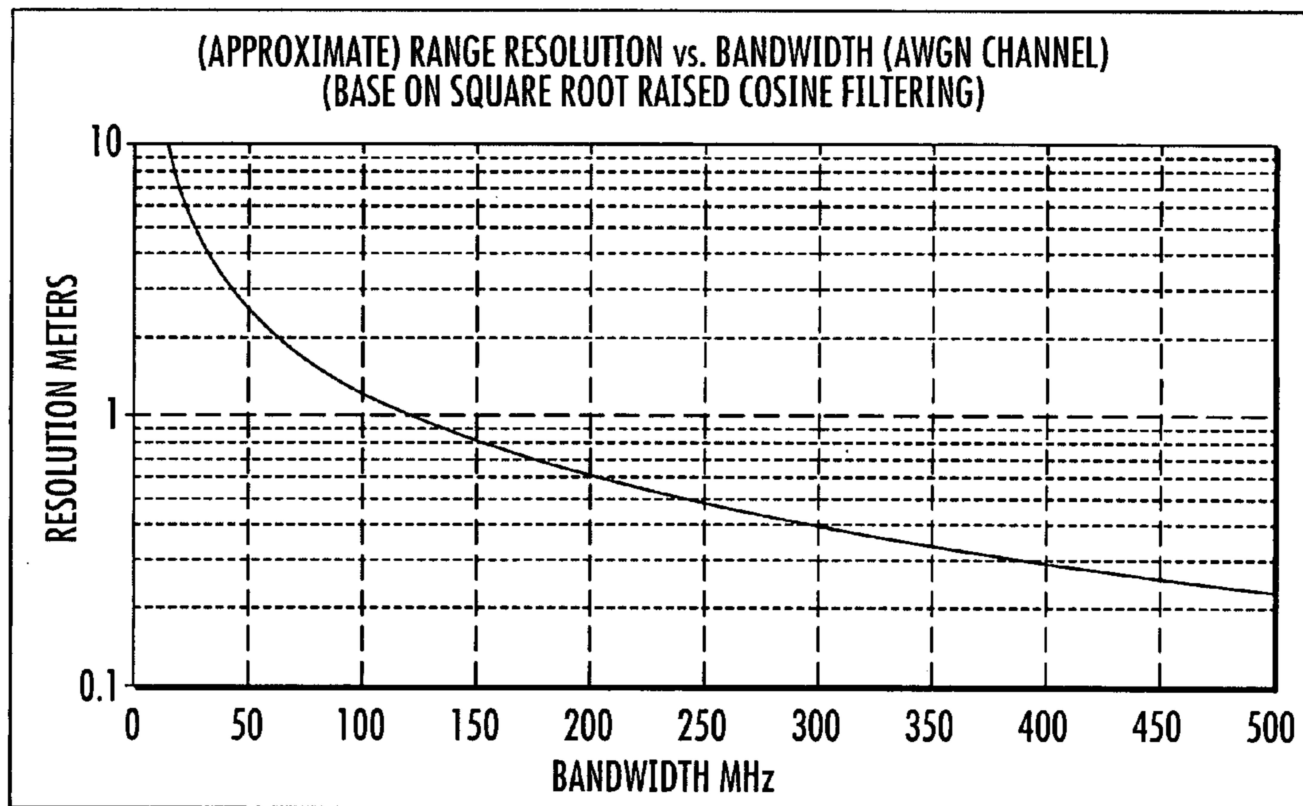
FIG. 4 PRIOR ART
