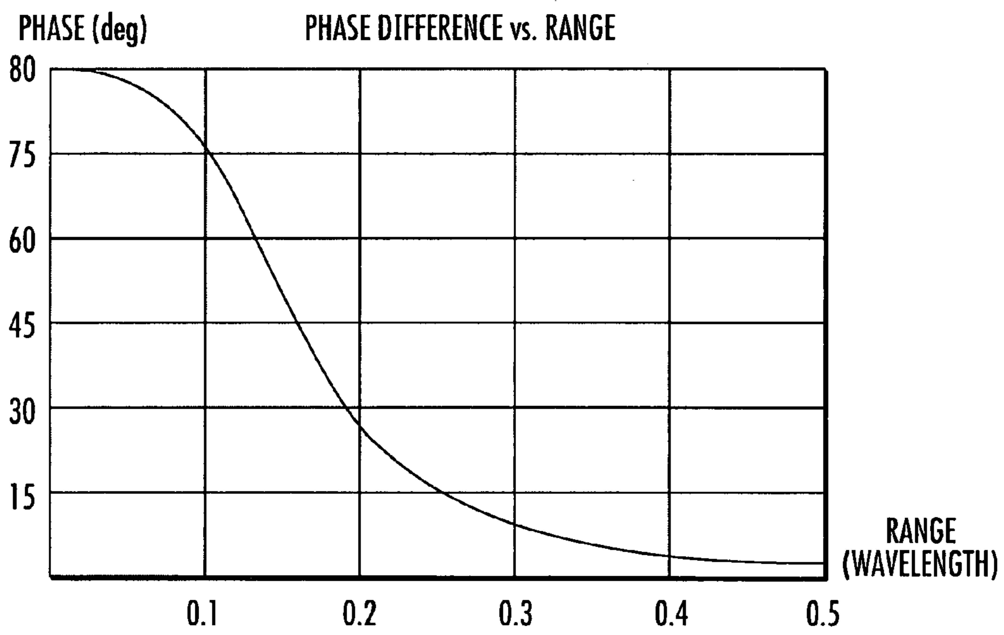
FIG. 9 PRIOR ART
