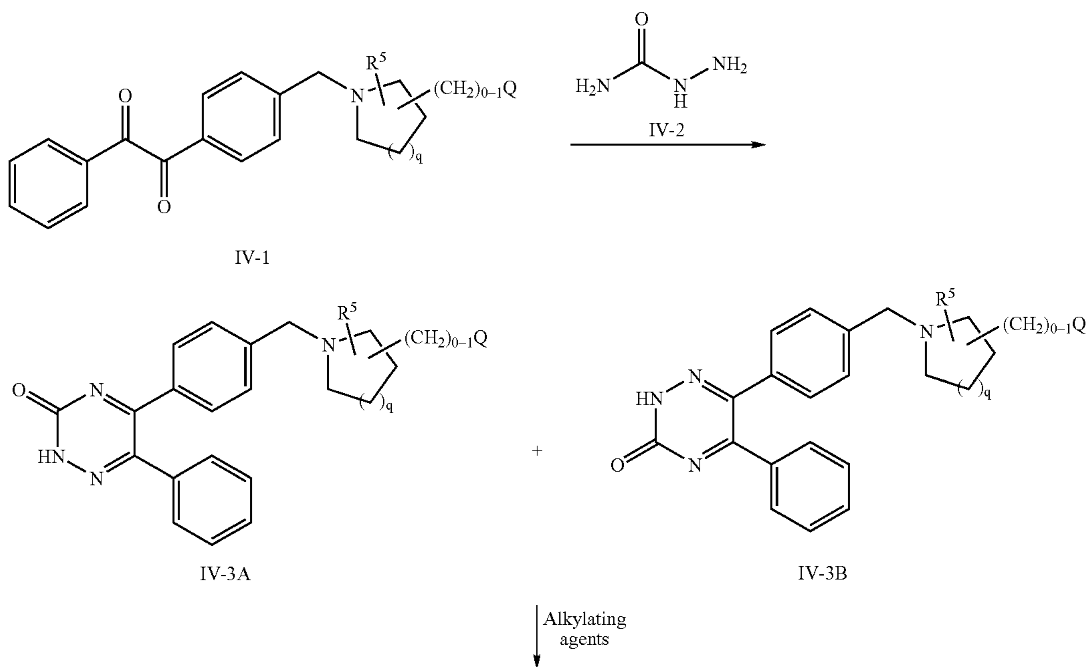
Reaction Scheme IV
