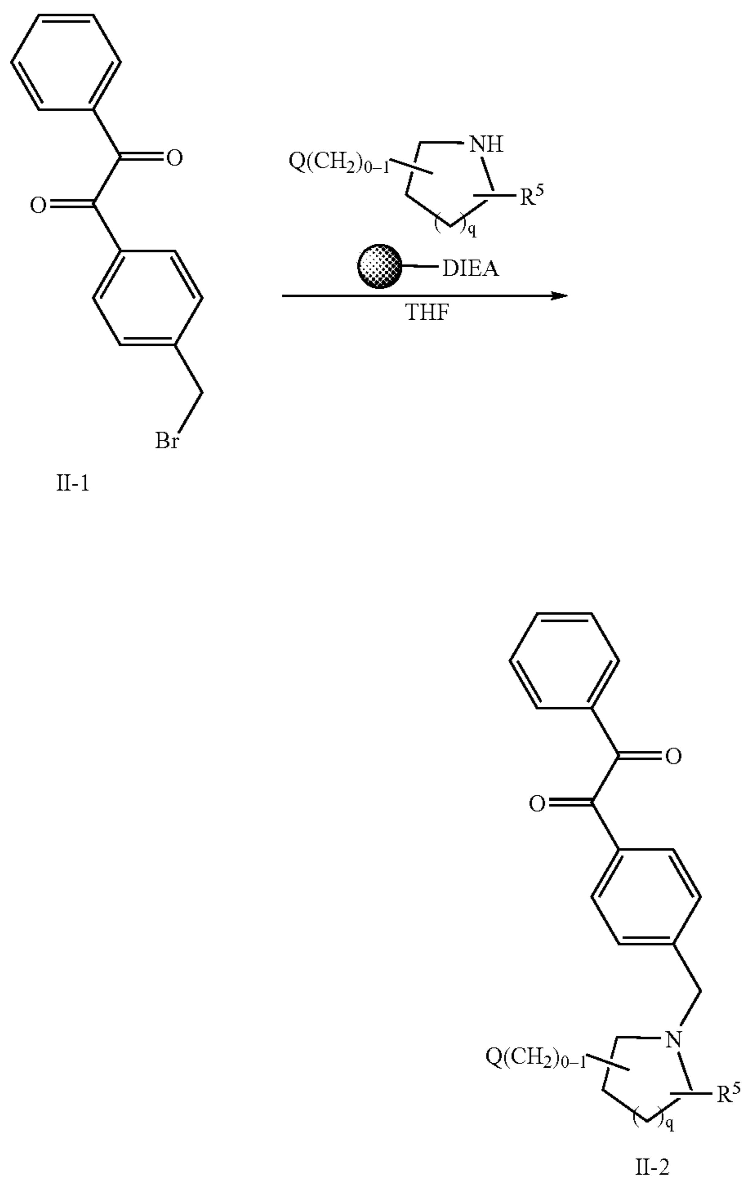
Reaction Scheme II
