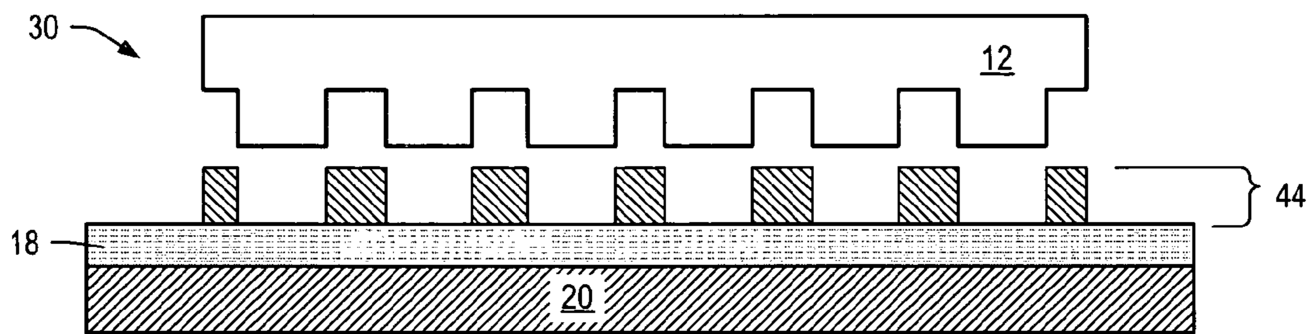
FIG. 2D
