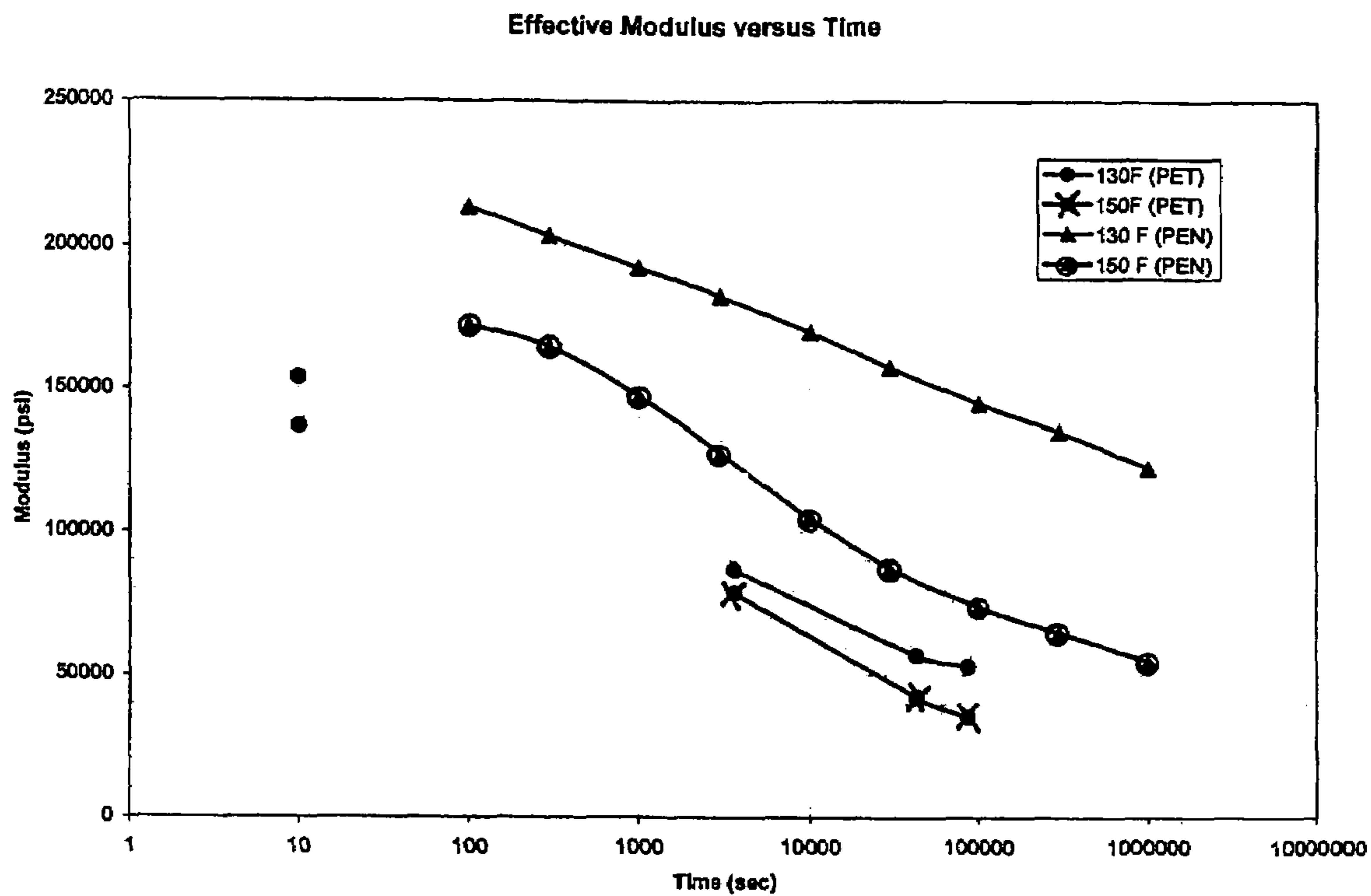
Effective Modulus vs. Time for PET / PEN at 130°F, 150° F
