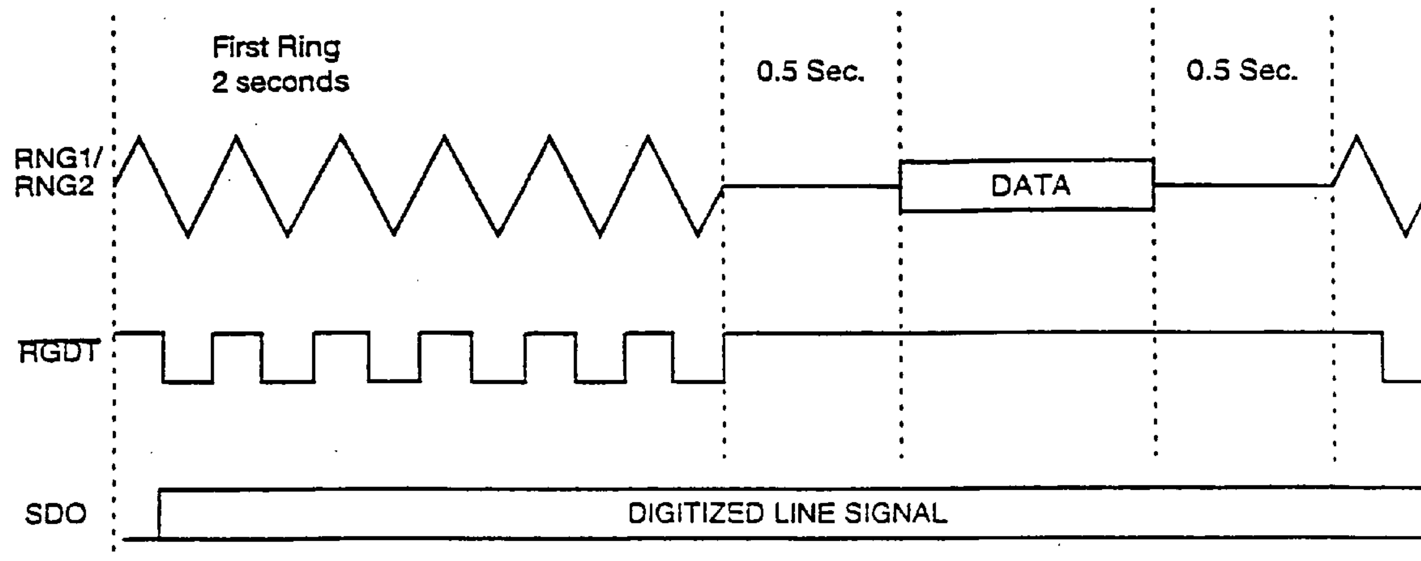
Figure 10. Ring Detect Timing
