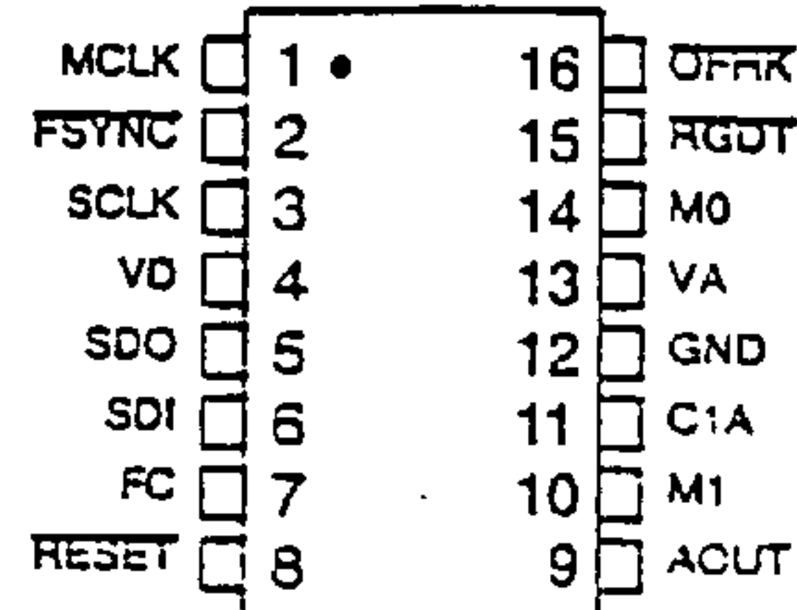
Figure 16. Si3032A Pin Configuration
