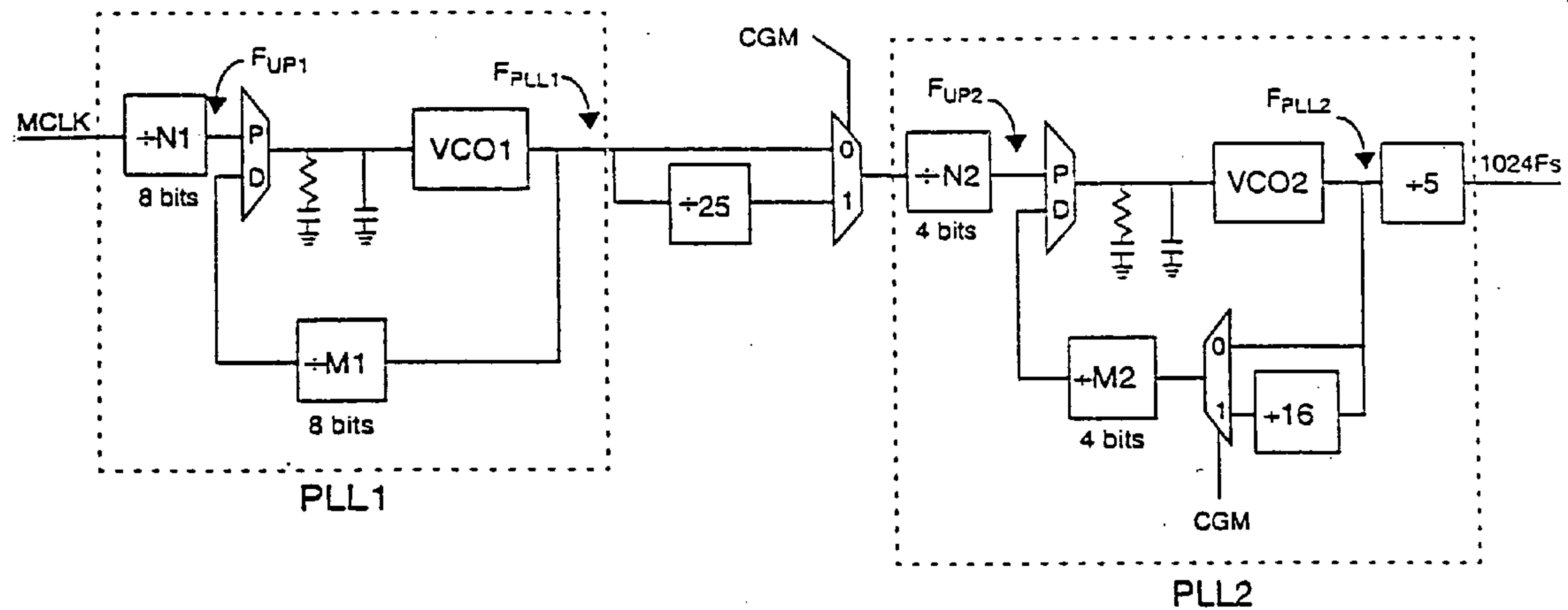
Figure 11. Clock Generation Subsystem
