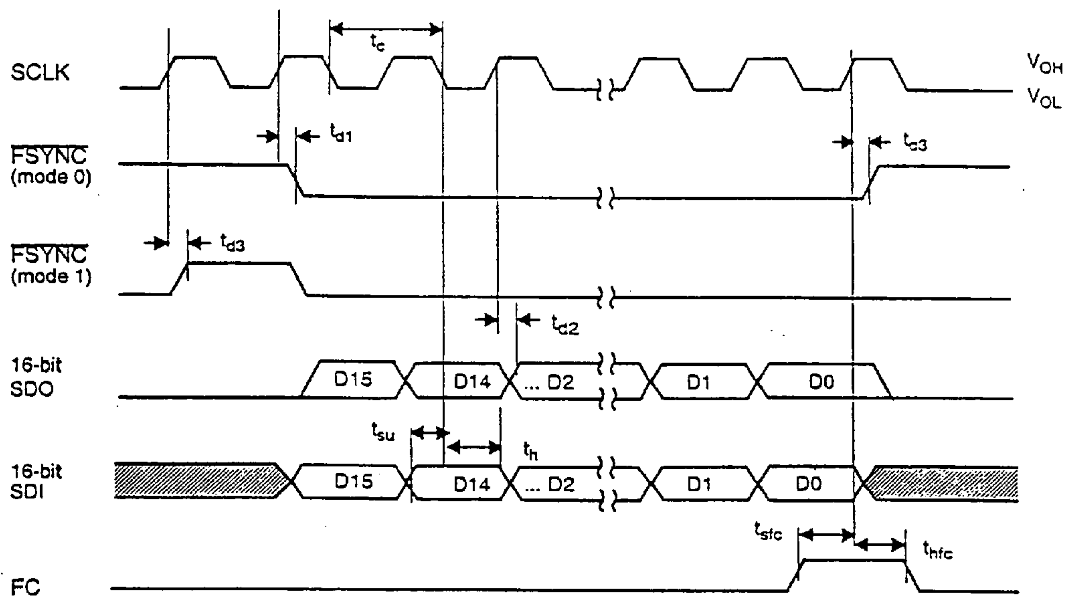
Figure 2. Serial Interface Timing Diagram
