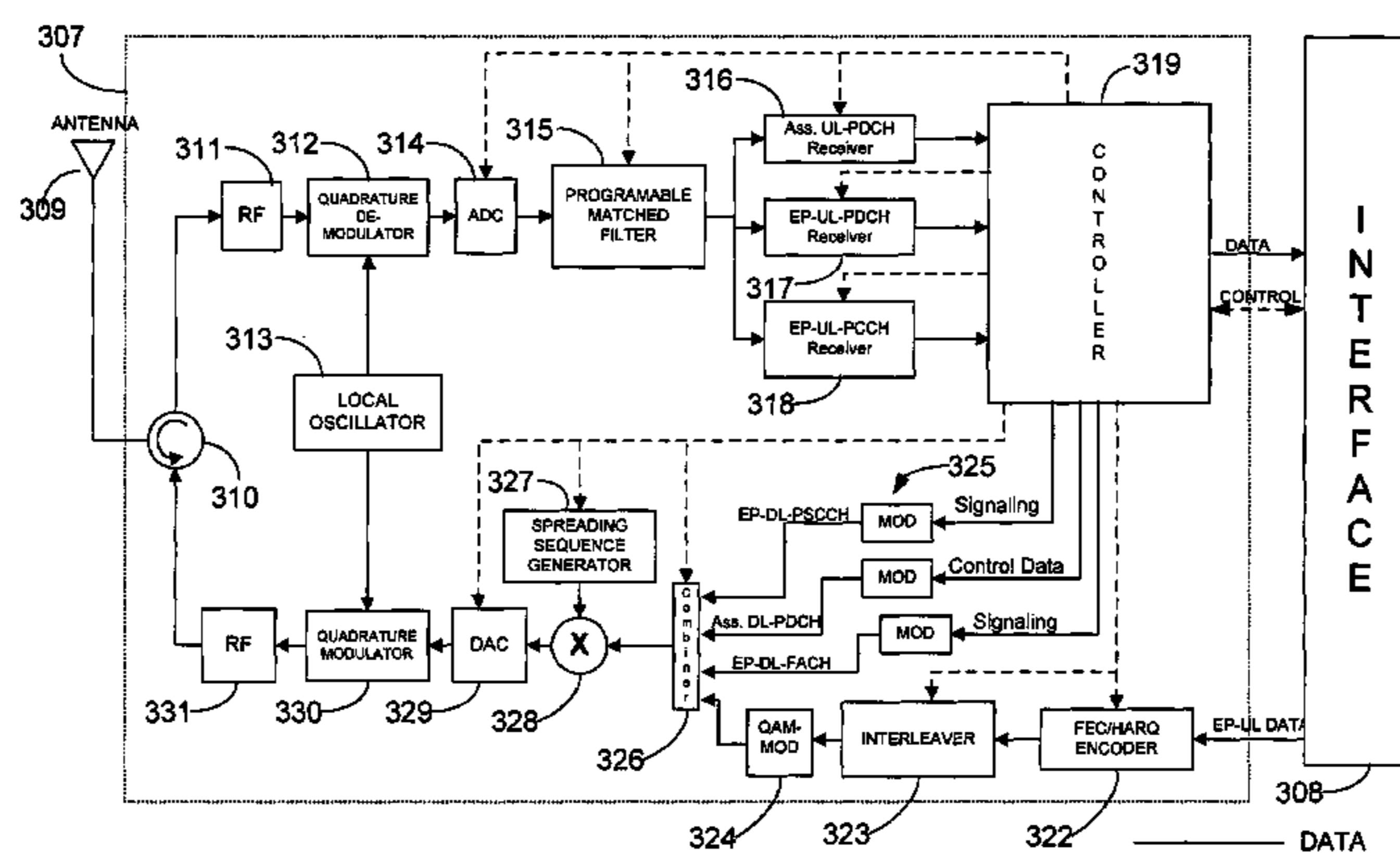
Base Station (Node-B) Tranceiver for Enhanced Uplink Packet Communications.
