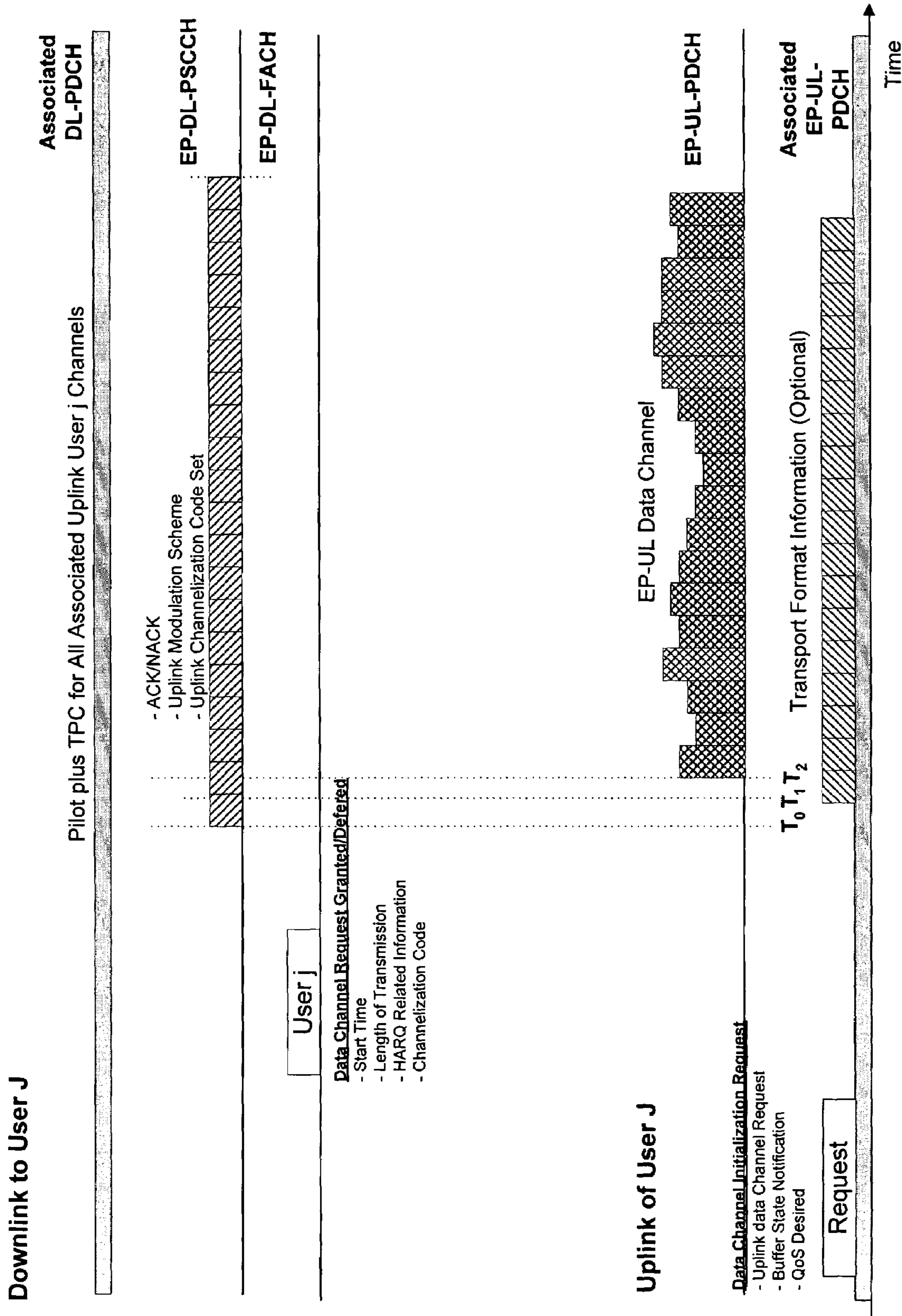
Fig. 3 EP-UL Packet Transfer Protocol
