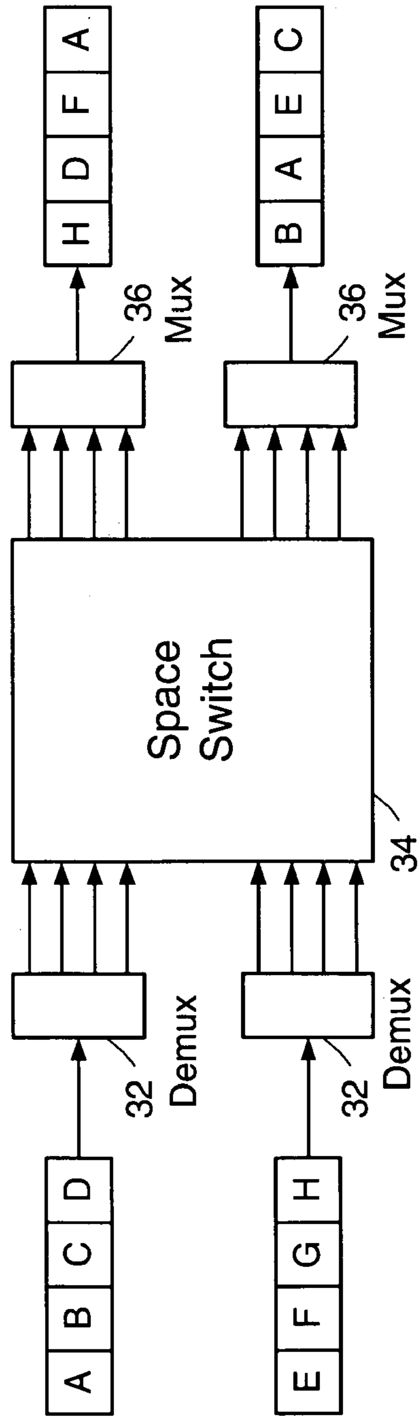
FIG. 2 PRIOR ART
