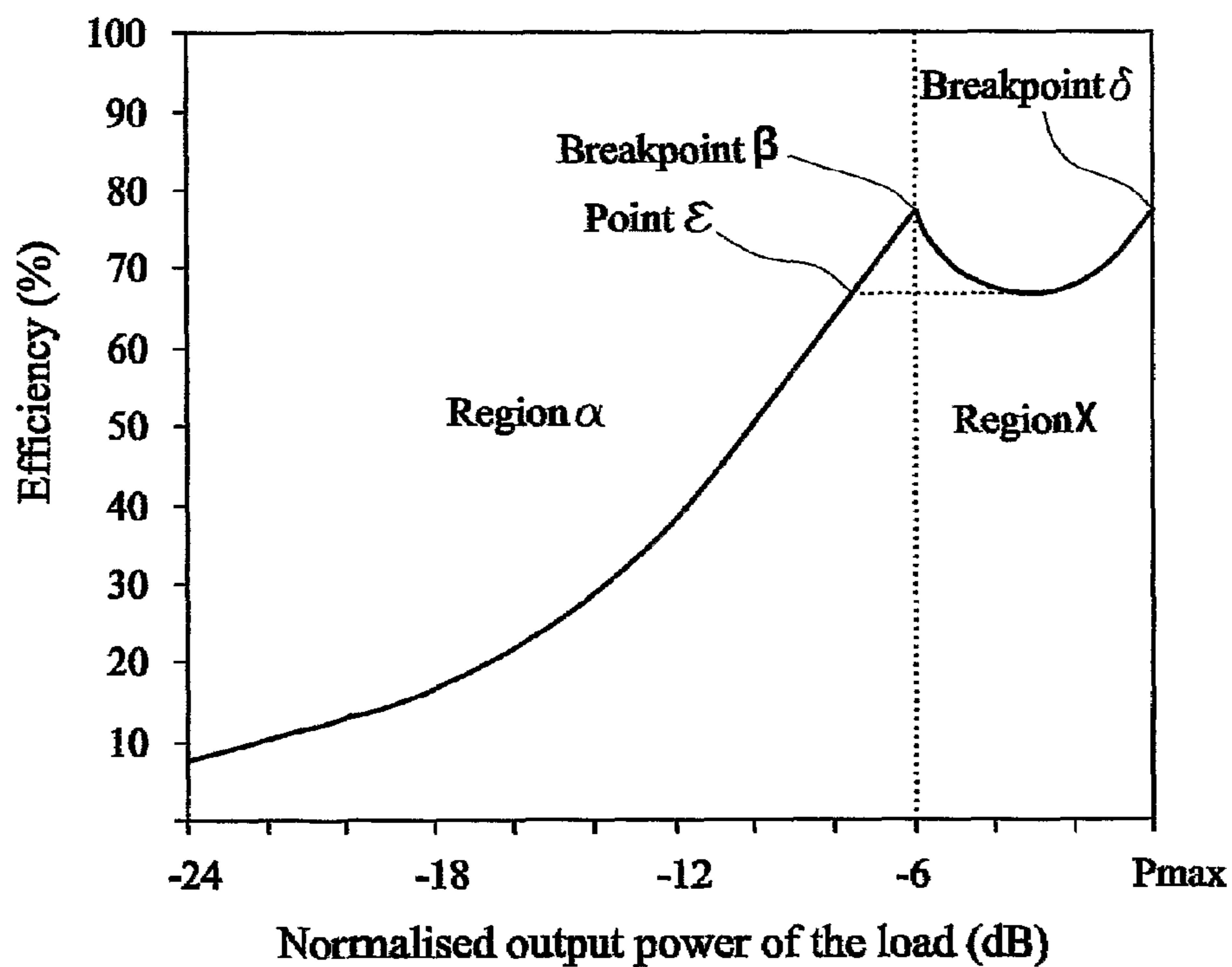
Theoretical efficiency v output power
