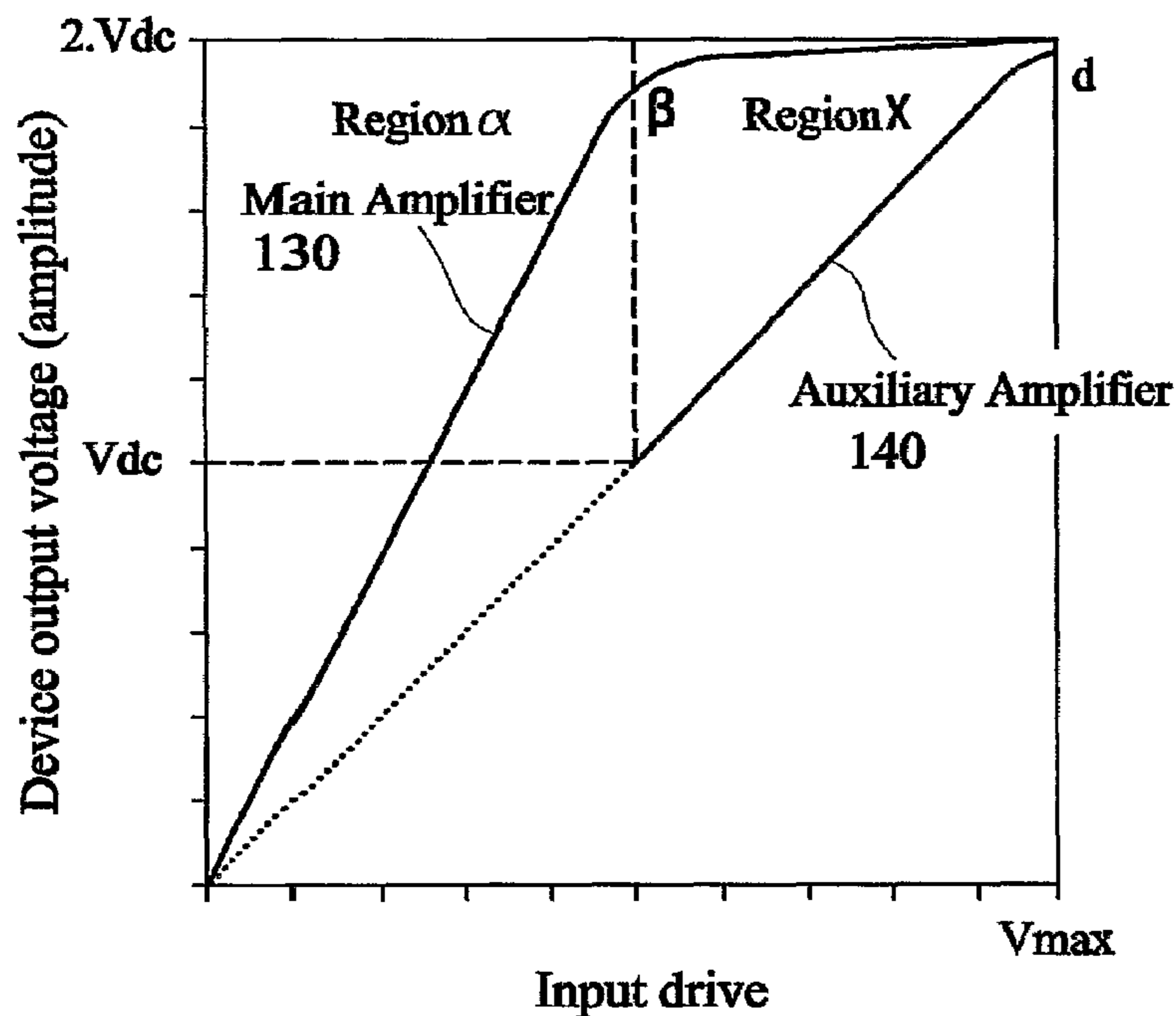
Theoretical plot of output voltage from each device v input drive
