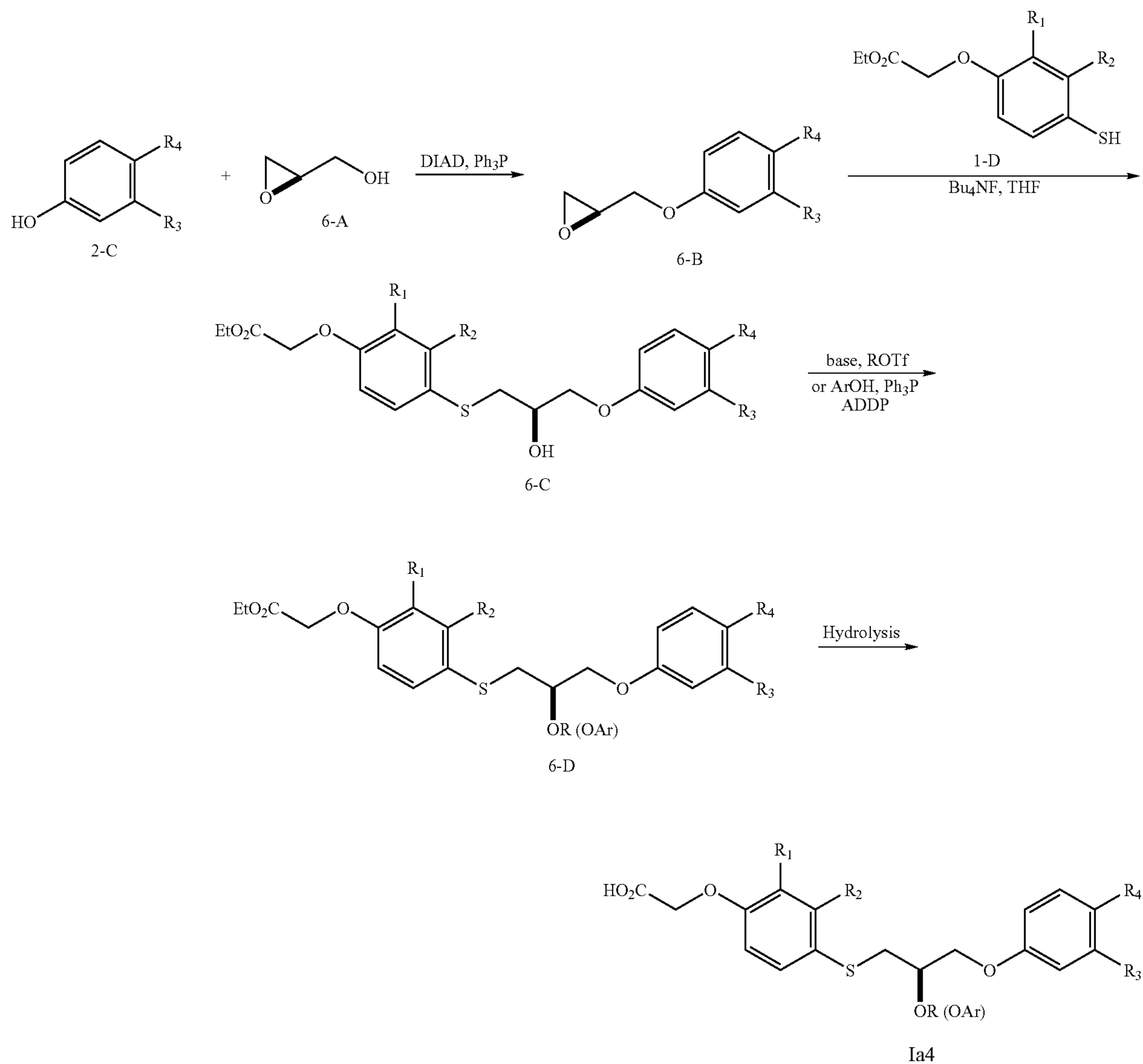
Scheme 6. Synthesis of Compound Ia4
