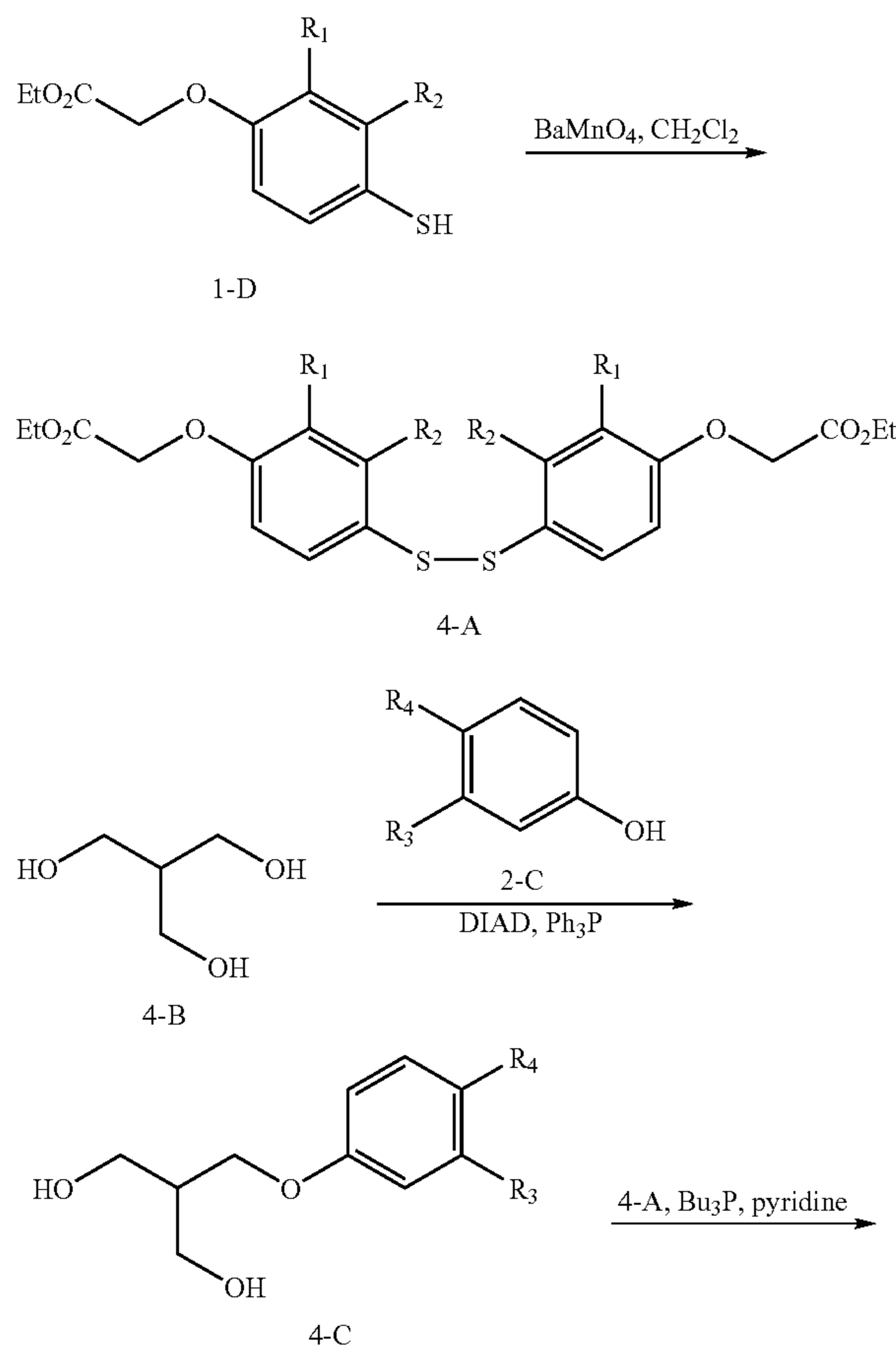
Scheme 4. Synthesis of Compound Ia2
