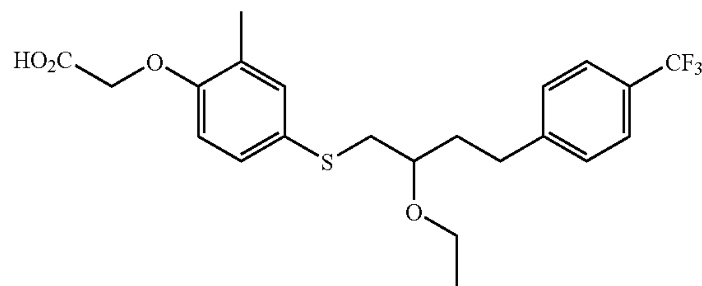
{4-[2-Ethoxy-4-(4-trifluoromethyl-phenyl)-butylsulfanyl]-2-methyl-phenoxy}acetic Acid
