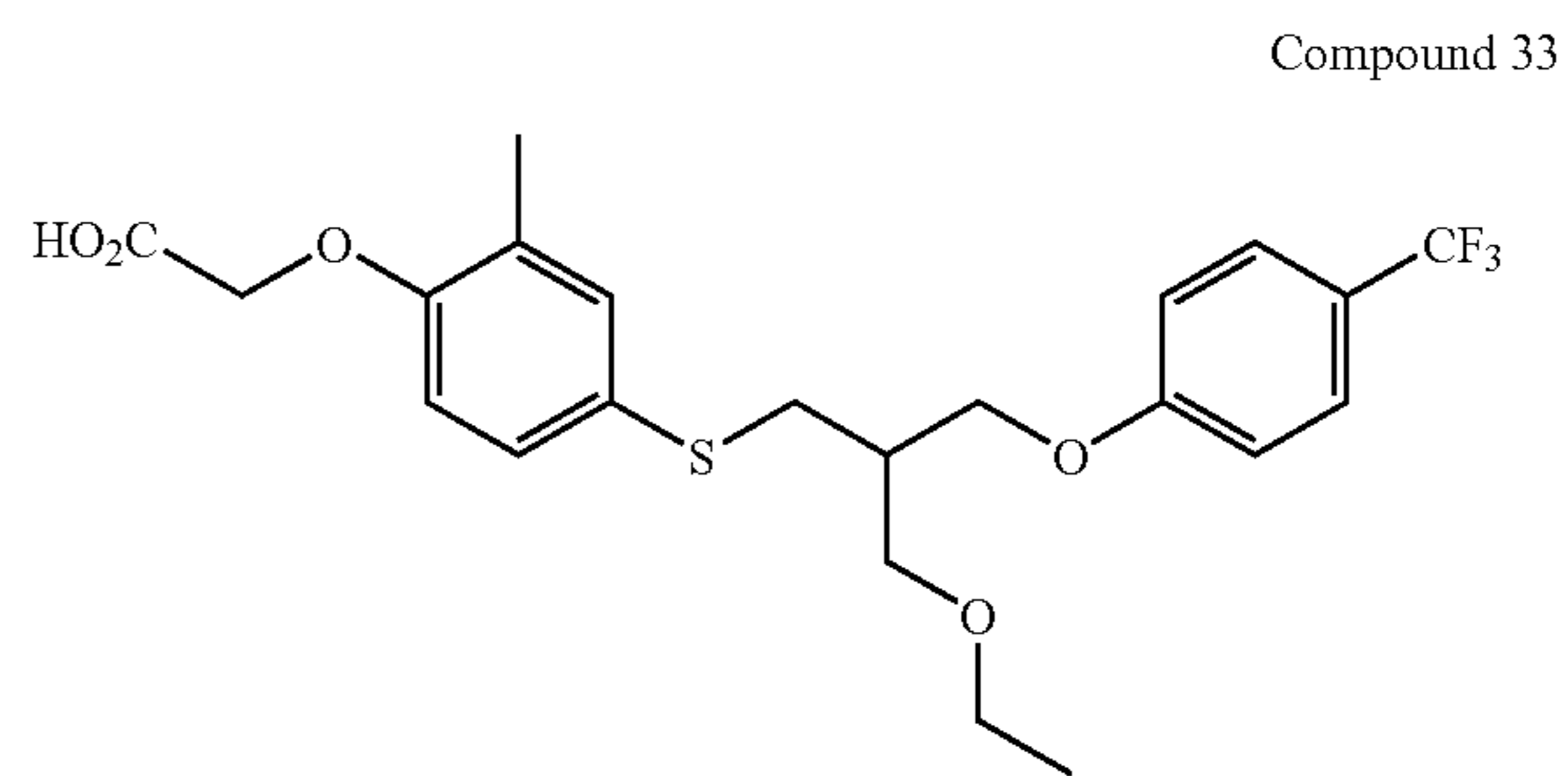
{4-[2-Ethoxymethyl-3-(4-trifluoromethyl-phenoxy)-propylsulfanyl]-2-methyl-phenoxy}-acetic Acid
