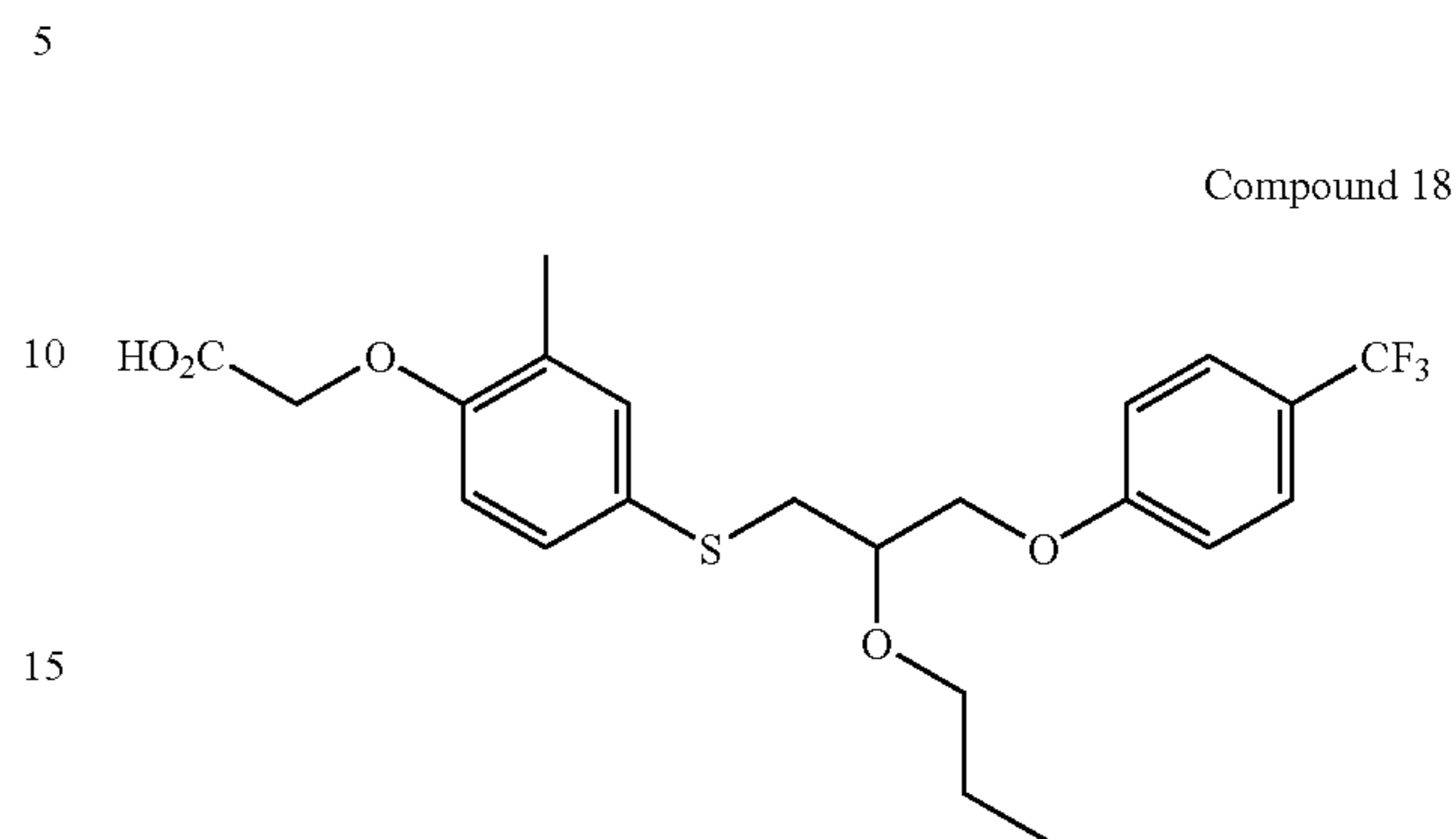
{2-Methyl-4-[2-propoxy-3-(4-trifluoromethyl-phenoxy)-propylsulfanyl]-phenoxy}acetic Acid
