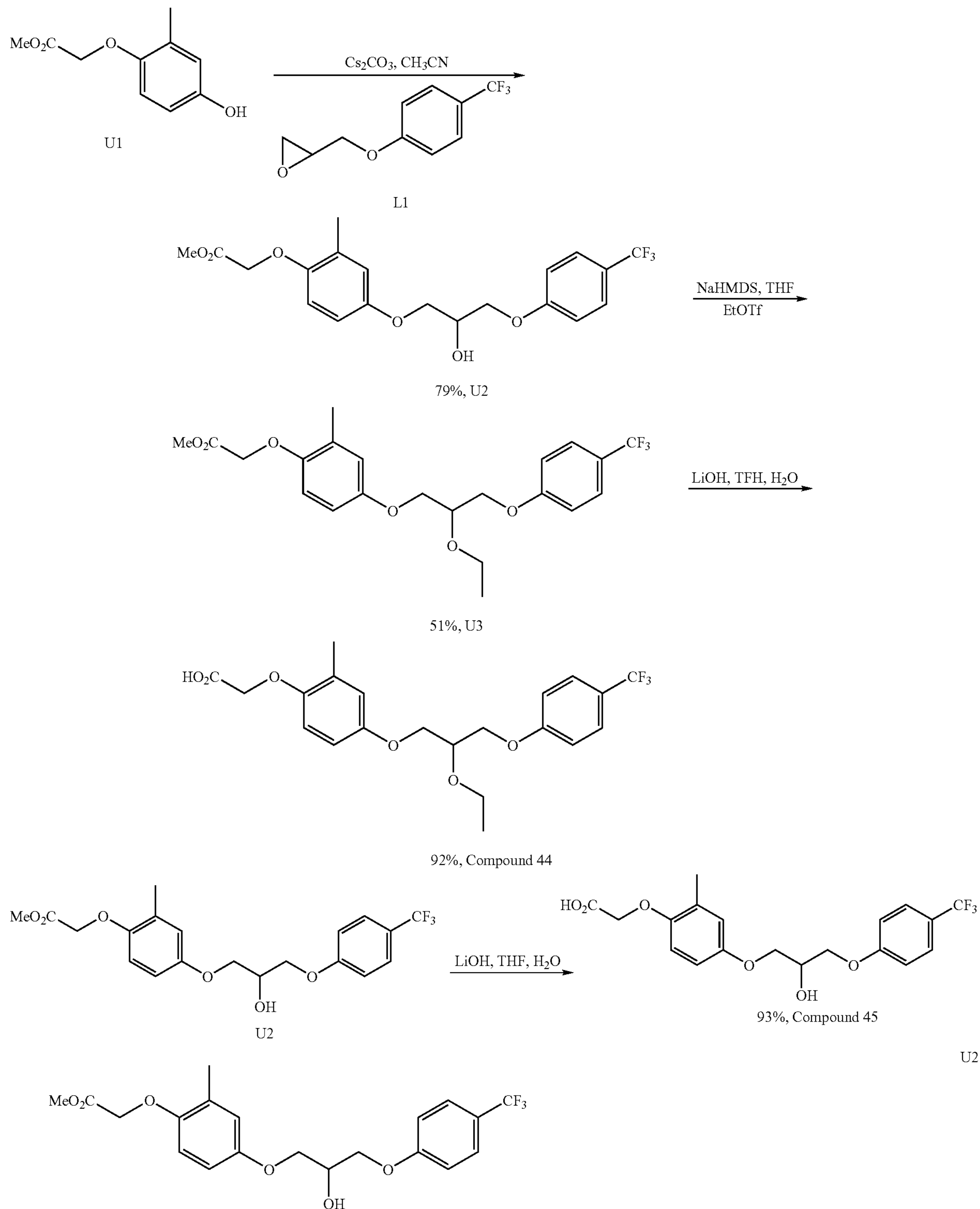
Scheme U
