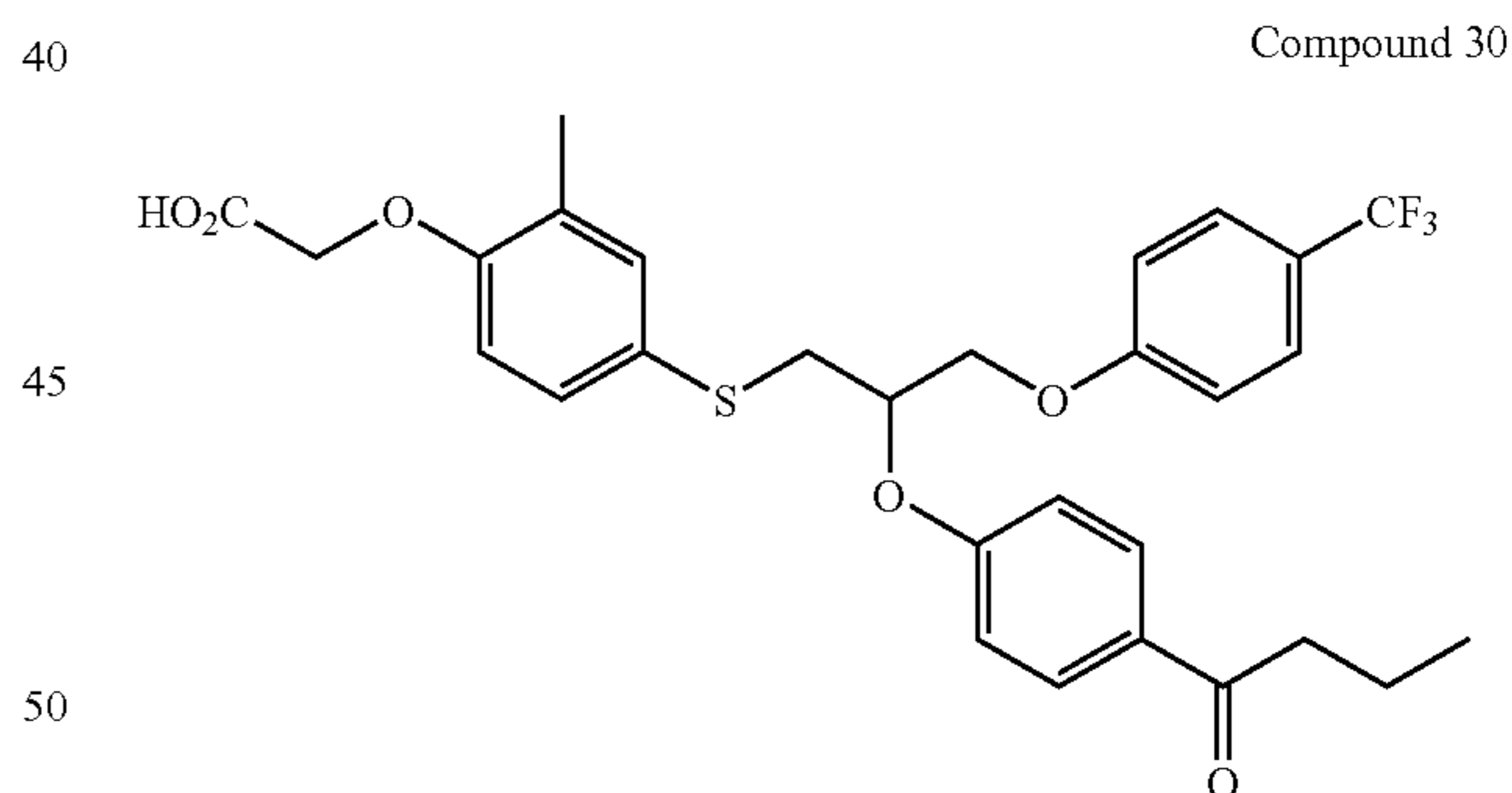
{4-[2-(4-Butyryl-phenoxy)-3-(4-trifluoromethyl-phenoxy)-propylsulfanyl]-2-methyl-phenoxy}-acetic Acid
