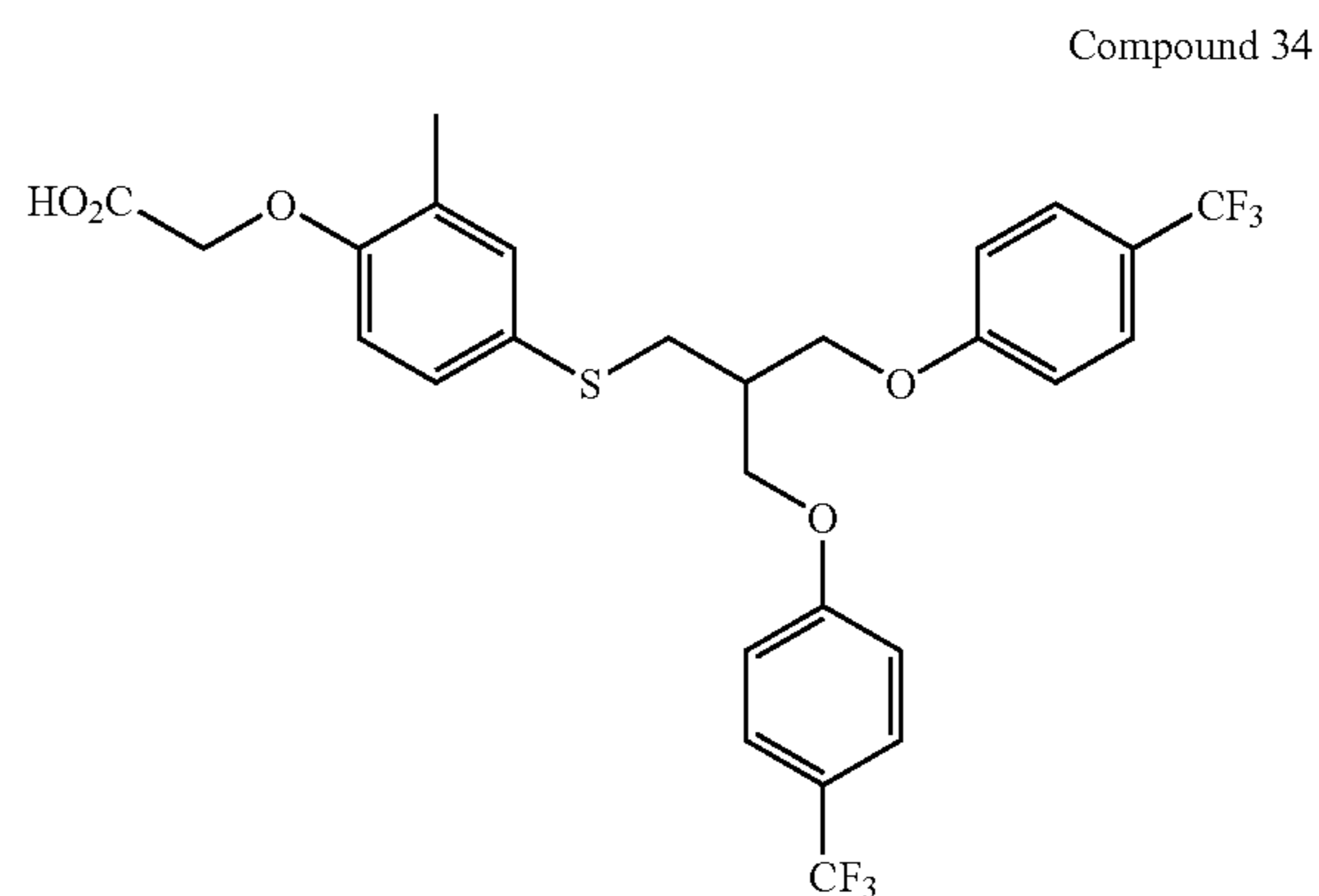
{2-Methyl-4-[3-(4-trifluoromethyl-phenoxy)-2-(4-trifluoromethyl-phenoxy)-propylsulfanyl]-phenoxy}-acetic Acid
