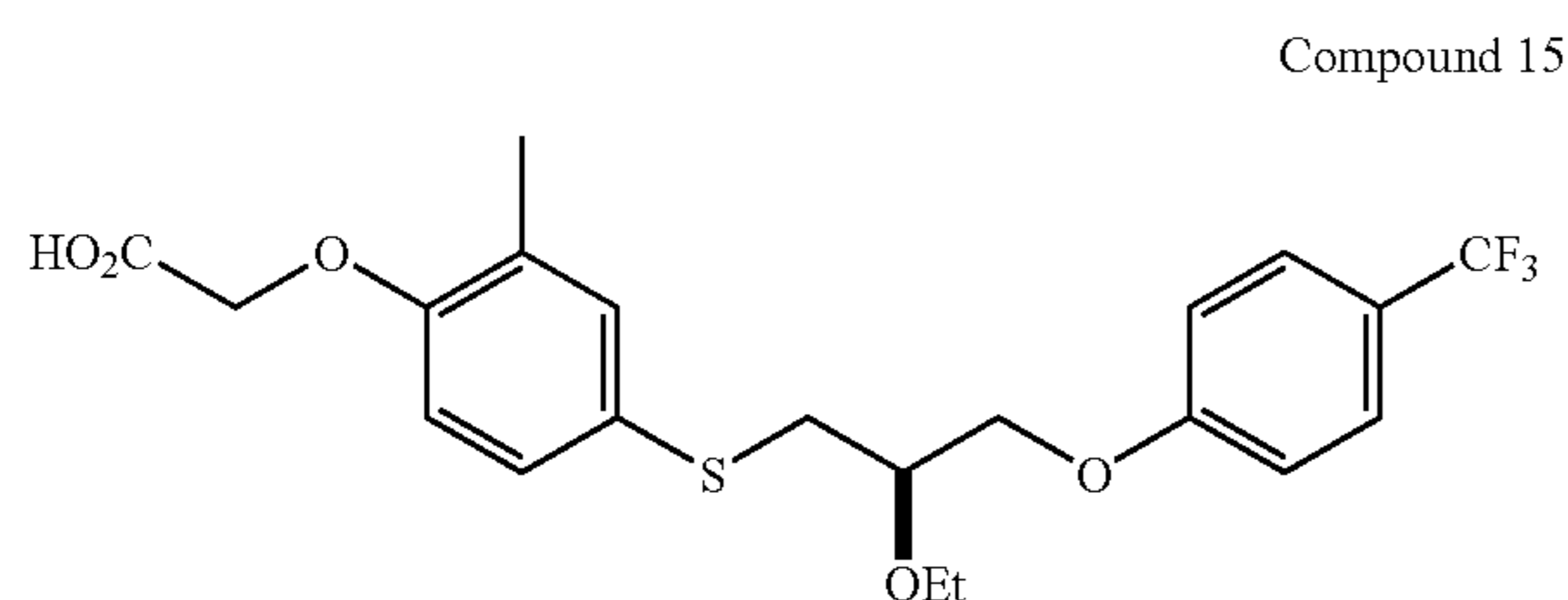
(R)-{4-[2-Ethoxy-3-(4-trifluoromethyl-phenoxy)-propylsulfanyl]-2-methyl-phenoxy}-acetic Acid
