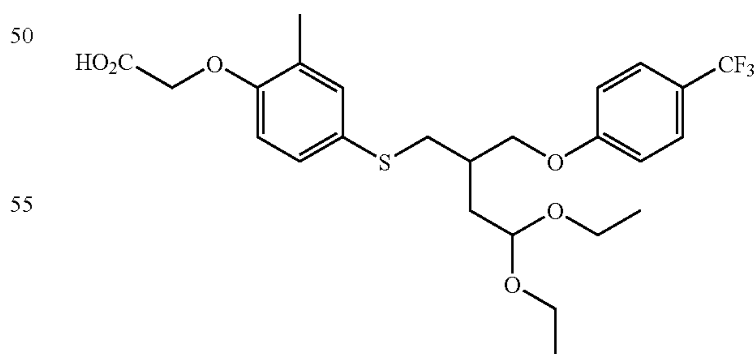
{4-[4,4-Diethoxy-2-(4-trifluoromethyl-phenoxyethyl)-butylsulfanyl]-2-methyl-phenoxy}-acetic Acid
