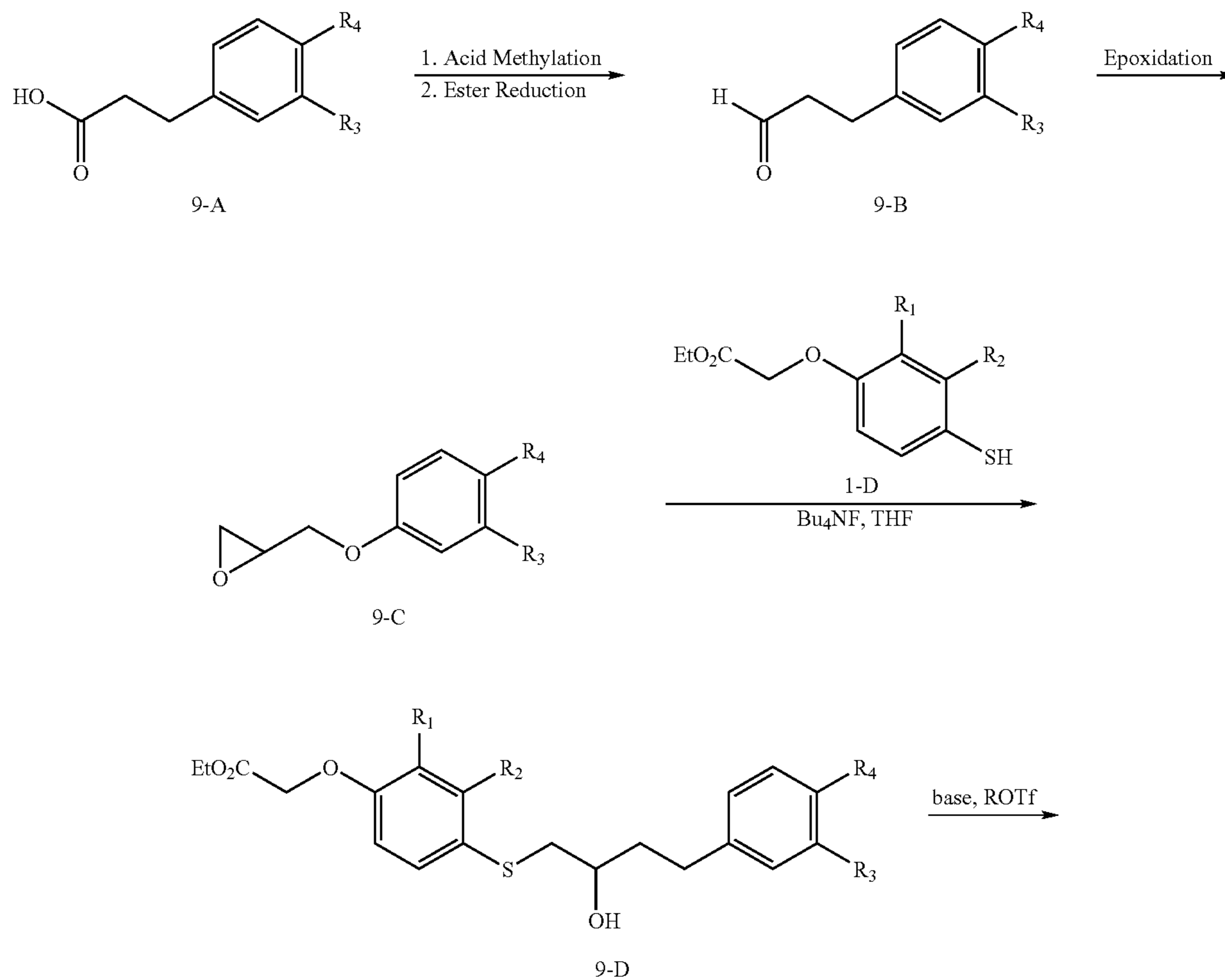
Scheme 8. Synthesis of Compound 1b1
