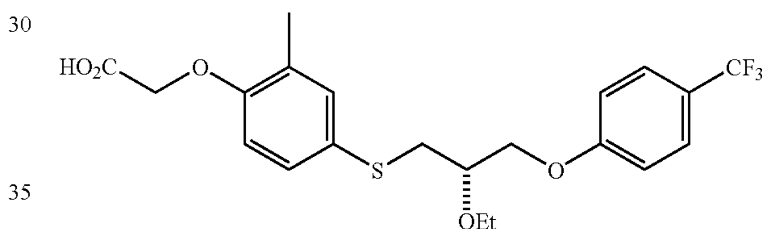
(S)-{4-[2-Ethoxy-3-(4-trifluoromethyl-phenoxy)-propylsulfanyl]-2-methyl-phenoxy}-acetic Acid
