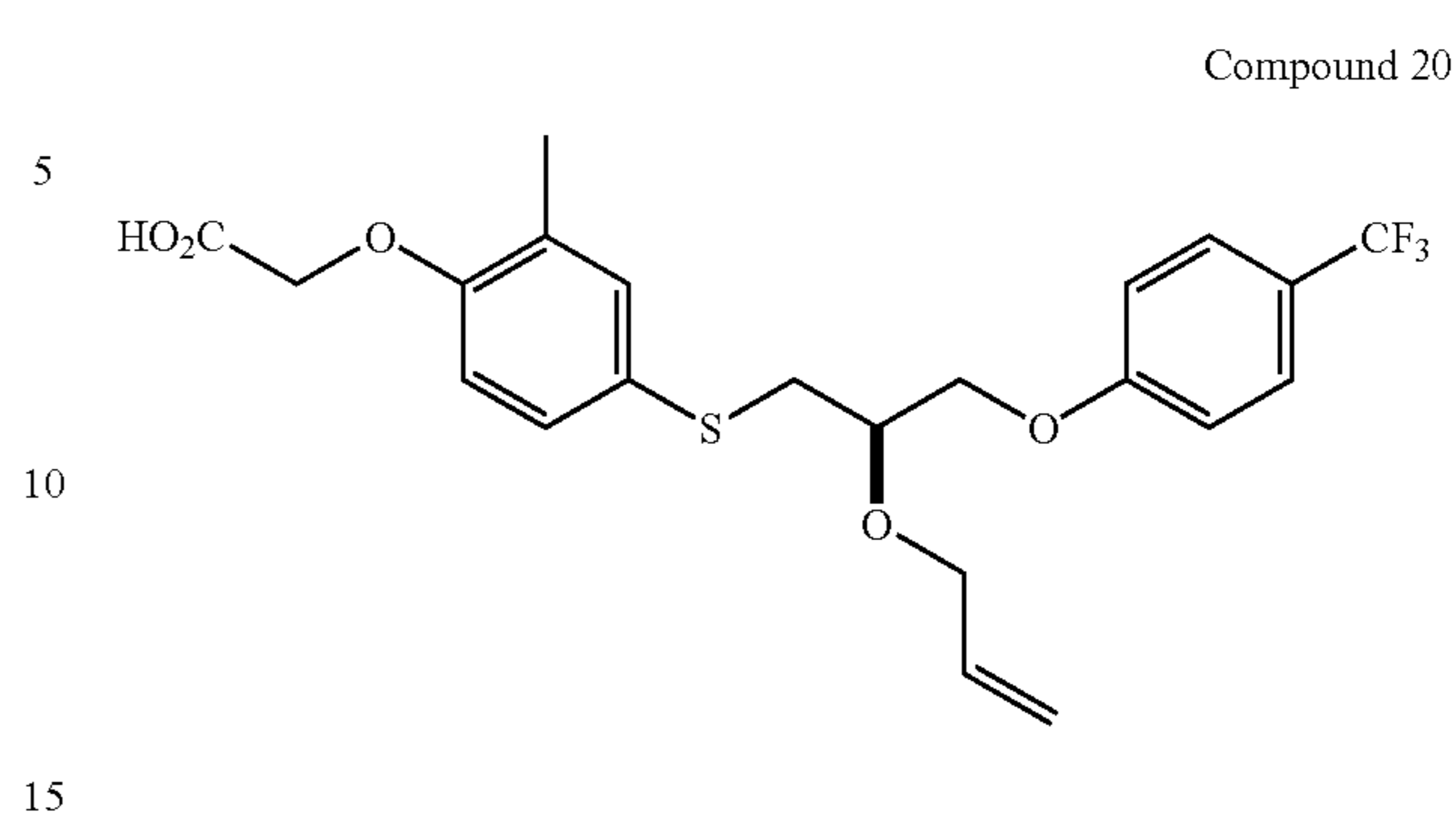
(R)-{4-[2-Allyloxy-3-(4-trifluoromethyl-phenoxy)-propylsulfanyl]-2-methyl-phenoxy}acetic Acid
