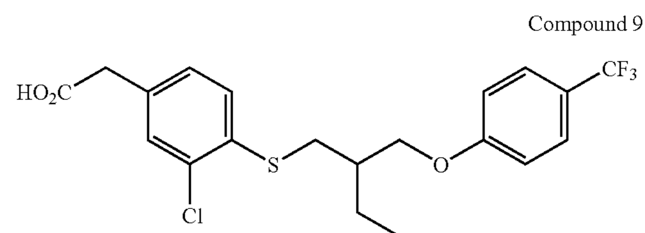
{3-Chloro-4-[2-(4-trifluoromethyl-phenoxy)ethyl]-butylsulfanyl]-phenyl}-acetic Acid
