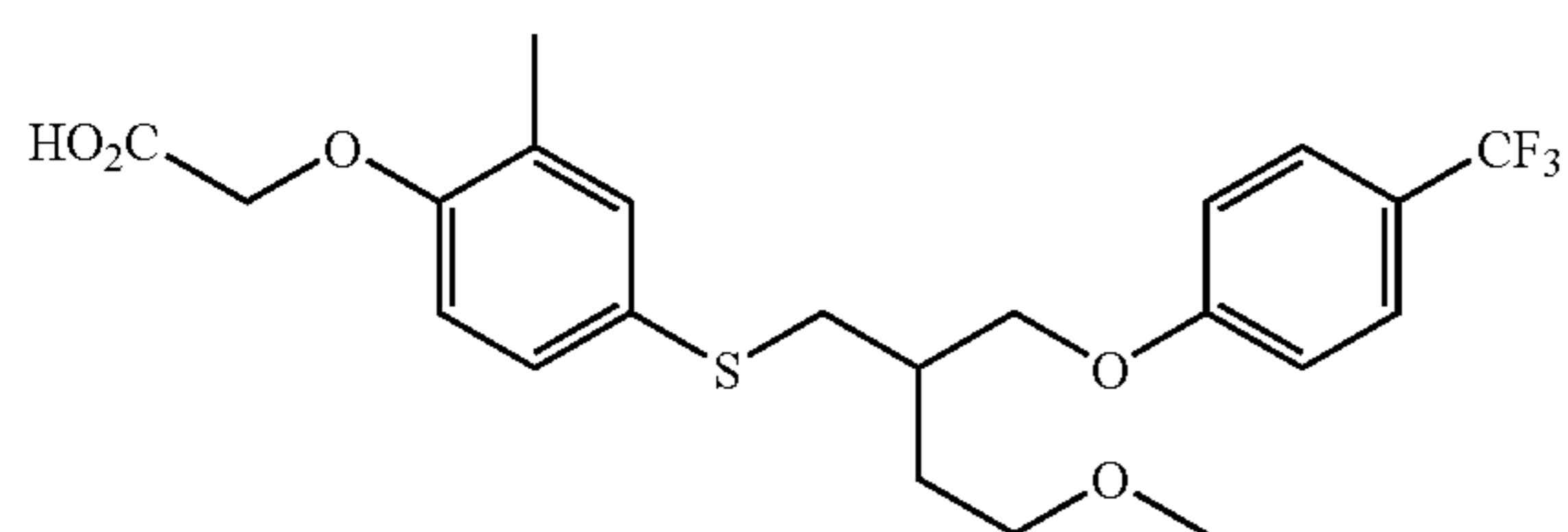
{4-[4-Methoxy-2-(4-trifluoromethyl-phenoxyethyl)-butylsulfanyl]-2-methyl-phenoxy}-acetic Acid
