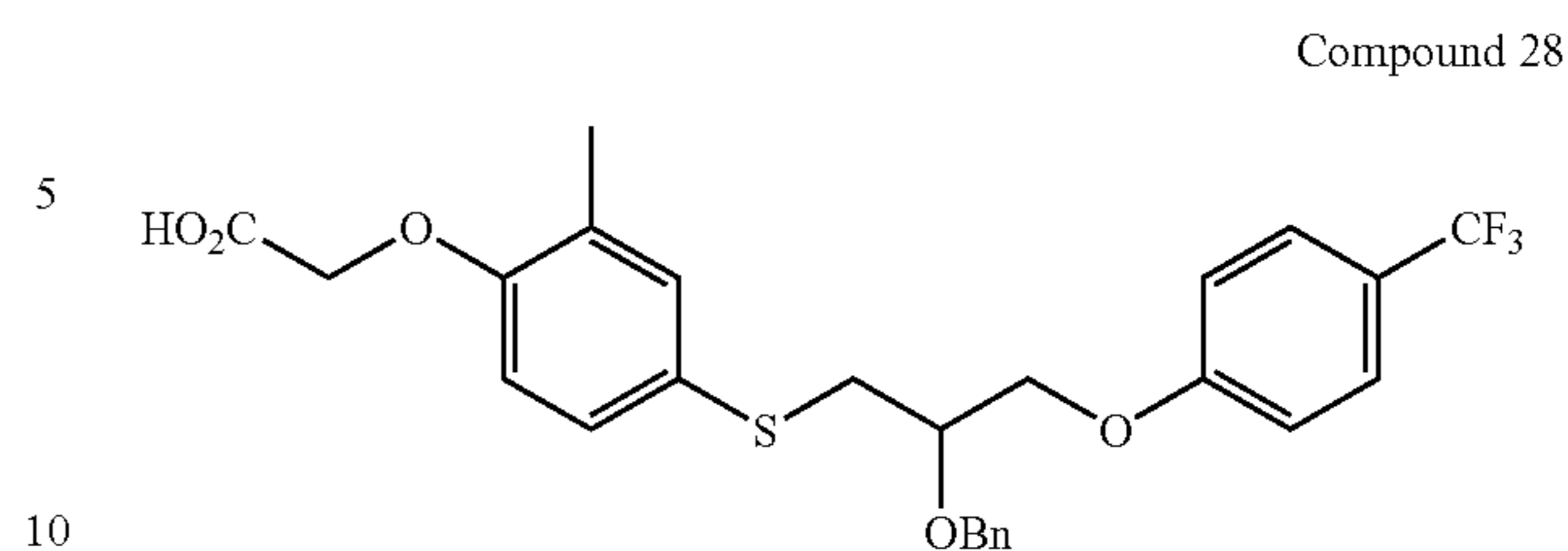
{4-[2-Benzyloxy-3-(4-trifluoromethyl-phenoxy)-propylsulfanyl]-2-methyl-phenoxy}-acetic Acid
