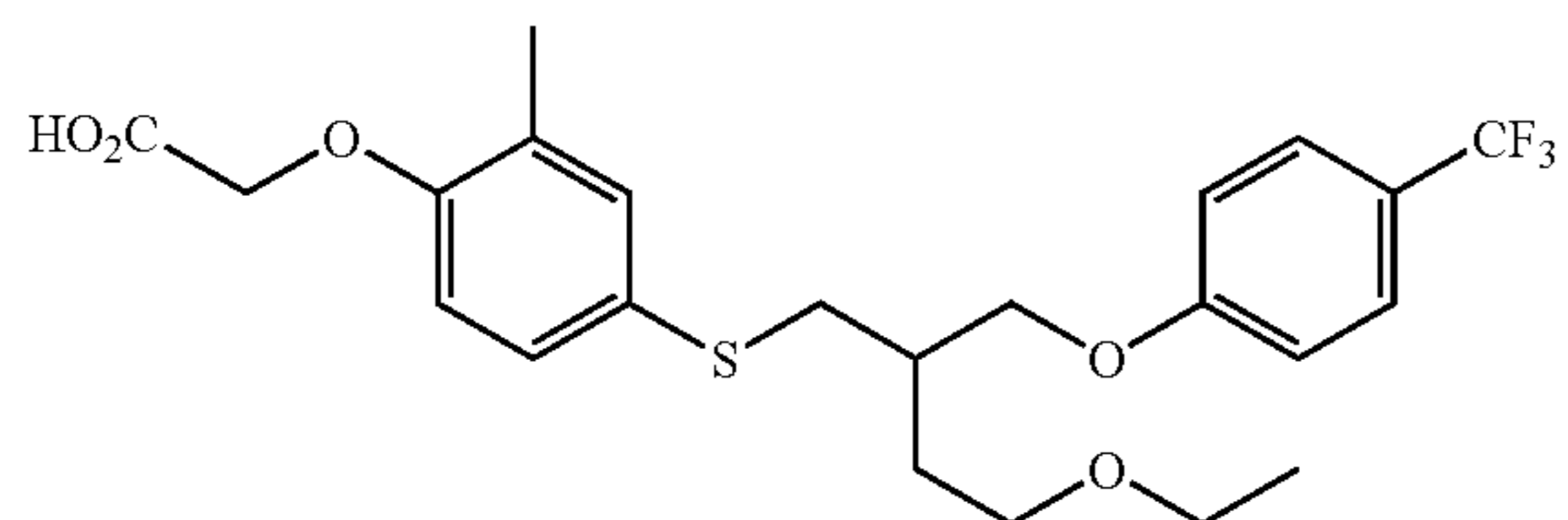
{4-[4-Ethoxy-2-(4-trifluoromethyl-phenoxy)-butylsulfanyl]-2-methyl-phenoxy}-acetic Acid
