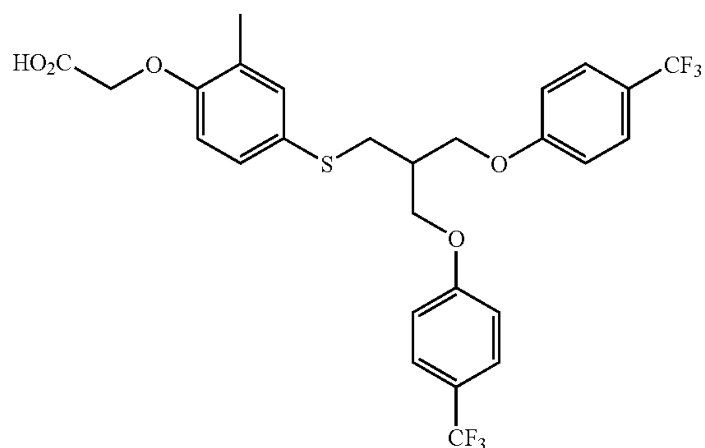
{2-Methyl-4-[3-(4-trifluoromethyl-phenoxy)-2-(4-trifluoromethyl-phenoxyethyl)-propylsulfanyl]-phenoxy}-acetic Acid
