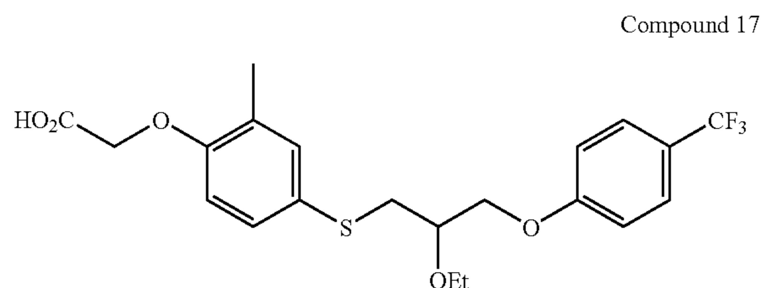
{4-[2-Ethoxy-3-(4-trifluoromethyl-phenoxy)-propylsulfanyl]-2-methyl-phenoxy}acetic Acid
