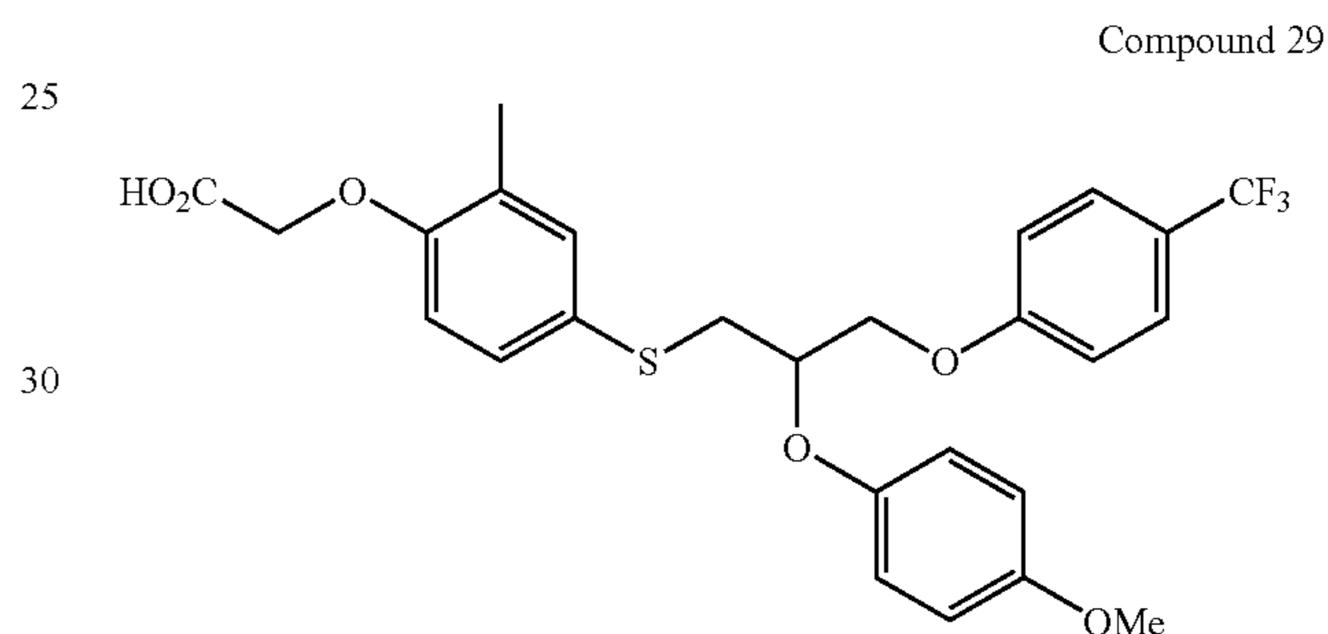
{4-[2-(4-Methoxy-phenoxy)-3-(4-trifluoromethyl-phenoxy)-propylsulfanyl]-2-methyl-phenoxy}-acetic Acid
