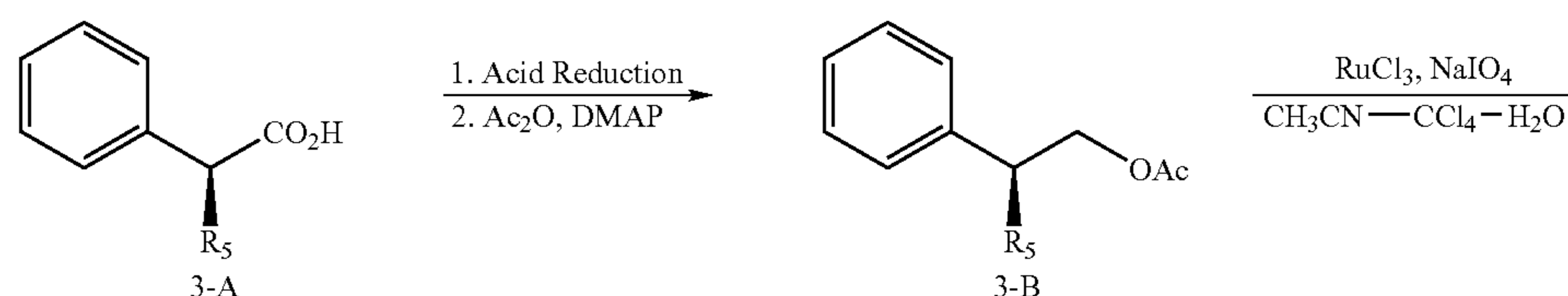
Scheme 3. Synthesis of Compound Ia1
