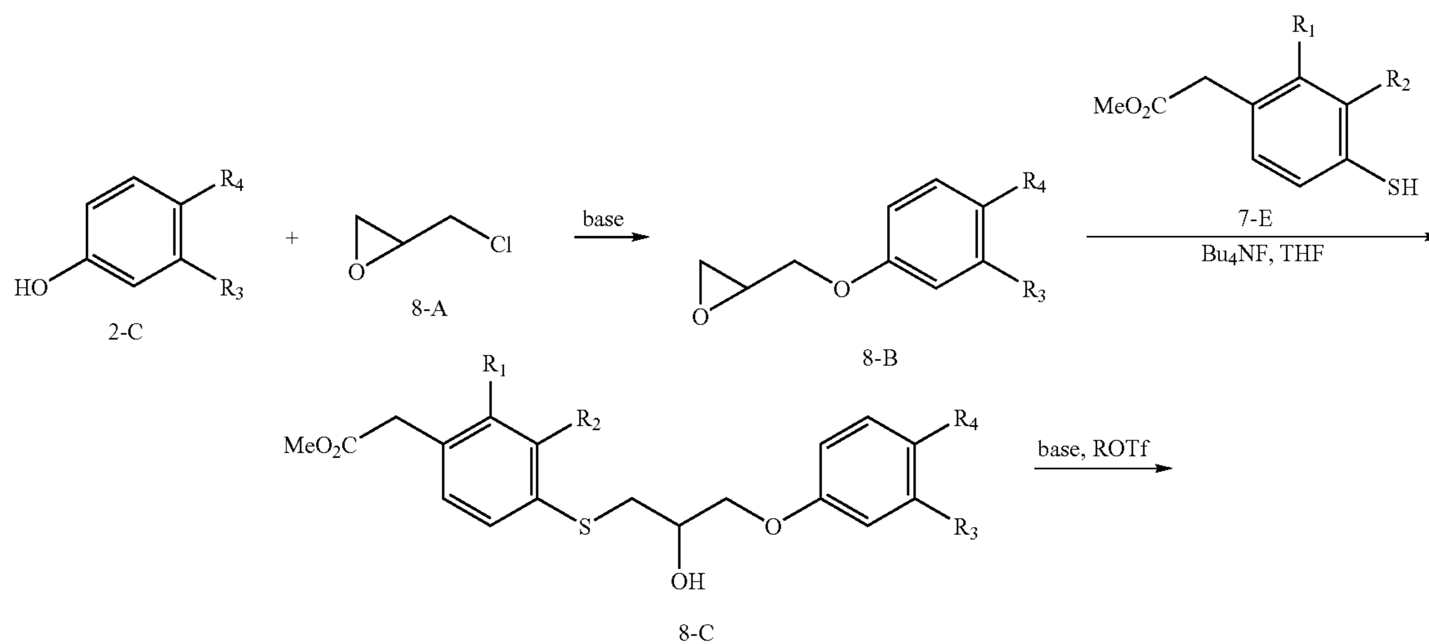
Scheme 8. Synthesis of Compound Ib1
