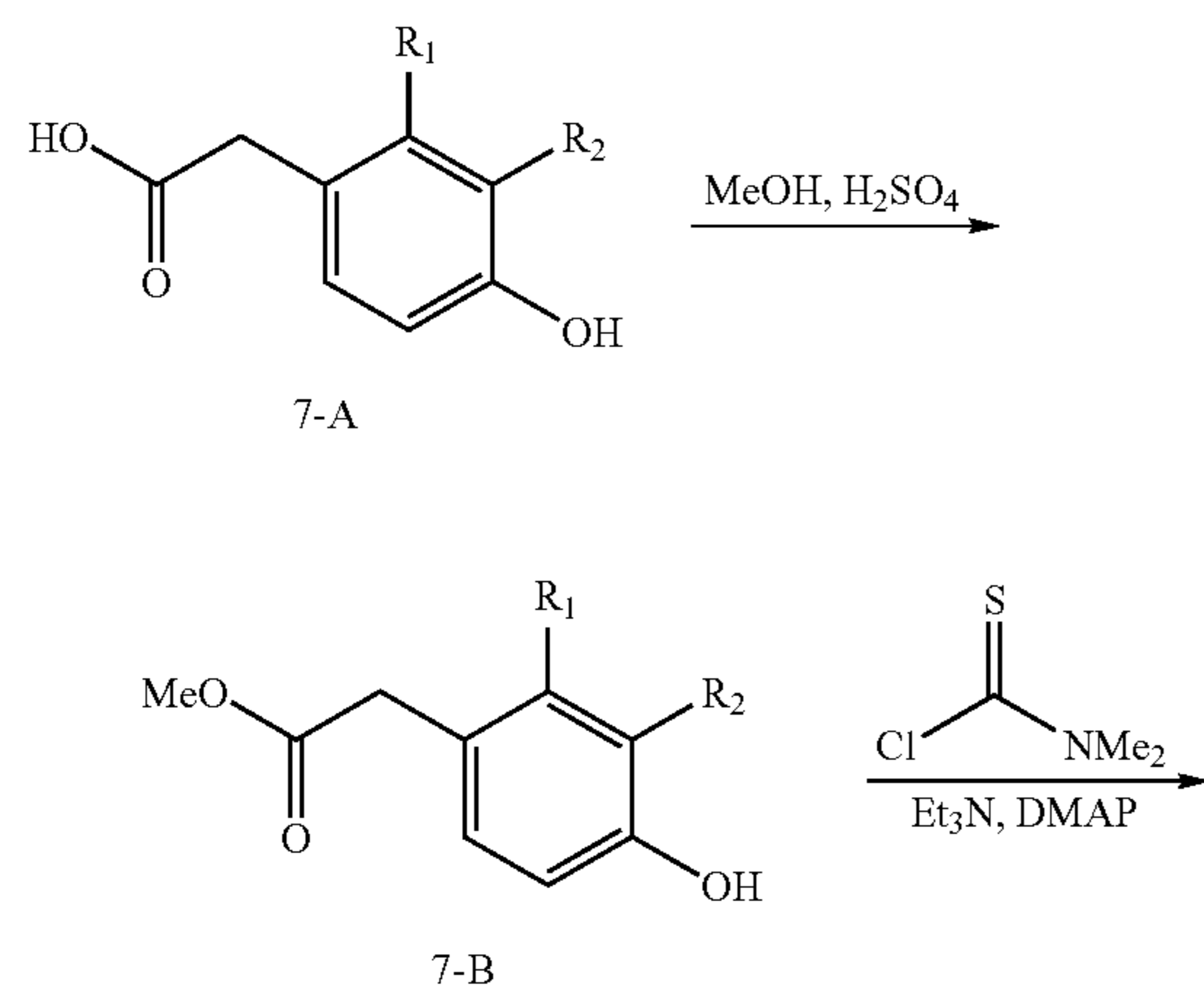
Scheme 7. Synthesis of Intermediate 7-E
