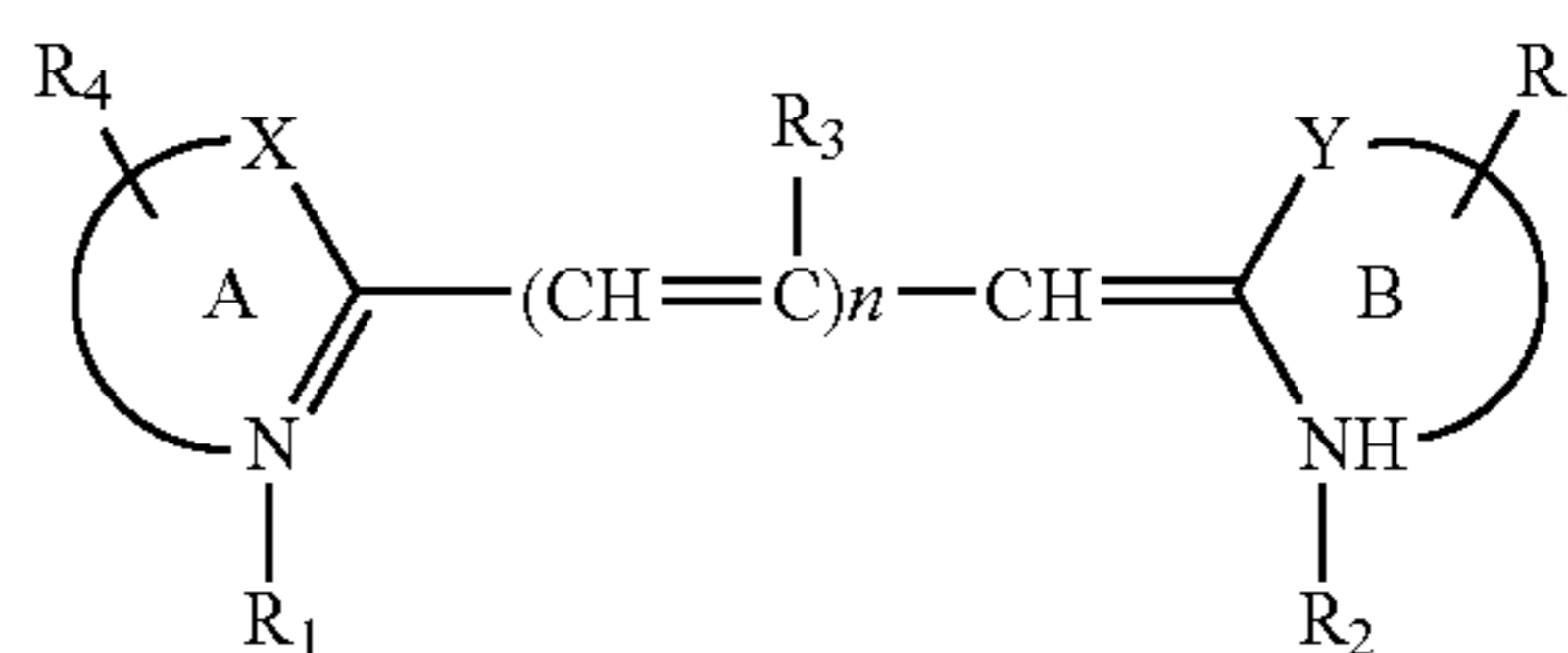
The Cyanine Chromophore.
