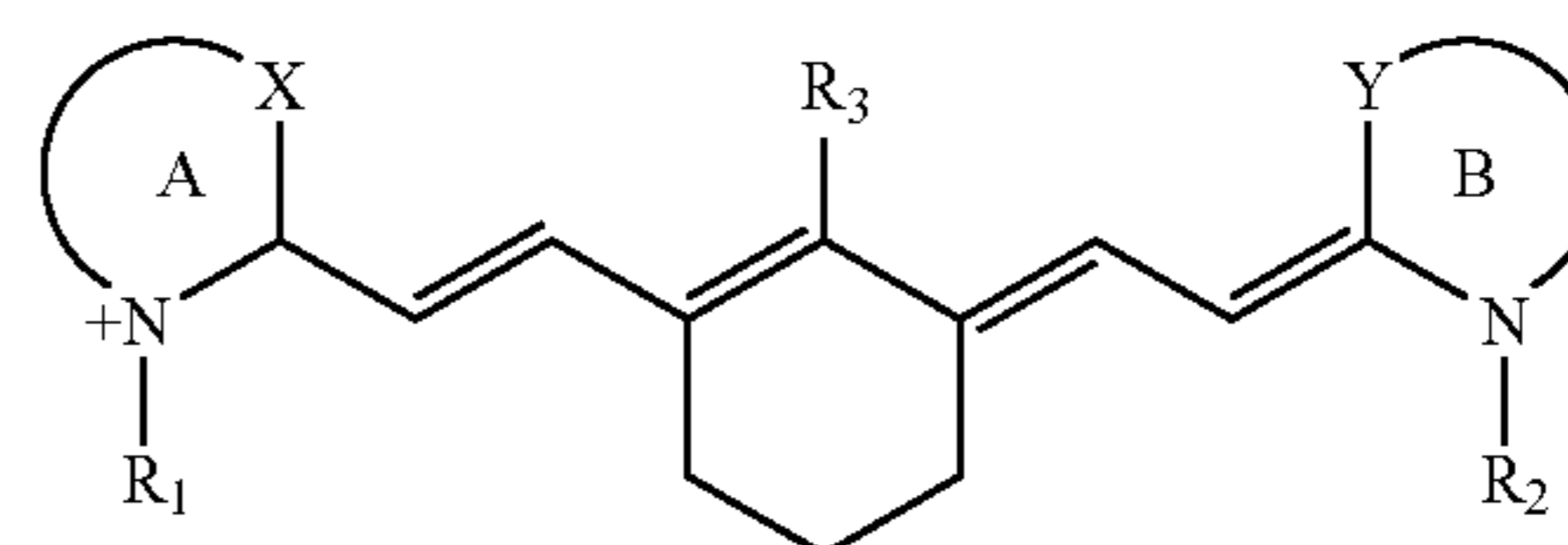
A Ring-locked Tricyanocyanine Chromophore.
