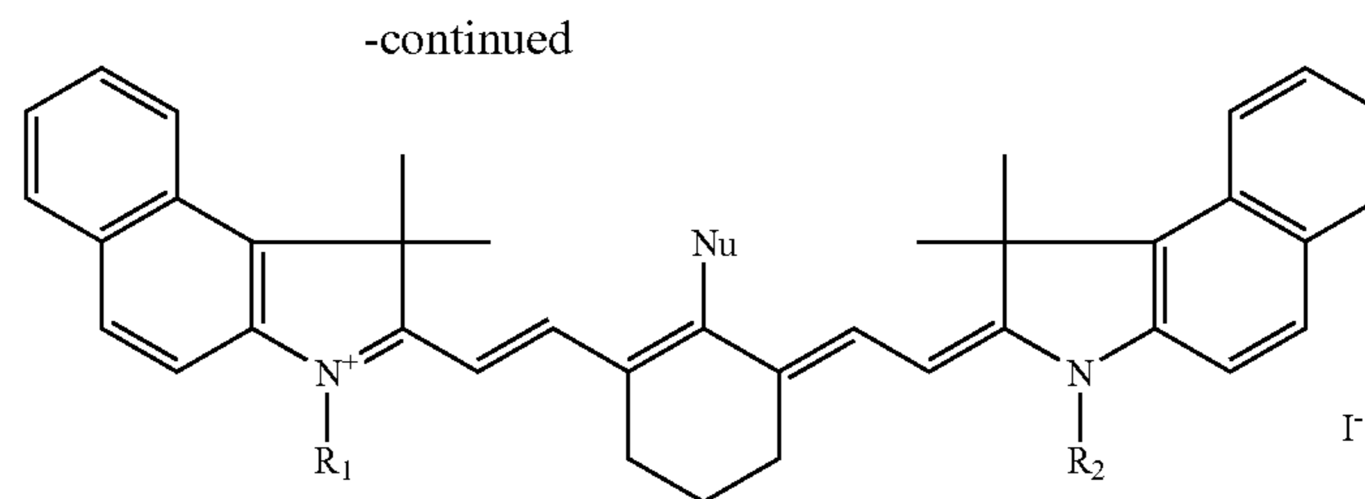
6, R_1 = R_2 = (\text{CH}_2)_2\text{CH}_3 , Nu = SPh
