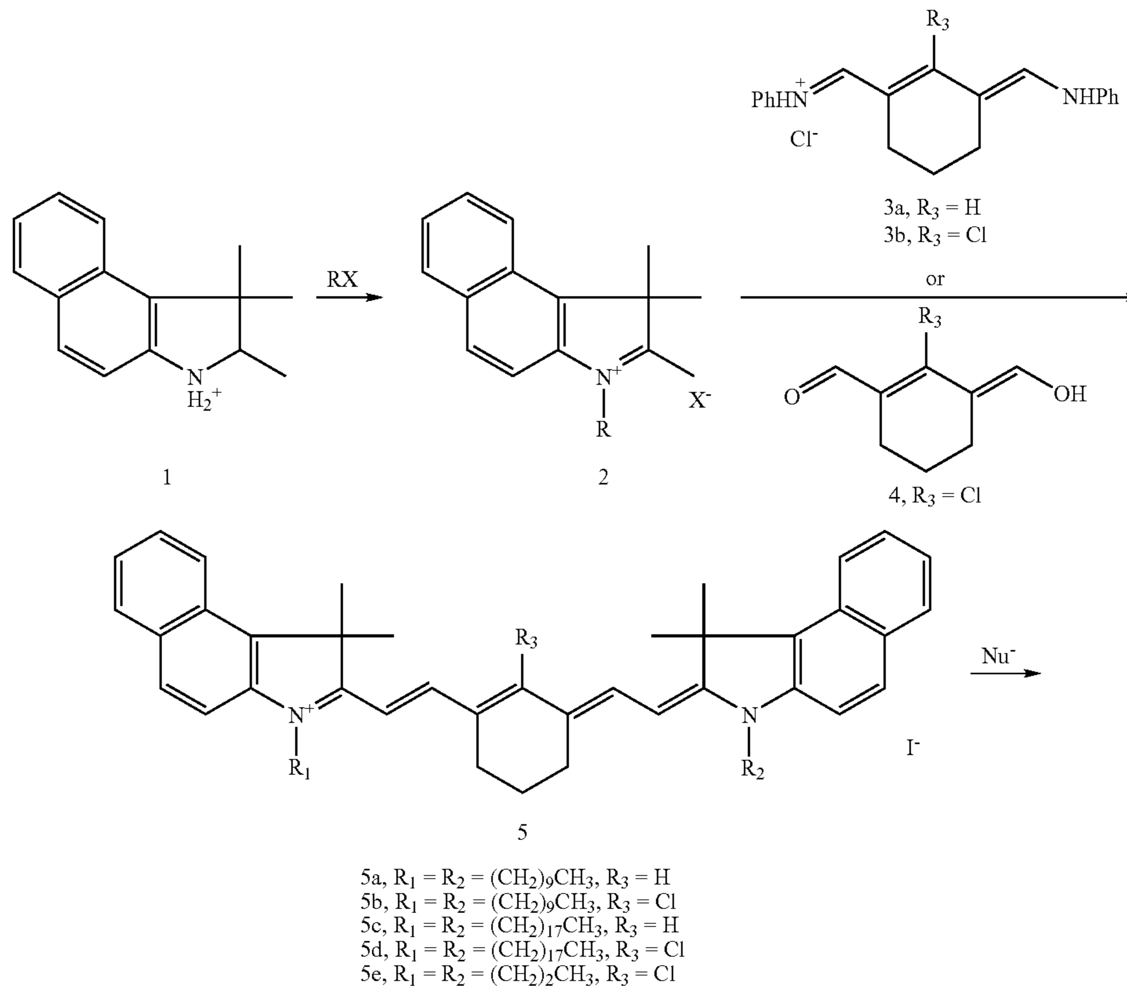
Scheme 1. Synthesis of Ring-locked Benzo-indotricarbocyanine Compounds.
