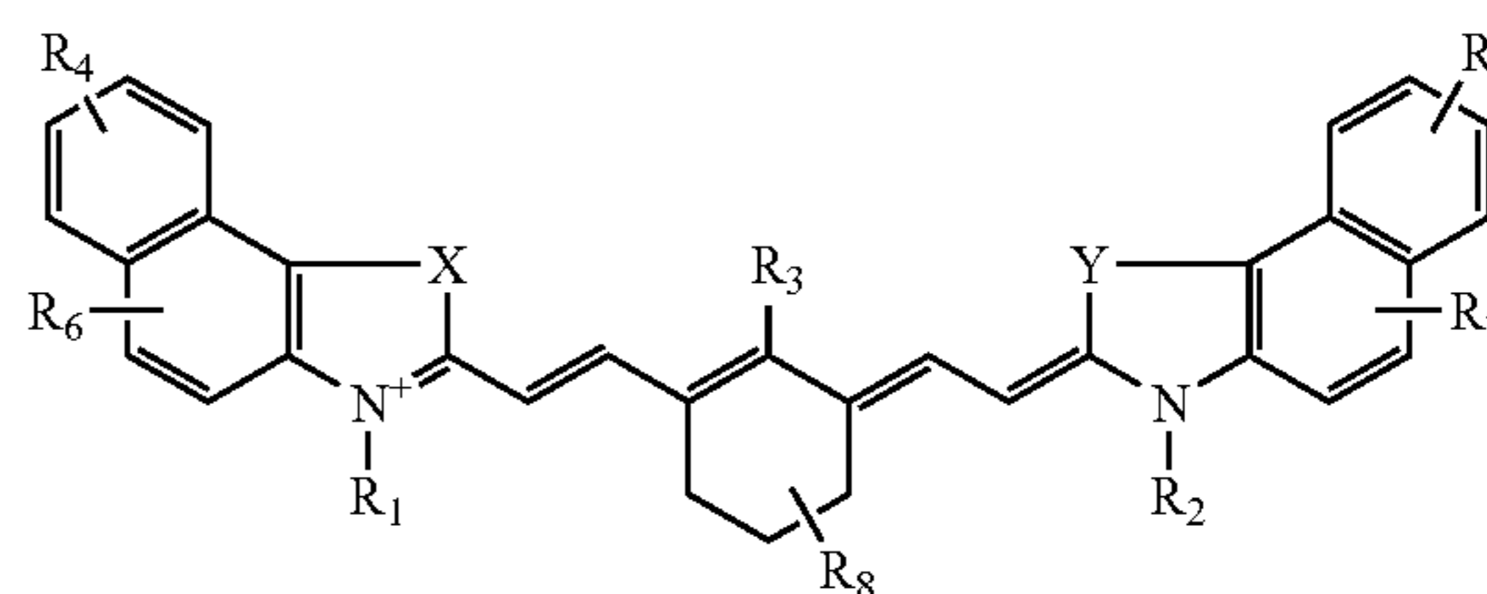
Ring-locked Benzo-indotricyanocyanine Compounds.
