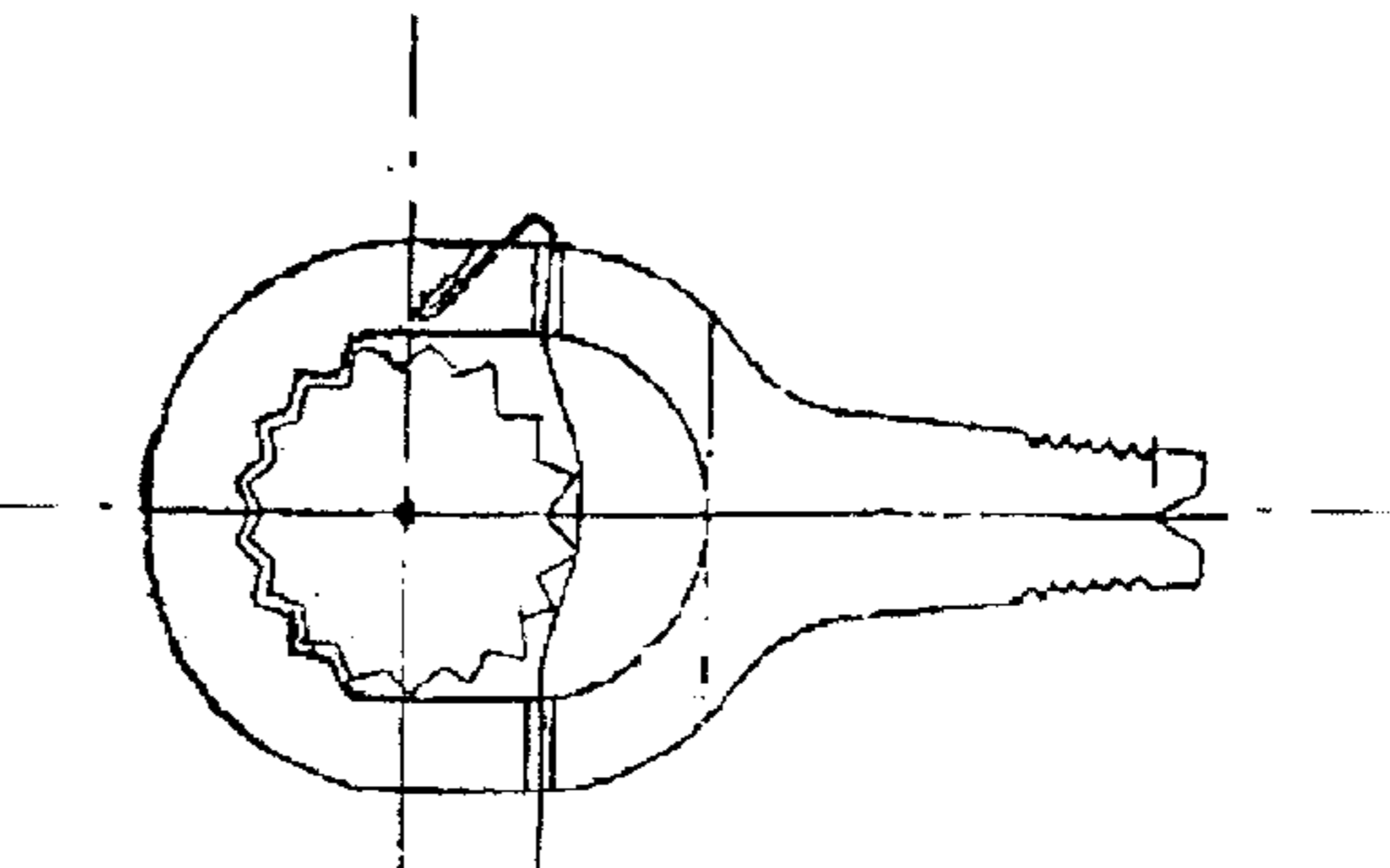
Fig. 5c Release handle to return to normal position, gas valve disk and handle are engaged
