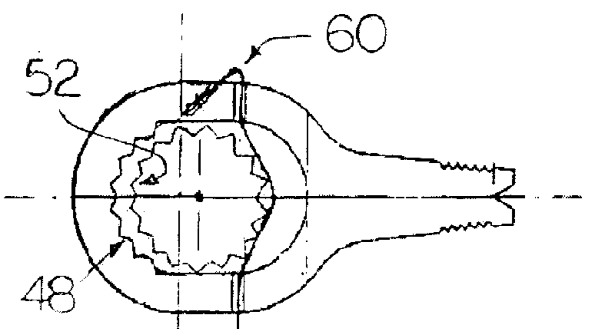
Fig. 5b Valve handle is pressed to disengage gas valve disk
