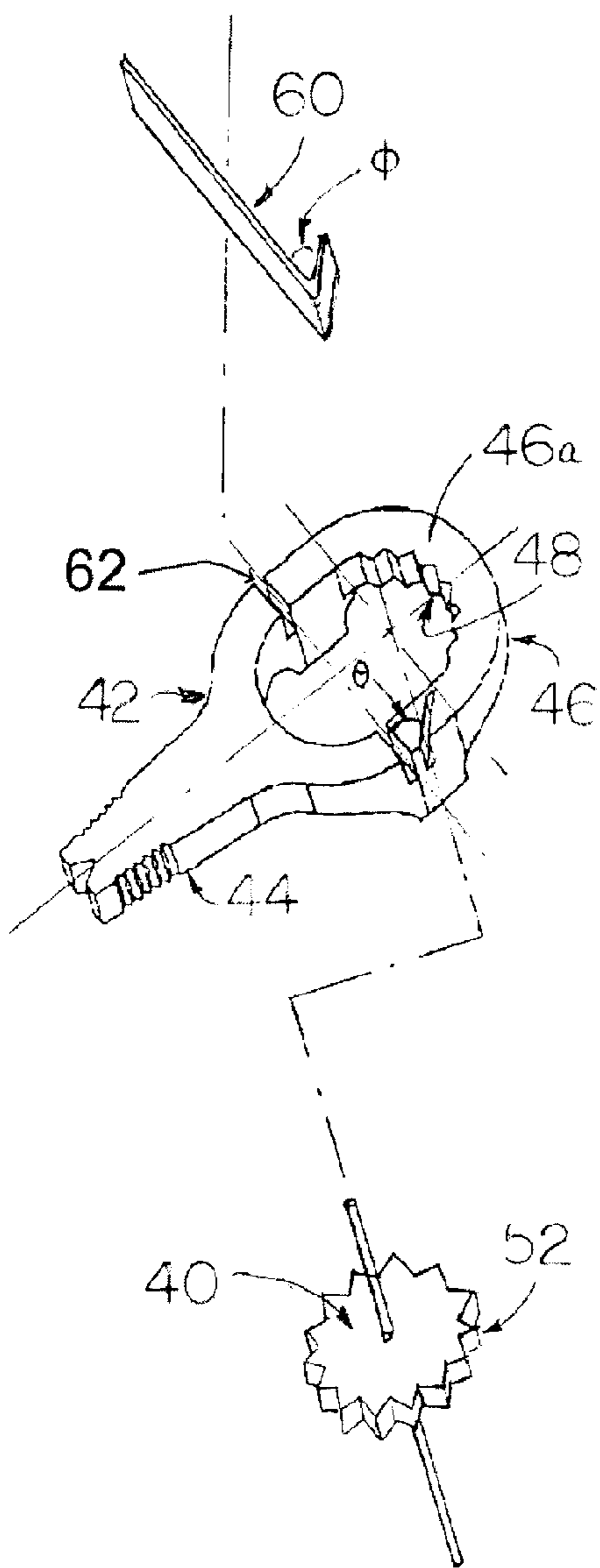
Fig. 4 Valve Handle Assembly
