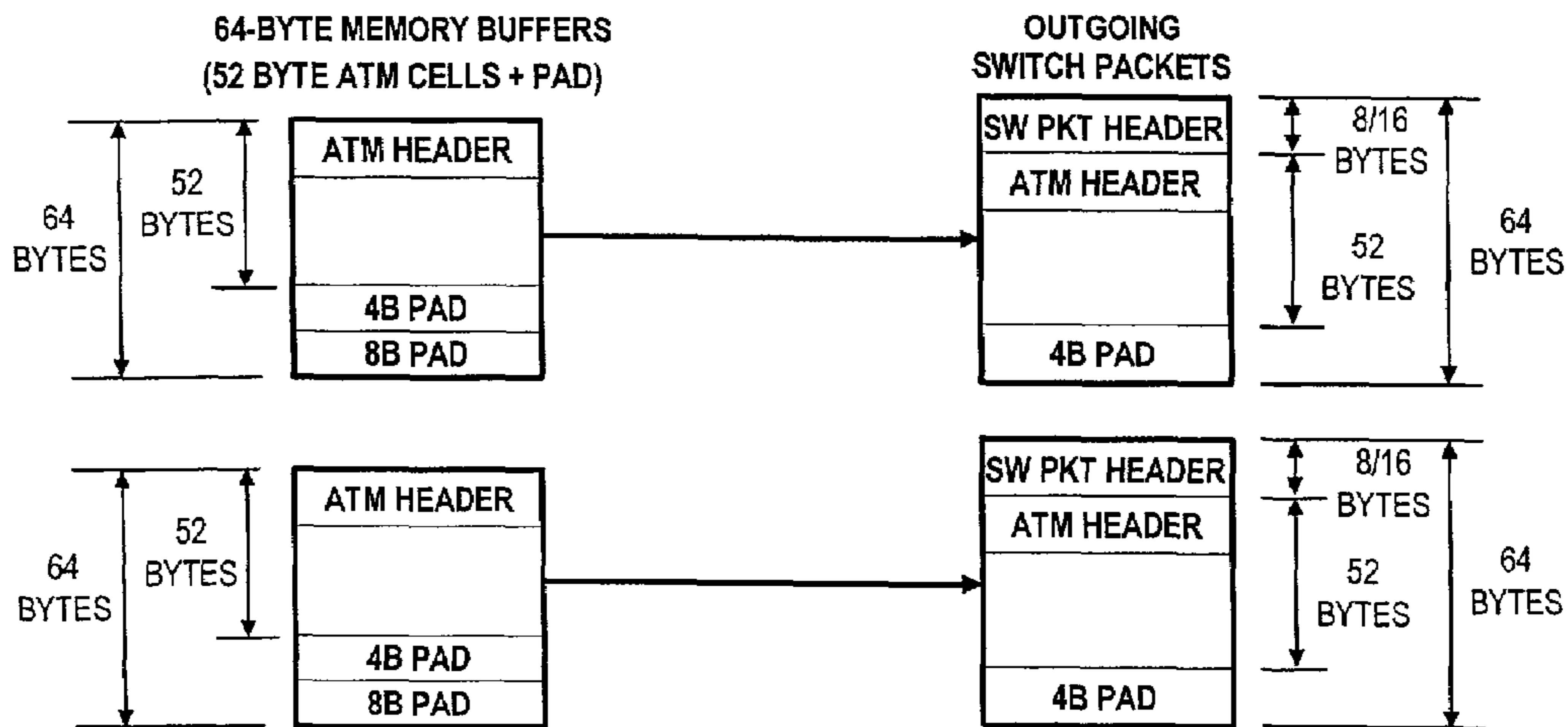
REASSEMBLY TYPE 2 (INGRESS APPLICATION TYPE 4)
