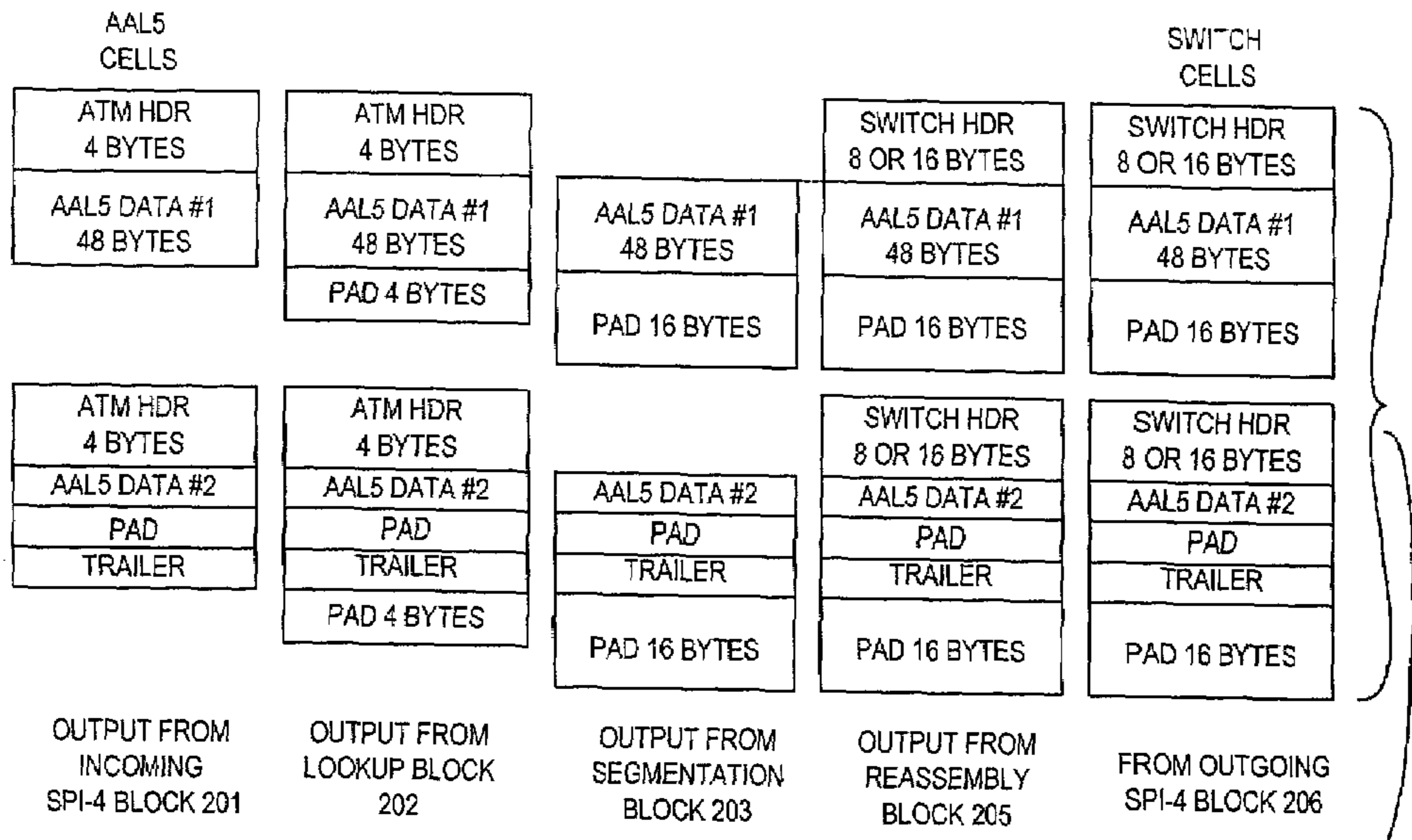
INGRESS APPLICATION TYPE 1
