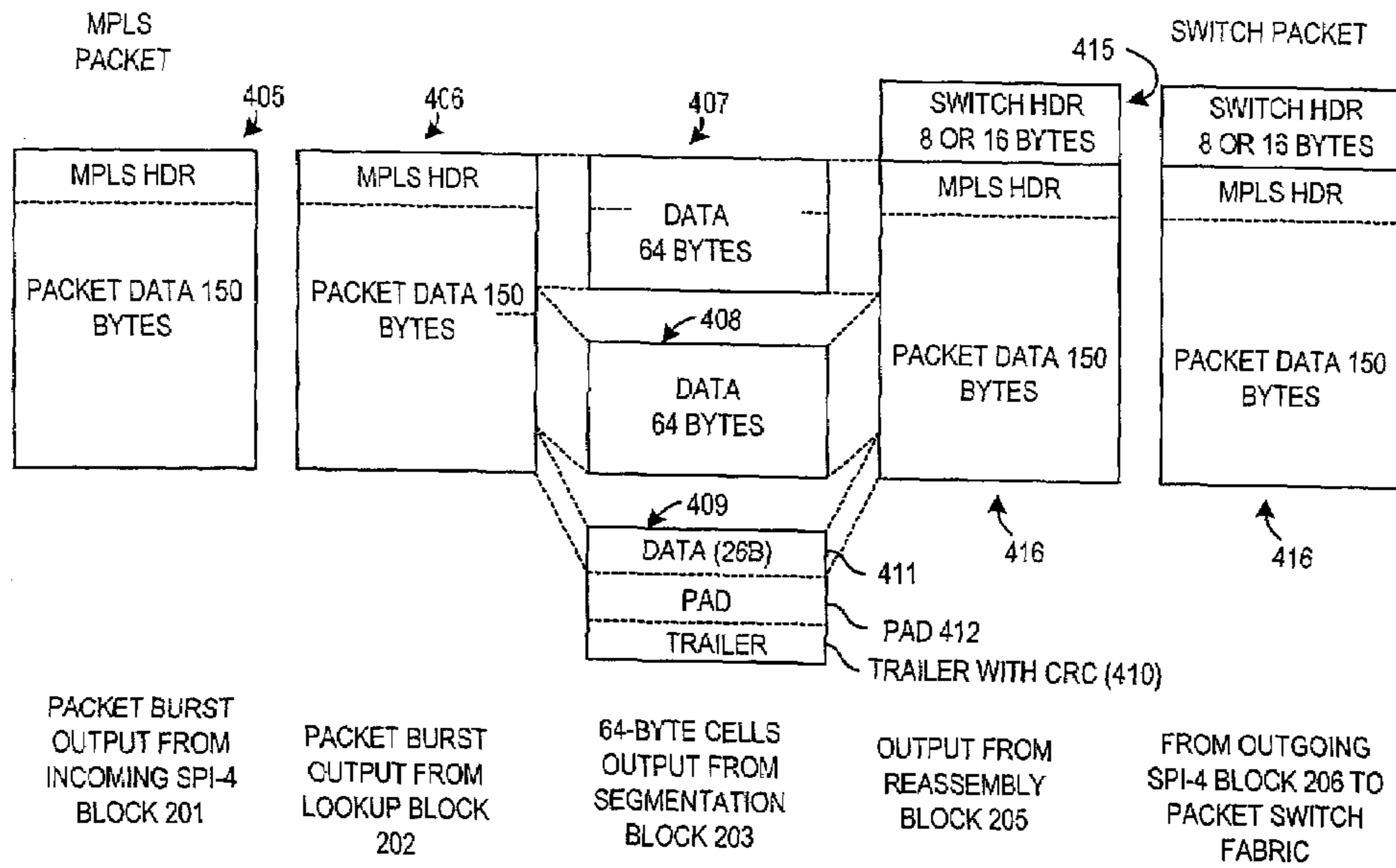
FLOW #2 INGRESS APPLICATION TYPE 6 FIG. 40
