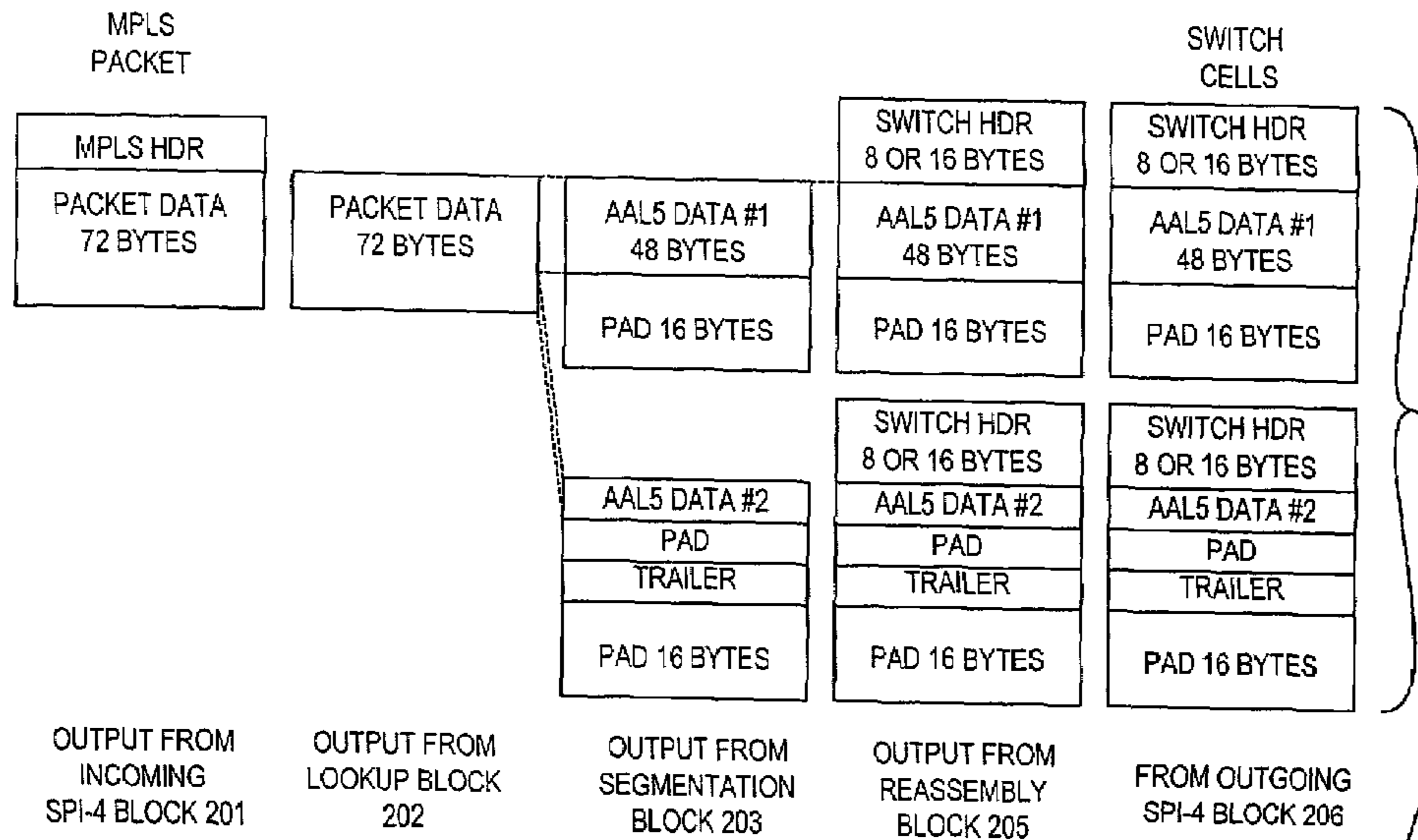
INGRESS APPLICATION TYPE 2
