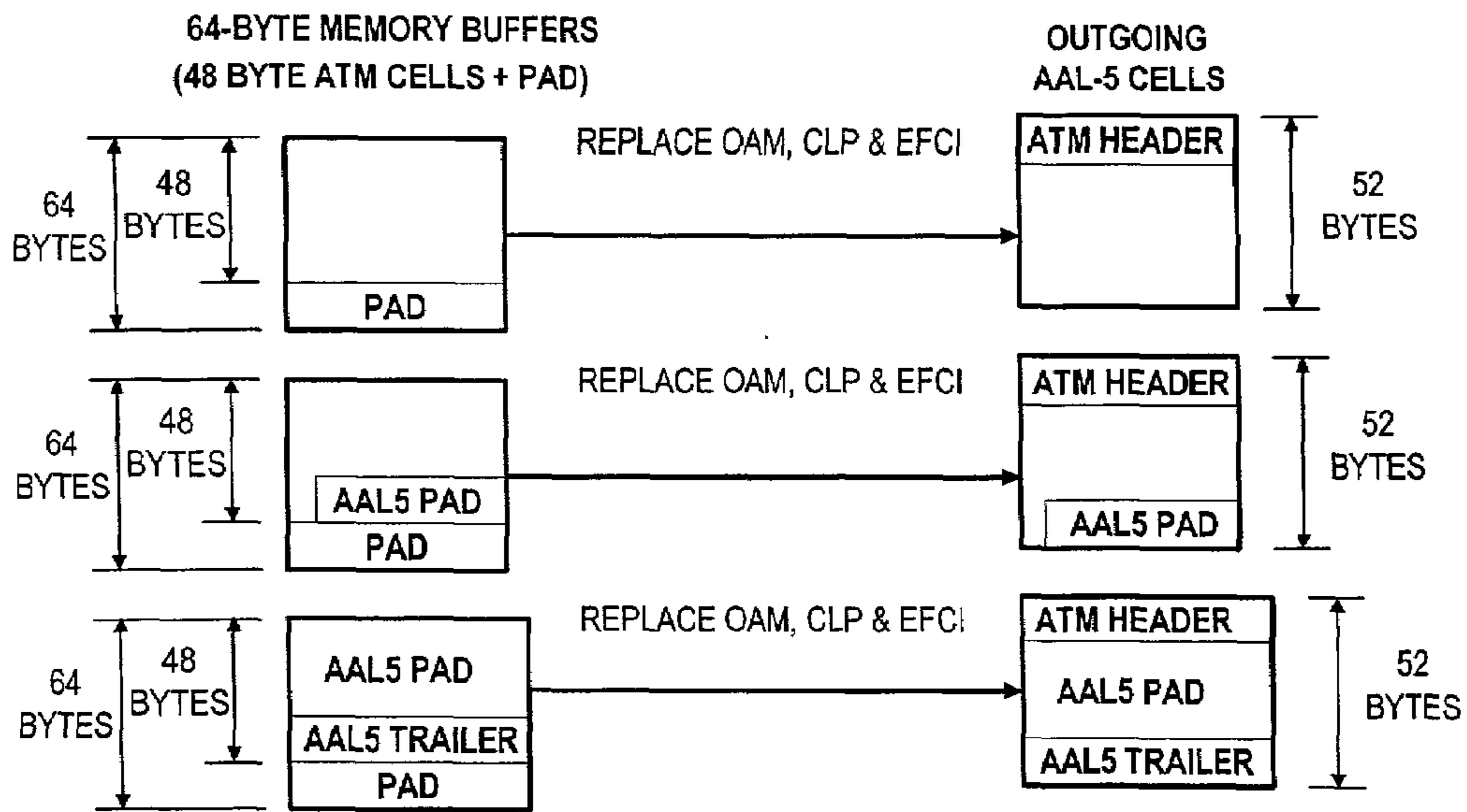
REASSEMBLY TYPE 7 (INGRESS APPLICATION TYPES 10 AND 13)
