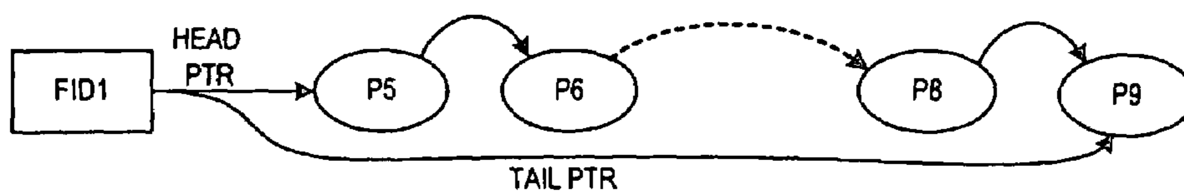
PACKET QUEUE
