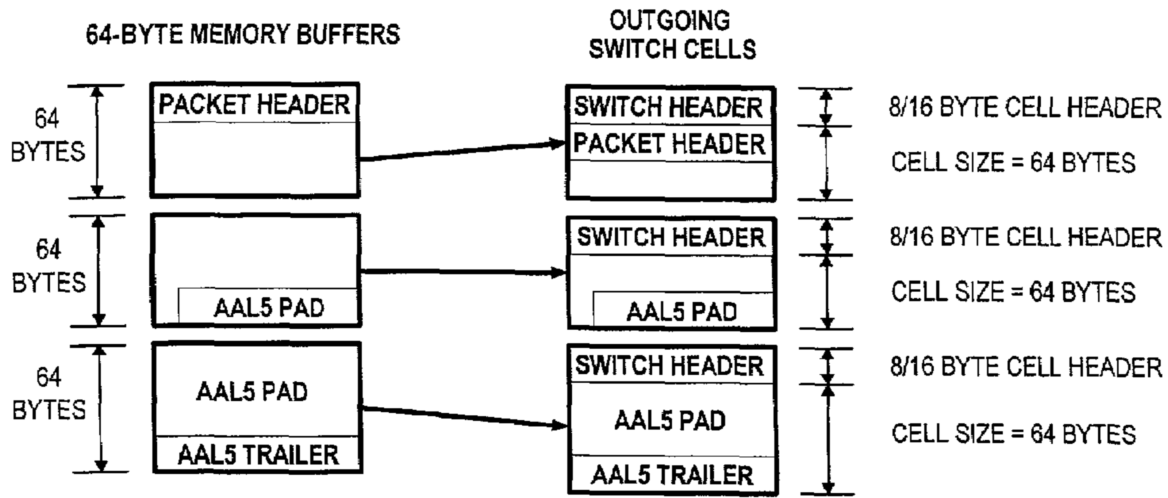
REASSEMBLY TYPE 1 (INGRESS APPLICATION TYPE 3)
