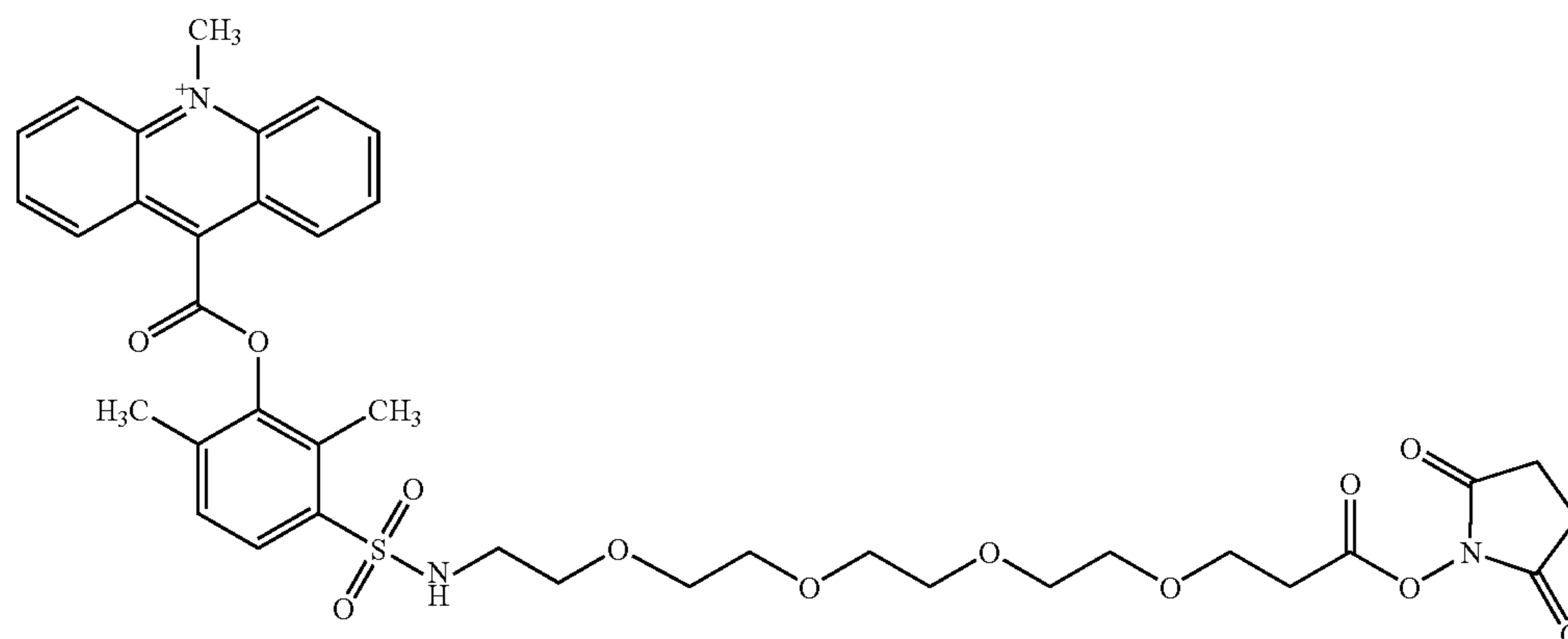
MeAE-PEO4-NHS
