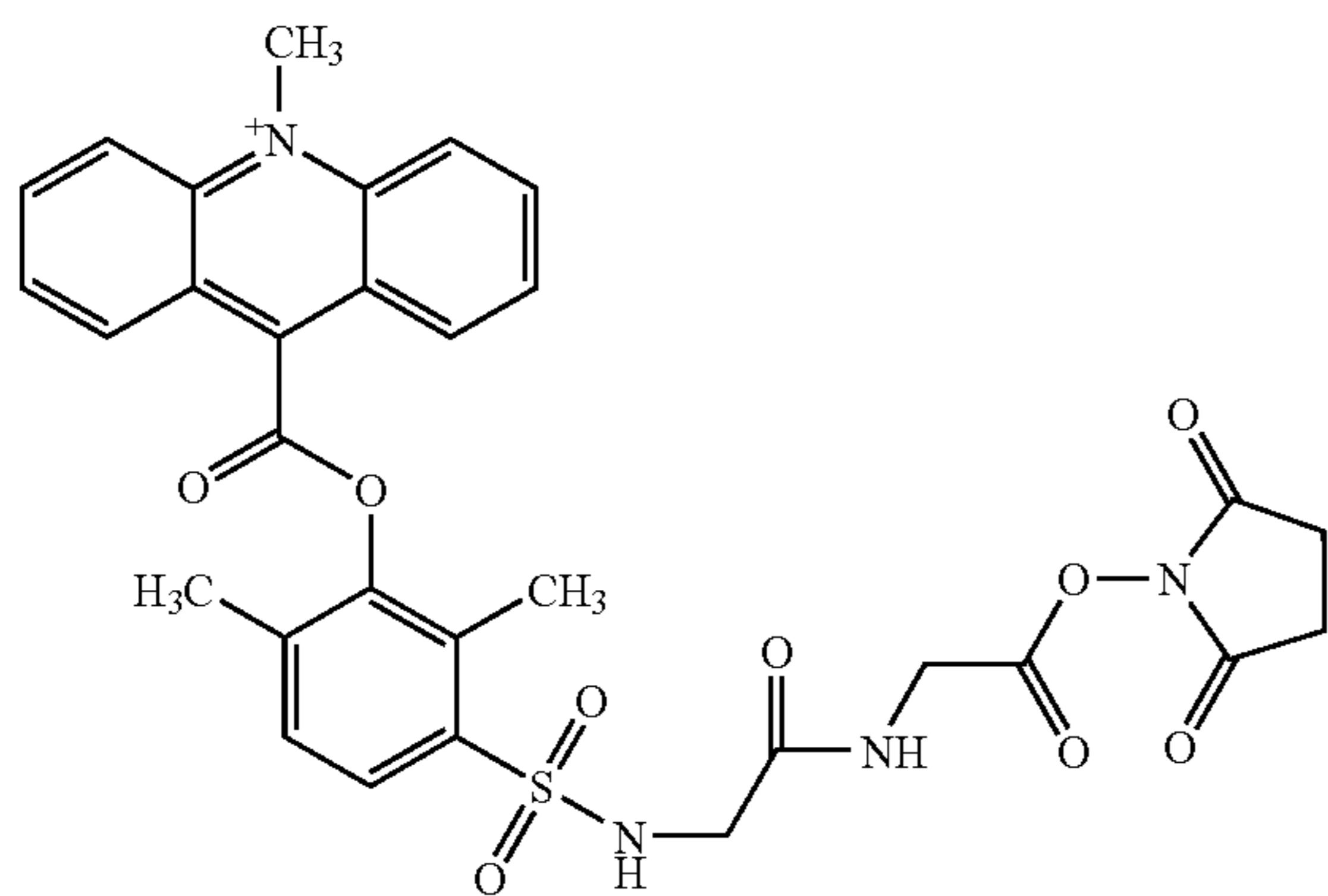
MeAE-Gly2-NHS
