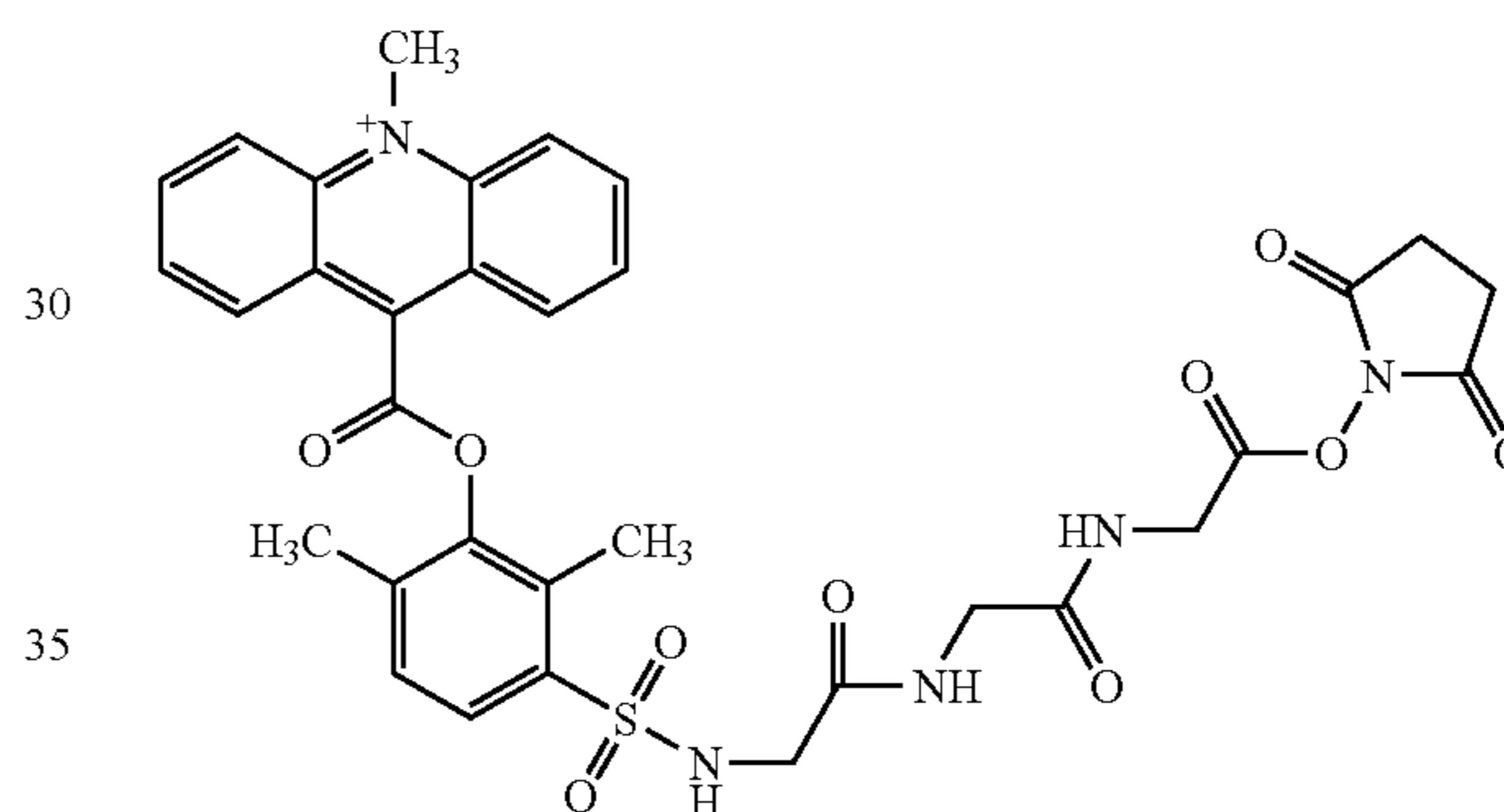
MeAE-Gly3-NHS
