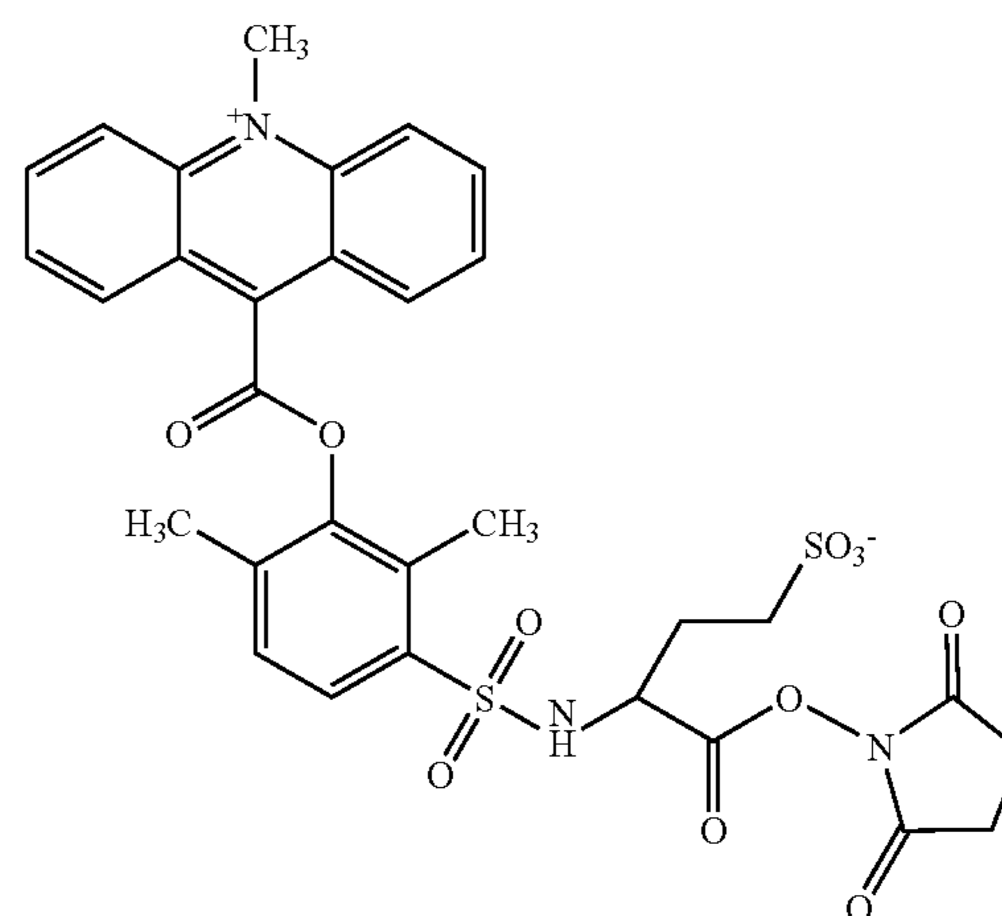
MeAE-HCA-NHS
