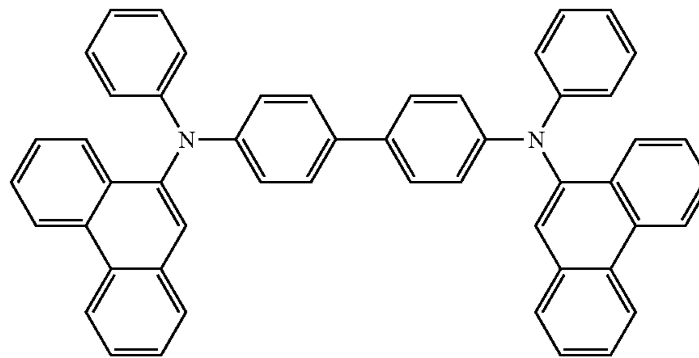
Chemical Formula 3
