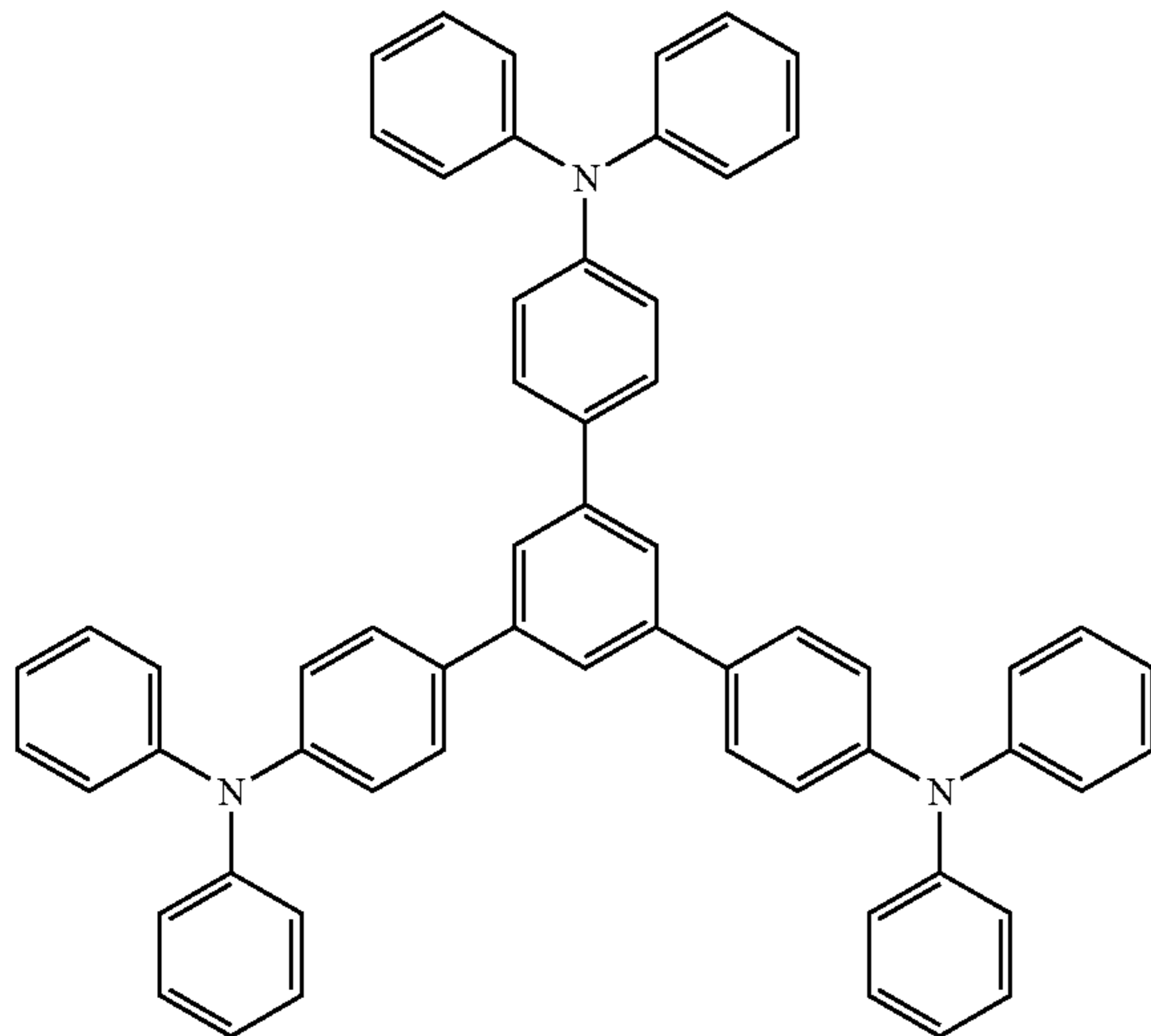
Chemical Formula 7
