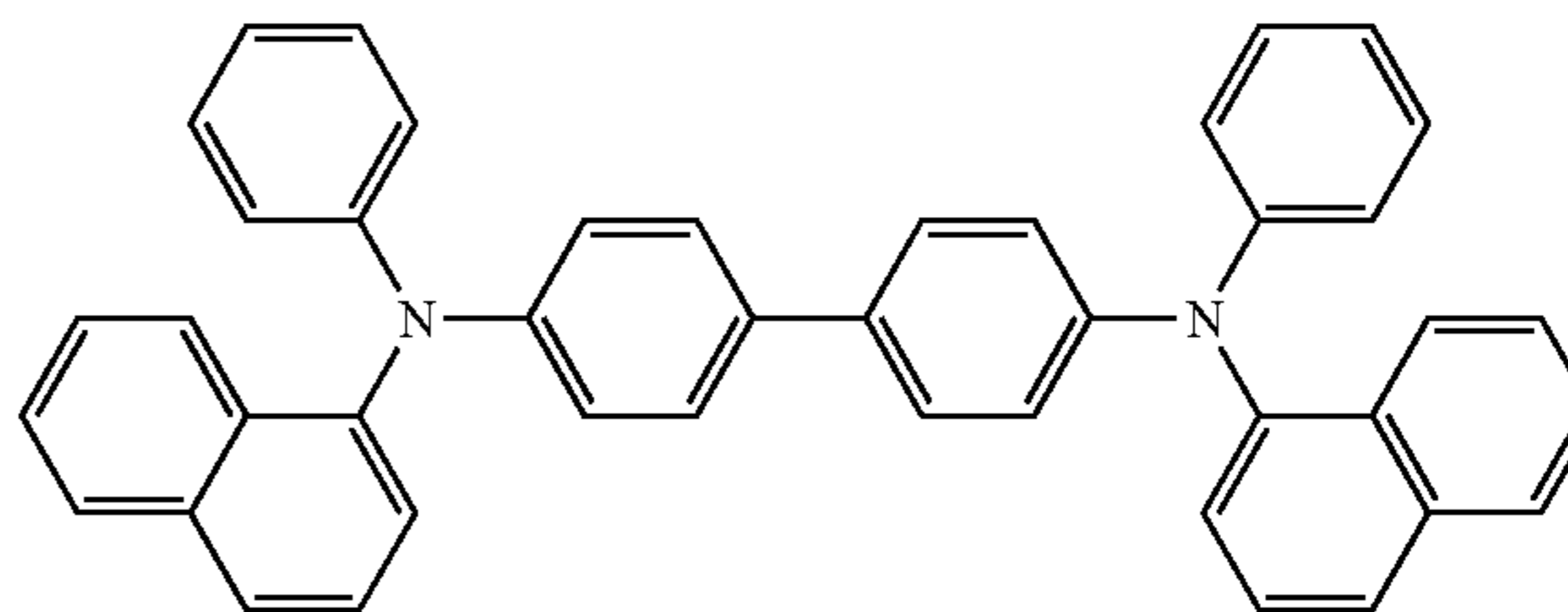
Chemical Formula 4
