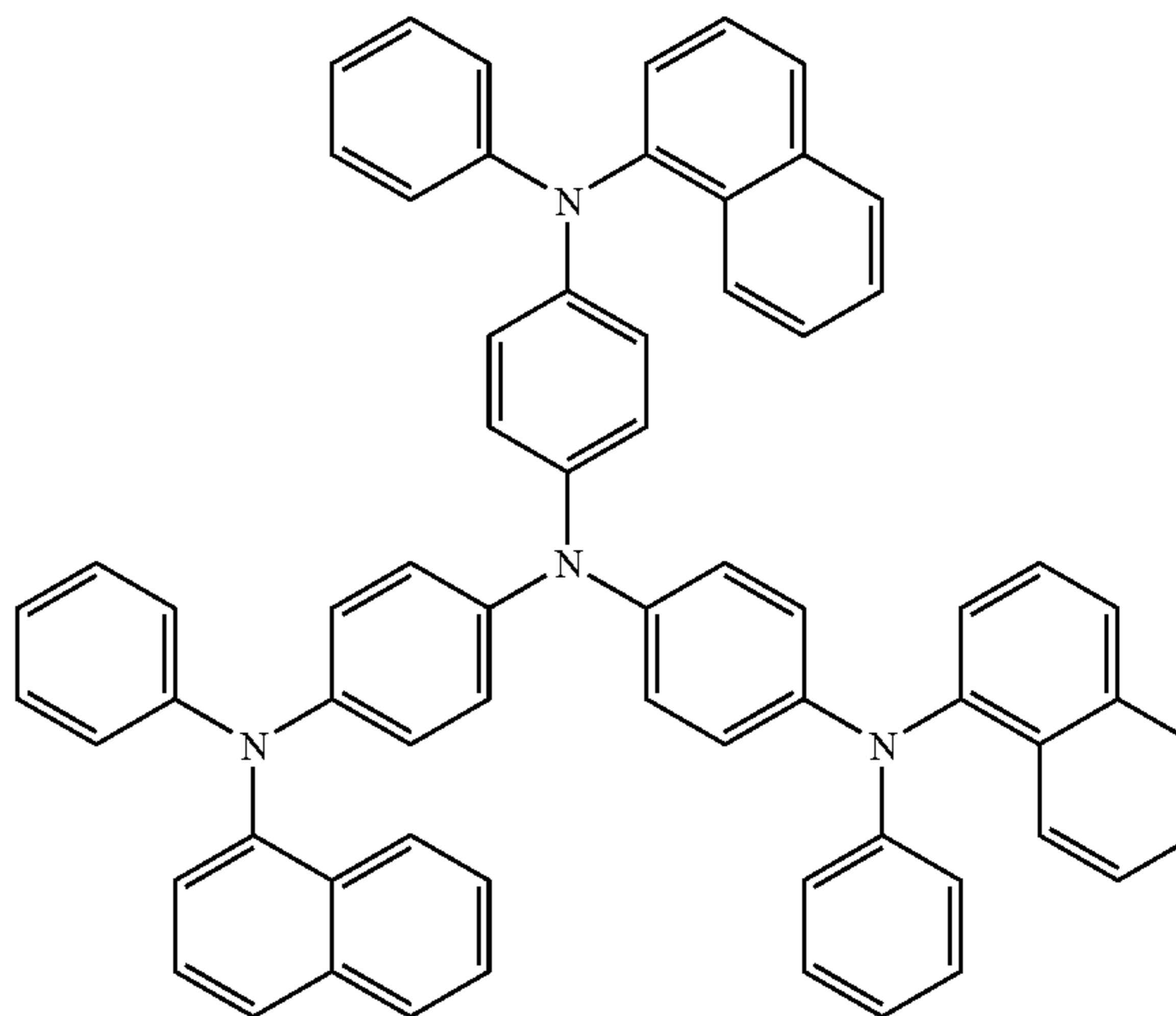
Chemical Formula 4
