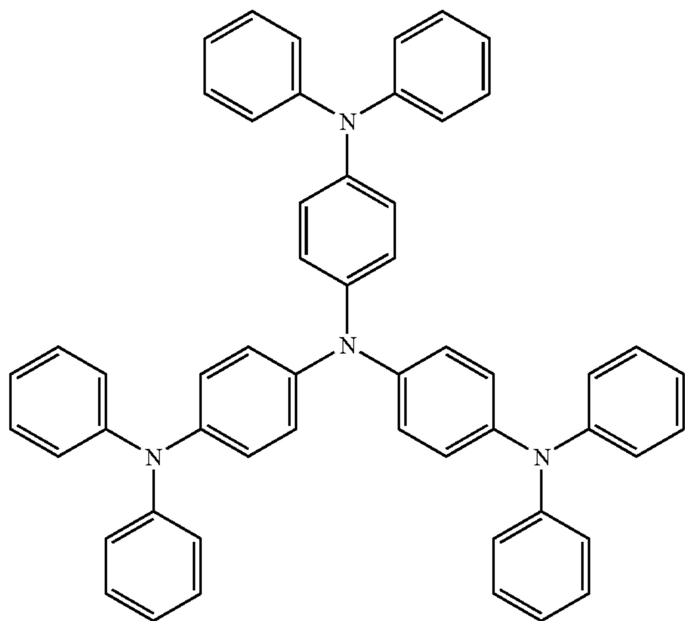
Chemical Formula 5
