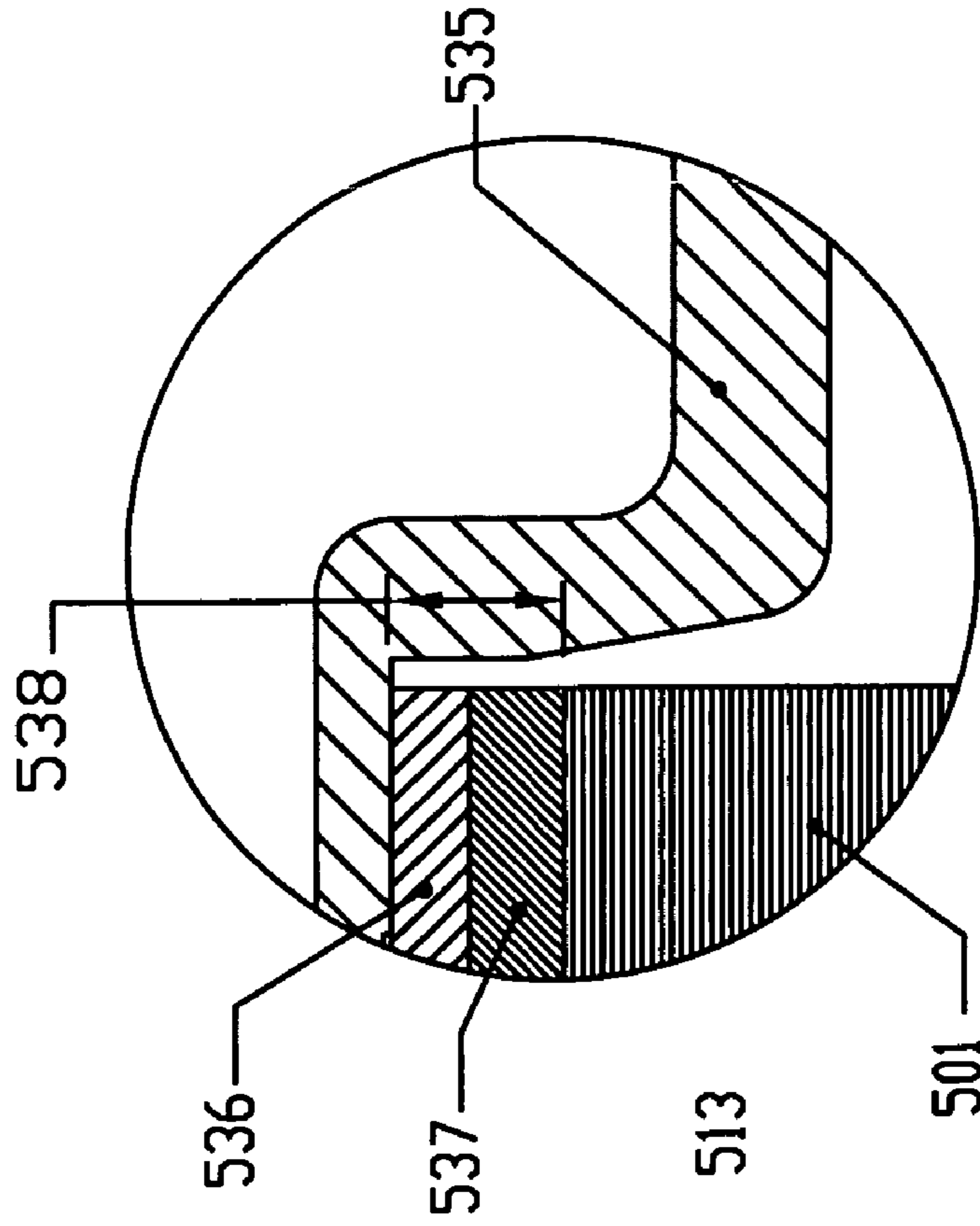
FIGURE 11 (PRIOR ART)
